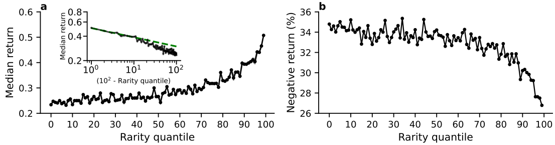
Figure F.14: High rarity leads to higher returns, and a lower chance of a negative return - Analysis without the rarest and least rare NFTs. a) Median return in USD by rarity quantile. Inset: median return against the quantity (100-q) , where q is the rarity quantile in log-log scale (black line) and the corresponding power law fit (green dashed line). b) Fraction of sales with negative return in USD by rarity quantile. This analysis was performed after discarding the 10% rarest and least rare NFTs from each collection.
