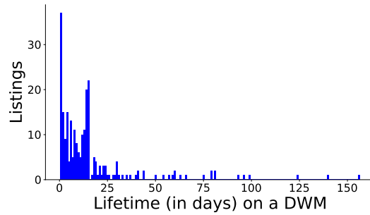
Figure B.4: Lifetime of listings on a DWM. Number of days during which listings were active on a DWM.
