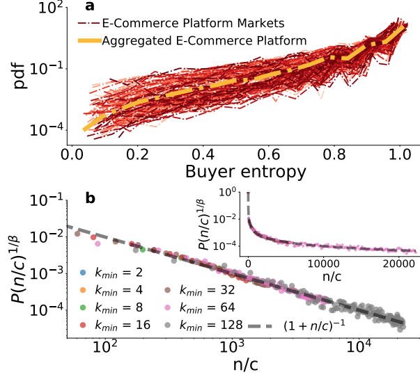
Figure 5.2: Buyer memory affects their purchase decisions. a) Normalised buyer entropy distribution for each e-commerce market (red), and the whole e-commerce platform (yellow), excluding users with zero entropy (mostly users with one transaction, see Fig. C.1) for visual clarity. The fat-tailed distributions span the full [0, 1] range, with most buyers almost equally buying from multiple sellers. b) P(n) is the probability to buy from a new seller after a buyer has already bought from n different ones. Each degree class k_{min} \leq k \leq 2 \cdot k_{min} - 1 is rescaled according to the fitted value of c and \beta (see Tab. C.1 for the values), with Eq.2 (dashed line) well reproducing the memory effect on the buyers' behaviour: the more sellers they try, the less likely they are to buy from a new one.
