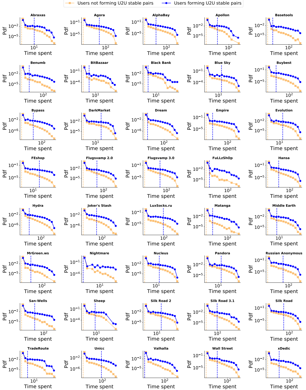
Figure E.4: Evaluation of the time users spent on a DWM. It extends Figure 7.4(inset) in the main text by considering each individual DWM. Statistical tests are carried using the two-sided Kolmogorov-Smirnov test and results are available in Table E.3. Vertical lines represent median values of the respective distributions.
