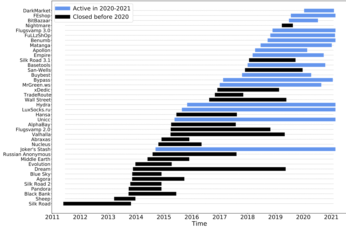
Figure E.1: Lifetime of DWMs in our dataset. Time interval between the first and last transaction of each DWM. A total of 17 DWMs participated in at least one transactions in either 2020 or 2021, while 23 closed before 2020.
