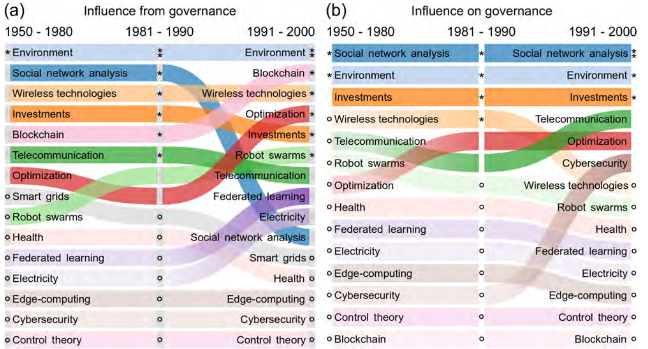
Figure D.8: The influence from/on Governance with regards to the rest of the (de)centralization literature. (a) Change of the ranking of the clusters most influenced by the Governance literature between its early period (1950-1980), its middle period (1981-1990), and its late period (1991-2000), calculated using the average knowledge flows K_{a \rightarrow b}(T) , where T is the selected period, and a is fixed to Governance. (b) Change of the ranking of the most influential clusters on the Governance literature between its early period (1950-1980), its middle period (1981-1990), and its late period (1991-2000), calculated using the average knowledge flows K_{a \rightarrow b}(T) , where T is the selected period, and b is fixed to Governance. In both cases, if K_{a \rightarrow b}(T) = 0 , we print a circle in the corresponding gray node and use a lighter color in the respective link. Moreover, we print a star when 0.01 < K_{a \rightarrow b}(T) \leq 0.1 , and two stars when K_{a \rightarrow b}(T) > 0.1 .
