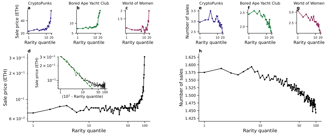
Figure F.7: Rare NFTs have a higher financial value and circulate less on the marketplace - Price in ETH. Median sale price in ETH (a-c) and average number of sales (e-g) by rarity quantile (with 20 quantiles considered) for three collections: CryptoPunks (a and e), Bored Ape Yacht Club (b and f), and World Women (c and g). d) Median sale price by rarity quantile (with 100 quantiles considered) considering all collections. Inset: median sale price against the quantity (100-q) , where q is the rarity quantile, in log-log scale (black line) and the corresponding power law fit (green dashed line). h) Median number of sales by rarity quantile considering all collections.
