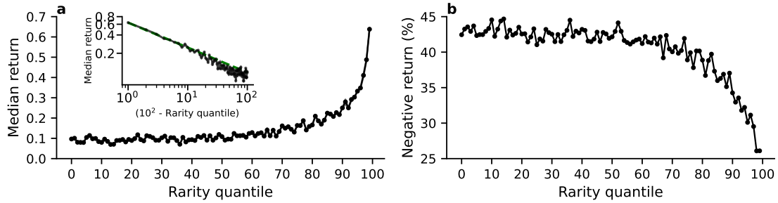
Figure F.12: High rarity leads to higher returns, and a lower chance of a negative return - Analysis on Q4 2021. a) Median return in USD by rarity quantile. Inset: median return against the quantity (100-q) , where q is the rarity quantile in log-log scale (black line) and the corresponding power law fit (green dashed line). b) Fraction of sales with negative return in USD by rarity quantile. This analysis only takes into consideration the sales happening during Q4 2021.
