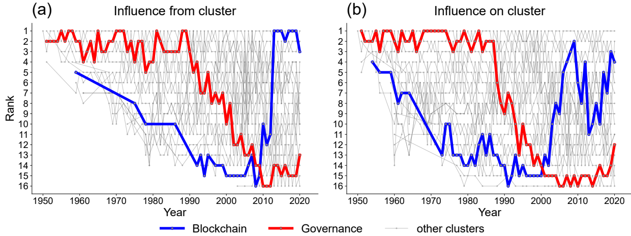
Figure 6.3: Ranking the influence of Blockchain and Governance in the (de)centralization literature. (a) Ranking in time of the influence coming from a cluster in the 3 rd hierarchical level, computed on the average knowledge flow K_{a \rightarrow \bullet}(Y) from papers in cluster a published in the year Y towards all other future papers. (b) Ranking in time of the influence to a cluster in the 3 rd hierarchical level, computed on the average knowledge flow K_{\bullet \rightarrow a}(Y) from papers published in the year Y towards future papers in cluster a . The blockchain cluster, highlighted in blue, has become a central actor in the recent literature on (de)centralization , supplanting the governance cluster, highlighted in red.
