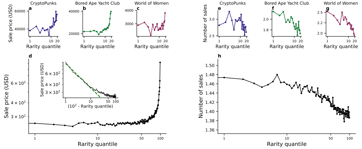
Figure F.13: Rare NFTs have a higher financial value and circulate less on the marketplace - Analysis without the rarest and least rare NFTs. Median sale price in USD (a-c) and average number of sales (e-g) by rarity quantile (with 20 quantiles considered) for three collections: CryptoPunks (a and e), Bored Ape Yacht Club (b and f), and World Women (c and g). d) Median sale price by rarity quantile (with 100 quantiles considered) considering all collections. Inset: median sale price against the quantity (100-q) , where q is the rarity quantile, in log-log scale (black line) and the corresponding power law fit (green dashed line). h) Median number of sales by rarity quantile considering all collections. This analysis was performed after discarding the 10% rarest and least rare NFTs from each collection.
