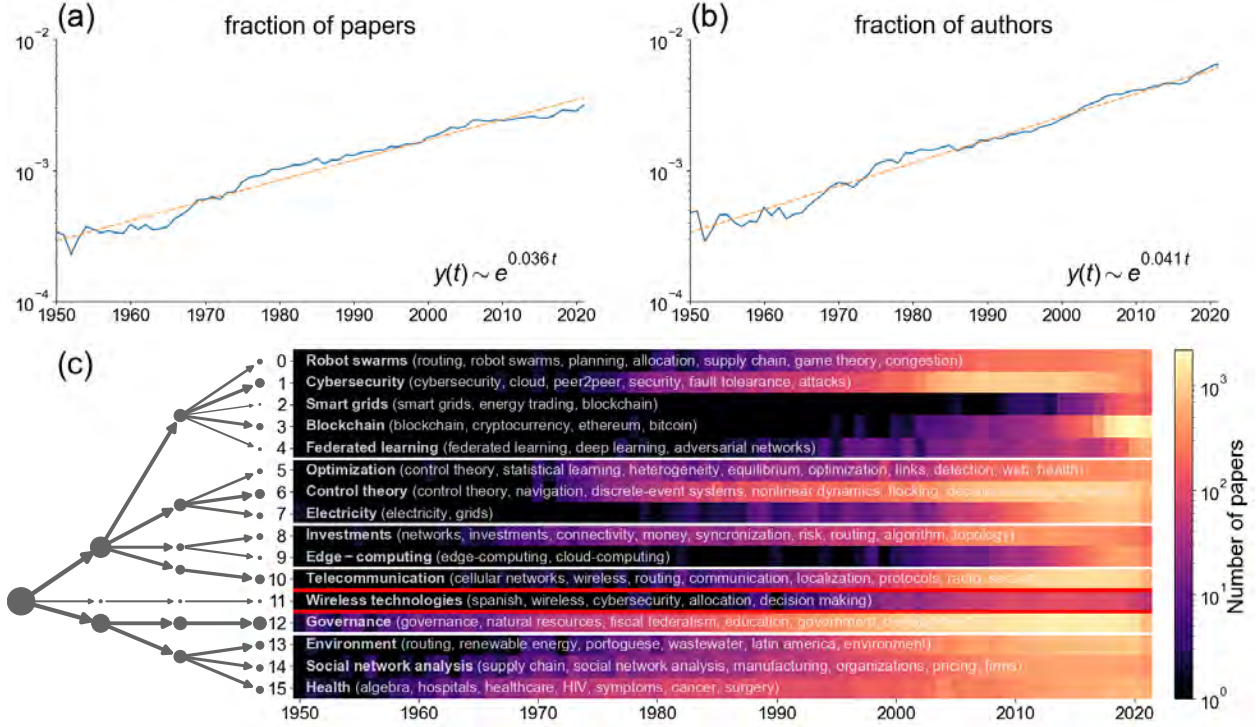
Figure 6.1: The rising interest of academic literature towards (de)centralization . (a) Fraction of papers mentioning (de)centralization in the Semantic Scholar corpus. (b) Fraction of authors mentioning (de)centralization in the Semantic Scholar corpus. Both fractions have been steadily increasing since the 1950s, showing growing interest in the topic. (c) Number of papers in the clusters at the 3 rd level of the hierarchy in each year. Clusters are ordered respecting the hierarchical network on the left, in which node and link sizes are proportional to the total number of papers in the related cluster. In the heatmap, white lines individuate clusters belonging to the same cluster at the 2 nd level of the hierarchy, while red lines divide different clusters at the 1 st level. The representative keyword of the clusters at level 3 is reported in bold in the respective rows, while all the specific keywords identified at the 4 th hierarchical level are shown within brackets. Clusters with less than 500 papers in total are not shown in the figure.
