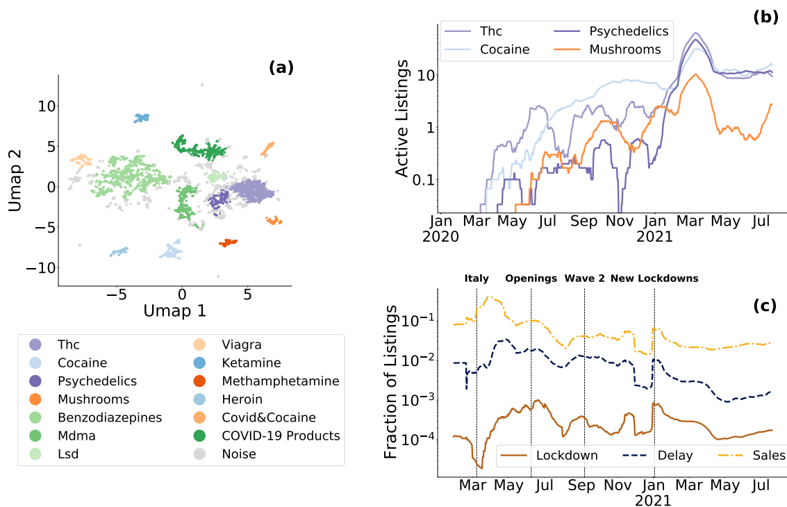
Figure 4.4: Characterization of COVID-19 mentions. (a) UMAP representation of doc2vec embeddings. hDBSCAN clustering finds 13 meaningful categories covering COVID-19 related products and all major drugs sold on DWMs. (b) 30-day rolling average of active listings in 4 categories of listings mentioning COVID-19: thc , psychedelics , cocaine , and mushrooms . (c) 30-day rolling average of fraction of previously identified drugs listings mentioning 3 different COVID-19 related themes: lockdowns, shipping delays and sales, with key pandemic events highlighted with vertical dashed black lines.
