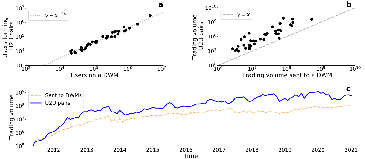
Figure 7.2: User-DWM and U2U transactions. (a) Total number of users interacting with a DWM against the total number of them forming U2U transactions. The dotted line corresponds to the result of a fitted power law function. (b) Trading volume in dollars sent to a DWM compared with the total trading volume in its surrounding U2U transactions. The dashed line is the bisector and allows to easily compare the two trading volumes. (c) Total monthly trading volume sent to all DWMs and exchanged in all unique U2U pairs. We do not include the trading volume received from DWMs because it is equivalent to the volume sent to DWMs.
