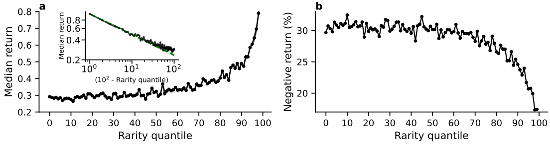
Figure F.10: High rarity leads to higher returns, and a lower chance of a negative return - Analysis on Q3 2021. a) Median return in USD by rarity quantile. Inset: median return against the quantity (100-q) , where q is the rarity quantile in log-log scale (black line) and the corresponding power law fit (green dashed line). b) Fraction of sales with negative return in USD by rarity quantile. This analysis only takes into consideration the sales happening during Q3 2021.
