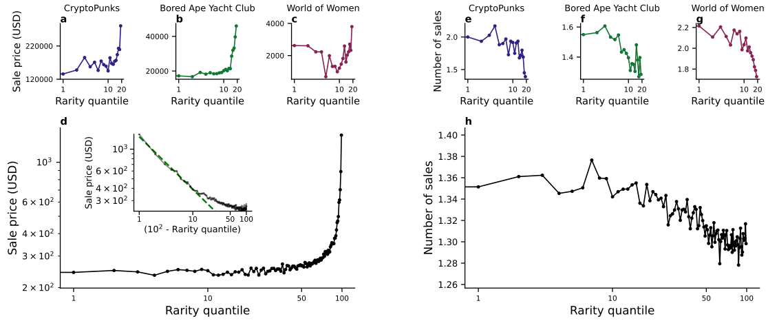
Figure F.9: Rare NFTs have a higher financial value and circulate less on the marketplace - Analysis on Q3 2021. Median sale price in USD (a-c) and average number of sales (e-g) by rarity quantile (with 20 quantiles considered) for three collections: CryptoPunks (a and e), Bored Ape Yacht Club (b and f), and World Women (c and g). d) Median sale price by rarity quantile (with 100 quantiles considered) considering all collections. Inset: median sale price against the quantity (100-q) , where q is the rarity quantile, in log-log scale (black line) and the corresponding power law fit (green dashed line). h) Median number of sales by rarity quantile considering all collections. This analysis only takes into consideration the sales happening during Q3 2021.
