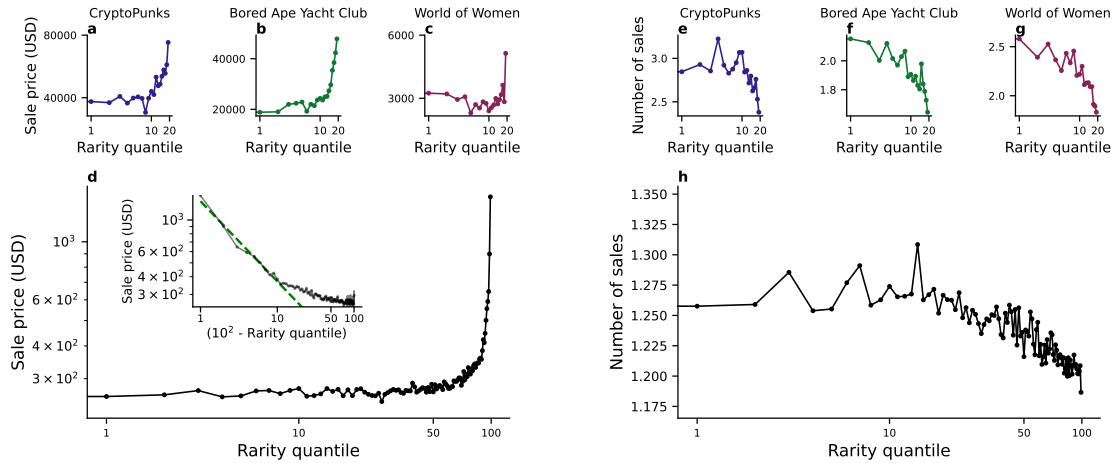
Figure F.11: Rare NFTs have a higher financial value and circulate less on the marketplace - Analysis on Q4 2021. Median sale price in USD (a-c) and average number of sales (e-g) by rarity quantile (with 20 quantiles considered) for three collections: CryptoPunks (a and e), Bored Ape Yacht Club (b and f), and World Women (c and g). d) Median sale price by rarity quantile (with 100 quantiles considered) considering all collections. Inset: median sale price against the quantity (100-q) , where q is the rarity quantile, in log-log scale (black line) and the corresponding power law fit (green dashed line). h) Median number of sales by rarity quantile considering all collections. This analysis only takes into consideration the sales happening during Q4 2021.
