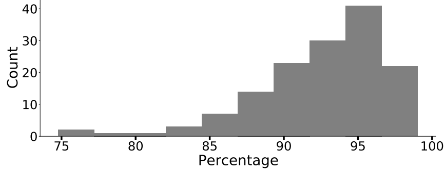
Figure C.1: Most buyers with zero entropy only have done one transaction. Histogram of percentage of buyers doing just one transaction for each e-commerce product market, among those with zero entropy. In most markets the percentage is well above 90%.
