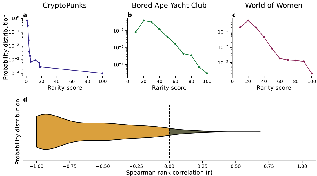
Figure 8.5: Rare NFTs are scarce within a collection. a-c) Distribution of the rarity score of the NFTs within three collections: CryptoPunks (a), Bored Ape Yacht Club (b), and World of Women (c). d) Violin plot of the Spearman Rank correlation computed between the rarity score and the number of NFTs with that score. 96% of the collections have a Spearman rank r \leq 0 (black dashed lines).
