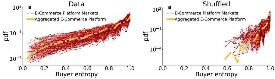
Figure C.2: The entropy distribution is significant against a null model. (a) Buyer entropy distribution for each market (red) and all markets (yellow) in the e-commerce datasets. (b) Same distributions build reshuffling the transaction links, such that buyers have the same number of transactions, but with random sellers. The distributions with the reshuffled data show considerably higher entropy, meaning that the buyers in the dataset show non-random effects of memory.
