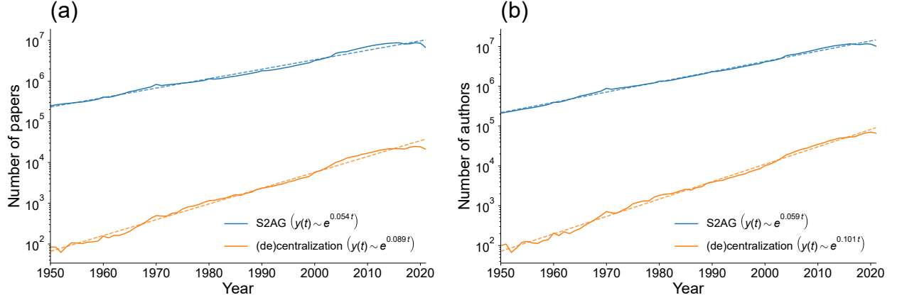
Figure D.1: Comparison of the increase in number of papers (a) and authors (b) between the whole S2AG corpus and the (de)centralization dataset. Exponential fits are shown as dashed line, with the fitted values between brackets in the legend.
