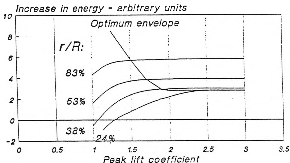
Fig 7.6 Determination of maximum useful C_L . extracted from Ref [65] ( r is local raduis, R is blade raduis).
