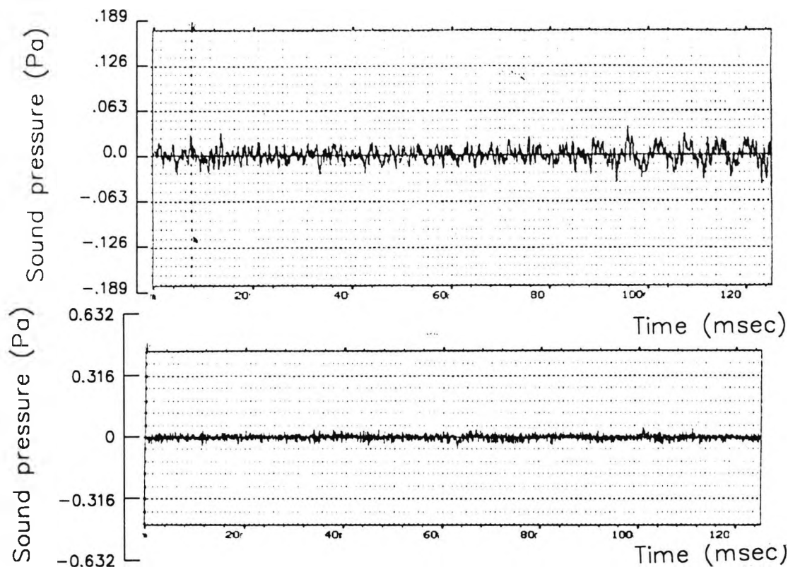
Figure 6.4 (a) Typical noise signals from the wind turbine (upper graph) and from the wind by itself (lower graph).
