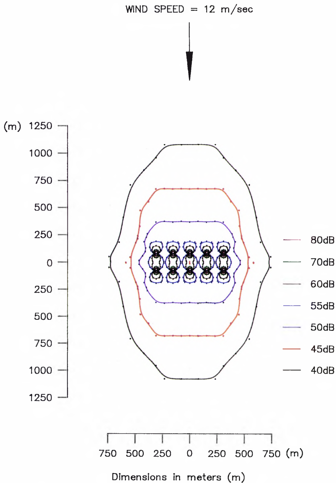
Fig 7.19 Predicted equal pressure contours for Wind Farm of 10 machines MS-1 by WTGNOISE.
