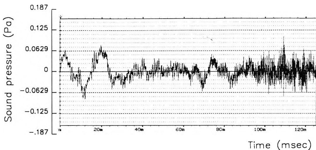
Fig 6.9 (a) Typical noise signal verses time at reference position [1], rotational speed= 200 rpm, average wind speed= 6.7 m/sec, average noise level directly measured =62 dB(A).
