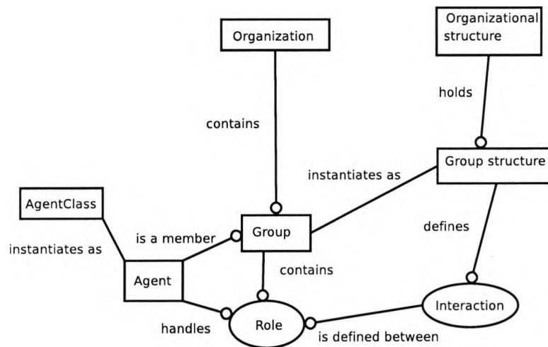
Fig. 6.1. The Agent/Group/Role model.
