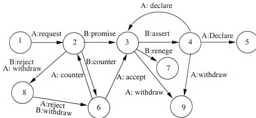
Fig. 3.2. Conversation for Action (Winograd and Flores, 1987)
