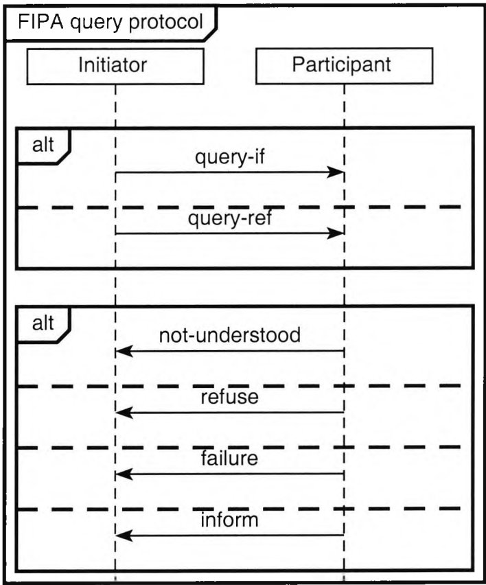
Fig. 3.1. FIPA Query Interaction Protocol
