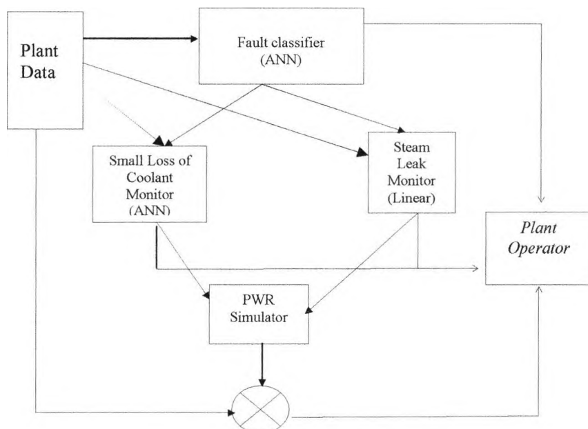
Figure 7.1 Block diagram of proposed Operators Advisory System
