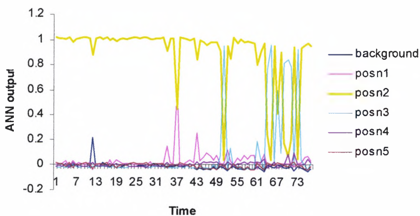
Figure 6.17 ANN output for Valve position 2
