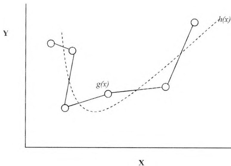
Figure 4.8 exact interpolation of a function with noise
