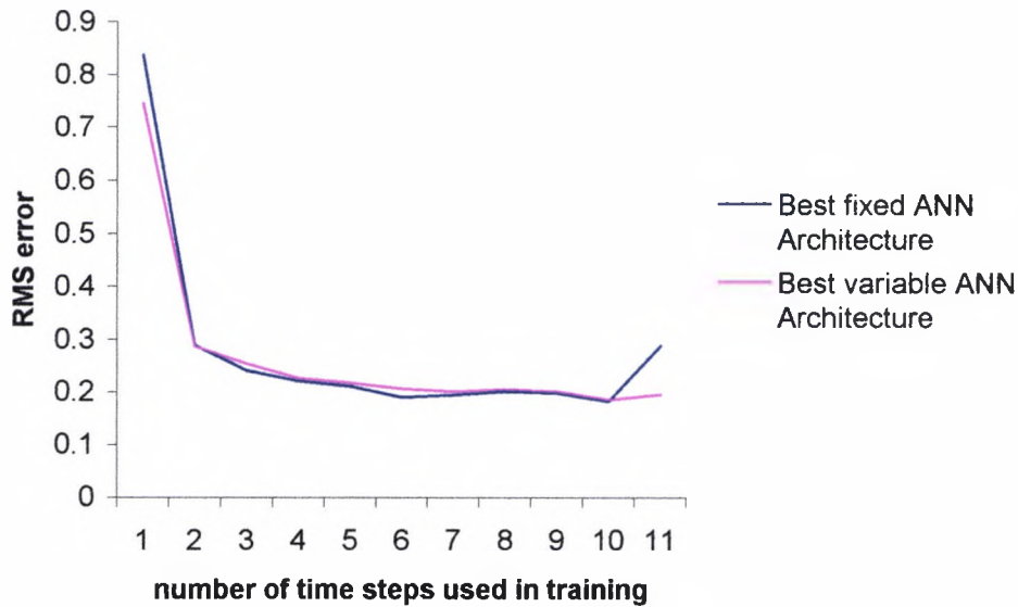
Figure 4.13 comparisons of fixed and variable ANN architectures
