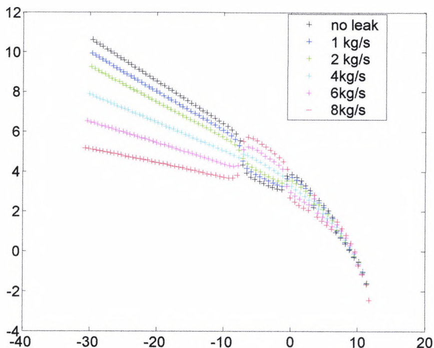
Figure 7.3 Sammon map for 5 LOCAS
