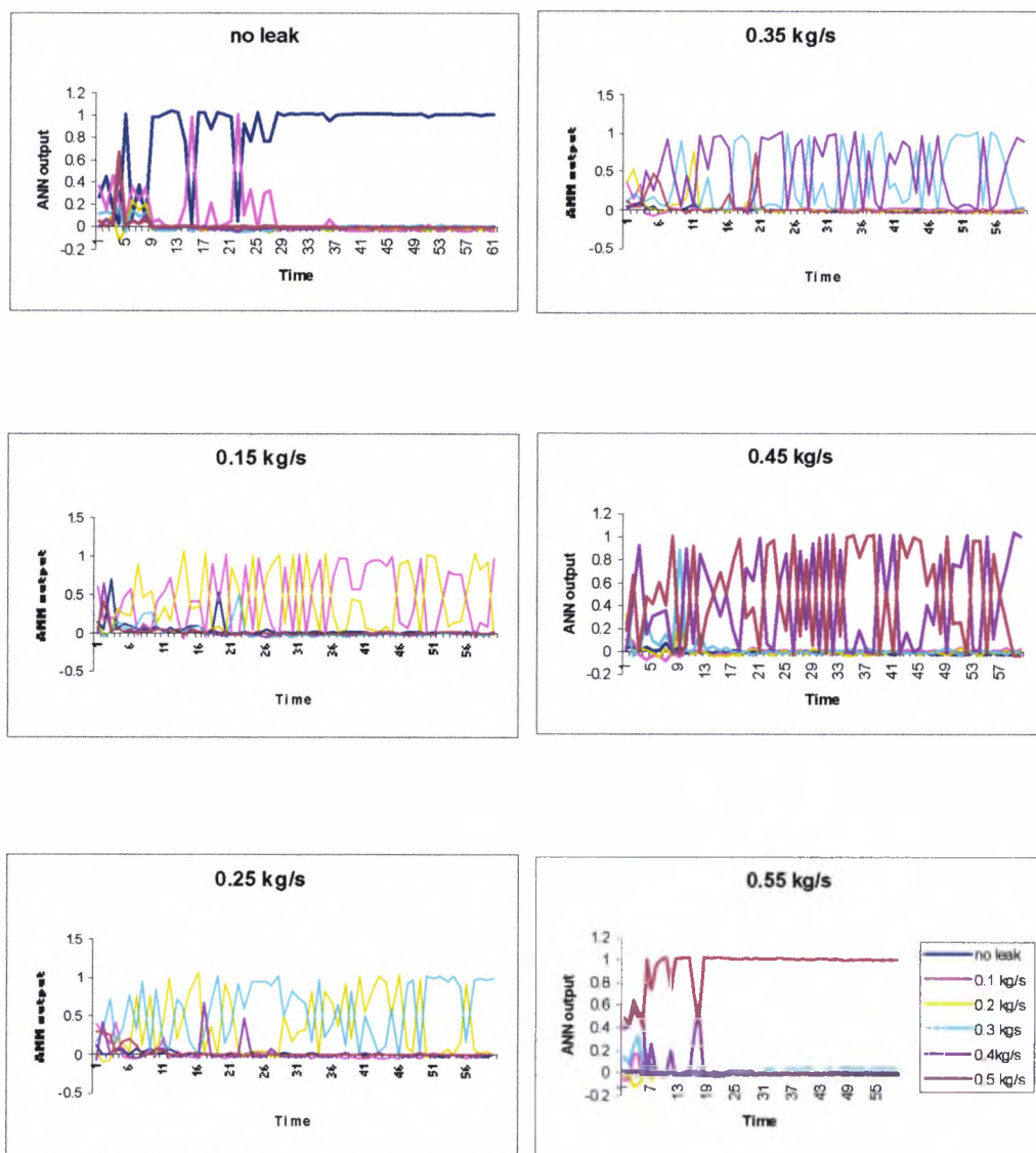
Figure 5.10 ANN results for intermediate LOCA
