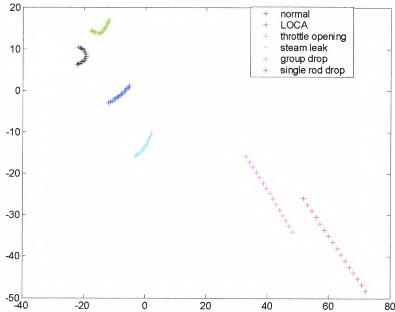
Figure 7.2 Sammon map of Major Fault Transients
