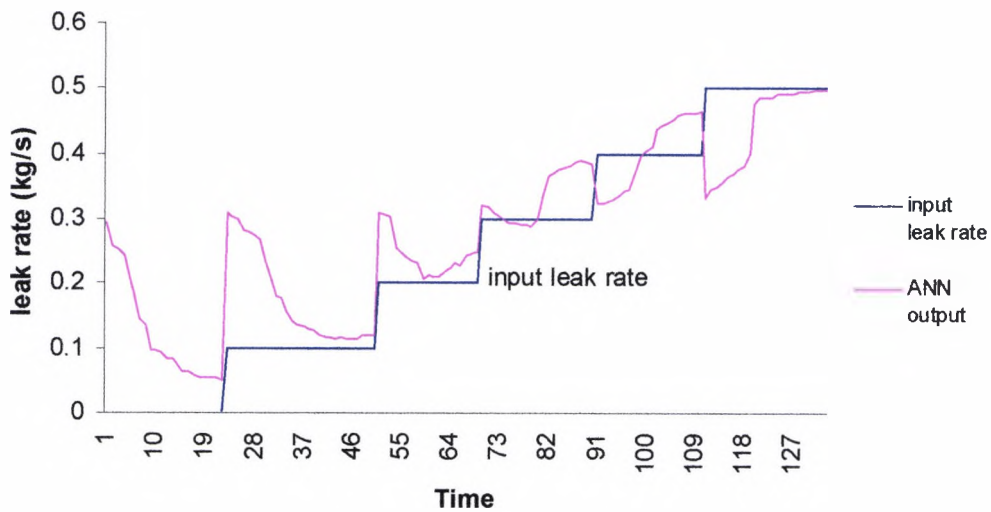
Figure 5.11 ANN results for classification of leak rate (5 times step)
