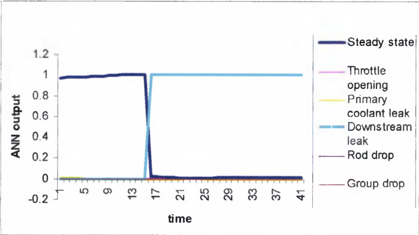
Figure 4.5 downstream leak at 60% full power
