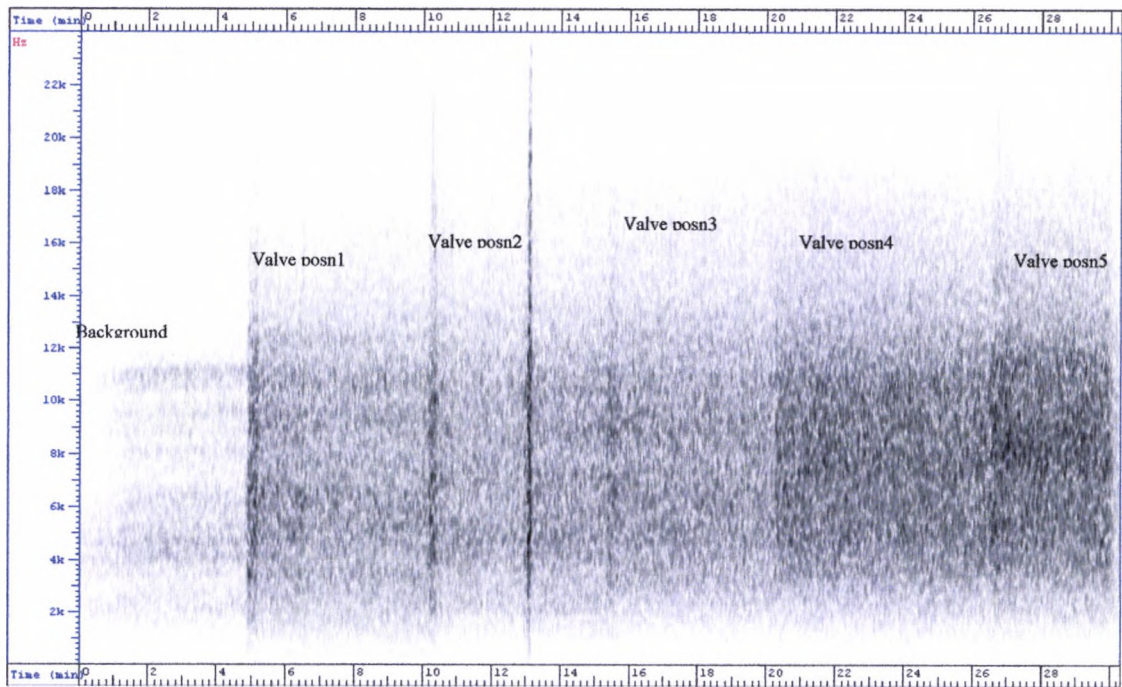
Figure 6.12 Spectrogram of steam leak recording
