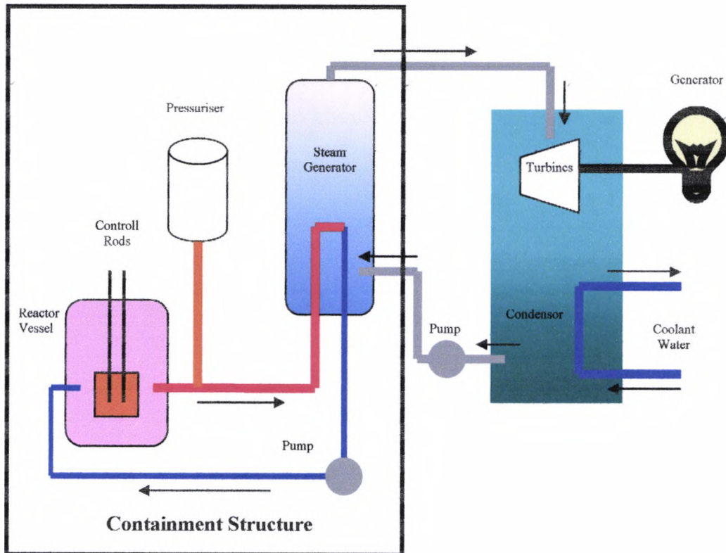
Figure 3.1 Schematic of a PWR
