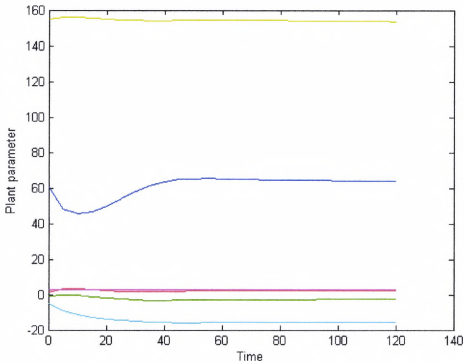
Figure 7.9 OAS trend data for a small primary coolant leak
