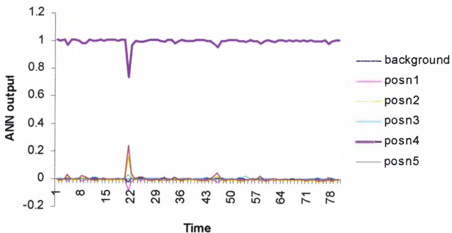
Figure 6.19 ANN output for valve position 4
