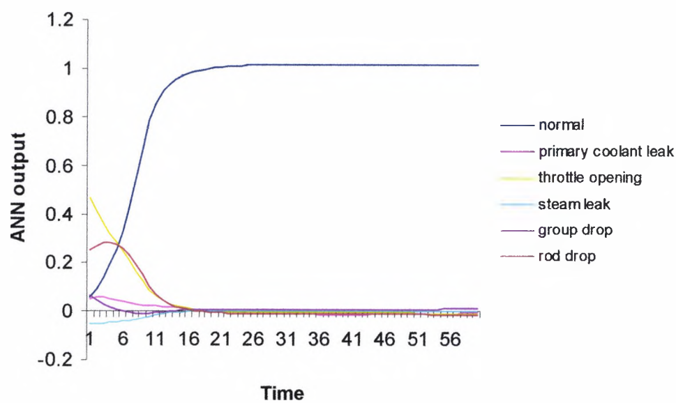
Figure 4.14 Normal Operating Conditions
