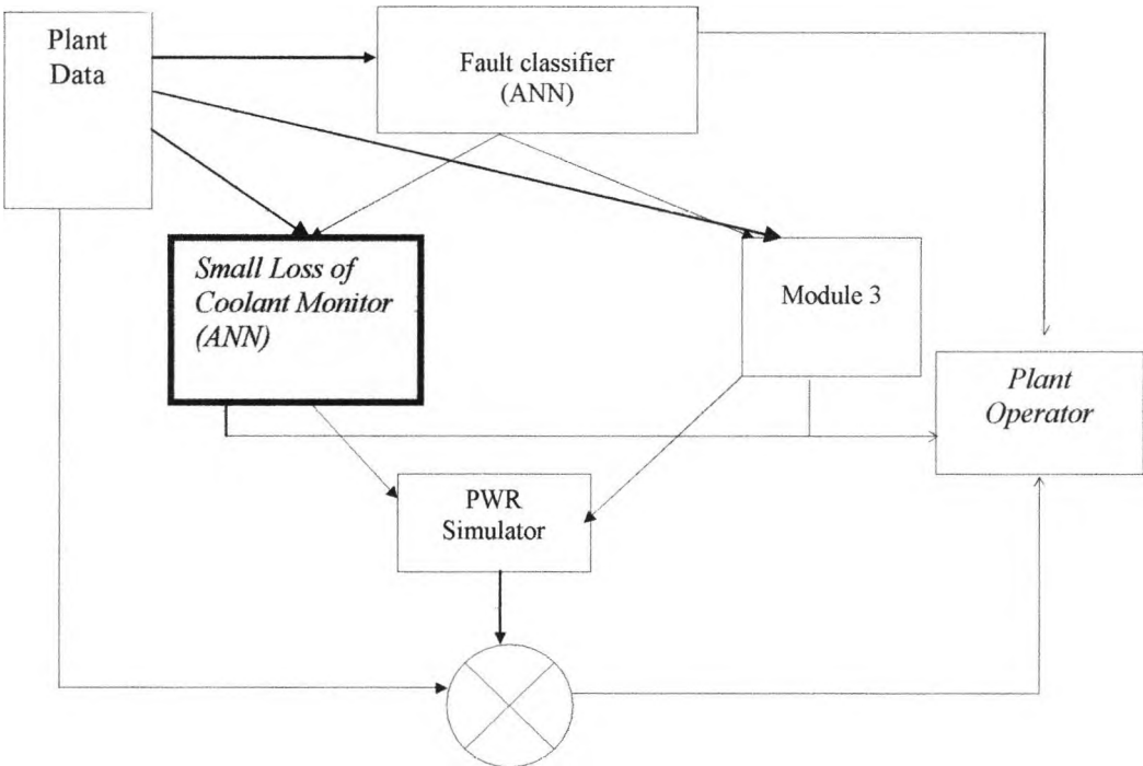
Figure 5.1 Embedded Small Loss of Coolant Monitor in OAS
