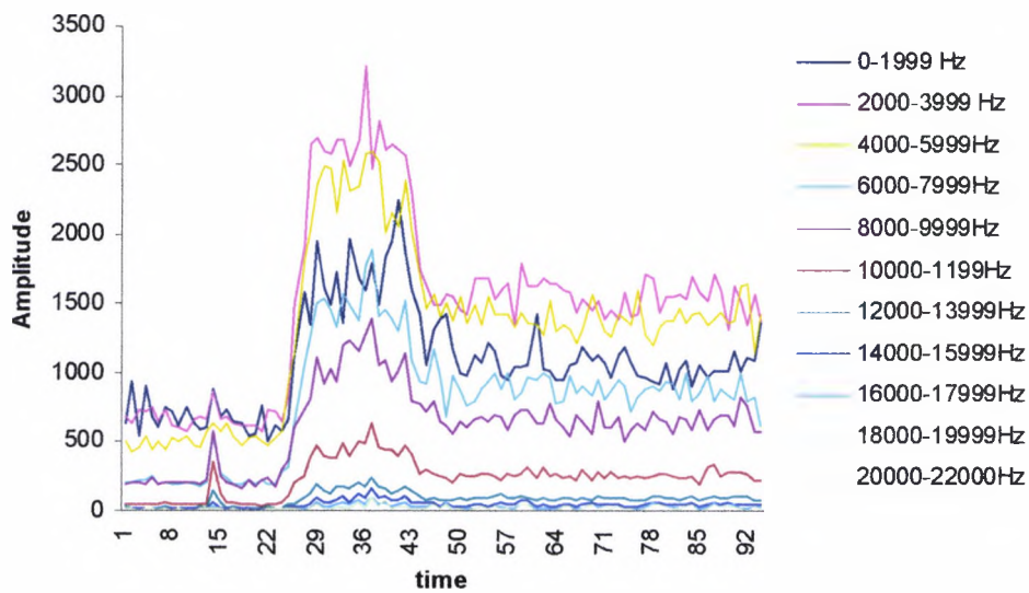
Figure 6.14 Transition from first to second valve position
