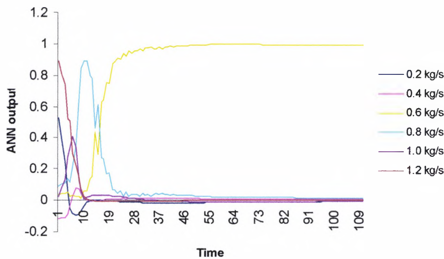
Figure 5.4: ANN output for a 0.6kg/s
