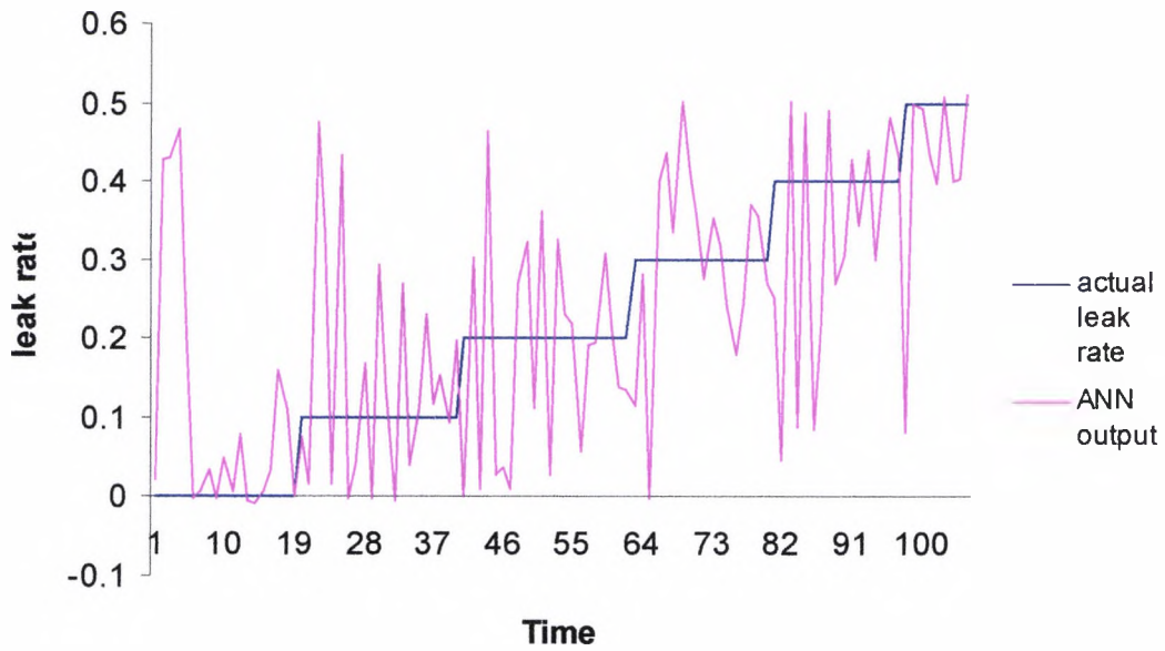
Figure 5.14 ANN results for classification of leak rate (10 times step, 5% noise)
