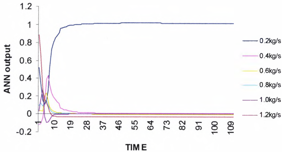
Figure 5.5 No Leak at 30% full power
