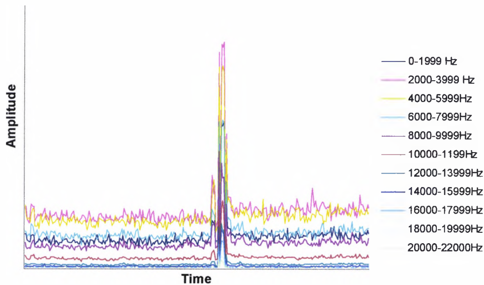
Figure 6.21 frequency bands for valve position 2
