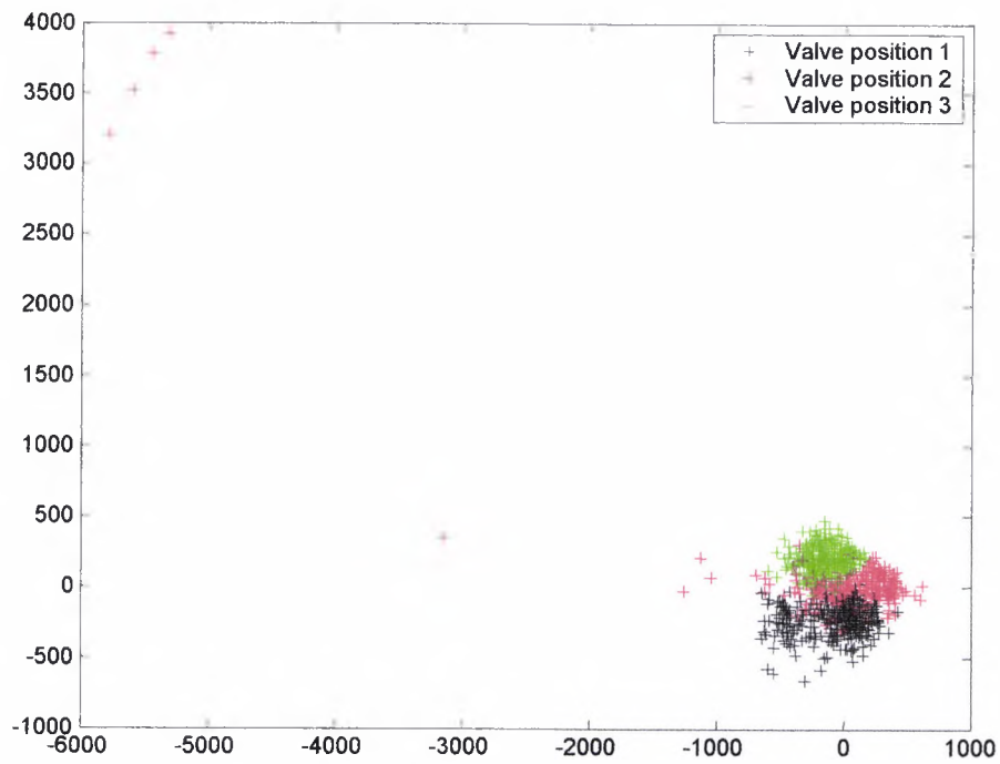
Figure 6.22 Sammon Mapping for valve positions 1,2 and 3 (With Artefact)
