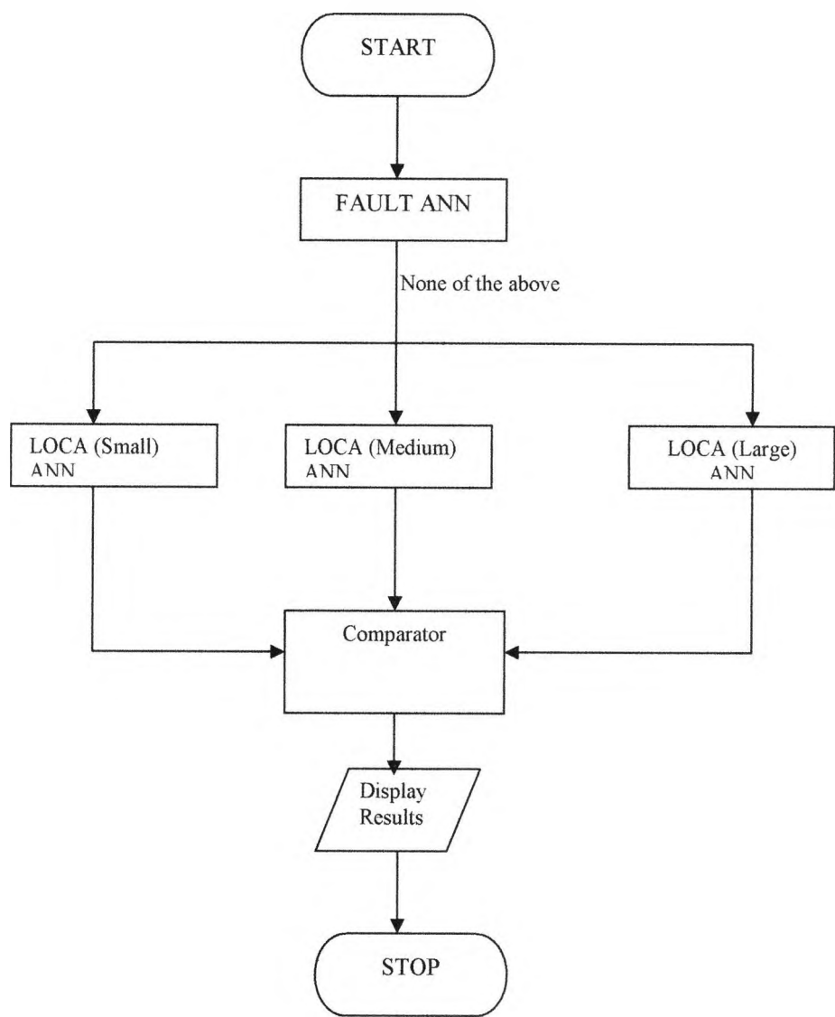
Figure 7.8 Flow diagram of LOCA Classification
