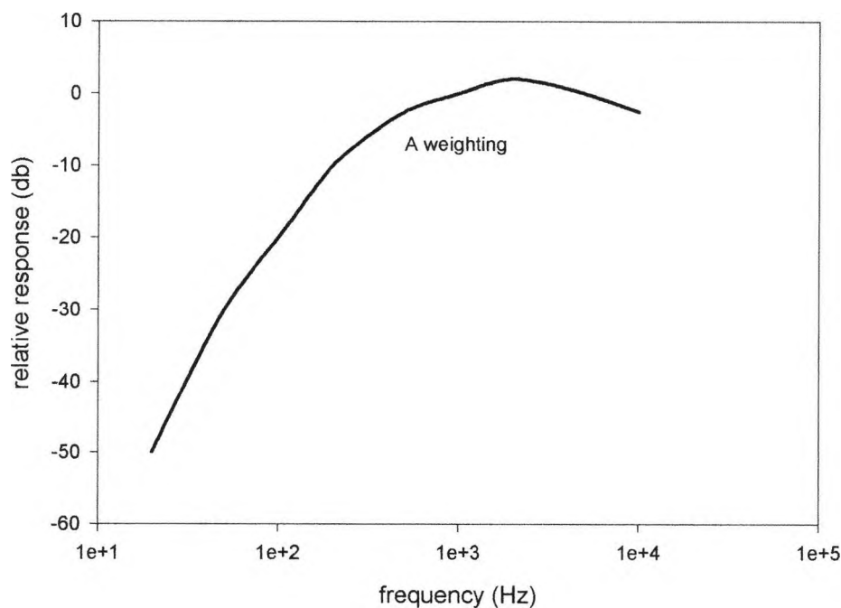
Figure 6.4 A Weighting Frequency Curve
