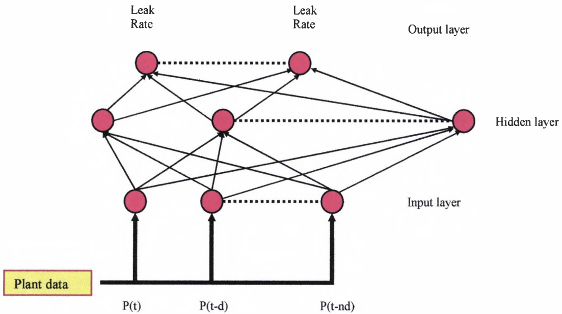
Figure 5.7 Time-Delay ANN
