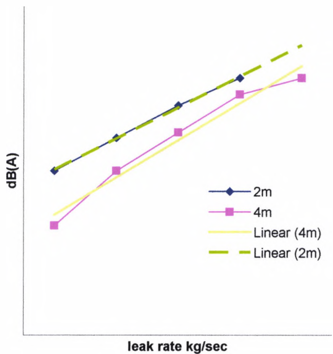
Figure 6.6 results of sound measurements
