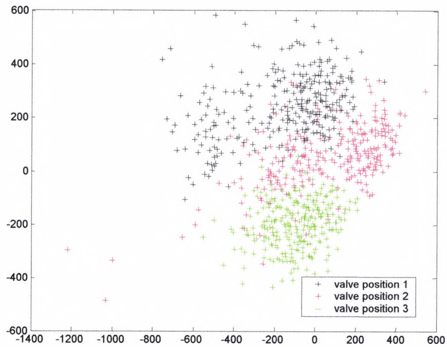
Figure 6.23 Sammon Mapping for valve positions 1,2 and 3 without artefact
