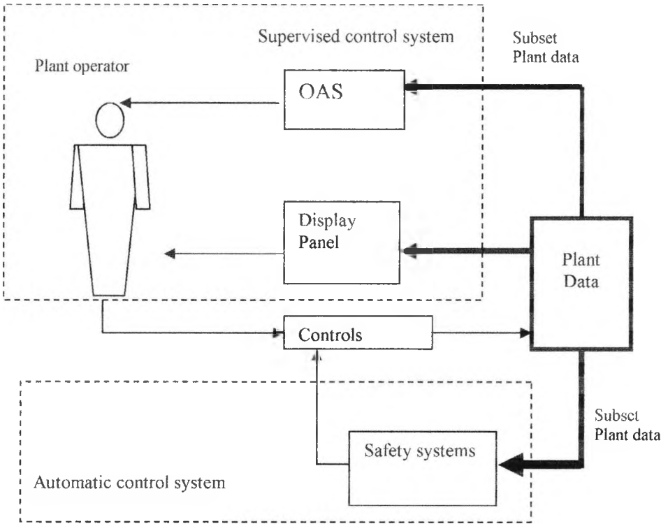
Figure 3.4 Plant Operation sub-systems
