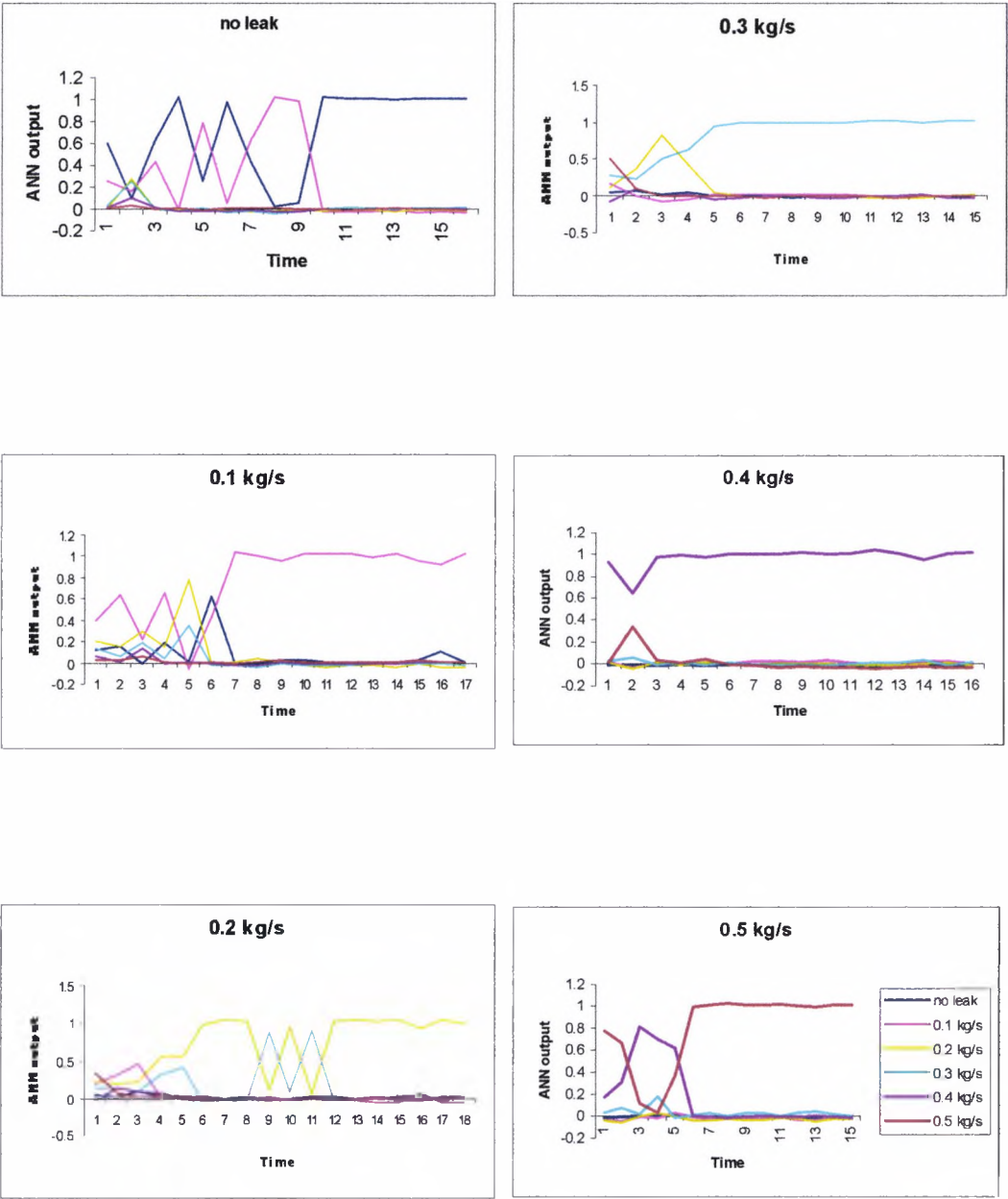
Figure 5.9 ANN results for LOCA 0-0.5 kg/s
