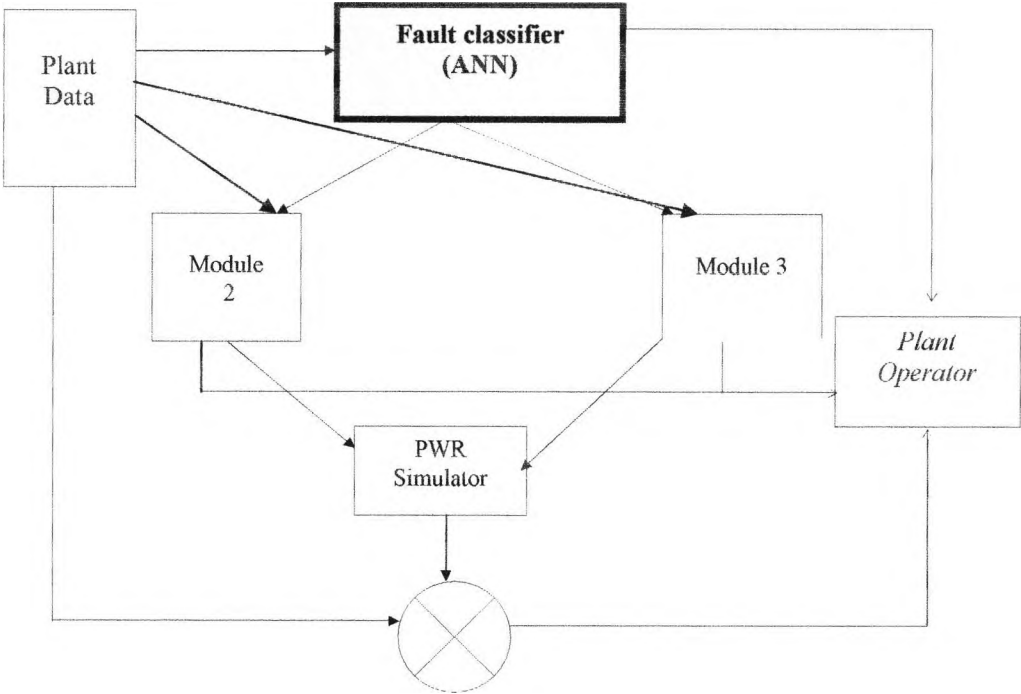
Figure 4.2 Embedded Fault classifier in proposed OAS
