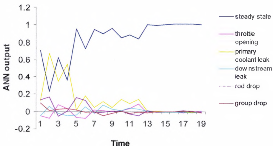
Figure 4.10 ANN output for a steady state condition with Gaussian noise added to training data set
