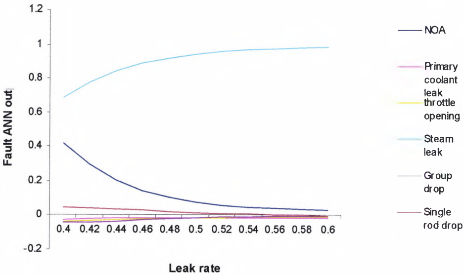
Figure 7.16 Fault ANN output for a range of downstream steam leaks
