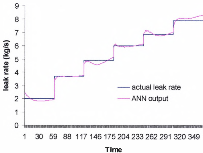
Figure 7.6 Estimation of large size leak rates
