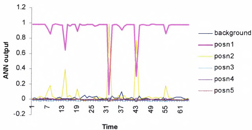
Figure 6.16 ANN output for Valve position 1
