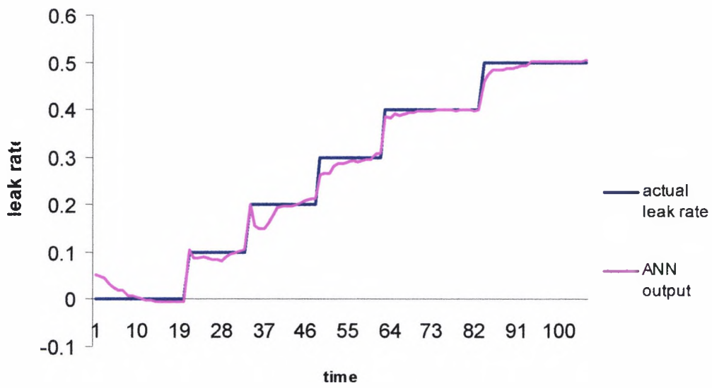
Figure 5.12 ANN results for classification of leak rate (10 times step) no noise
