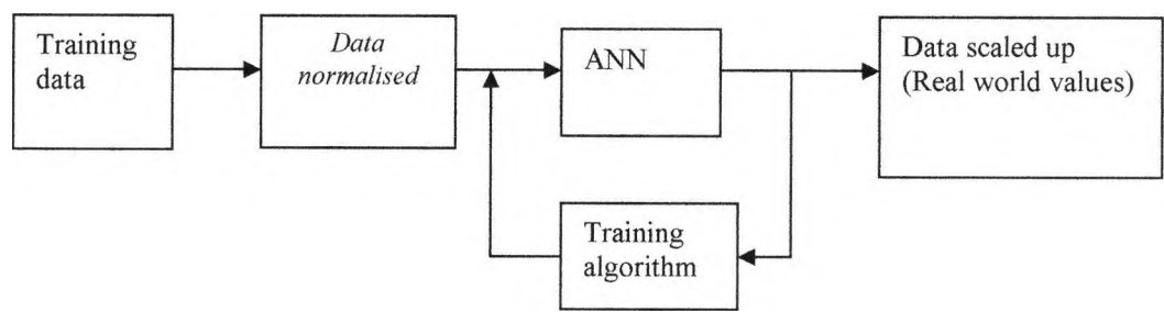
Figure 7.11 Supervised learning model
