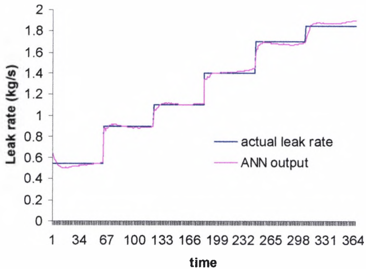
Figure 7.5 Estimation of medium size leak rates
