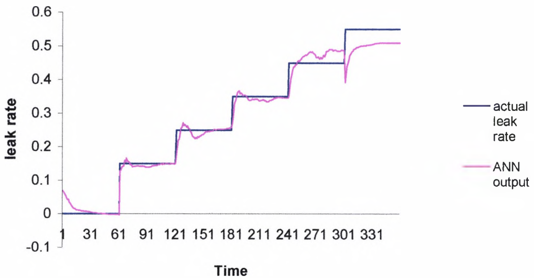
Figure 5.15 ANN results for classification for intermediate leak rate
