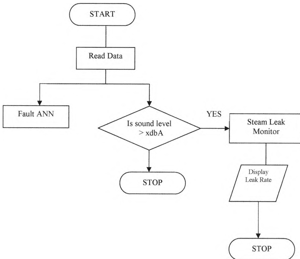
Figure 7.15 Implementation of Steam leak Monitor
