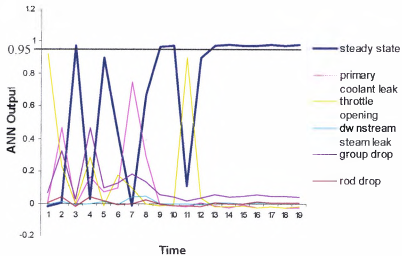
Figure 4.6 ANN Output for a steady state condition with 2% Gaussian noise in validation set
