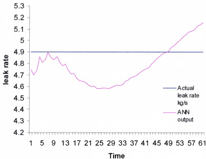
Figure 7.7 Estimation of a leak rate of 4.9 kg/s
