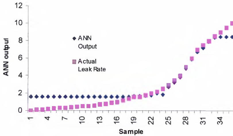
Figure 7.14 Estimated leak rate
