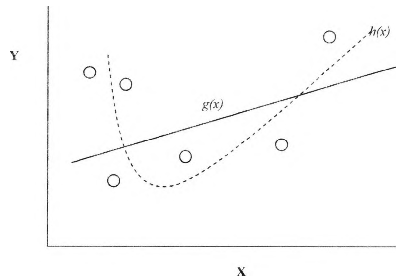
Figure 4.7 fixed function approximation of a function with noise
