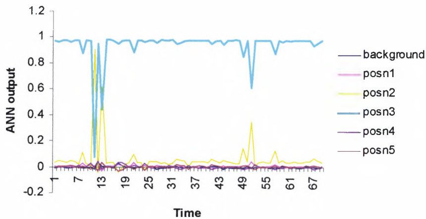
Figure 6.18 ANN output for Valve position 3
