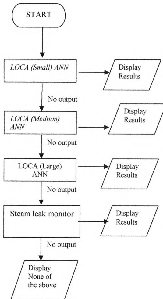
Figure 7.18 Flow diagram for Steam leak Monitor in OAS
