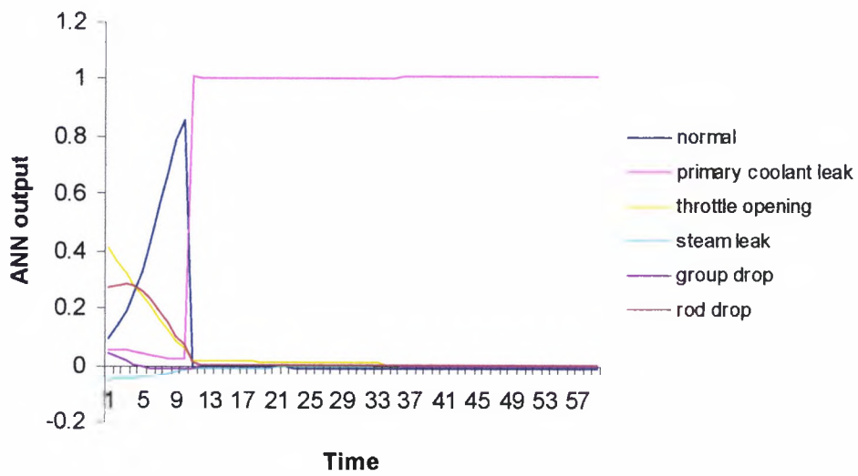
Figure 4.15 Primary Coolant Leak Transient
