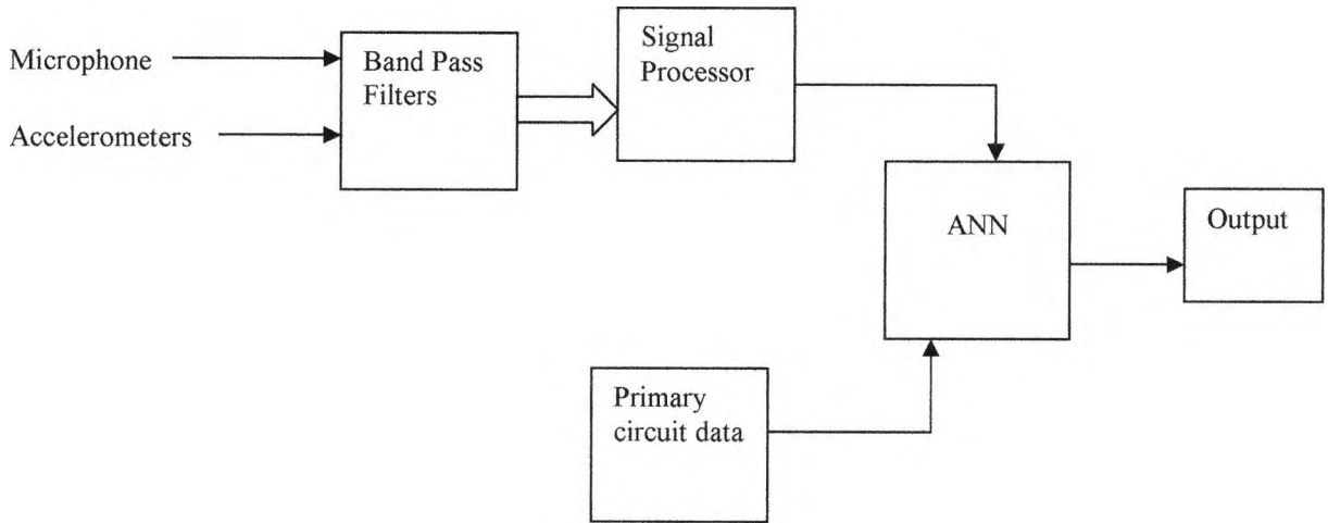
Figure 6.24 Possible acoustic Neural Net Monitor
