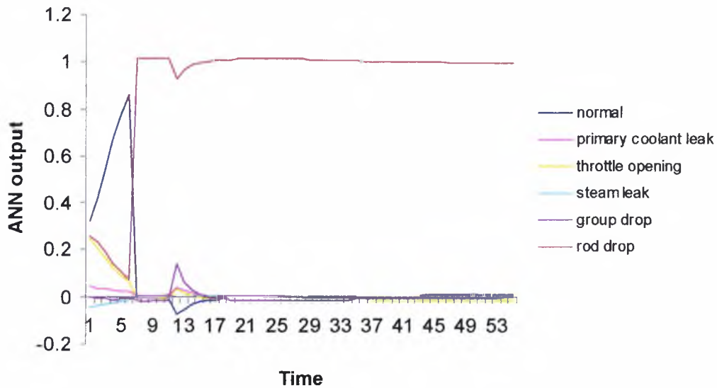
Figure 4.19 Single Rod Drop Transient
