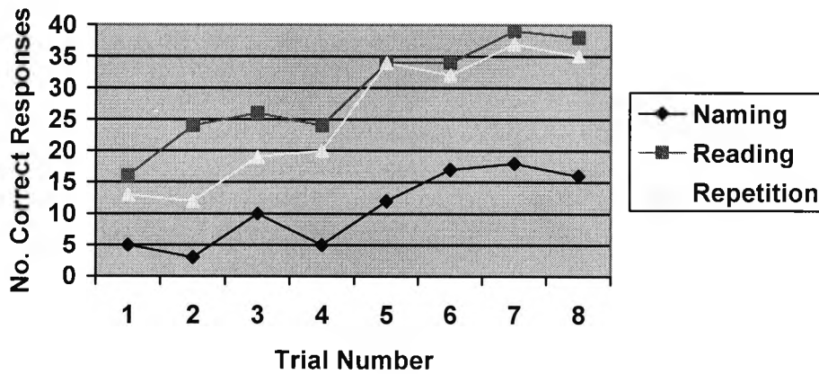
Figure 9.1: TK: Change over Time on Noun Tasks
