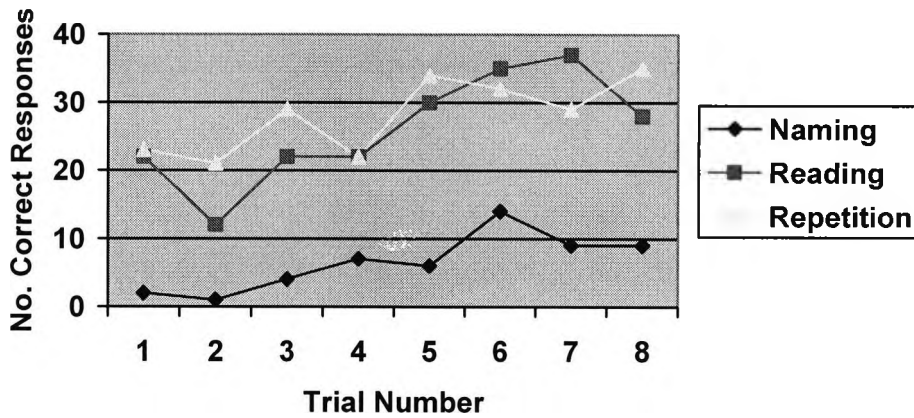
Figure 9.2: TK: Change over Time on Verb Tasks
