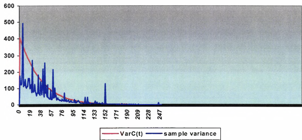
Figure 6.3: VarC(t) vs Sample Variance, spread period = 25 years, \sigma_{\lambda} = 0.1
