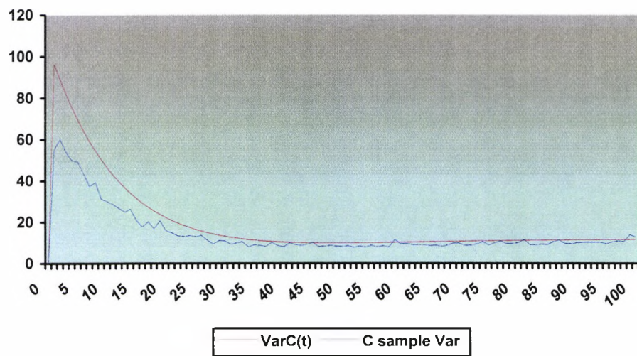
Figure 6.5: \text{VarC}(t) vs Sample Variance, \sigma_i = \sigma_\lambda = 0.05
