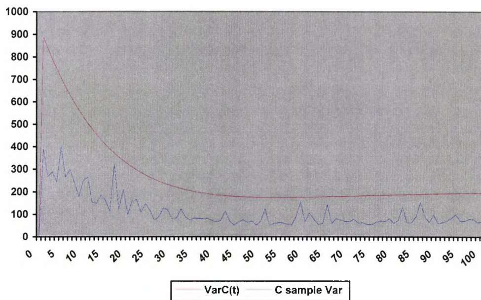
Figure 6.7: VarC(t) vs Sample Variance, \sigma_i = 0.1 and \sigma_\lambda = 0.15
