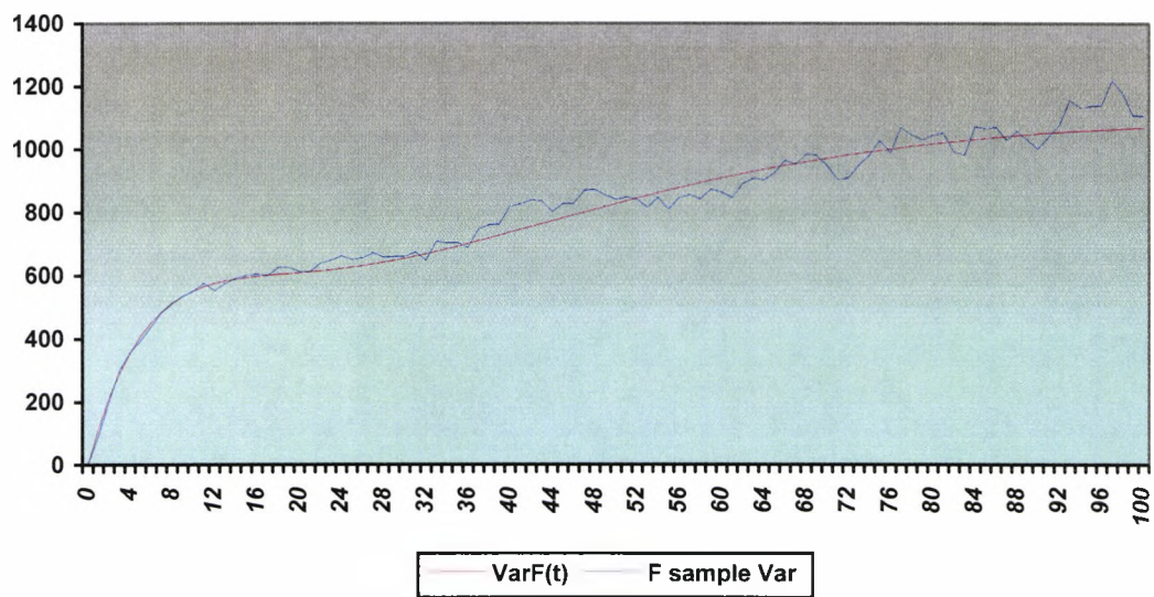
Figure 6.4: \text{VarF}(t) vs Sample Variance, \sigma_i = \sigma_\lambda = 0.05
