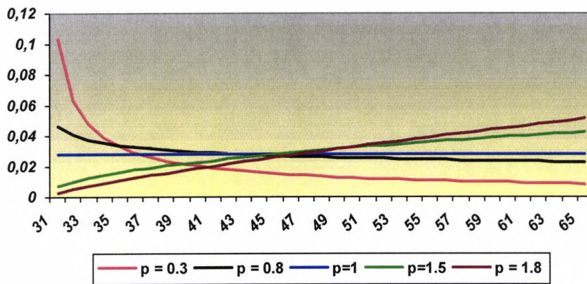
Figure 3.1 m(x) s development under the different Power function parameter values
