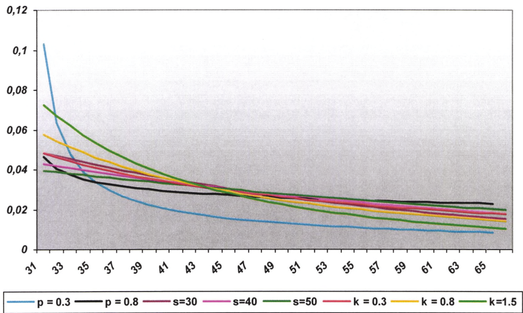
Figure 3.7 m(x) s development under the different distributions parameter values
