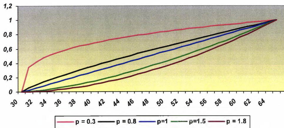
Figure 3.2 M(x) s development under the different Power function parameter values
