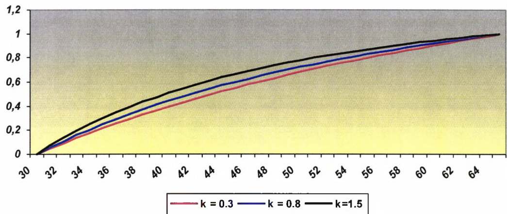
Figure 3.4 M(x) s development under the different Truncated Pareto parameter values
