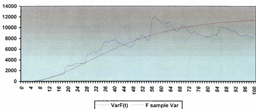
Figure 6.2: VarF(t) vs Sample Variance, E(i(t)) = 0.05 , \sigma_i = 0.15
