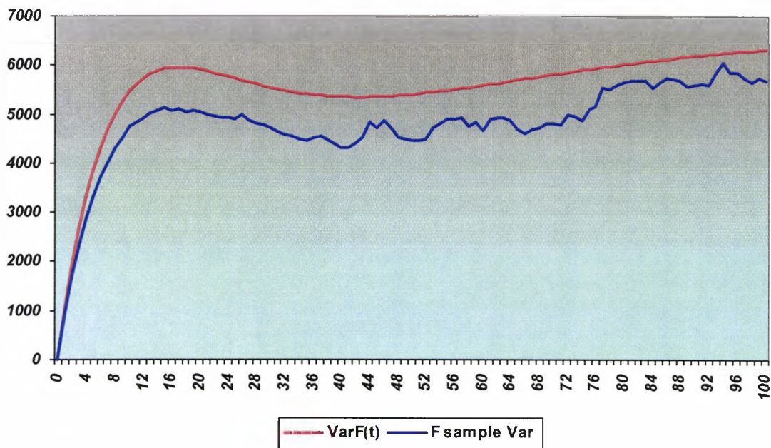
Figure 6.6: VarF(t) vs Sample Variance, \sigma_i = 0.1 and \sigma_\lambda = 0.15
