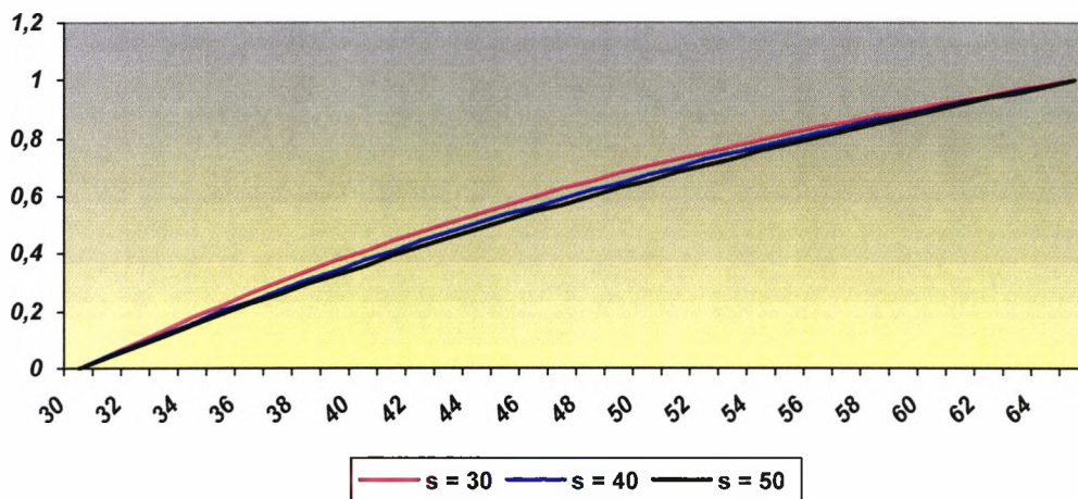
Figure 3.6 M(x) s development under the different Truncated Exponential parameter values
