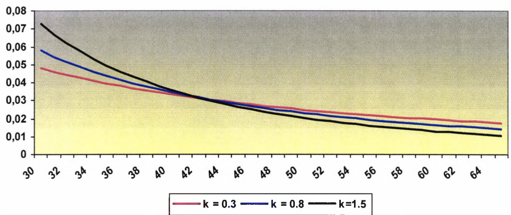
Figure 3.3 m(x) s development under the different Truncated Pareto parameter values
