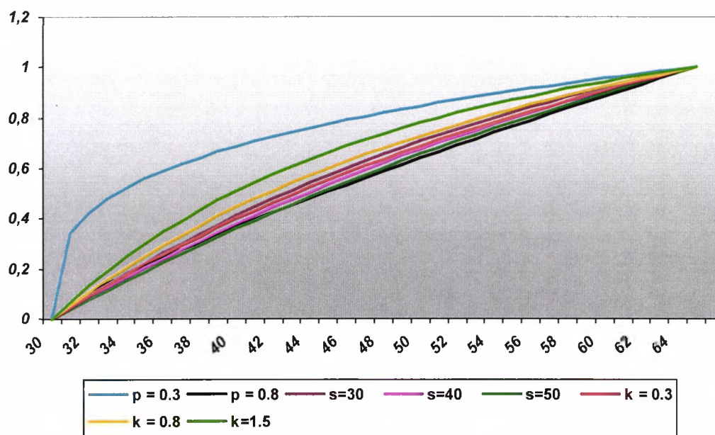
Figure 3.8 M(x) s development under the different distributions parameter values
