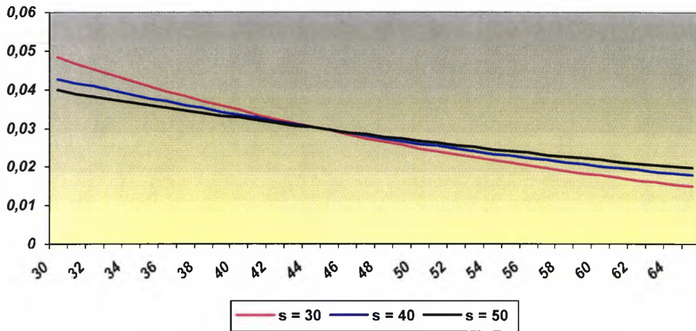
Figure 3.5 m(x) s development under the different Truncated Exponential parameter values
