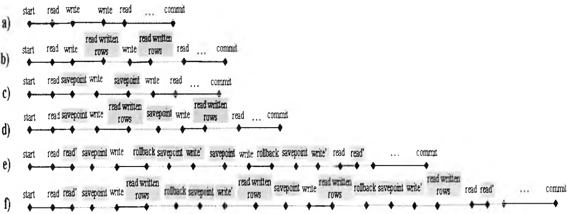
Fig. 11 - A transaction execution sequence in the experimental setups. The shaded boxes represent the fault tolerant mechanism used and the dotted lines represent the additional delays from their use. The second executions of the statements are proxies for rephrased versions of statements.
