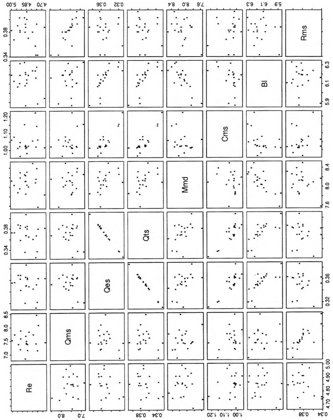
Fig. 5.6 Correlations between factors
