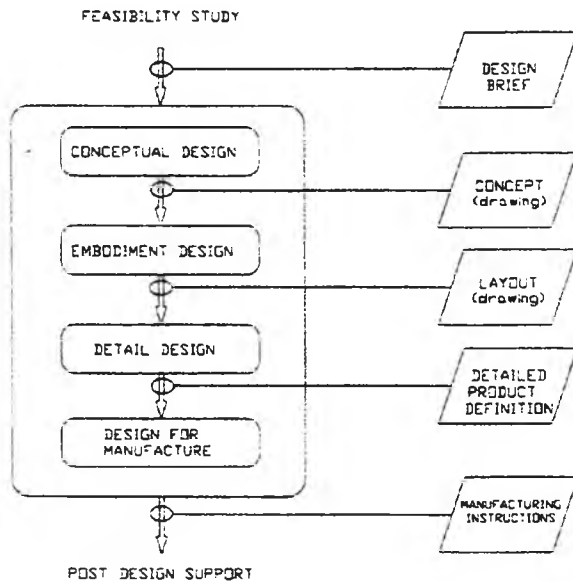
Fig. 1.13 The BS 7000 design model (BS7000, 1990)
