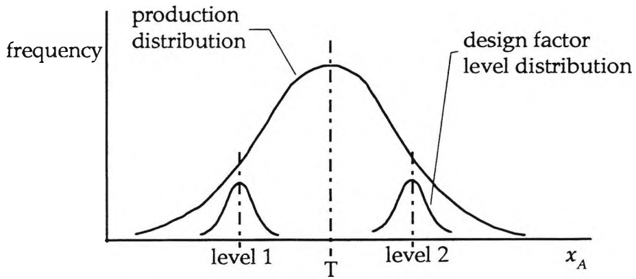
Fig. 3.12 Idealised production distribution of parameter value with “sub-six sigma” design factor levels (means of level 1 and level 2).
