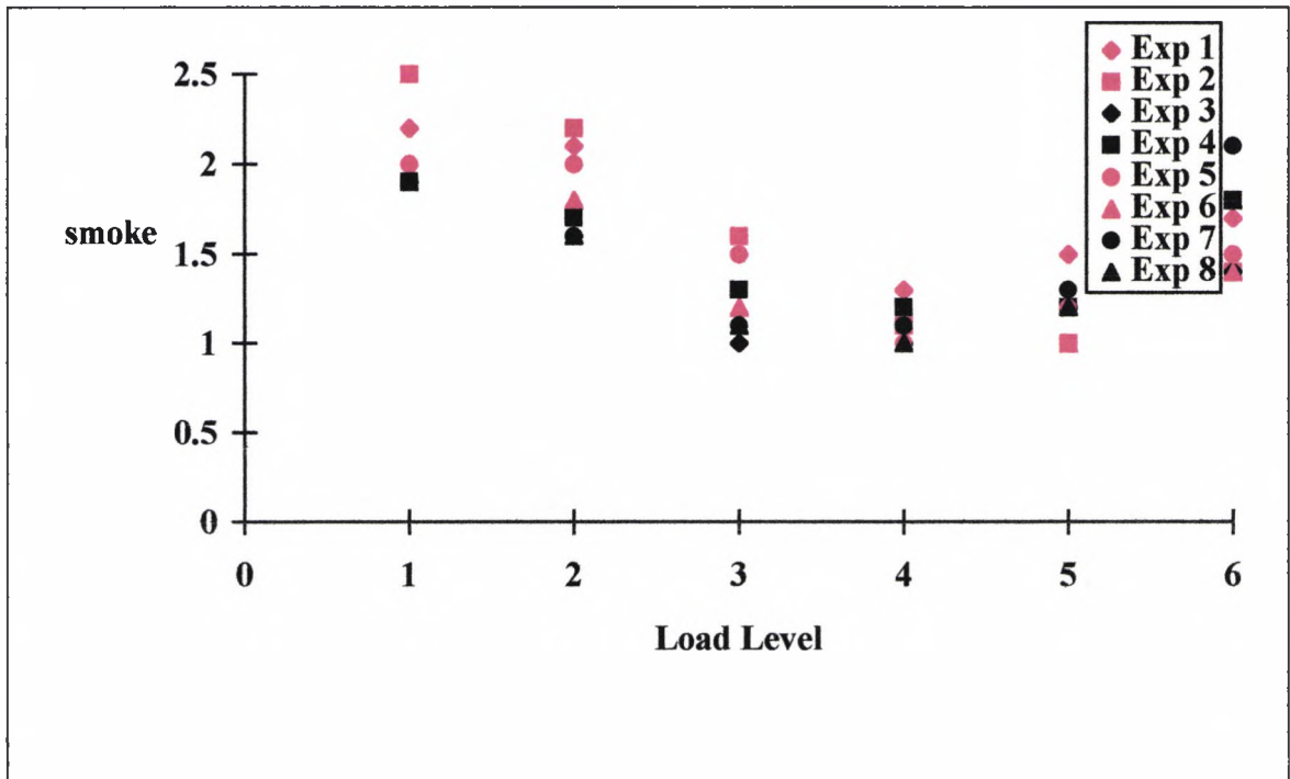
Fig. 7.6 Smoke emissions vs engine load for 8 experiments
