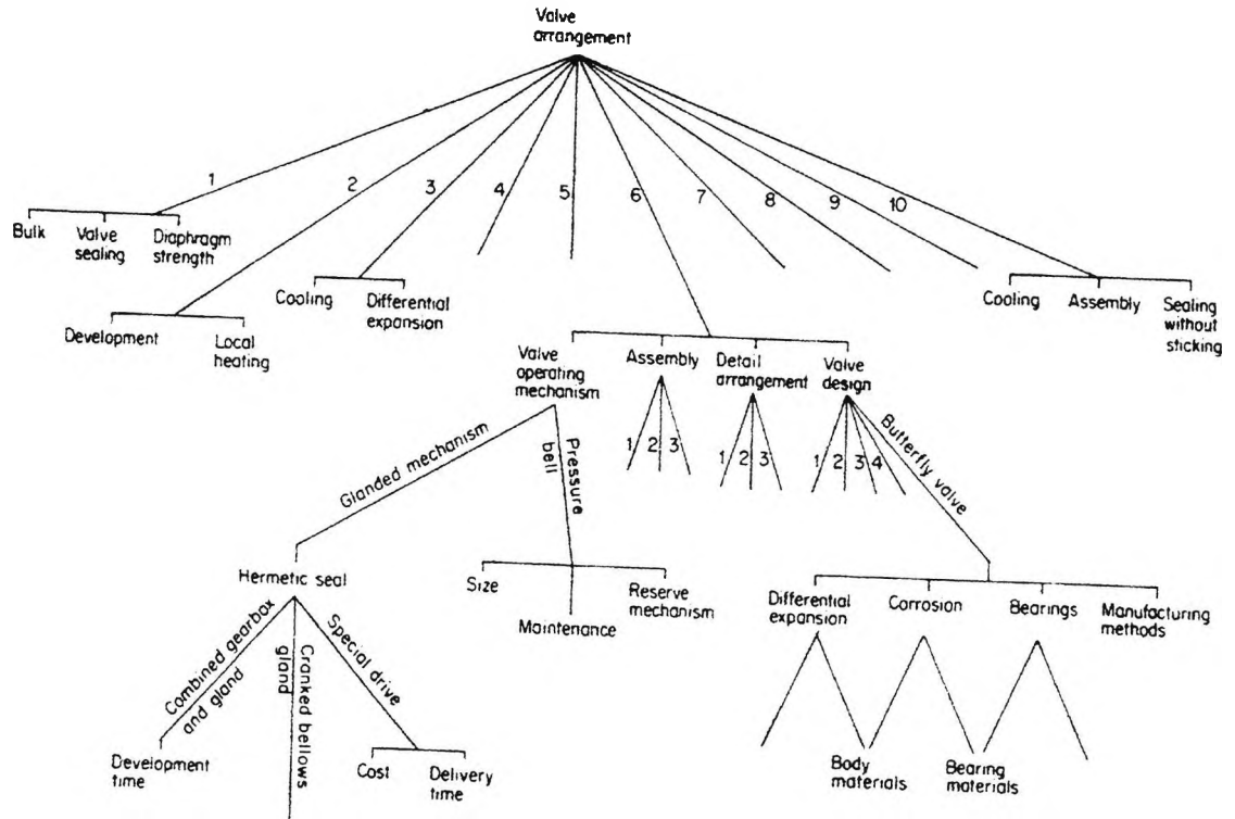
Fig. 1.5 Part of the problem structure in a nuclear reactor valve design problem (Cross, 1989)
