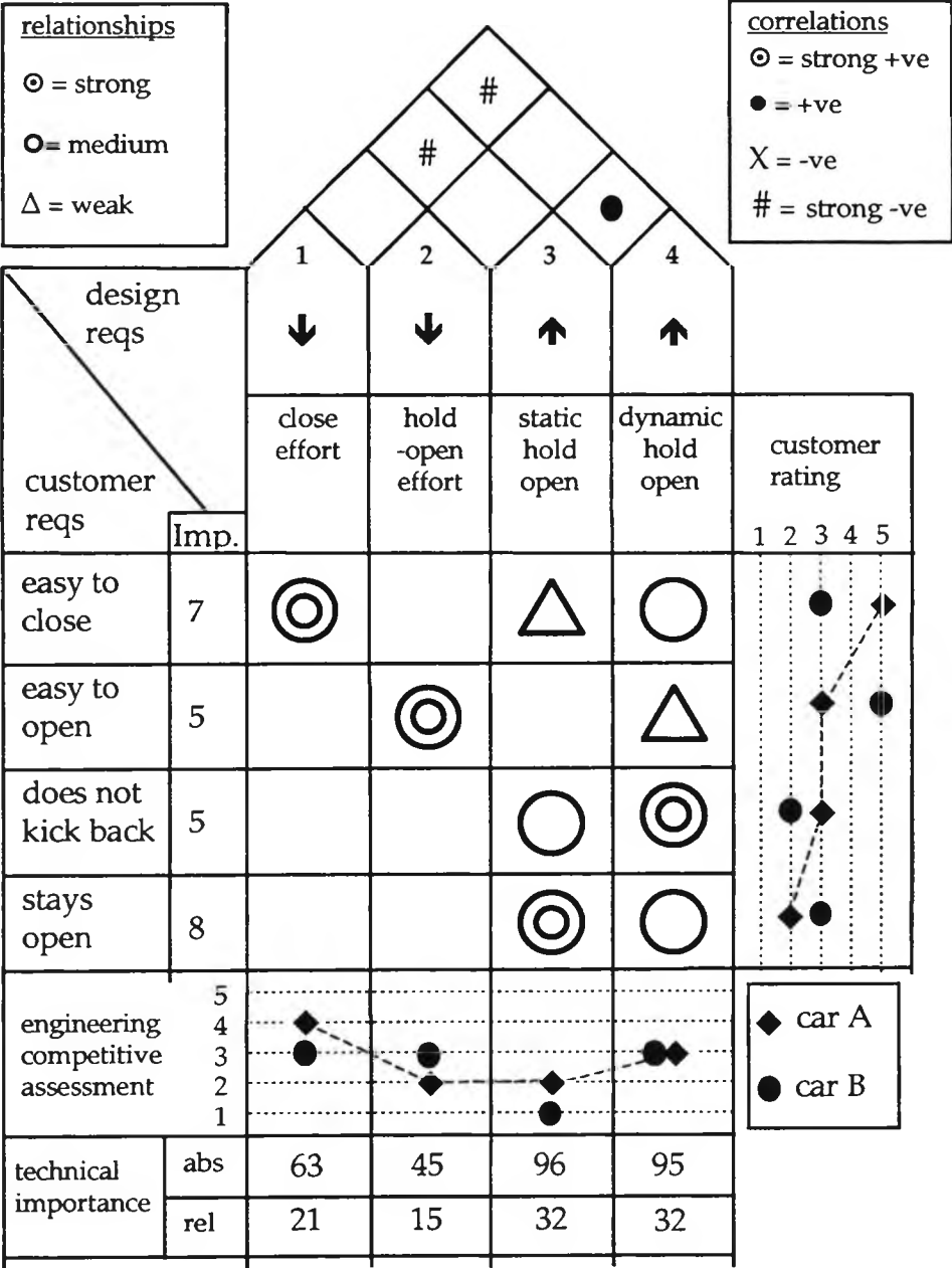
Fig. 1.17 QFD phase 1 chart
