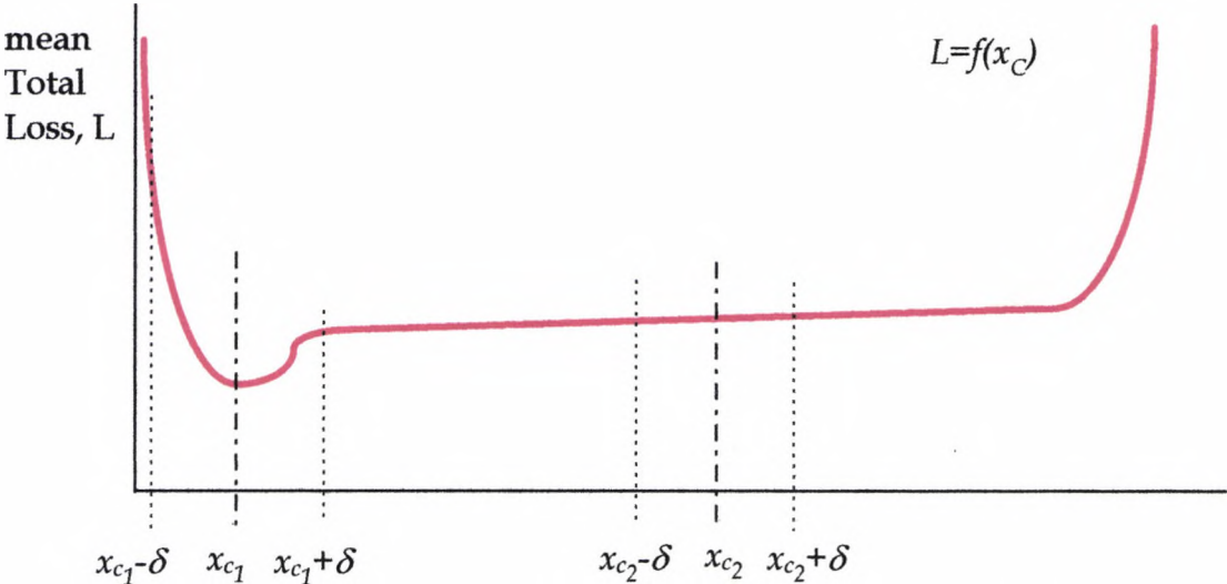
Fig 3.17 Total loss versus design factor setting with capability mapping
