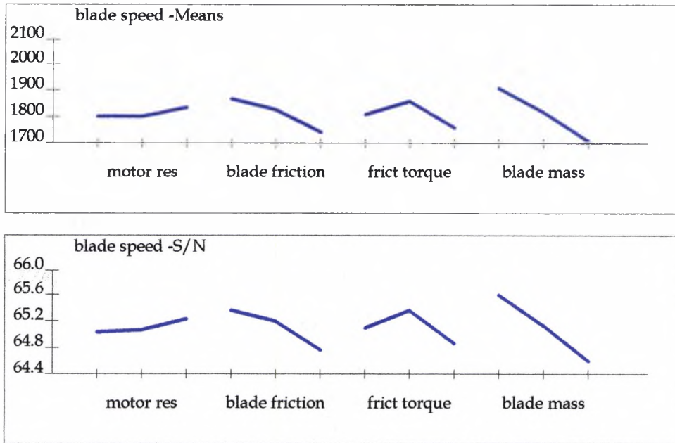
Fig. 6.8 Response graphs for physical experiments.
