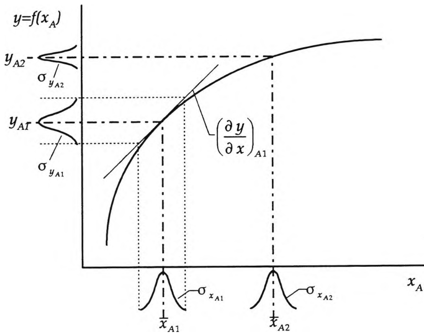
Fig. 3.15 Behaviour of \sigma_y , \sigma_x and \frac{\partial y}{\partial x} local to level 1 of Factor A
