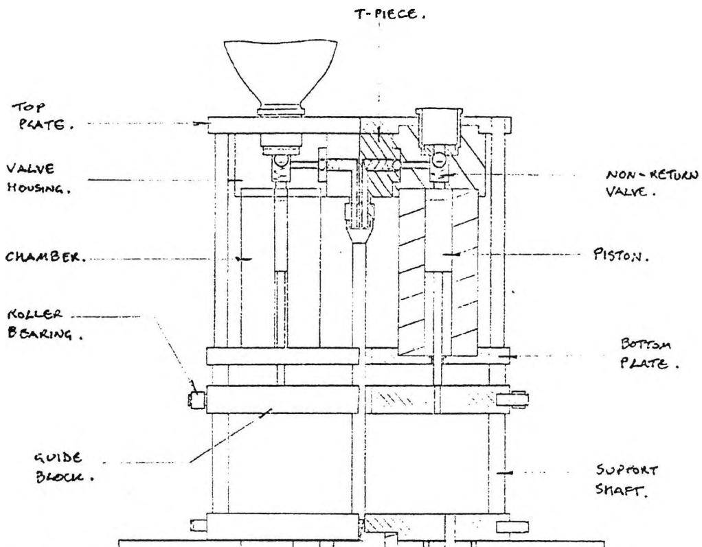
Fig. 4.4 Close-up of mixing head (Cattini, 1997)
