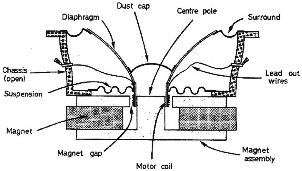
Fig. 5.1 Moving-coil loudspeaker driver unit (Colloms, 1991)
