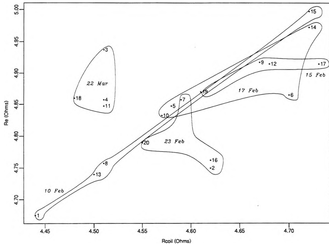
Fig. 5.8 R_e versus R_{coil} for twenty driver units
