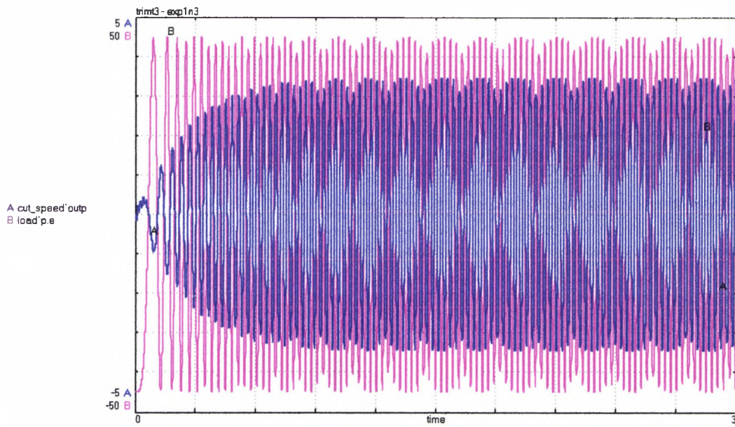
Fig. 6.6 Simulation output of hedgetrimmer from 20-sim package.
