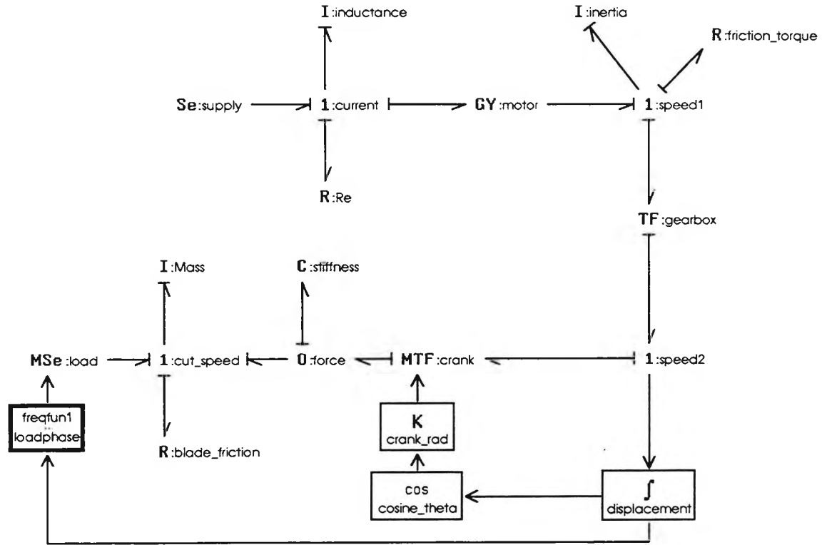
Fig. 6.5 Bond graph of motor-blade system
