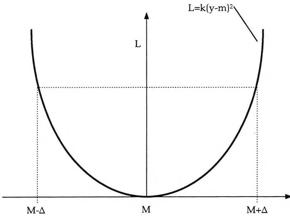
Fig. 1.14 Taguchi's quality loss function (Taguchi, 1986)
