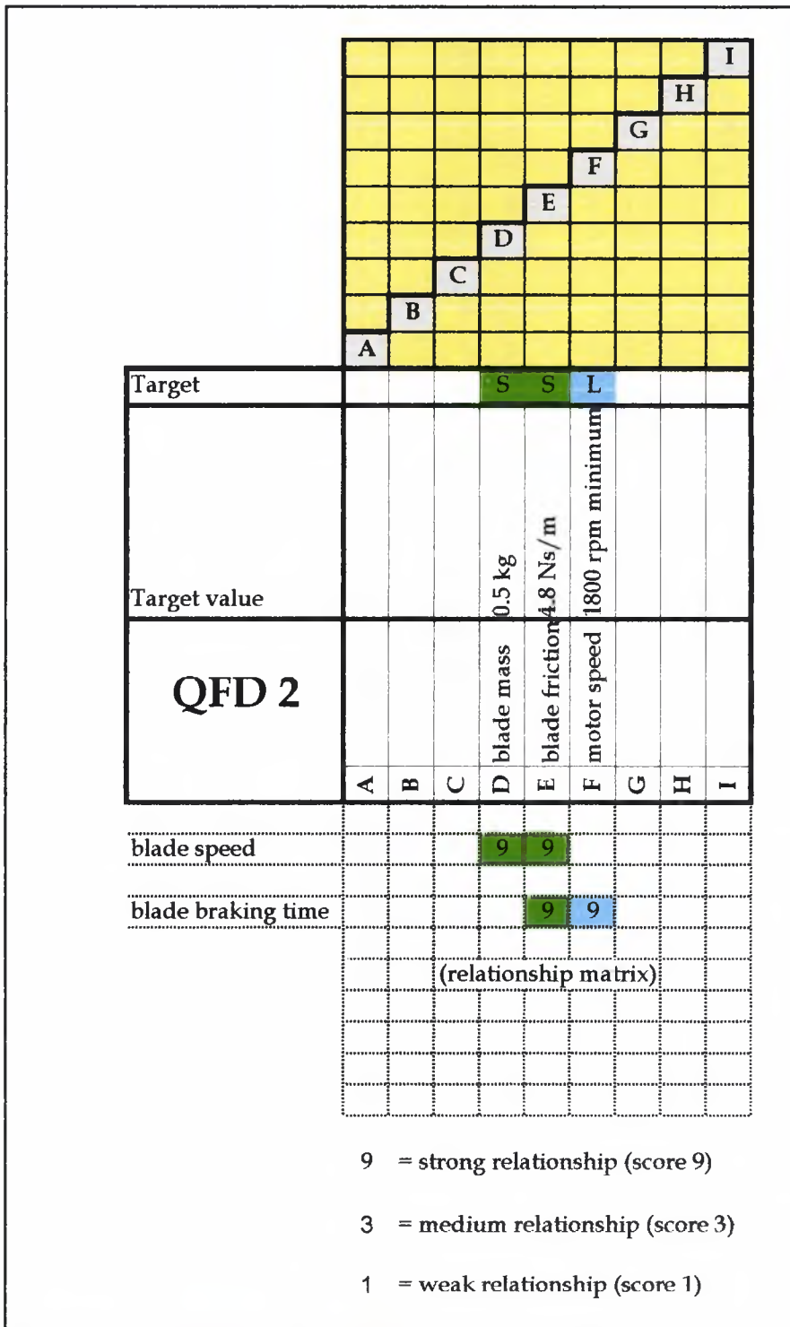
Fig. 6.9 QFD phase 2 entries for motor-blade system
