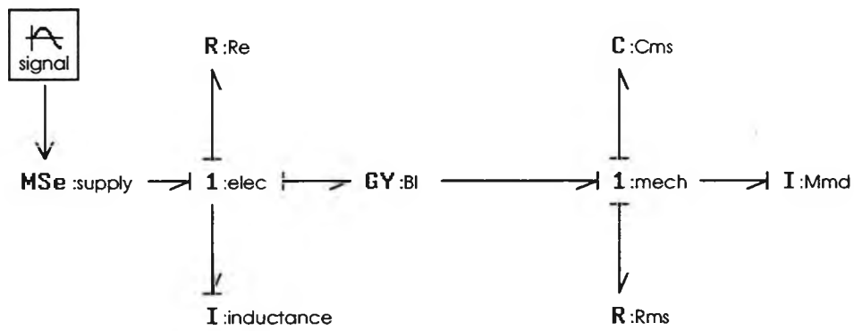
Fig. 5.3 Bond graph model of loudspeaker voice-coil
