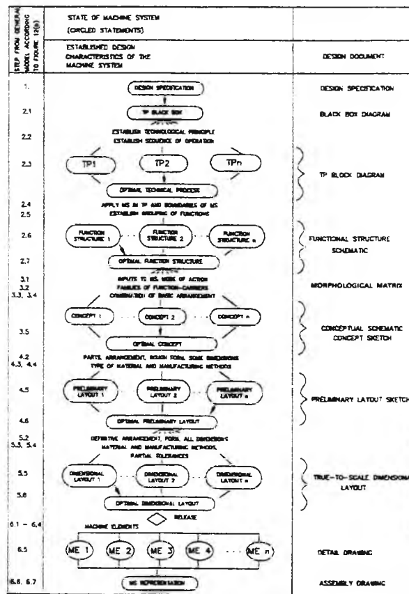
Fig. 1.10 The design model by Hubka (1982)
