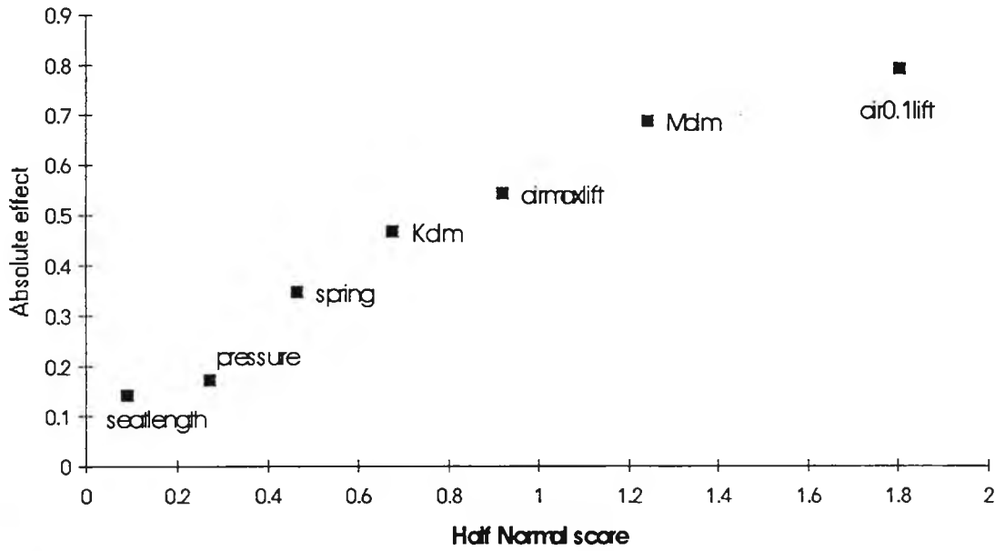
Fig. 7.9 Daniel plot of smoke emissions data (Appendix A)
