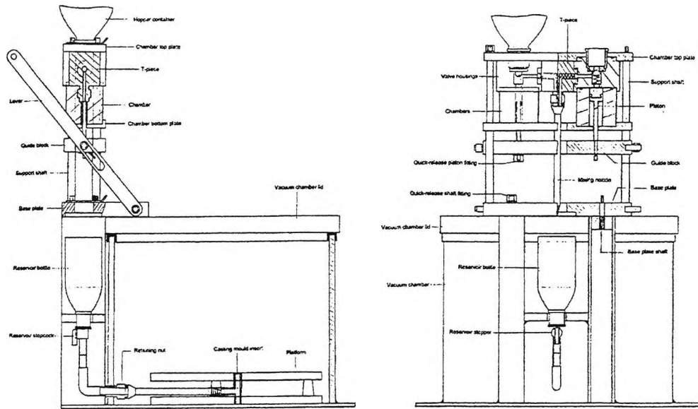
Fig. 4.3 Elevations of vacuum casting equipment (Cattini, 1997)
