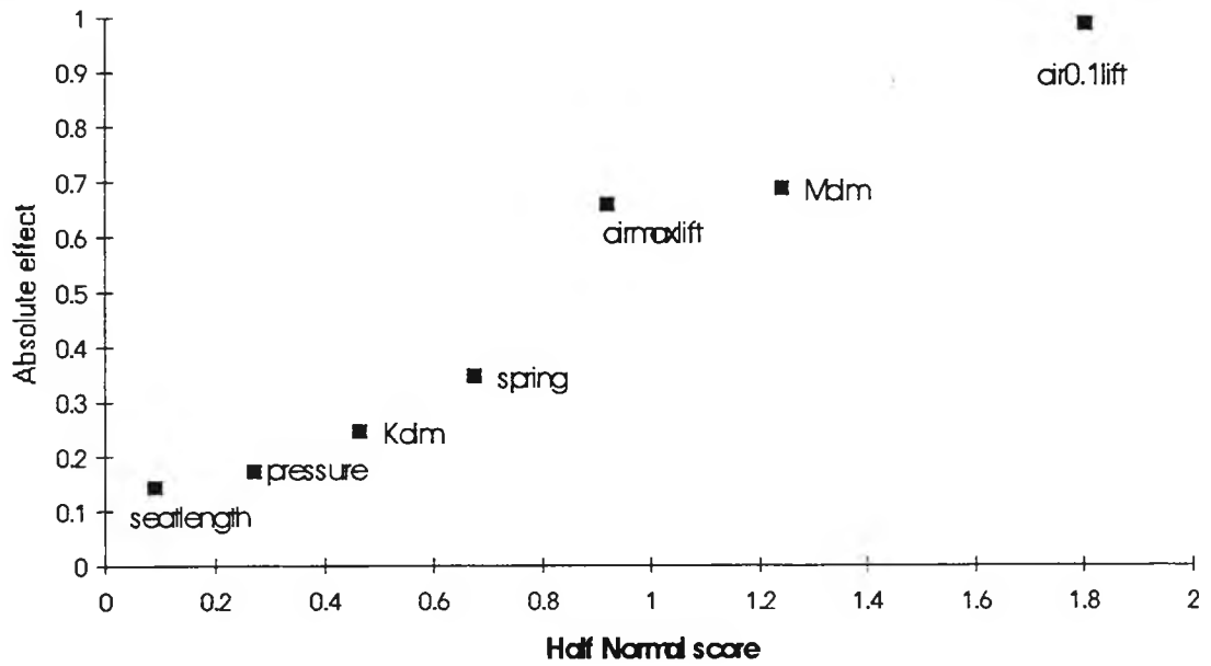
Fig. 7.10 Daniel plot of adjusted data for smoke emissions
