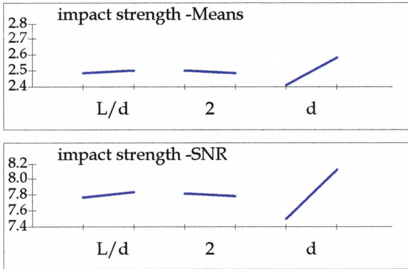
Fig. 4.6 Response graphs for impact data
