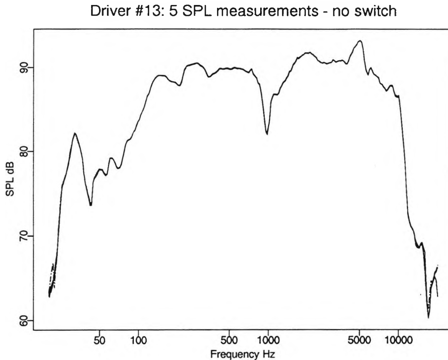
Fig. 5.5 Five SPL measurements of driver #13 without Z switch
