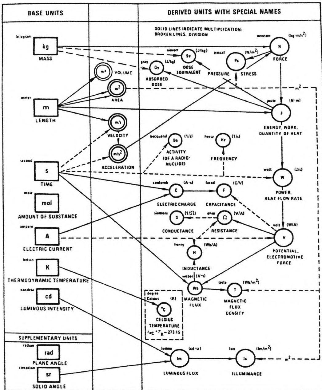
Fig. 3.11 Relationship between SI metric units (Campbel, 1993)
