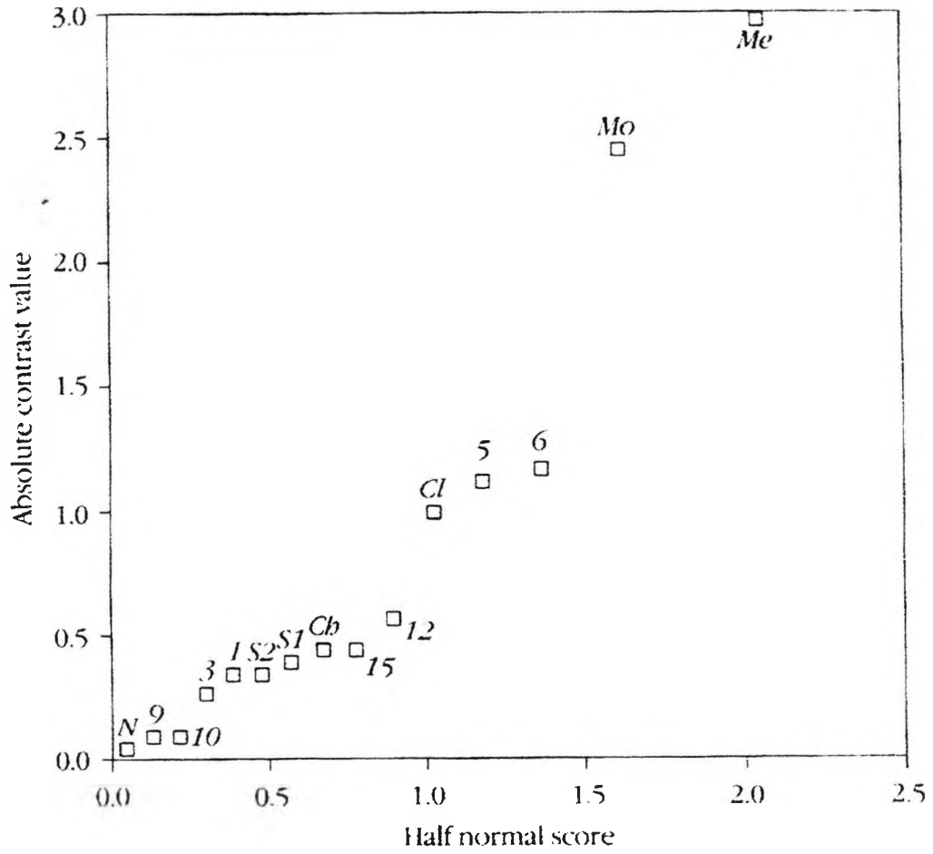
Fig. 1.26 Daniel plot for glove box lid experiment (Grove & Davis, 1992)
