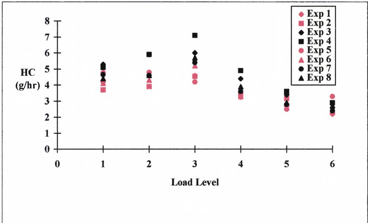
Fig. 7.5 Hydrocarbon emissions vs engine load for 8 experiments
