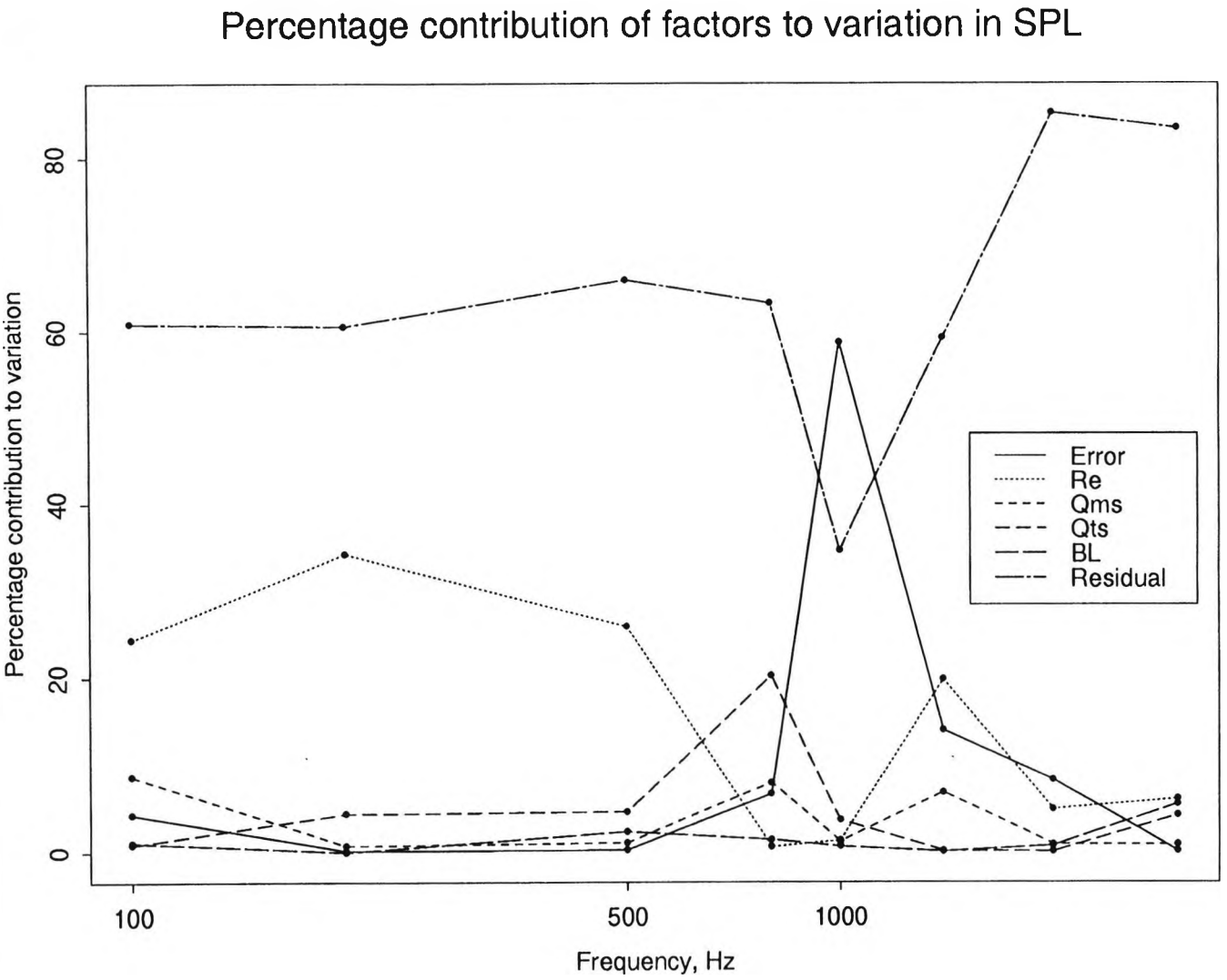
Fig. 5.7 Results of ANOVA @ 100, 200, 500, 800, 1000, 1400, 2000, 3000Hz
