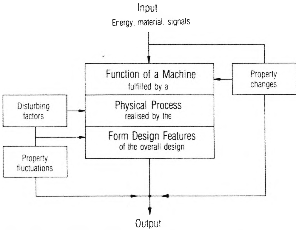
Fig. 1.27 Design steps according to Rodenacker (1970)
