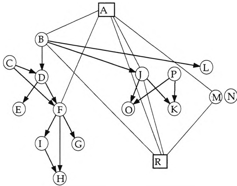
Fig. 6.2 Raw correlation chain network for hedgetrimmer
