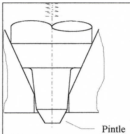
Fig. 7.4 Schematic diagram showing pintle end of injector valve-nozzle assembly
