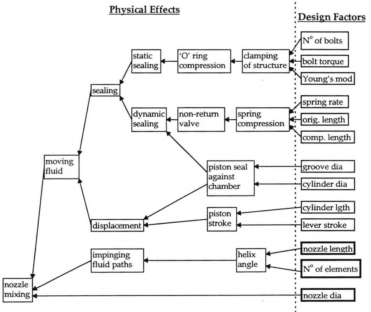
Fig. 4.5 Physical effects and potential design factors
