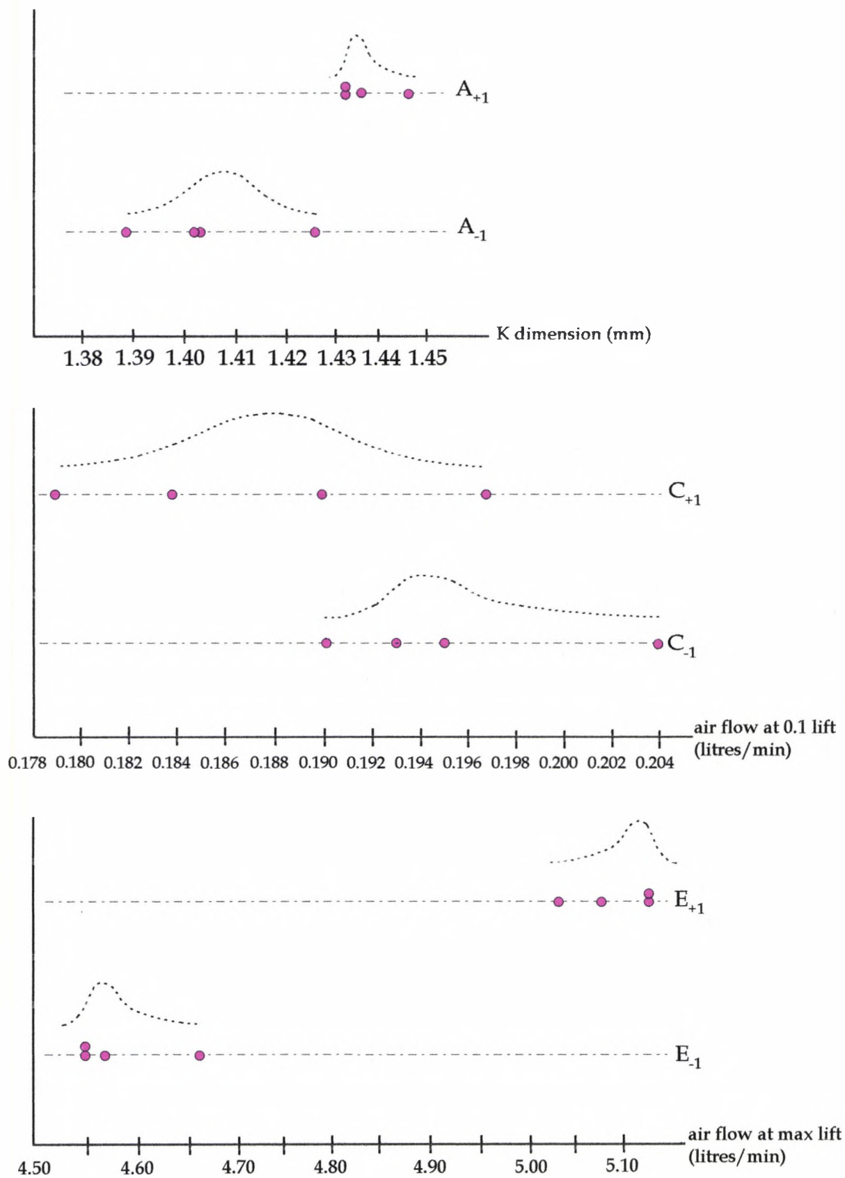
Fig. 7.8 Distribution of factor levels from production
