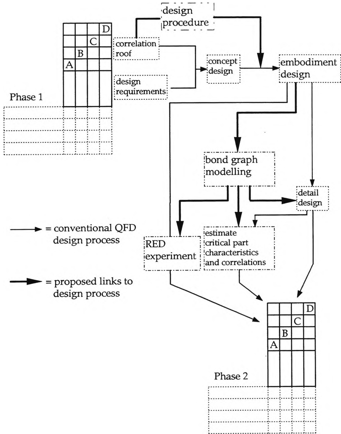
Fig. 3.10 Proposed link between bond graphs and QFD
