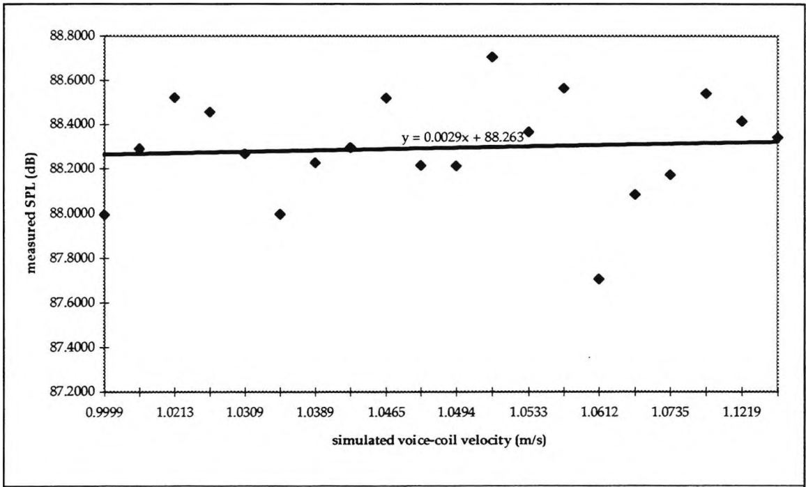
Fig. 5.10 Comparison of experimental and simulation results
