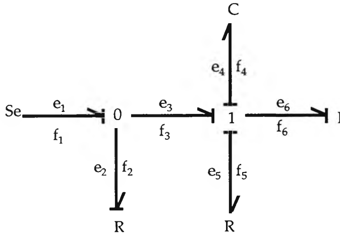
Fig. 2.13 Bond graph with integral causality
