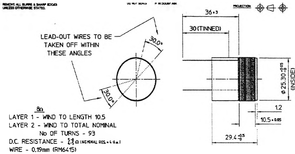
Fig. 5.2 Example of a loudspeaker voice-coil
