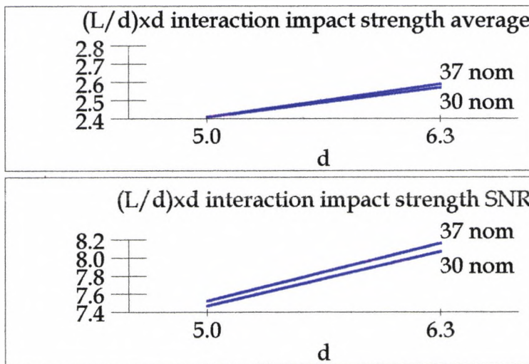
Fig. 4.7 Interaction plot of d and l/d
