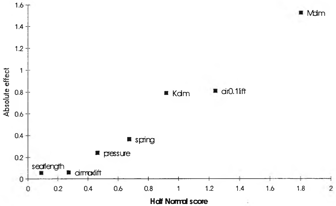
Fig. 7.11 Daniel plot of HC emissions data (Appendix A)
