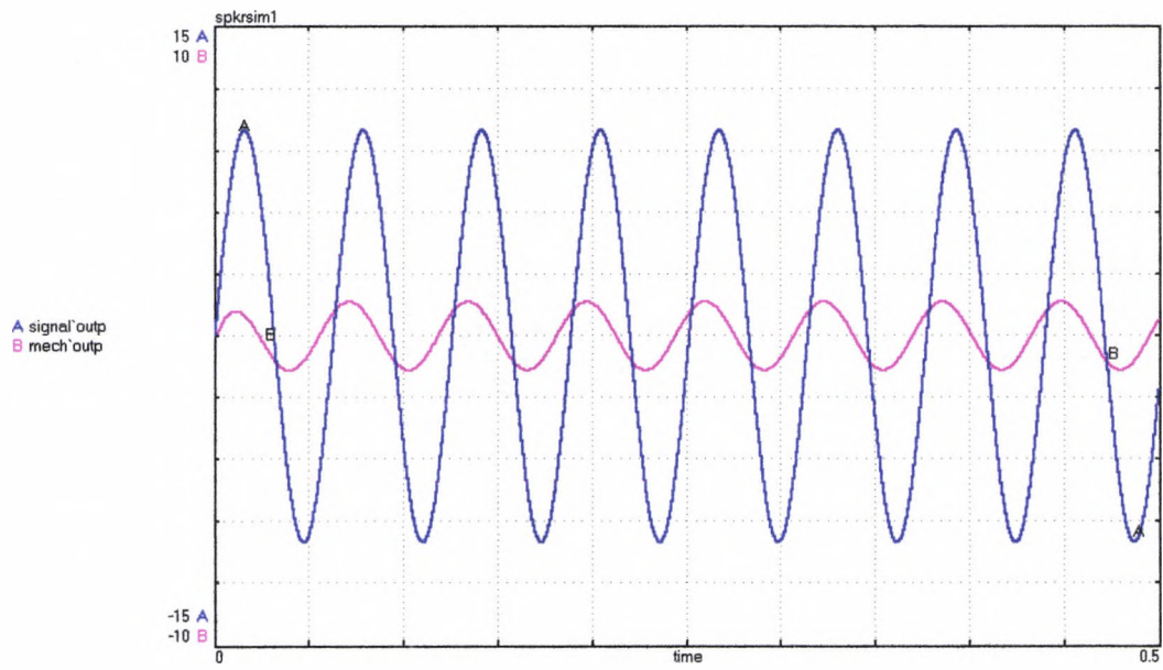
Fig. 5.9 Simulation output for bond graph model of voice-coil
