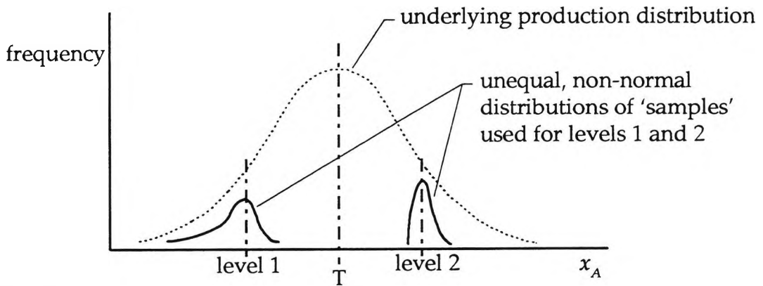
Fig. 3.14 Possible distributions of tolerance noise about nominal design factor levels
