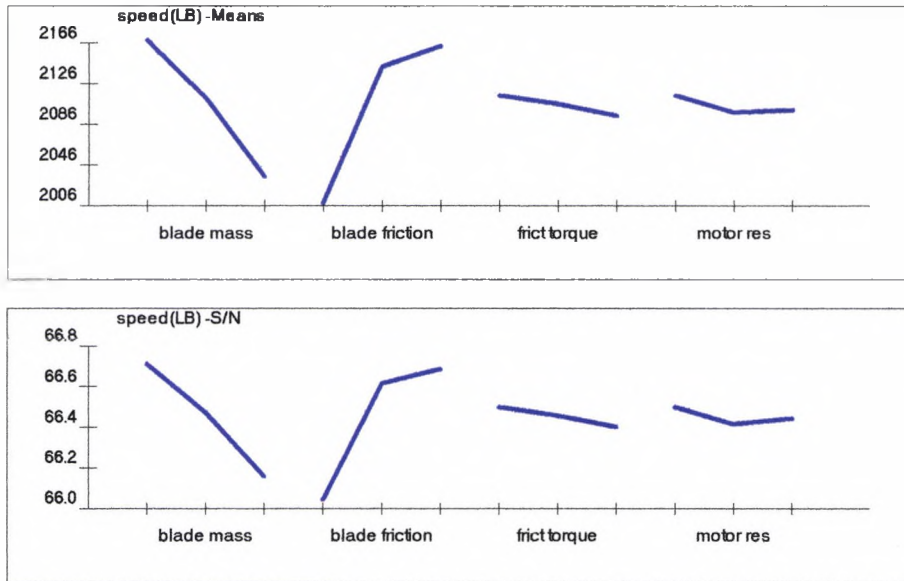
Fig. 6.7 Response graphs for simulation experiment.
