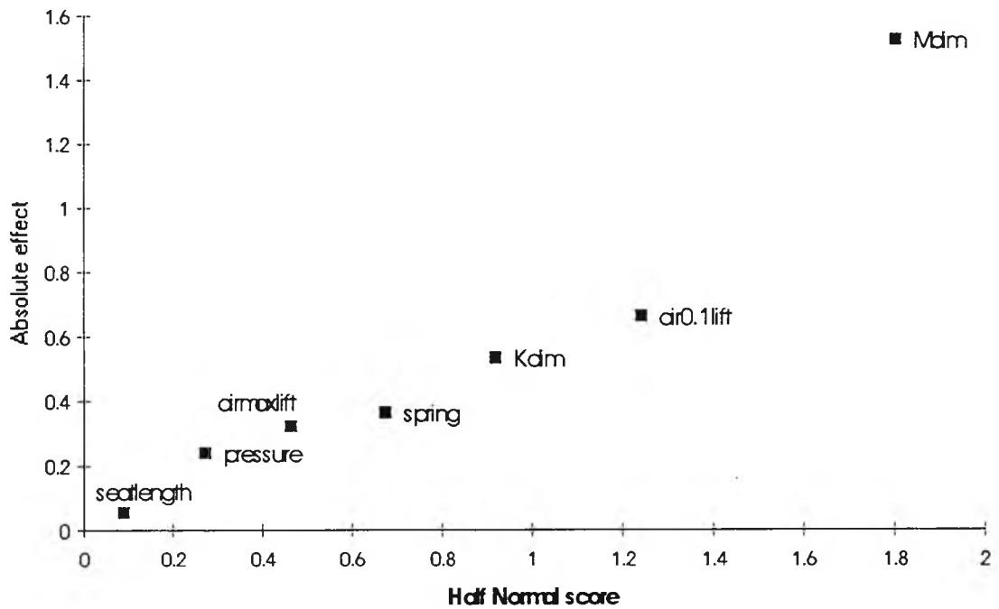
Fig. 7.12 Daniel plot of adjusted data for HC emissions
