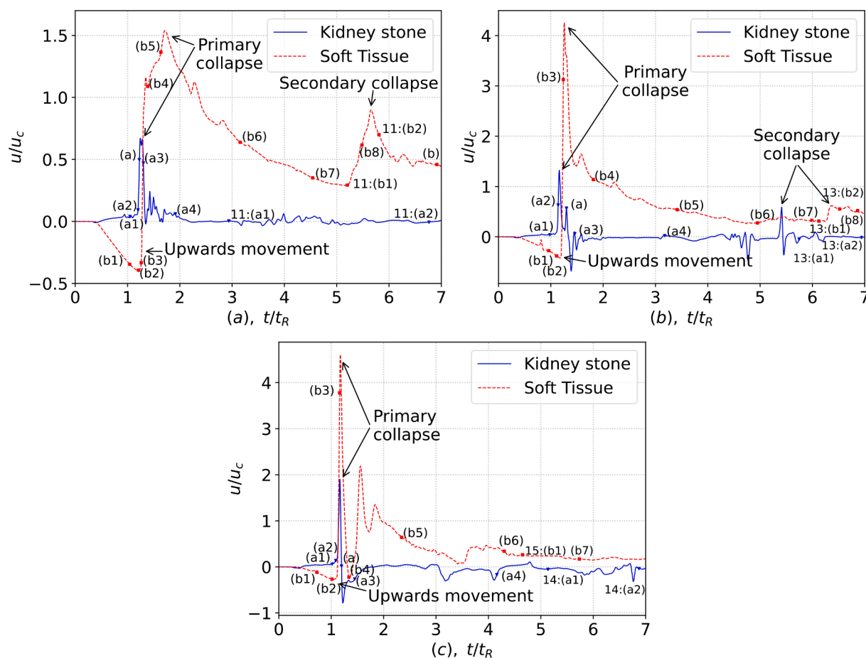
Fig. 10. Effect of stand-off distance/attachment on solid boundary's velocity overtime at r/R_0 = 0 . (a) Detached bubbles with stand-off distance S/R_0 = 1.2 , (b) Attached bubbles with stand-off distance S/R_0 = 0.6 and an acute angle, (c) Attached bubbles with stand-off distance S/R_0 = -0.2 and obtuse angle. Time instances given are: (a-a4) for KS, and for ST (b-b8) from Figs. 8, 12,14. References to secondary collapse Figs. 11, 13,15 are given with their corresponding number.
