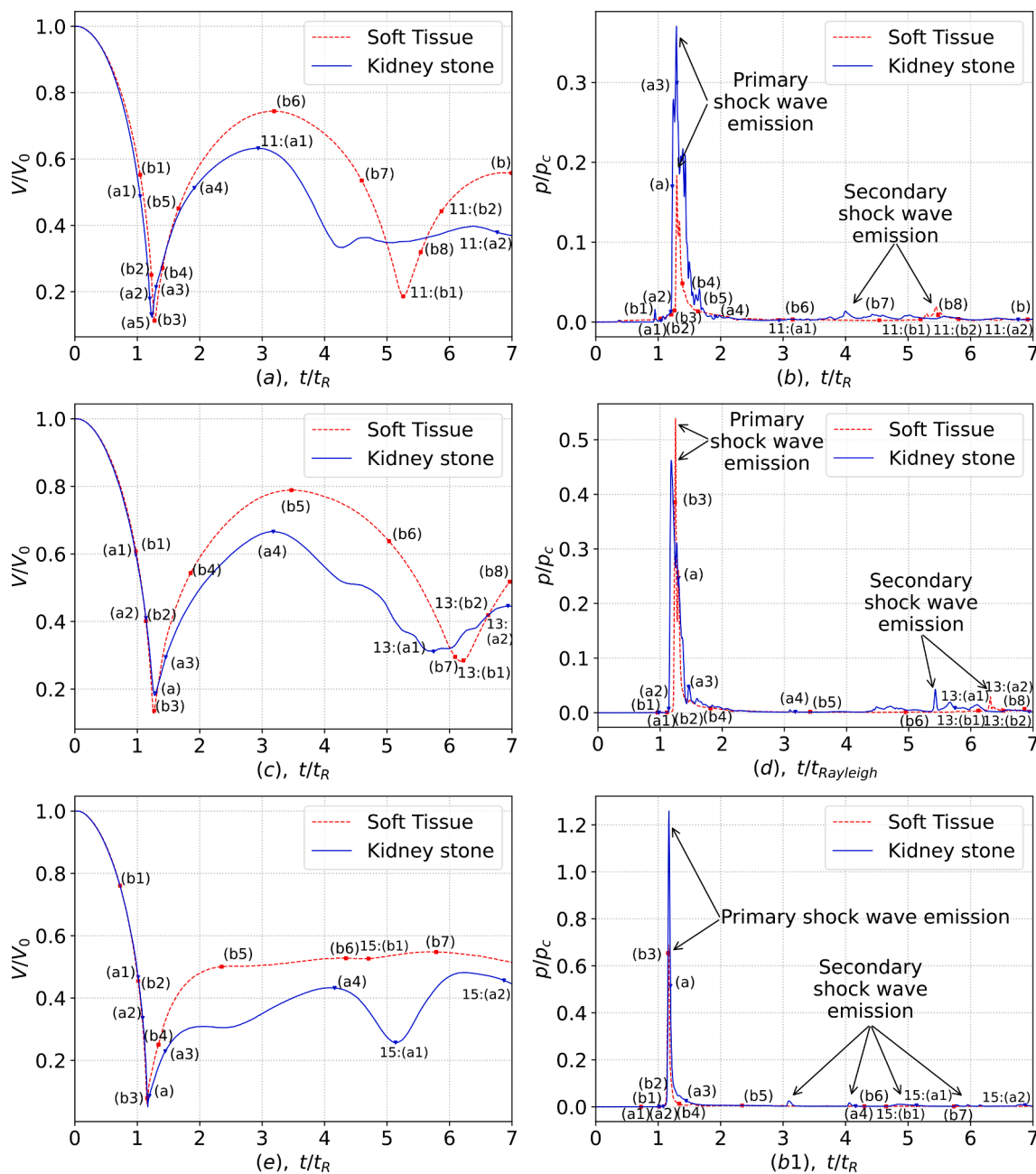
Fig. 9. Effect of stand-off distance/attachment on non-dimensionalized gas volume evolution over time and non-dimensionalized pressure on the solid interface at r/R_0 = 0 . (a)/(b) Detached bubbles with stand-off distance S/R_0 = 1.2 , (c)/(d) Attached bubbles with stand-off distance S/R_0 = 0.6 and acute angle, (e)/(f) Attached bubbles with stand-off distance S/R_0 = -0.2 and obtuse angle. Time instances given are: (a-a4) for KS, and for ST (b-b8) from Figs. 8, 12,14. References to secondary collapse Figs. 11, 13,15 are given with their corresponding number. Same magnification in all figures, except the (a/b), and (b5-b8).
