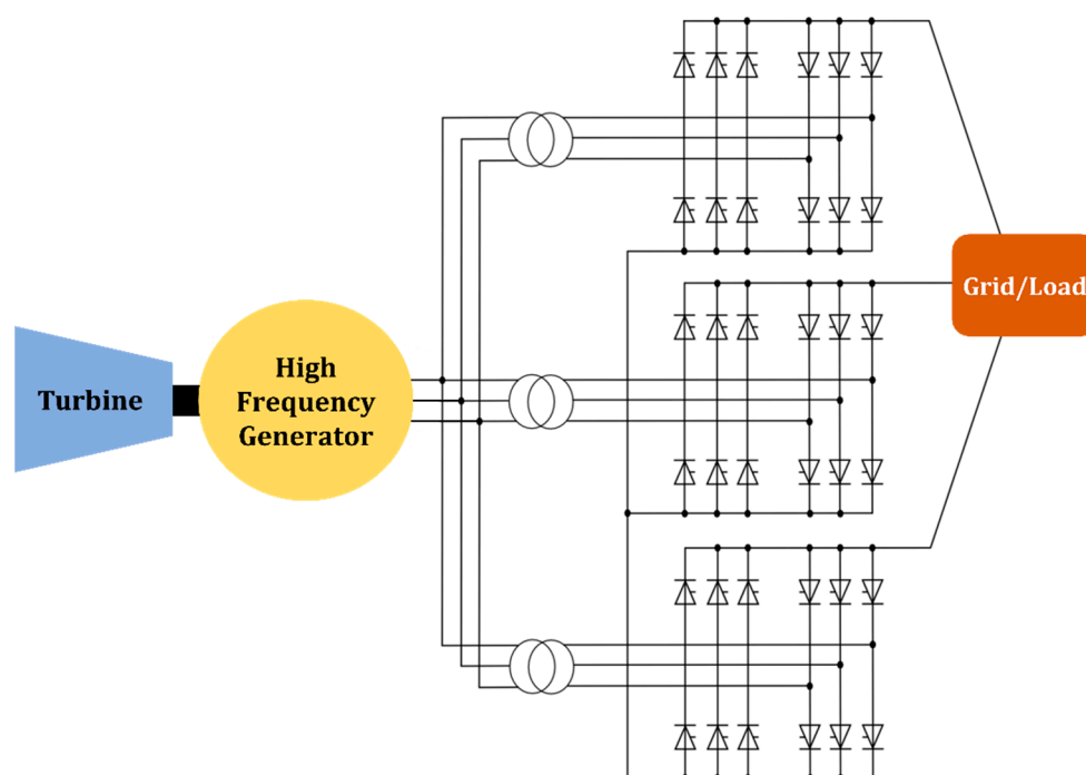
Figure 4. Cycloconverter topology in microturbines.
