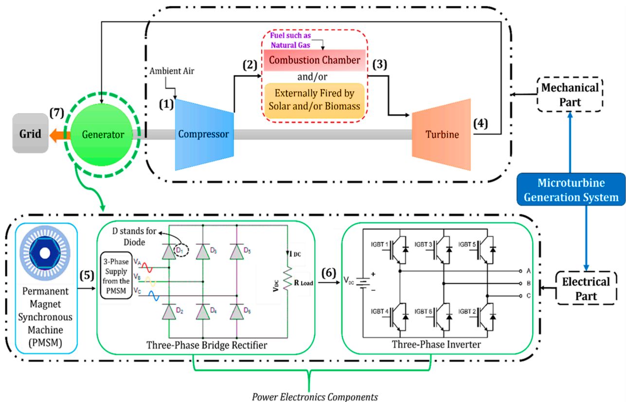
Figure 1. Microturbine generation system topology.
