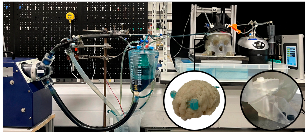
Figure 1. Head phantom, including both circulatory systems. On the left, the pulsatile pump, tubes and reservoirs of the blood circulation. On the right, the syringe pump, tubes and reservoir of the CSF circulation.
