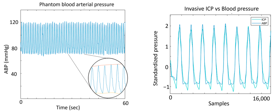
Figure 7. Phantom blood arterial pressure.
