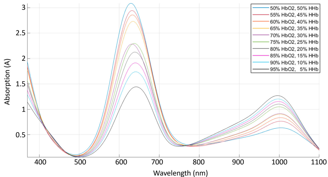
Figure 8. Spectra of the dye-based artificial blood mixtures.
