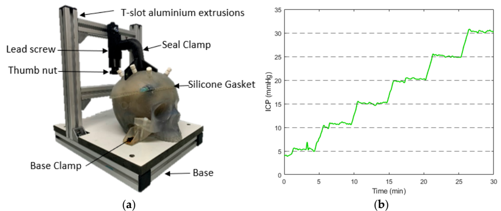
Figure 5. Skull seal description and performance: (a) parts of the seal system; and (b) graphical results of the seal test.
