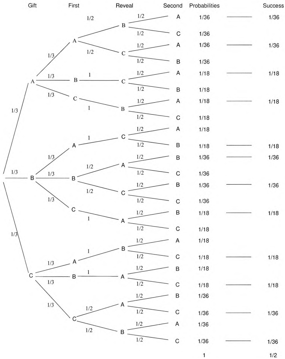
Figure 7.3: Probability Tree for strategy \gamma ; with ChooseWith = 1/2 .
