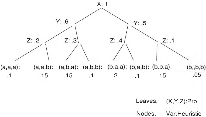
Figure 6.5: Tree illustrating probabilistic approximation.
