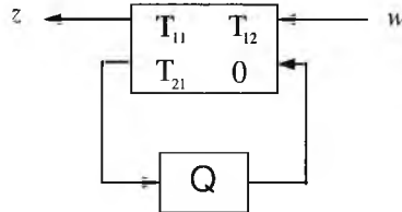
Figure 3.6: Closed loop as a lower LFT interconnection, in terms of parameter Q .
