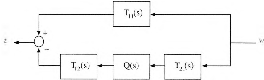
Figure 3.5: Model-matching problem.
