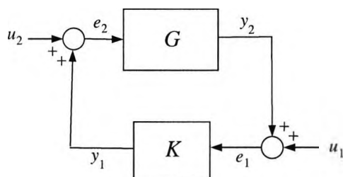
Figure 3.1: General feedback interconnection.
