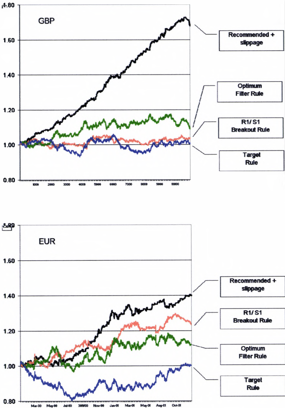
Figure 3. Value of positions based on recommended trades and selected mechanical rules, GBP and EUR, hourly, 2000-1. (Value of $1)
