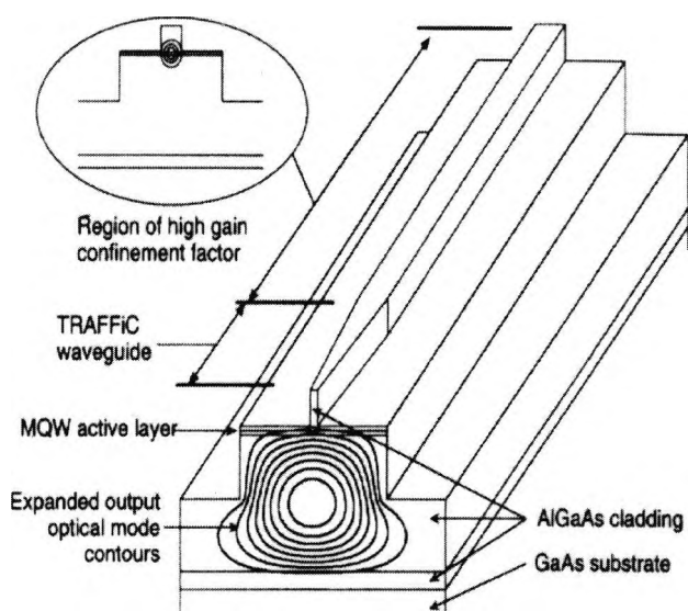
Fig. 6.4 Tapered twin rib structure with contours of optical mode at the input and output (Vawter et al. , 1997)
