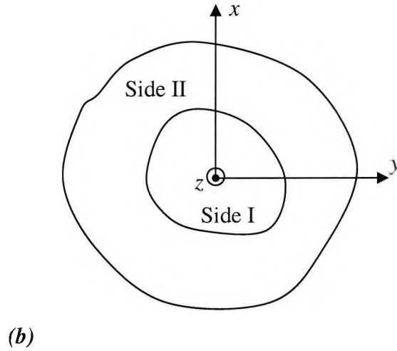
Fig. 5.2 Discontinuity junction of two dielectric waveguides (a) Vertical section of the discontinuity between side I and II. (b) Transverse cross section of the discontinuity at the junction of two sides.
