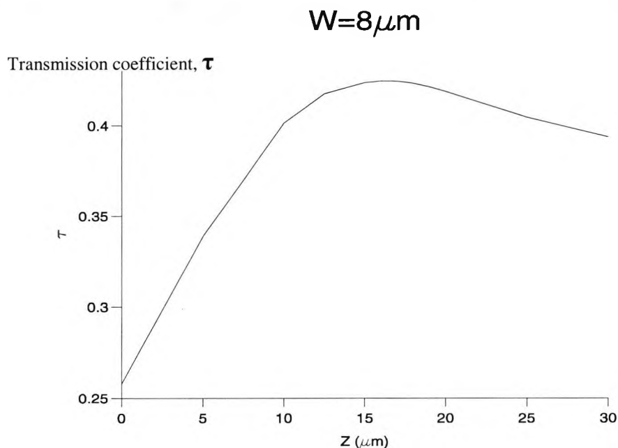
Fig. 5.7 Variation of optical power coupled to the SMF with the axial distance, z .
