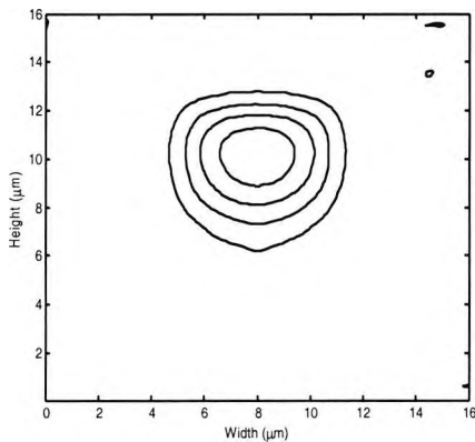
Fig. 7.34. Case 6. TE mode profile at point B = 1949 μm in fig 31 for the spot-size expansion of the tapered SSC.
