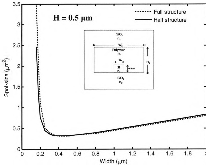
Fig. 6.5 Variation of spot-size profile along the width of the waveguide to determine the width for the modal cut-off region for the structure with indices 3.48/3.0/2.98.
