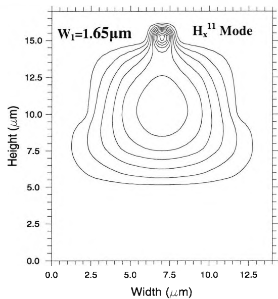
Fig. 5.20 H_x field contour for the fundamental quasi-TM mode when W_1 = 1.65 \mu\text{m} .
