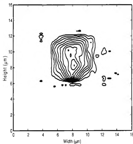
Fig. 7.18. Case 4. The output TE mode field profile from the FVBPM at the end of the mode conversion in the laterally tapered SSC. W_f = 0.14 \mu\text{m} .
