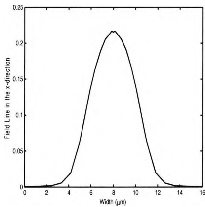
Fig. 7.35. The field line in the x-direction for point A = 1848 μm where the spot-size first peak occurred.
