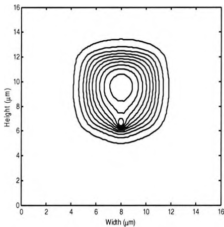
Fig. 7.33. Case 6. TE mode profile at point A = 1842 μm in fig 31 for the spot-size expansion of the tapered SSC.
