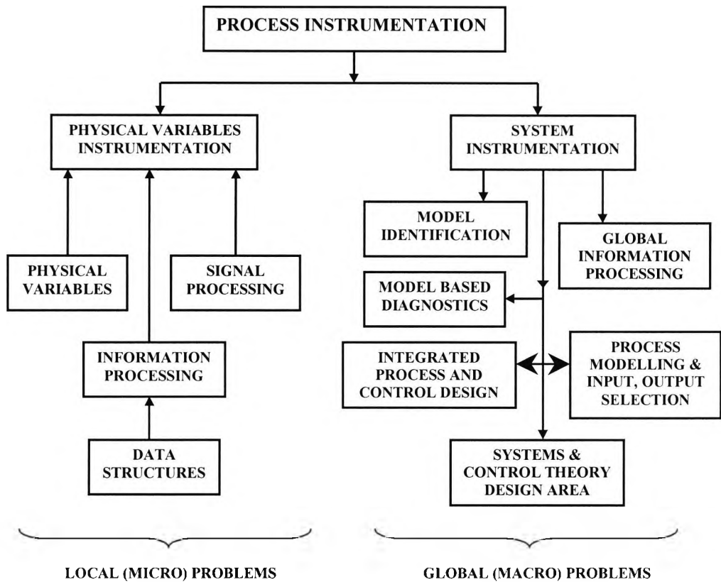
Figure 6.7: The area of Global Process Instrumentation
