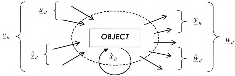
Figure 3.3: Embedding of an Object and Classification of Variables
