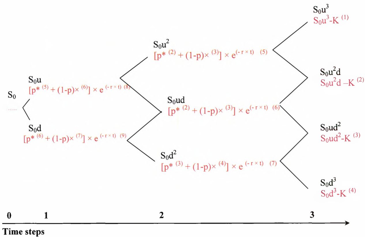
Figure 7.4: Option valuation lattice for a call option (Three time-steps Recombining lattice)
