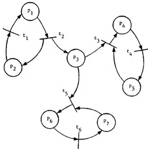
Figure 5.4: A simple example of a Petri net [Pet].
