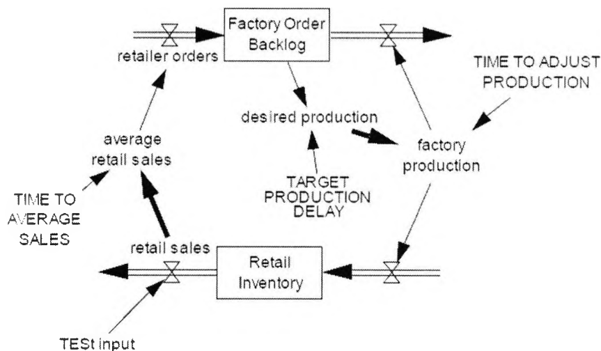
Figure 5.7: A stock and flow diagram of the model [Kirk].
