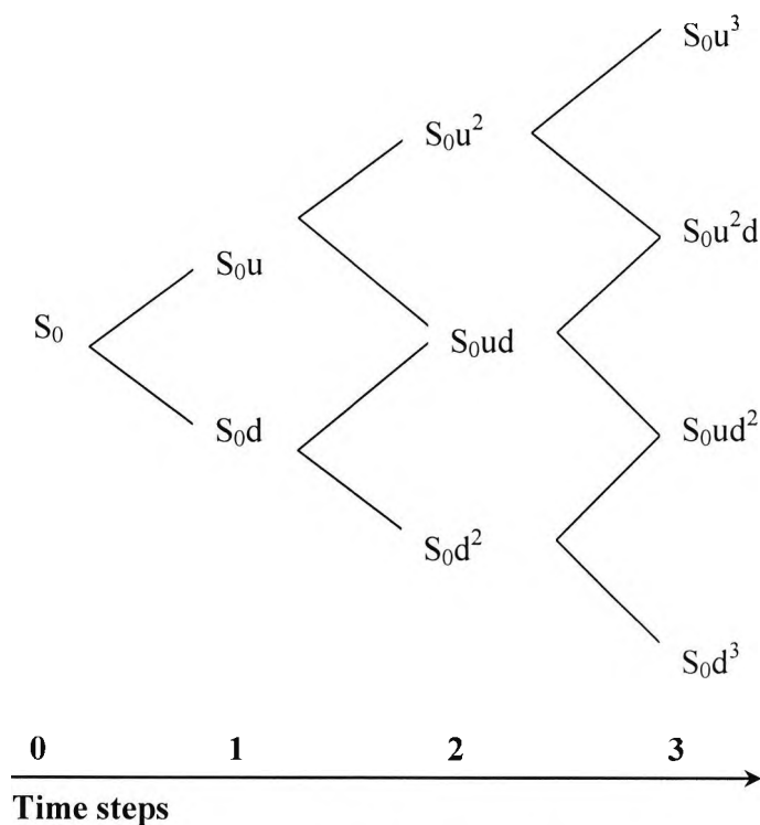
Figure 7.3: Binomial lattice of the underlying asset value (Recombining lattice).
