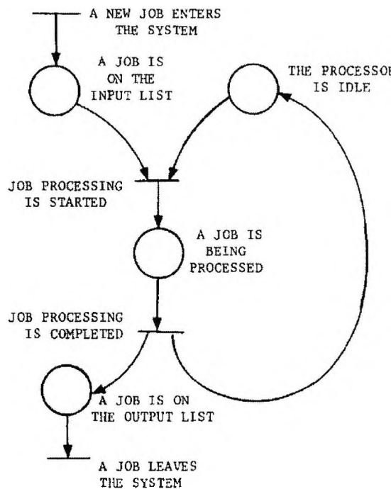
Figure 5.5: Modelling of a simple computer system [Pet].
