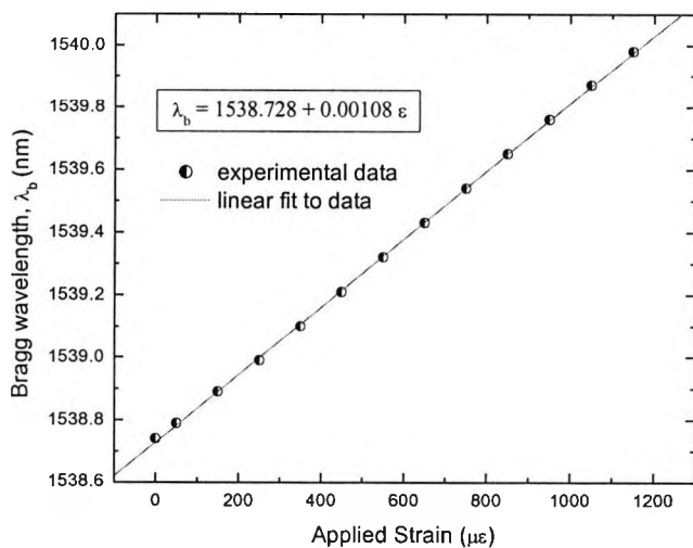
Fig. 6.10: Strain response of the FBG in terms of \lambda_b -shift, measured at 22°C. The solid line is linear fit to data. Error bars are smaller than the data points.
