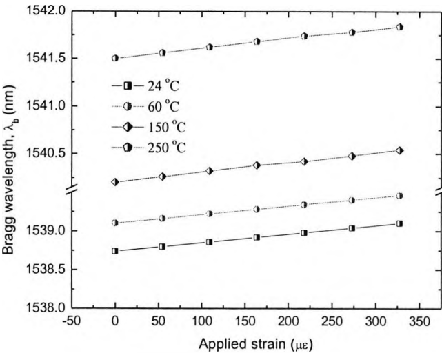
Fig. 6.12: Bragg wavelength shift versus the applied strain at various sets of temperature (24 °C, 60 °C, 150 °C and 250 °C) to observe the temperature-effect on strain-sensitivity. The error bars are smaller than the data points.
