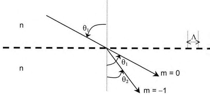
Fig 2.7: The diffraction of a light ray through a grating.
