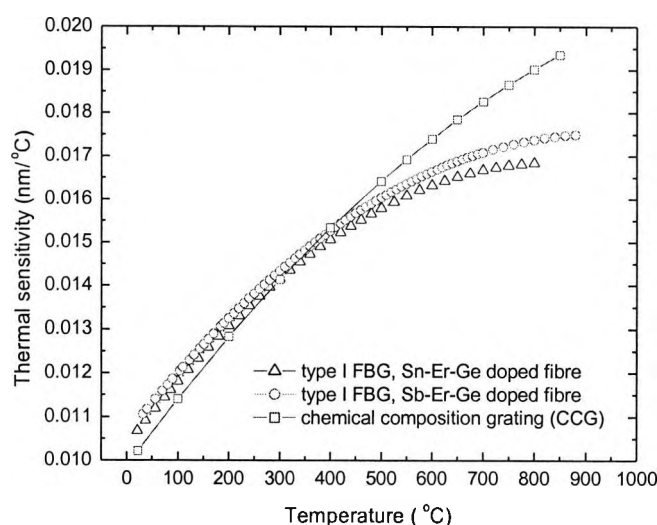
Fig. 5.10: Variation of the values of the thermal sensitivity of various gratings (type I FBG written in Sn-Er-Ge and Sb-Er-Ge doped fibre along with a CCG) over a wide range of studied temperatures.
