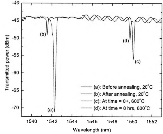
Fig. 6.15(b): Grating spectra at different times and temperatures during the process of annealing.
