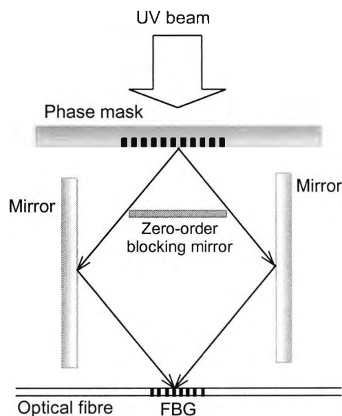
Fig. 2.5(b): Non-contact Talbot interferometric configuration for grating writing using a phase mask.
