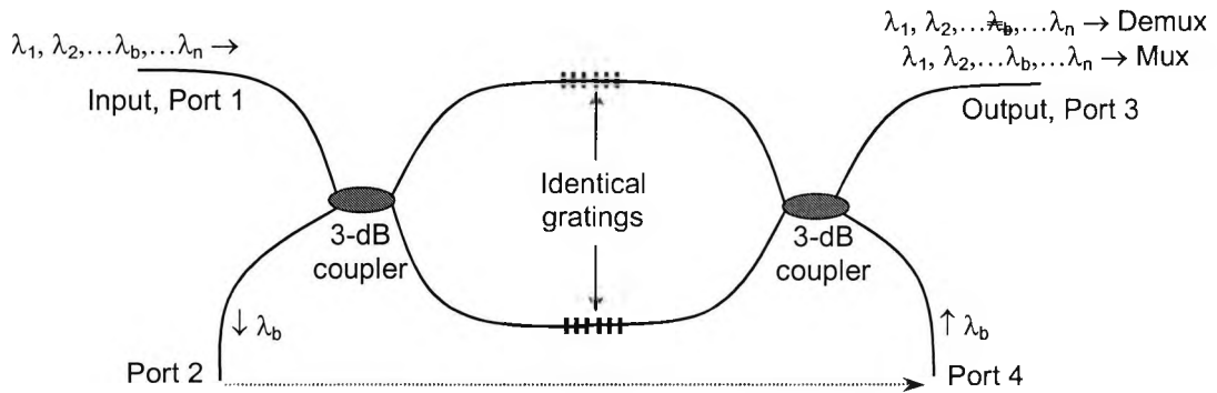
Fig. 2.13: A schematic of Add/Drop Multiplexer/Demultiplexer.
