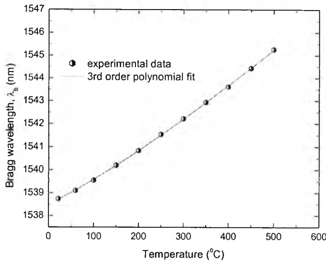
Fig. 6.9: Bragg wavelength shift of the FBG with temperature (22-500)°C. The solid line is the best fitted 3 rd order polynomial regression to the experimental data. The error-bars are smaller than the data points.
