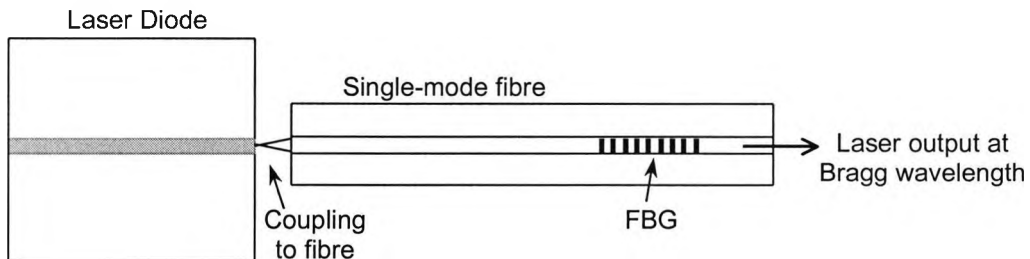
Fig. 2.9: A schematic of a “hybrid” FBG-based diode laser.
