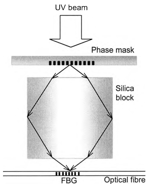
Fig. 2.5(a): Non-contact interferometric phase mask technique for grating writing using a silica block.
