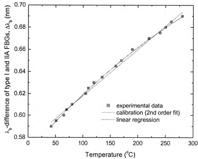
Fig. 6.28: Calibration graph for direct measurement of the strain independent temperature over the range of 25 - 300^\circ\text{C} . Solid and dotted lines represent the best polynomial ( 2^{\text{nd}} order) and the linear regression respectively.
