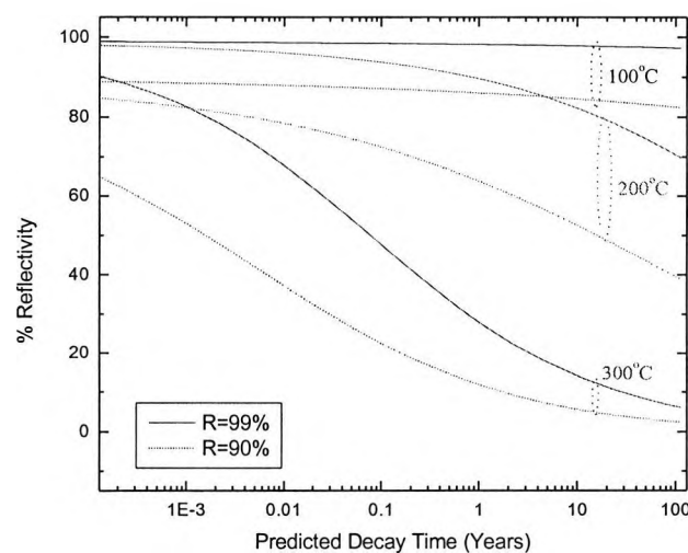
Fig. 4.8: Prediction of thermal decay of FBGs in terms of reflectivity, with initial reflectivity values of 99% and 90% at 100^\circ\text{C} , 200^\circ\text{C} and 300^\circ\text{C} over a simulated period of 100 years.
