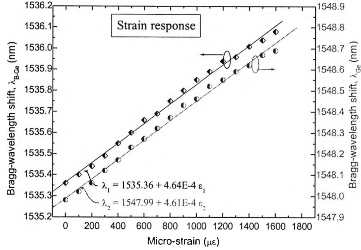
Fig. 6.4: Strain response of the grating-sensor.
