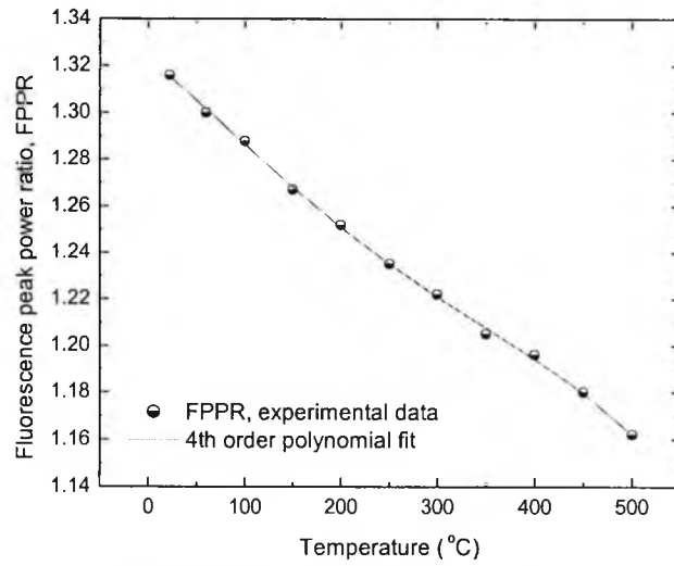
Fig. 6.8: Variation of FPPR with temperature (22-500)°C. The solid line is the best fitted 4 th order polynomial regression to the experimental data. The error-bars are smaller than the data points.
