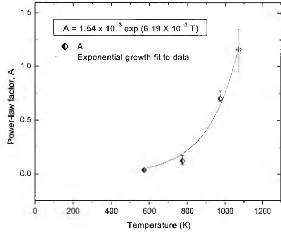
Fig. 4.13(b): Exponential fit for the Power-Law factor, A , in a linear scale.
