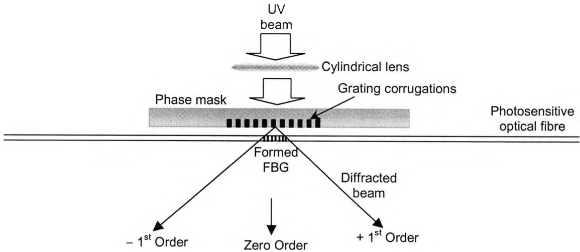
Fig. 2.4: A schematic of fabrication of FBGs using a phase mask.
