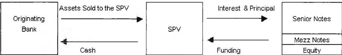
Figure 2.1: CDO diagram.
