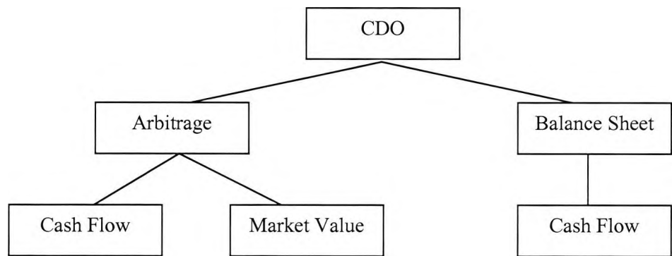
Figure 2.3: CDO structure.
