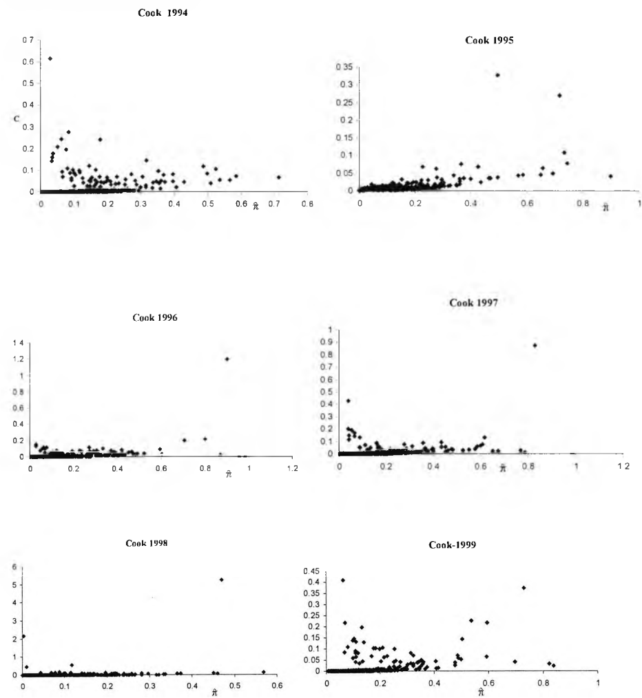
Figure 3.9.3 Cook's statistic
