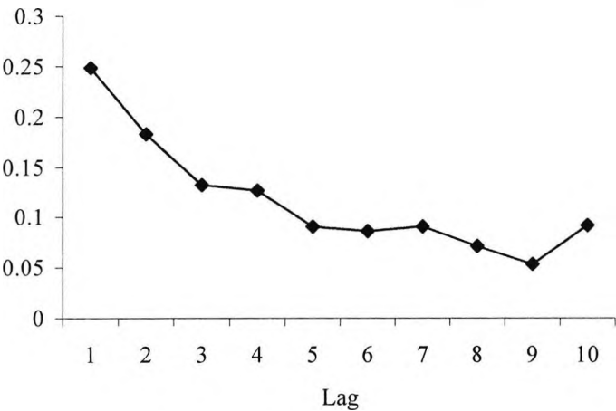
Figure 5.6: Autocorrelation Functions of Squared Returns
