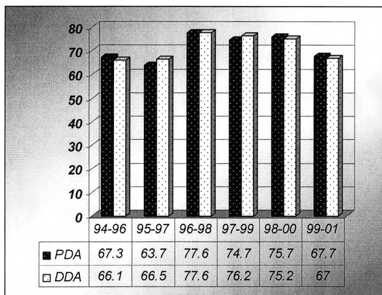
Figure 3.7.5: Overall Hit rates by both approaches
