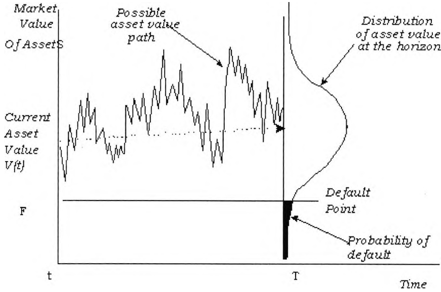
Figure 1.4: Default Probability in the Merton Model
