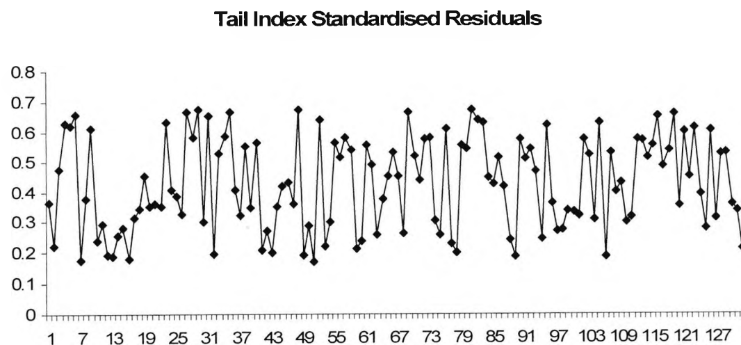
Figure 4.14 \xi Coefficient Estimates Residuals
