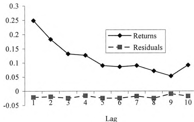
Figure 5.8 Autocorrelation Functions of Squared Series
