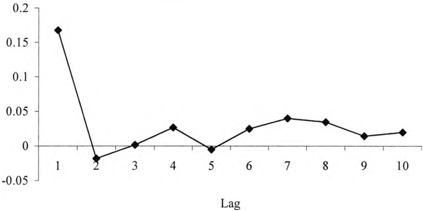
Figure 5.5: Autocorrelation Functions of Returns
