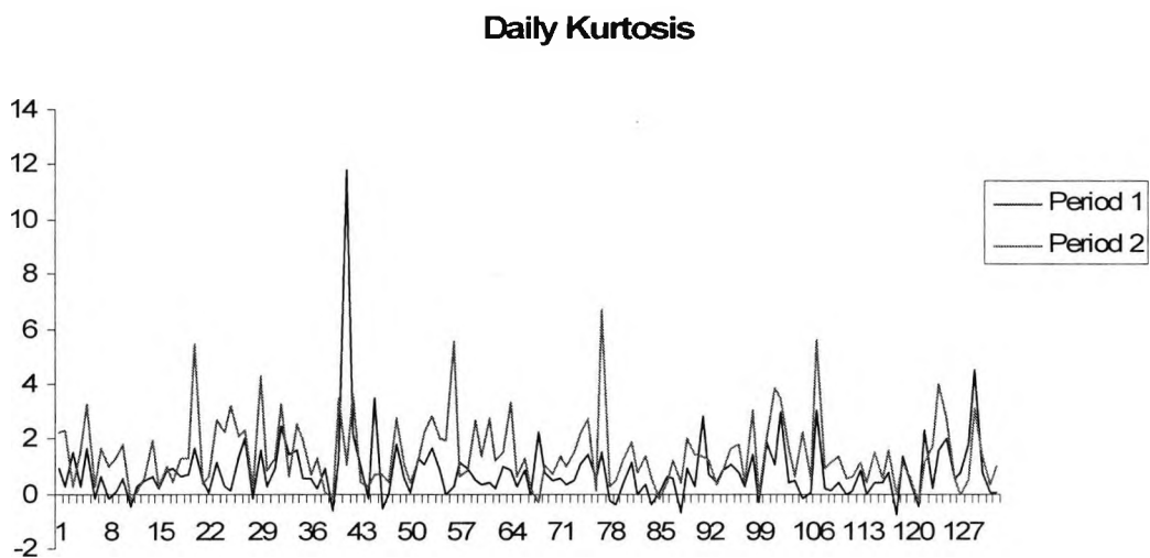
Figure 4.8: Excess Kurtosis Coefficient
