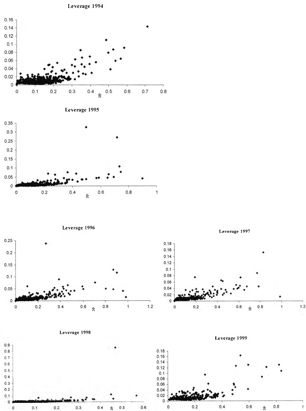
Figure 3.9.2 – Leverage Values
