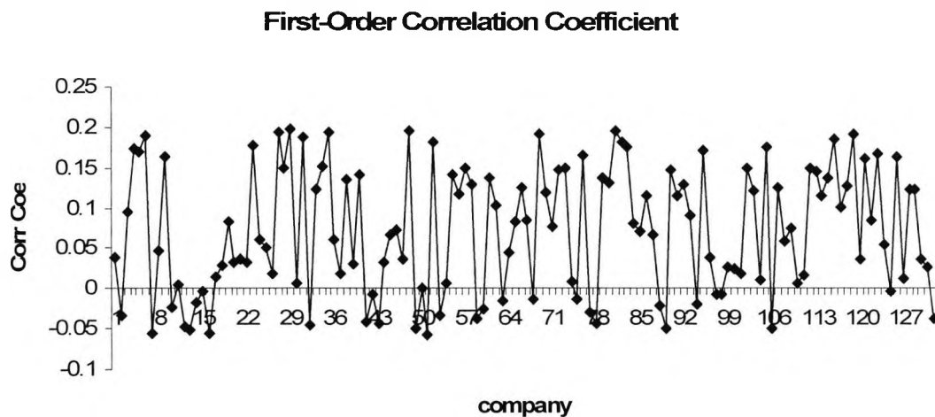
Figure 4.9 Autocorrelation Coefficient
