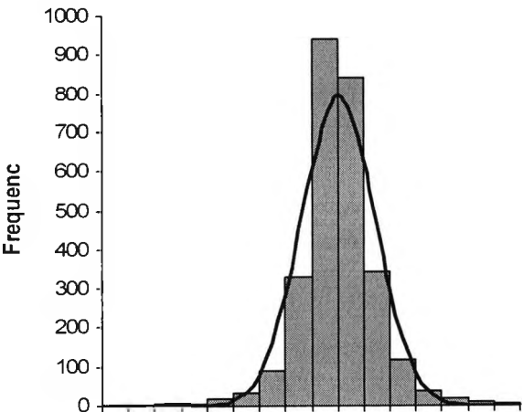
Figure 5.2: Frequency Distribution of Daily Returns of the General Index
