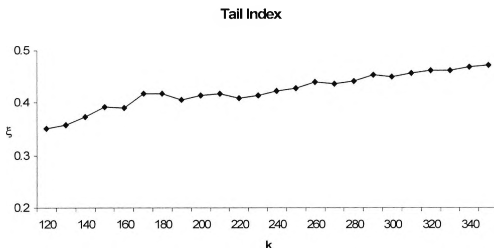
Figure 5.4 Estimated \xi for different k
