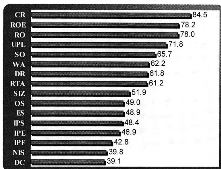
Figure 3.7.2: Ranking of factors in terms of group 1 average L-O-O hit rate n_{11}/n_1
