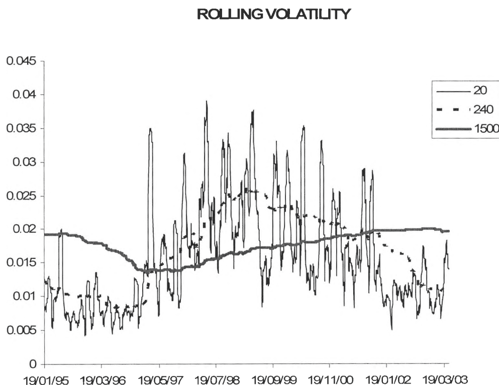
Figure 5.10: Rolling Volatility estimates based on different sample sizes
