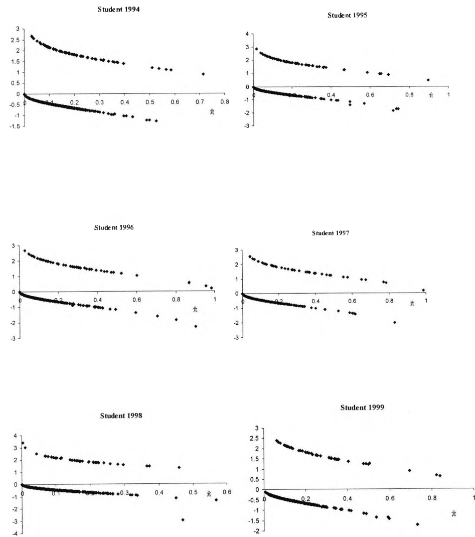
Figure 3.9.4 Studentized Residuals
