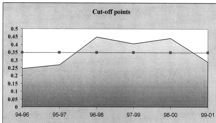
Figure 3.7.3 : Cut-off points
