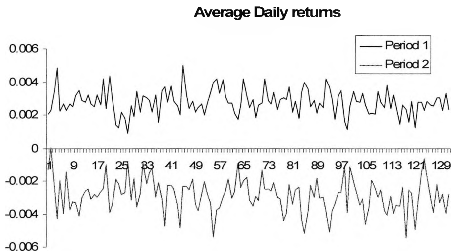
Figure 4.4: Average Daily Returns
