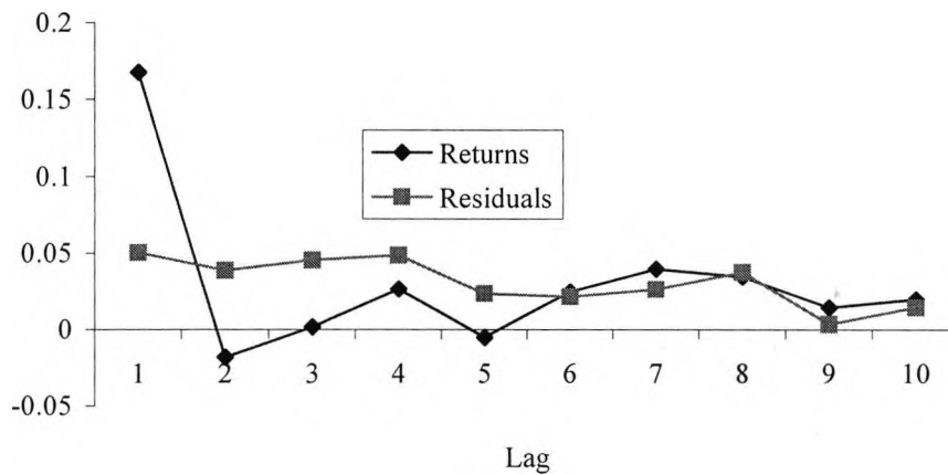
Figure 5.7: Autocorrelation Functions
