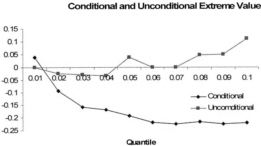
Figure 5.9: Comparison of the Conditional and Unconditional Extreme Value Quantiles
