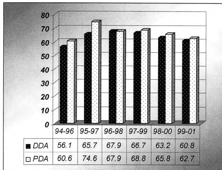
Figure 3.7.4 Hit rates for group 1 by the two approaches
