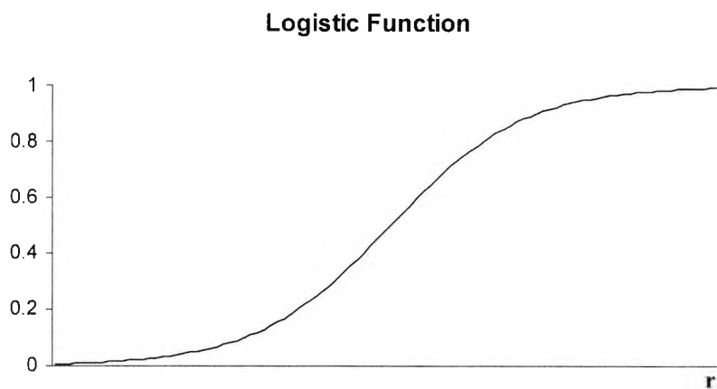
Figure 3.4.1: Logistic Function
