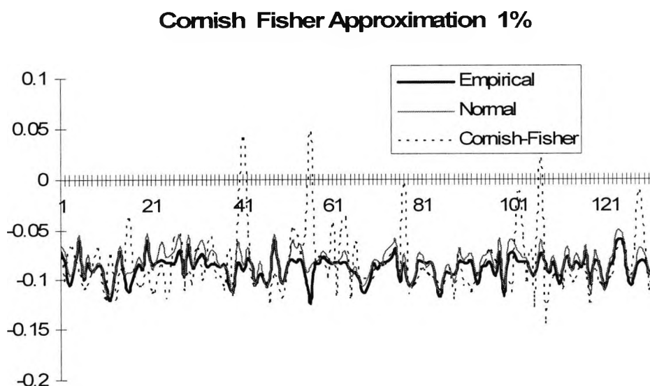
Figure 4.15 1% Quantile Estimation via Cornish –Fisher Approximation
