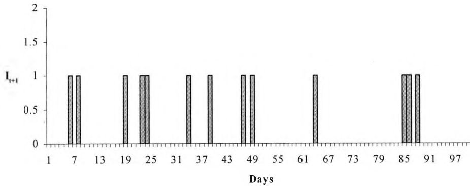
Figure 5.1: Hit Variable values
