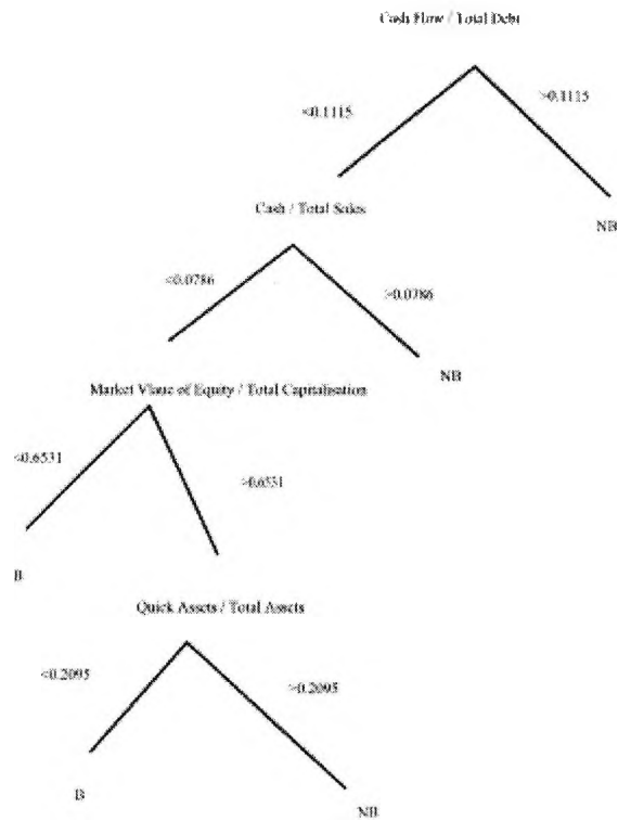
Figure 1.6: The RPA(1) Classification Tree
