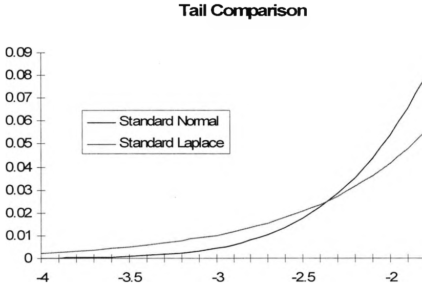
Figure 4.1: Kurtosis and Tails
