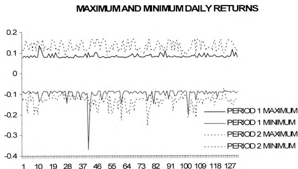
Figure 4.6: Maximum and Minimum Values of Daily Returns
