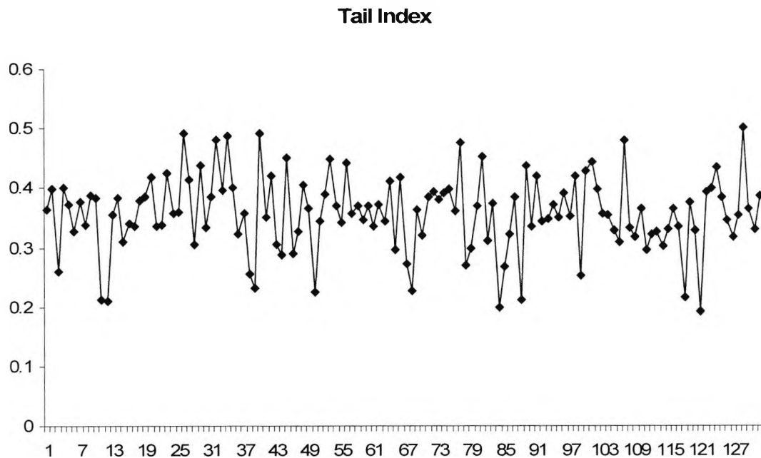
Figure 4.13 \xi Coefficient Estimates Raw Series
