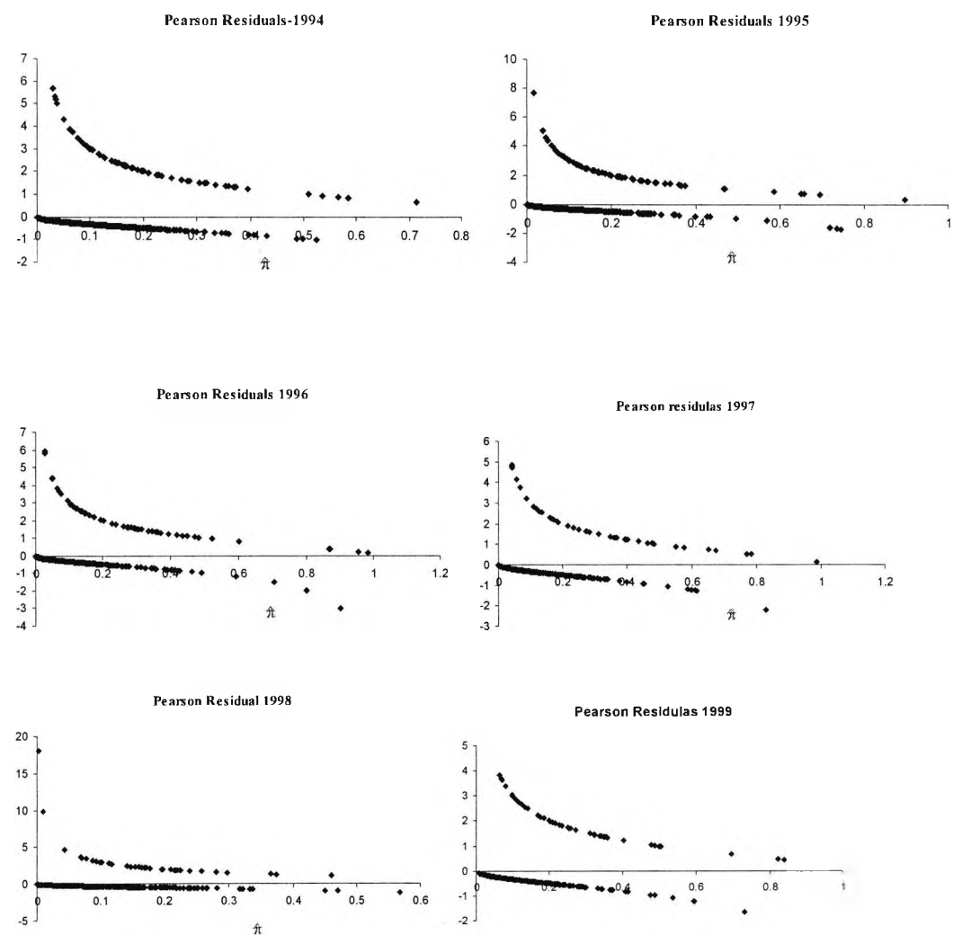
Figure 3.9.1 Pearson Residuals
