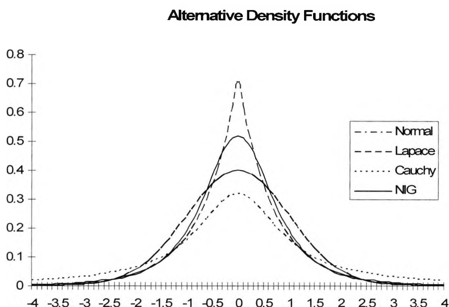
Figure 4.2: Example of Model Risk
