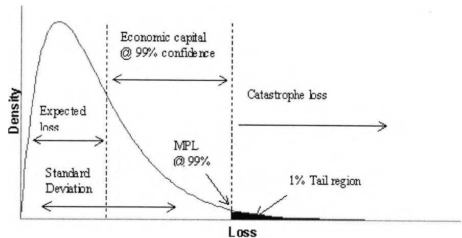
Figure 1.2: Value at Risk Definition
