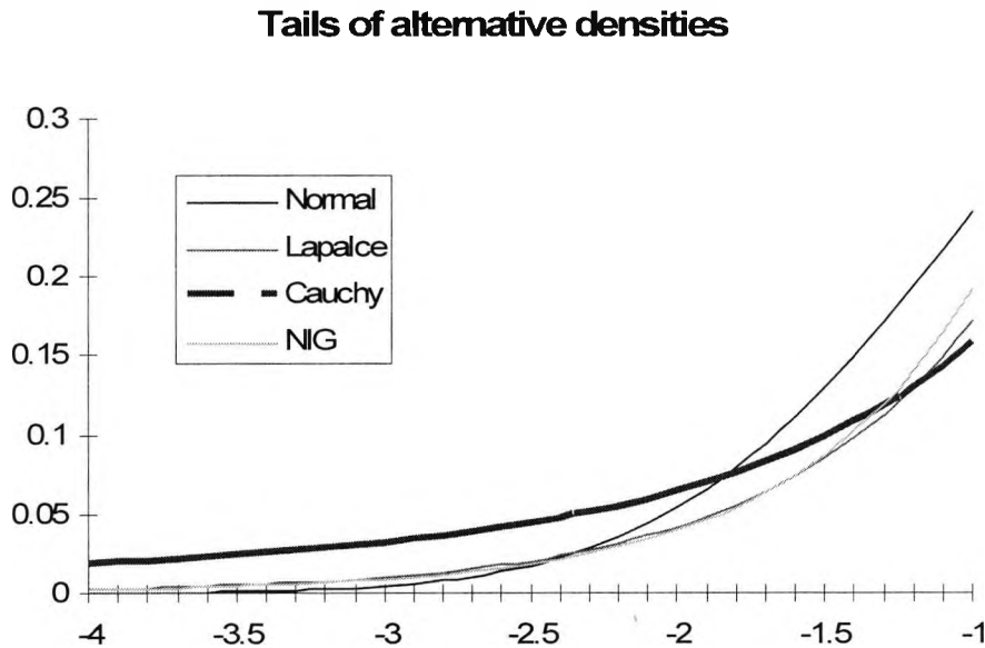
Figure 4.3: Model Risk and Tails
