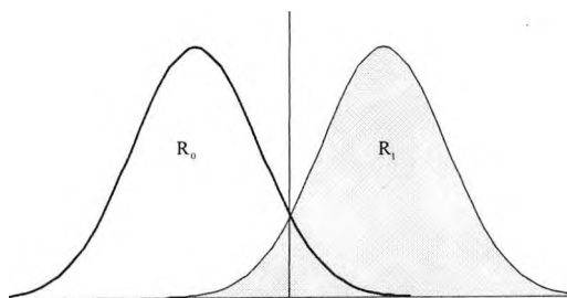
Figure 3.2.1: Classification regions
