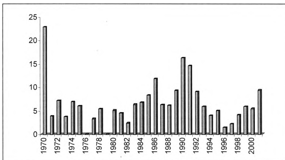
Figure 1.3: Annual Default Rates for a Moody's B rated company.
