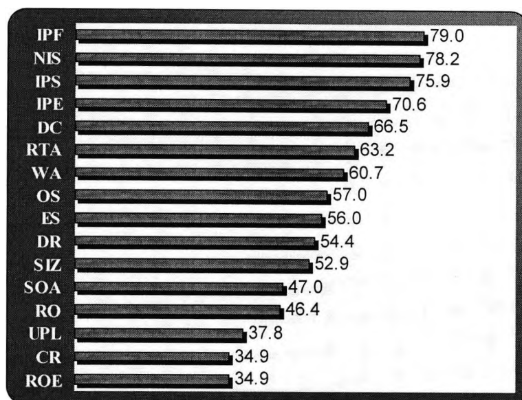
Figure 3.7.1: Ranking of Factors in terms of Group 0 average L-O-O hit rate ( n_{00}/n_0 ).
