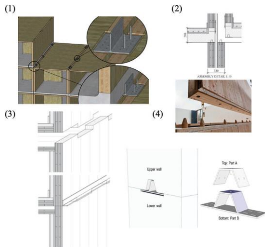
Figure 2: Novel connection systems for specific CLT volumetric projects: (1) Jakarta Hotel [6]; (2) Heidelberg Student Accommodation [3]; (3) Moxy Modular Hotels (Marriott) [3]; (4) A novel system proposed by the University of British Columbia [7]
