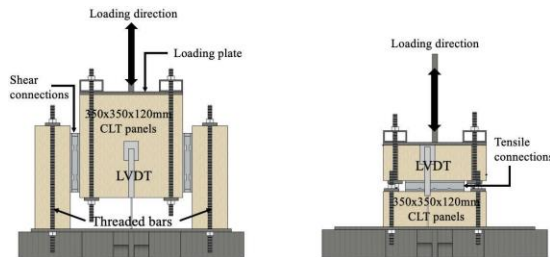
Figure 7: Experimental set-ups of the push-out (left) and pull-out test (right) on shear and tensile connectors
