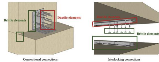
Figure 6: Capacity design of conventional plate connections (left) and novel interlocking connections with damage avoidance philosophy (right)
