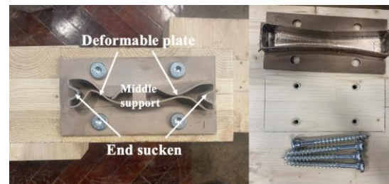
Figure 9: The tested shear connection specimens and screw removal
