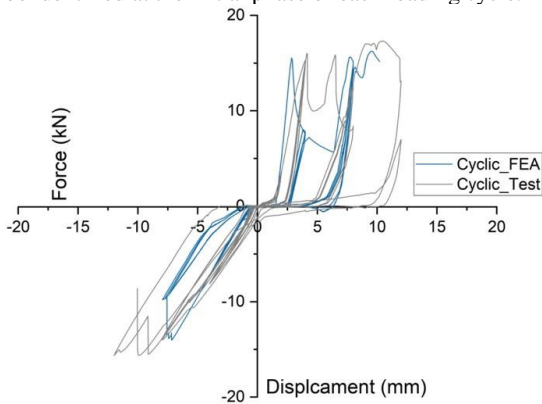
Figure 12: Force-displacement curve of the shear connection [8]
