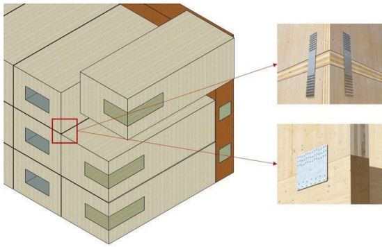
Figure 1: Illustration of inter-module connection locations and the conventional hold-down (top) and bracket (bottom) that could be used in CLT volumetric structures
