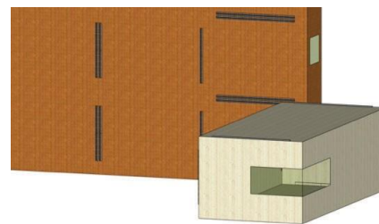
Figure 4: The preinstalled connections that are used as guiding system to assist modules installation
