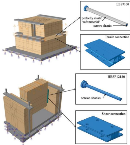
Figure 13: FE models for tensile connection (top) and shear connection (bottom) validation
