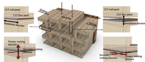
Figure 3: Interlocking tensile (left) and shear (right) connection and CLT modules assembly (middle) with the pre-installed connections
