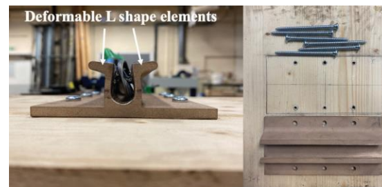
Figure 10: The tested tensile connection specimens and screw removal
