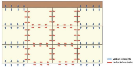
Figure 5: Continuous reinforcement along CLT modules edges provided by assembled connections [8J]
