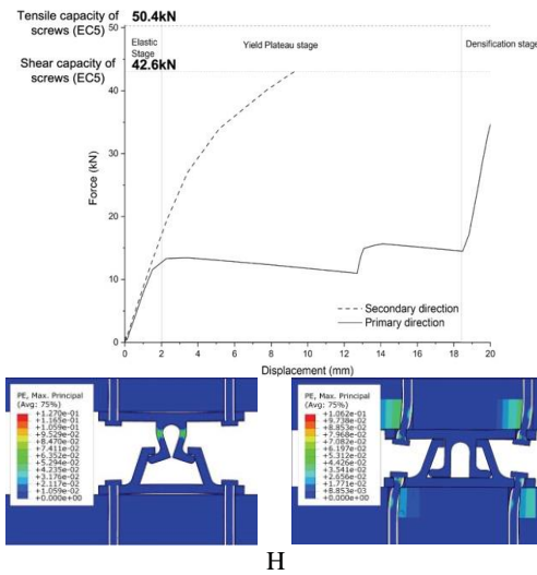
Figure 15: Force and displacement curve of tensile connection with S235 and connection deformation on primary (bottom left) and secondary directions (bottom right) under 15mm displacement [8J]
