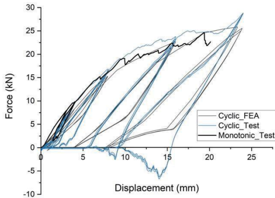
Figure 11: Force-displacement curve of the tensile connections [8]
