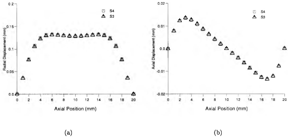
Figure 4.13: Comparisons of the predicted (a) radial, and (b) axial displacements using general purpose three-node and four-node shell elements.
