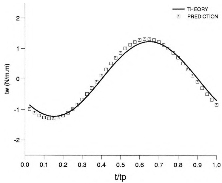
Figure 4.16: Predicted (symbols) and analytical (lines) wall shear stress for oscillatory flow in an elastic tube.
