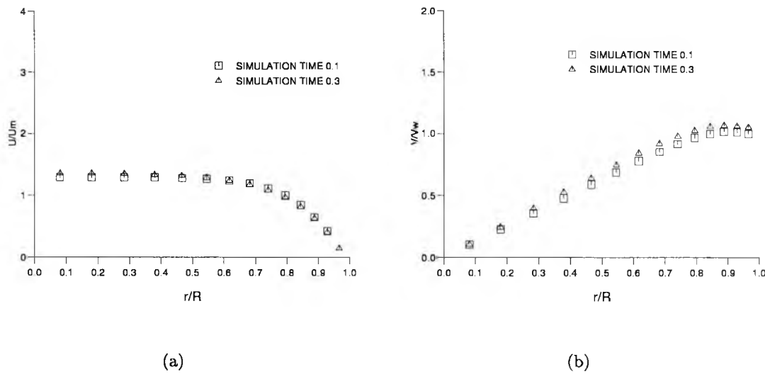
Figure 4.2: Comparisons of the distributions of (a) axial, and (b) radial velocity in an contracting tube with Re=-10.0 , between simulation time of 0.1s and simulation time of 0.3s.
