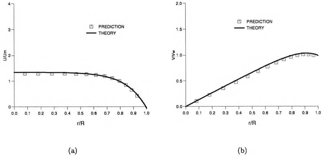
Figure 4.1: Comparisons of the distributions of (a) axial, and (b) radial velocity in an contracting tube with Re=-10.0 , and simulation time of 0.1s.
