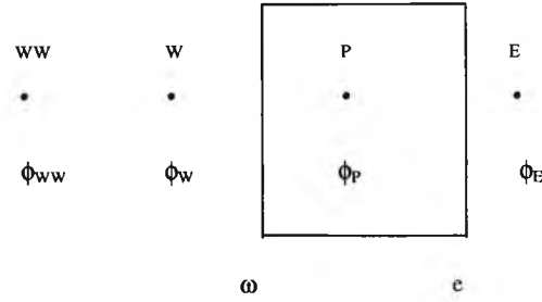
Figure 3.3: Control volume notation.
