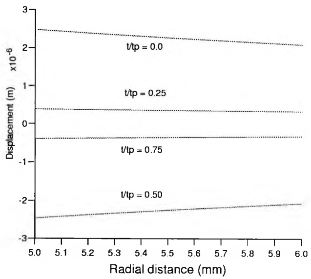
Figure 4.17: Predicted distribution of radial displacements across the wall (elastic model).
