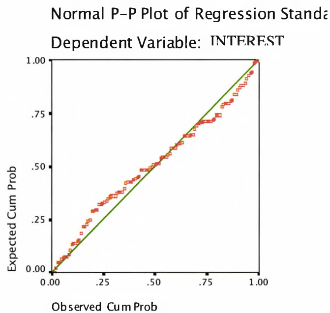
Exhibit VI-f: Normal P-P Plot of Residuals
