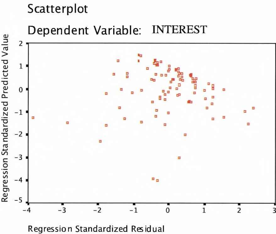
Exhibit VI-d: Standardized Predicted Variable and Residuals
