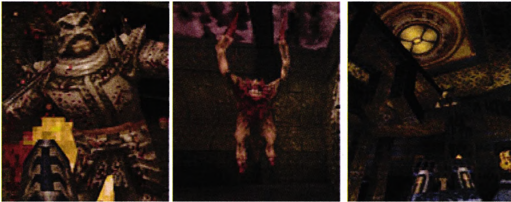
Exhibit VII-c: Quake Statistics
