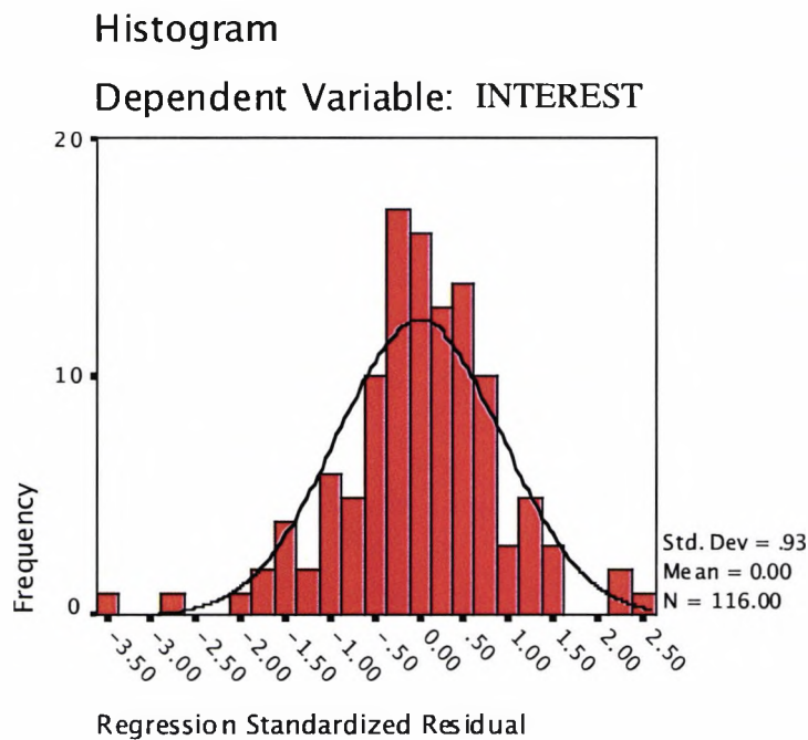
Exhibit VI-e: Histogram of Idealized Normal Curve
