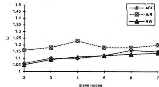
Fig 10-28. ZIFF-DAVIS [Replication]: restricted iterations on CSP algorithm, load imbalance (AP3000)
