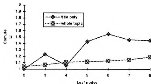
Fig 9-14. BASE1: Type B retrieval efficiency, computational load imbalance for passage retrieval
