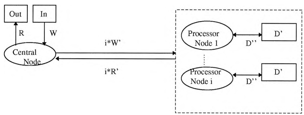
Fig 1-4: Example of abstract task on inverted file partitioning.
