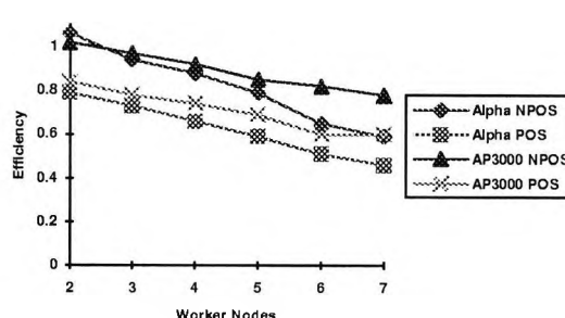
Fig 6-13. BASE1 distributed build [TermId]: indexing efficiency (WC only)
