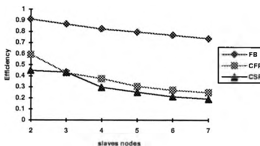
Fig 10-21. ZIFF-DAVIS [Replication]: add reweight operation parallel efficiency for term selection (AP3000)
