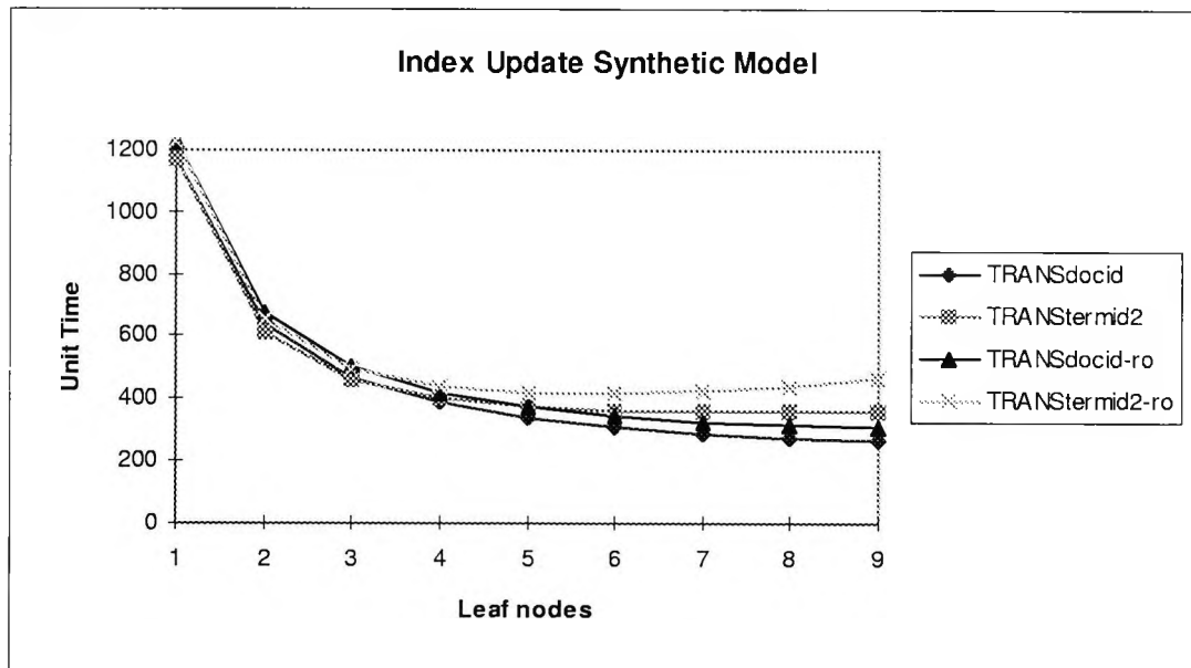
Fig 5-12. Comparison between partitioning methods in presence and absence of index update
