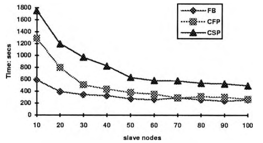
Fig 10-32. ZIFF-DAVIS [On-the-fly]: add only average term selection elapsed time in seconds (AP1000)
