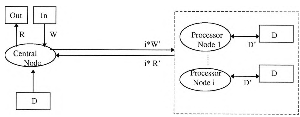
Fig 1-3: Example of abstract task on inverted file replication.
