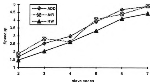
Fig 10-26. ZIFF-DAVIS [Replication]: restricted iterations on CSP algorithm, speedup (AP3000)
