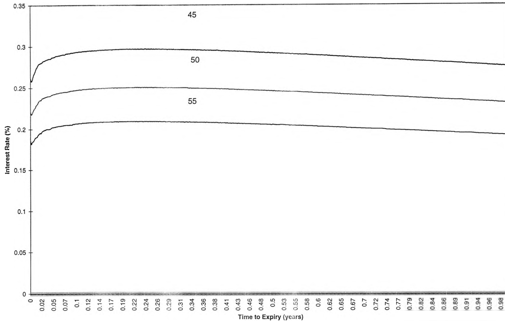
Figure 5: Brennan-Schwartz model, 5 year bond, 1year put option
