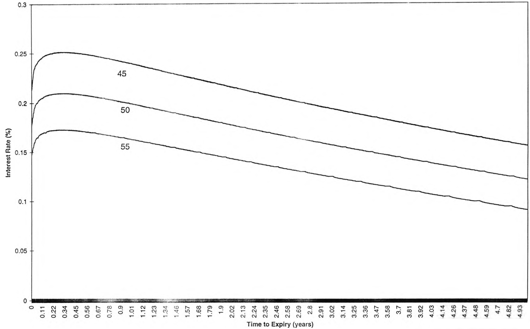
Figure 6: Brennan-Schwartz model, 10 year bond, 5 year put option
