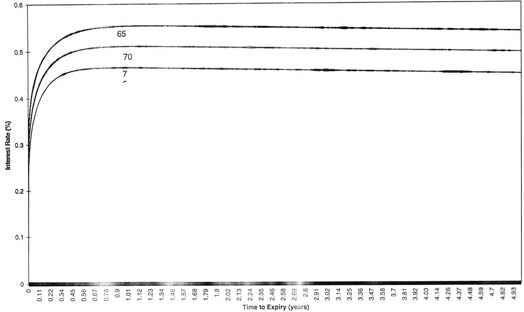
Figure 2: Vasicek model, 10 year bond, 5 year put option
