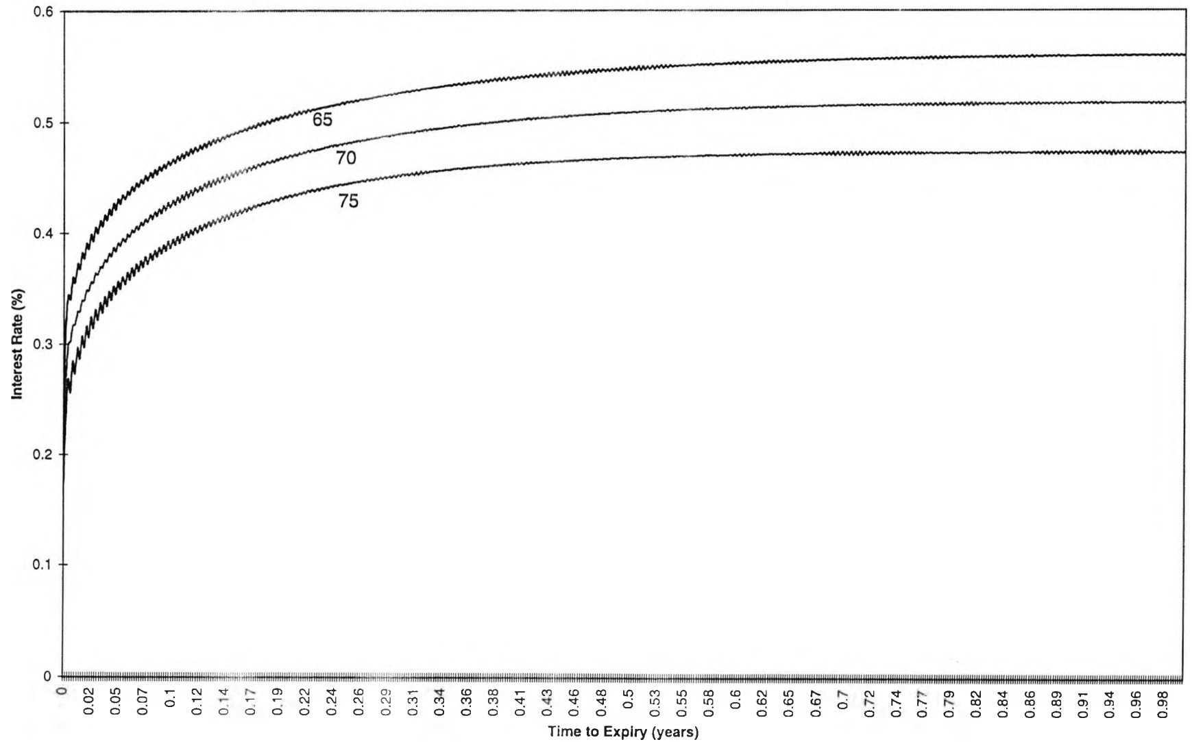
Figure1: Vasicek model, 5 year bond, 1 year put option
