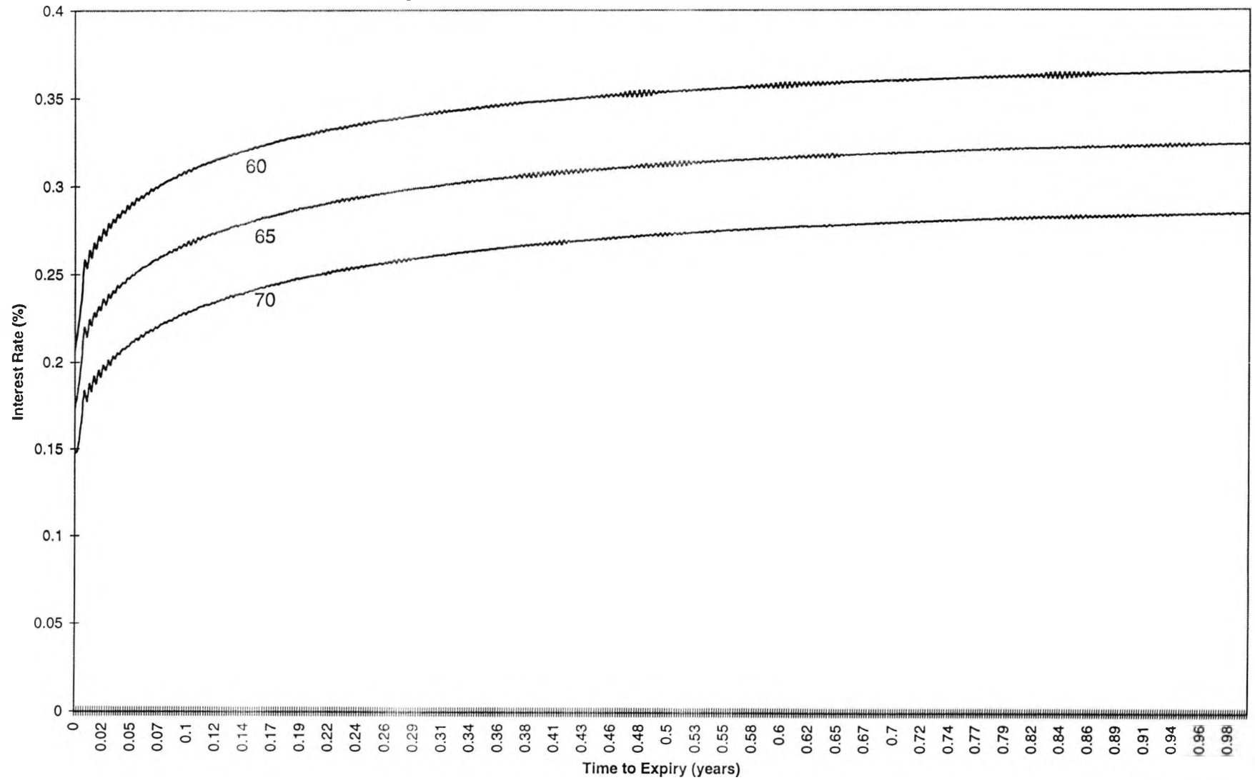
Figure 3: CIR model, 5 year bond, 1 year put option
