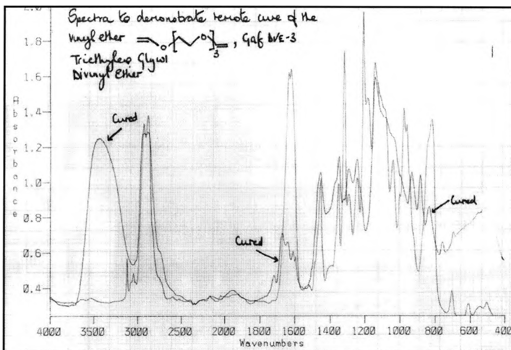
Figure 3.3-34 IR Spectra, Remote cure of Diethylene Glycol Divinyl Ether
