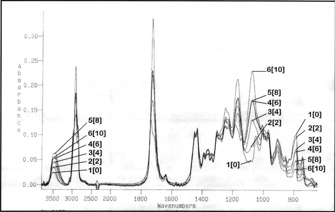
Figure 6.5-2 Remote curing in PTFE apparatus, IR spectra for remote curing of epoxide, 0.2g DPIHFP, resin formulation 4, film thickness = 4 µm +/- 1 µm
