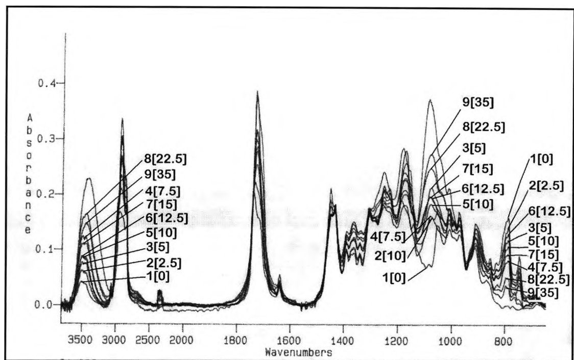
Figure 6.4-1 Remote curing in PTFE apparatus, IR spectra for remote curing of epoxide, 0.2g Irgacure 261, resin formulation 4
