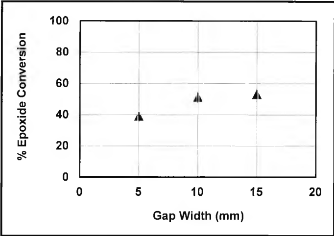
Figure 3.3-10 Remote cure, effect of gap width on epoxide
