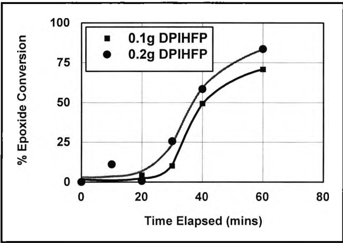
Figure 3.3-27 Remote curing, effect of doubling initiator quantity on epoxide conversion
