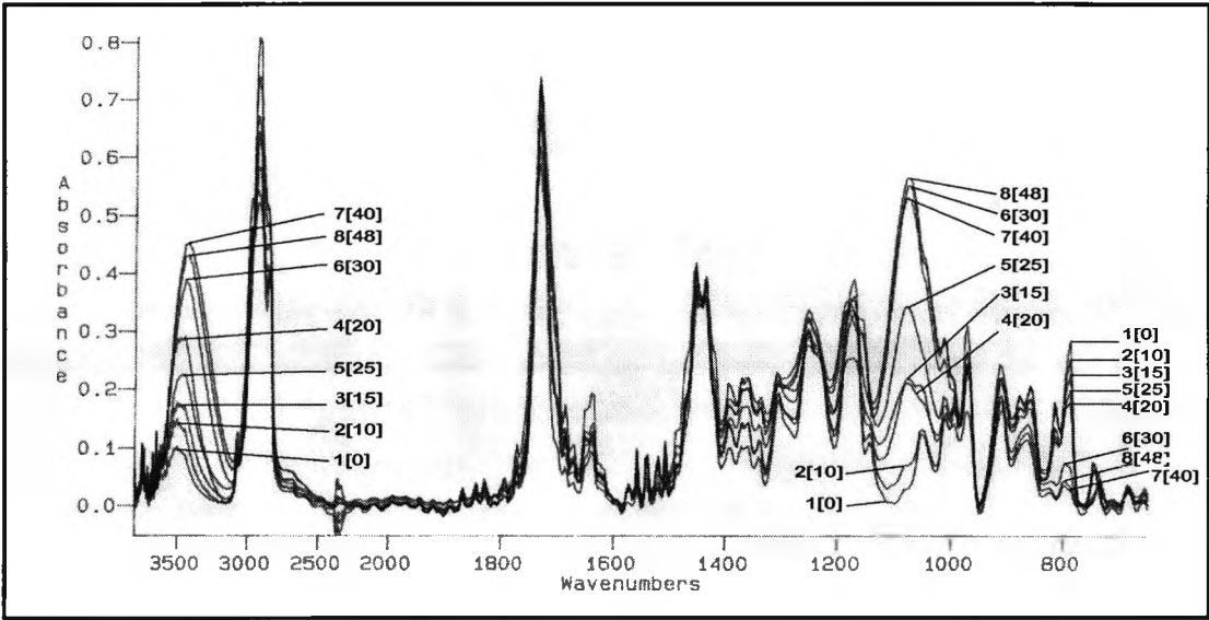
Figure 6.2-1 Remote curing in glass apparatus, IR spectra for remote curing of epoxide, 0.1g DPIHFP, resin formulation 1
