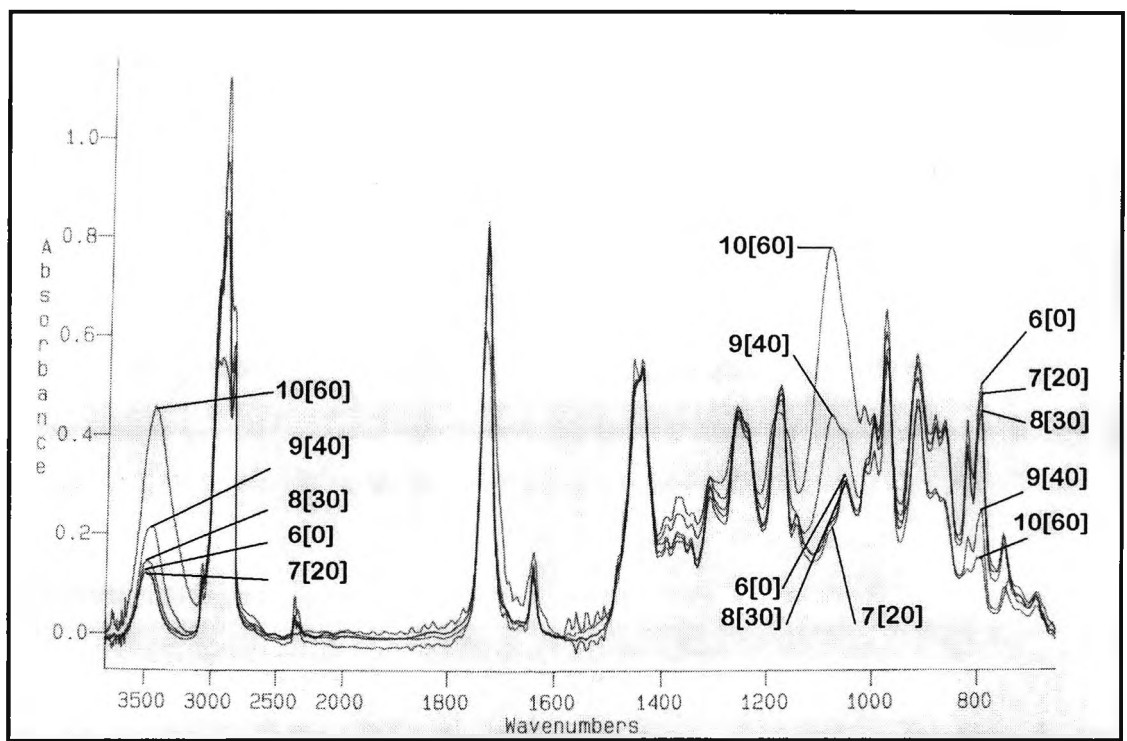
Figure 6.10-2 Remote curing in glass apparatus, IR spectra for remote curing of epoxide, 0.1g DPIHFP, resin formulation 1
