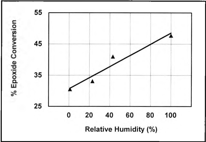
Figure 3.3-20 Remote cure, epoxide conversion at various levels of humidity
