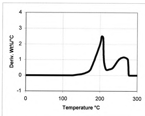
Figure 2.2-10 1st derivative TGA profile for DPIHFP
