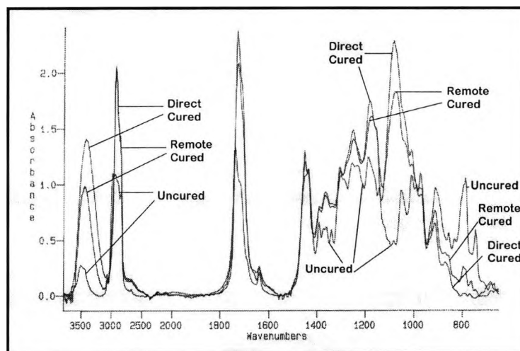
Figure 3.3-9 Comparison of IR spectra for epoxide cured by remote and direct methods
