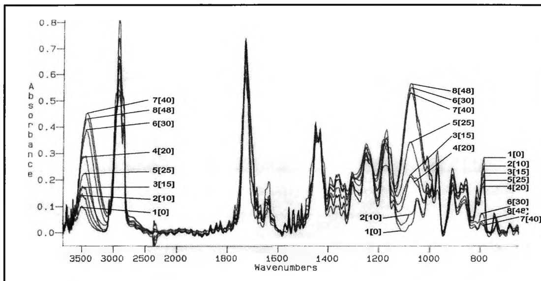
Figure 3.3-4 Remote curing, IR spectra for remote curing of epoxide
