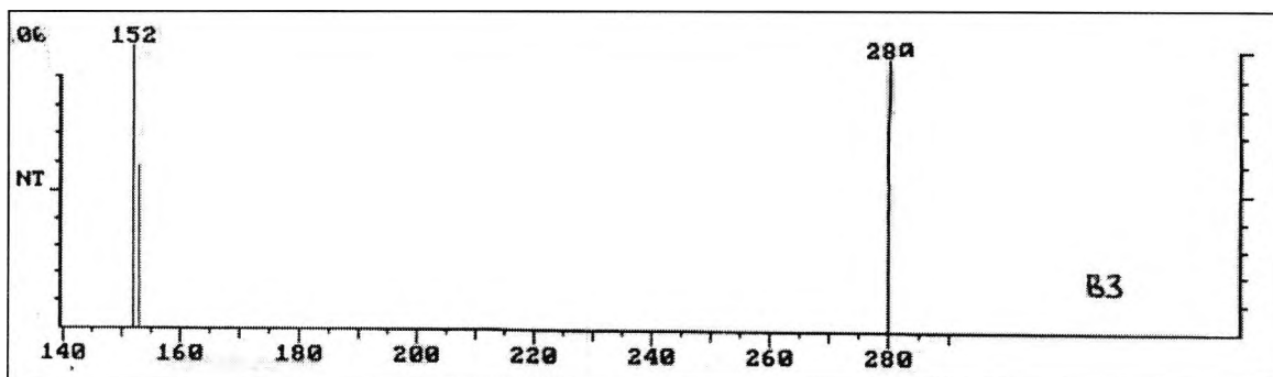
Figure 5.2-4 MS for GC fraction B3 at reference time 350, product obtained from UV irradiation of solid state DPIHFAs
