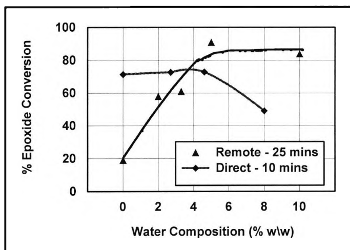
Figure 3.3-24 Effect of bulk water on epoxide conversion in direct and remote curing
