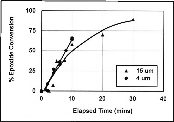
Figure 3.3-14 Remote Cure, effect of film thickness on epoxide conversion – reaction profiles at 4µm and 15µm thickness
