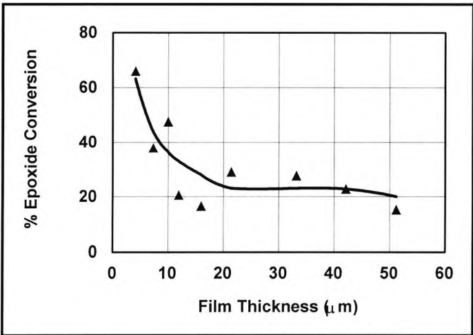
Figure 3.3-15 Remote cure, variation in epoxide conversion with film thickness
