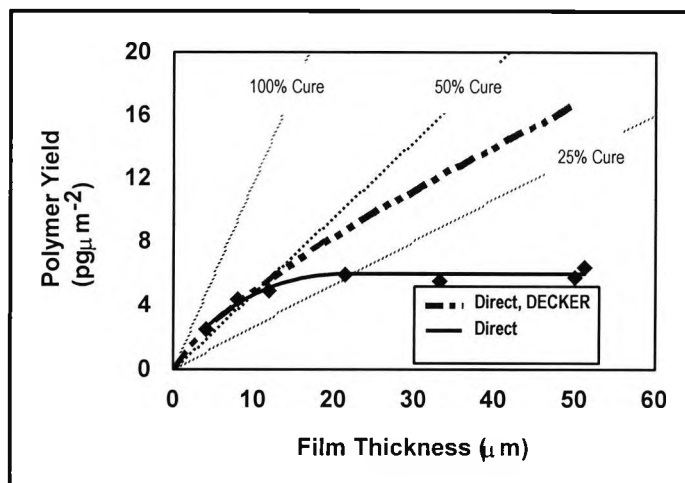
Figure 3.3-17 Direct cure, effect of epoxide film thickness on polymer yield – comparison of experimental and literature data
