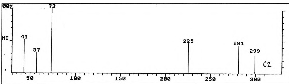
Figure 5.3-3 MS for GC fraction C2 at reference time 365, product obtained from UV irradiation of solid state TPSHFSb
