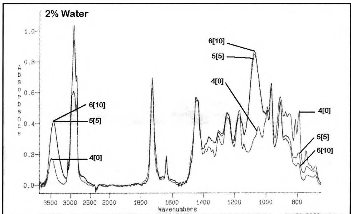
Figure 6.9-2 Direct curing, IR spectra for direct curing of epoxide, 1.5% w/w DPIHFP, resin formulation 9, 0-10 mins. of UV exposure and 2% w/w added bulk water
