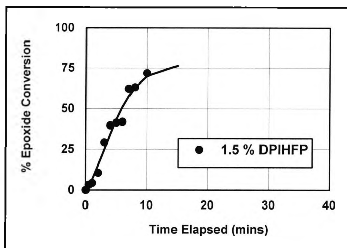
Figure 3.3-2 Direct Curing, epoxide conversion for direct cure
