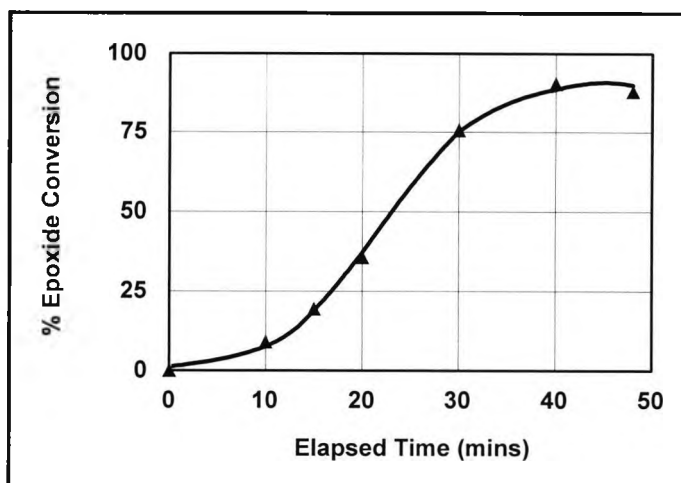
Figure 3.3-6 Remote curing, epoxide conversion, in glass apparatus
