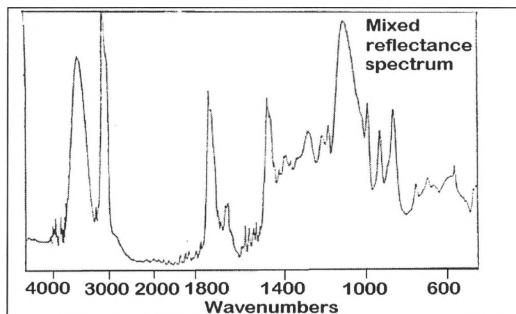
Figure 3.2-10 Mixed reflectance IR spectrum of uncured epoxide formulation – typical conditions
