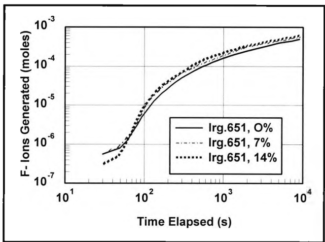
Figure 2.3-13 Fluoride ion evolution following UV irradiation of solid-state DPIHFP in the presence of Irg.651
