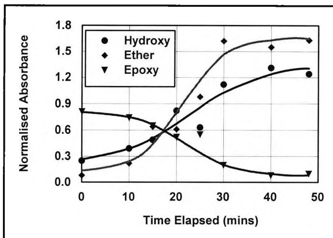
Figure 3.3-5 Remote curing, IR absorbance band for relevant groups in remote epoxide polymerisation
