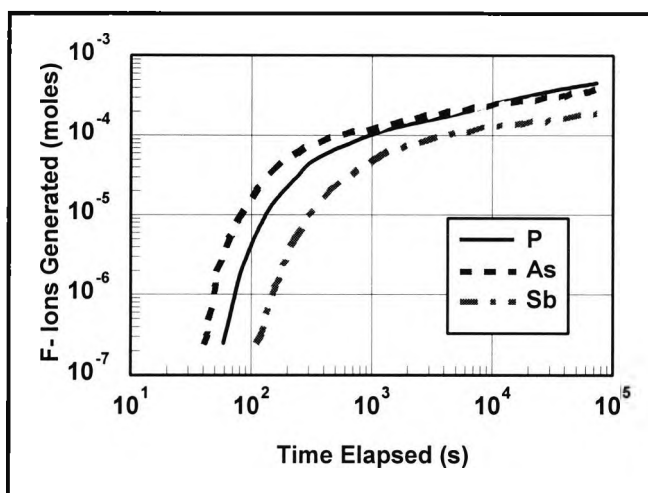
Figure 2.3-8 Fluoride evolution following UV irradiation of solid-state DPI hexafluoro-(group 5) salts
