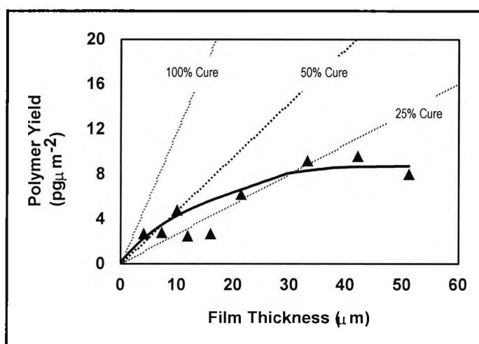
Figure 3.3-18 Remote cure, effect of epoxide film thickness on polymer yield
