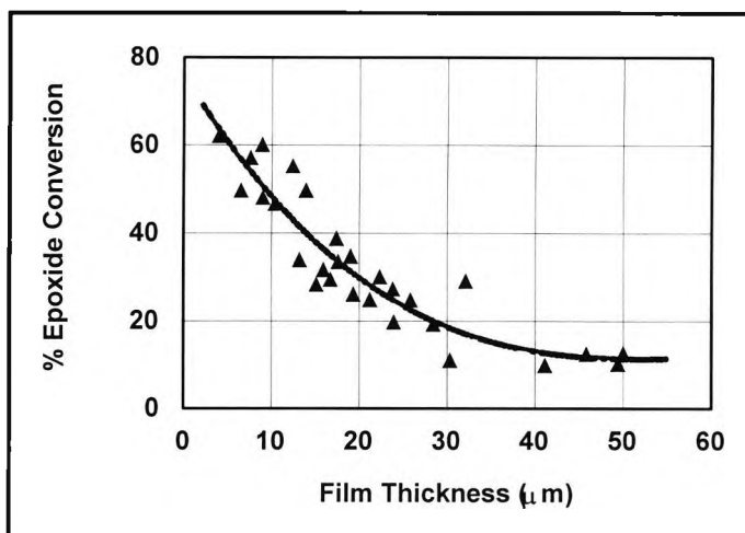
Figure 3.3-16 Direct cure, variation in epoxide conversion with film thickness
