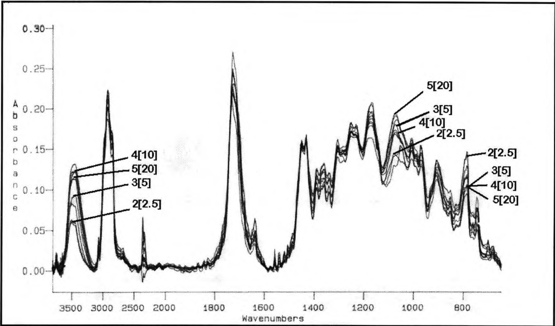
Figure 6.2-3 2-step remote curing in PTFE apparatus, IR spectra for 2-step remote curing of epoxide, 0.2g DPIHFP, resin formulation 4
