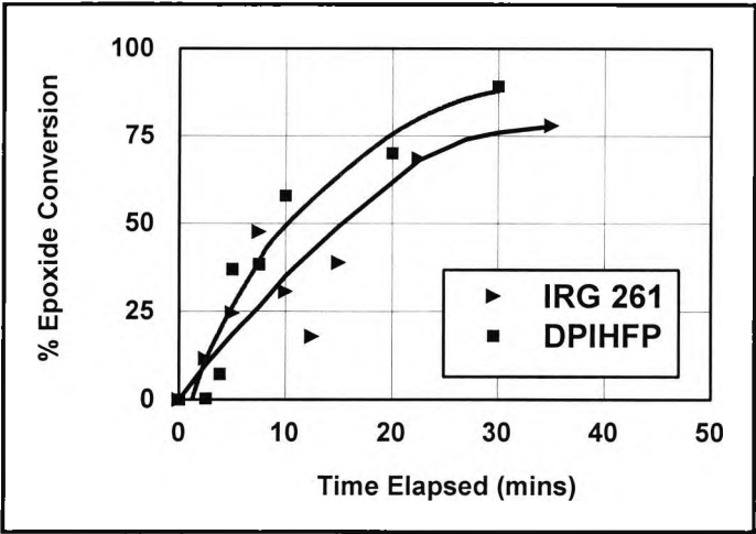
Figure 3.3-11 Remote cure, epoxide conversion in remote cure with DPIHFP and Irg261 initiators
