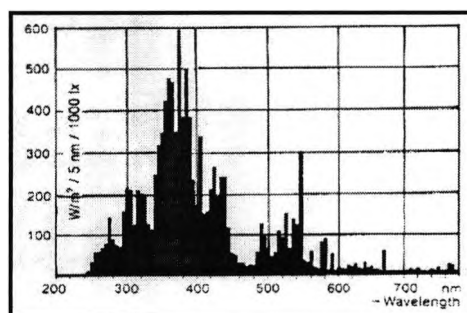
Figure 2.2-4 'D bulb' UV spectral output for solid-state photodecomposition experiments
