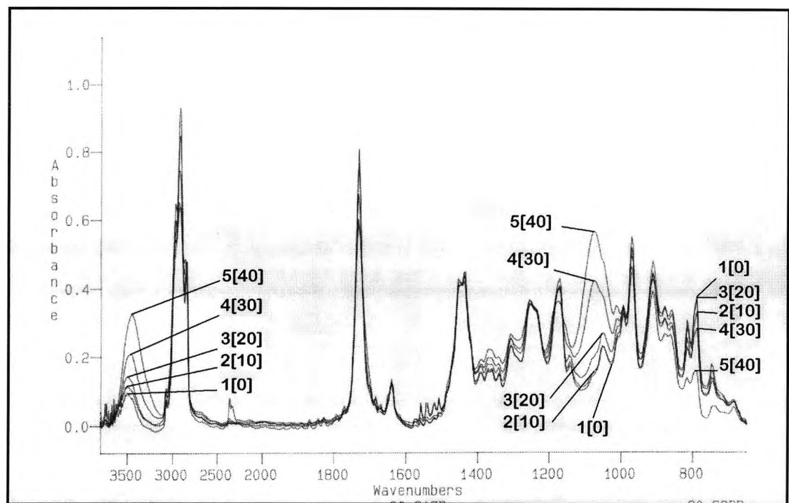
Figure 6.10-1 Remote curing in glass apparatus, IR spectra for remote curing of epoxide, 0.2g DPIHFP, resin formulation 1
