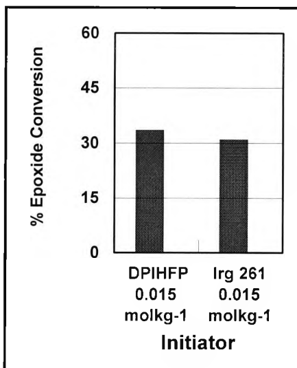
Figure 3.3-13 Direct cure, epoxide conversion in direct cure of epoxide with DPIHFP and Irg261 initiators
