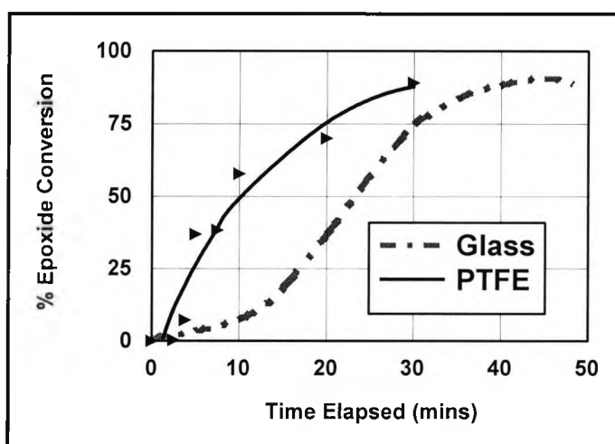
Figure 3.3-7 Remote curing, comparison of epoxide conversion in glass and PTFE apparatus
