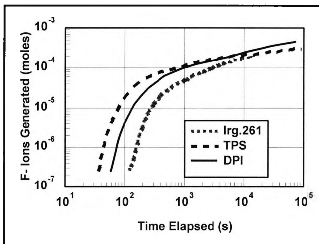
Figure 2.3-11 fluoride ion evolution following irradiation of various solid-state initiators bearing the HFP anion - effect of cation variation
