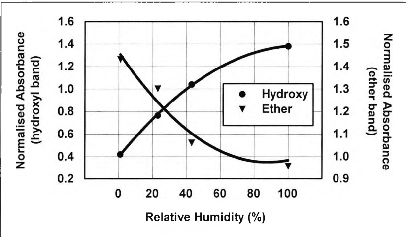
Figure 3.3-21 Remote cure, development of ether and hydroxyl IR spectral bands as a function of humididty
