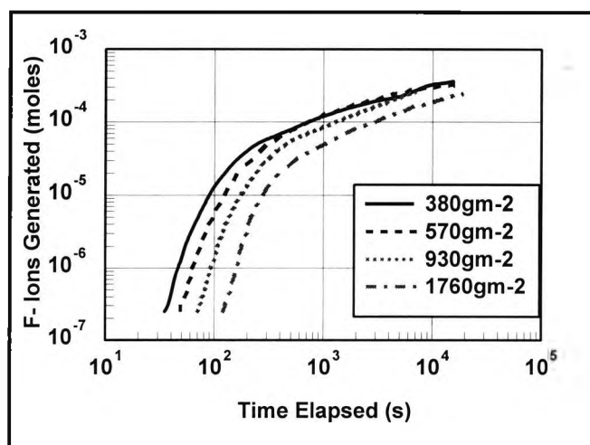
Figure 2.3-15 Fluoride ion evolution following UV irradiation of solid-state Irg.261 at various surface density values - effect of photoinitiator surface density
