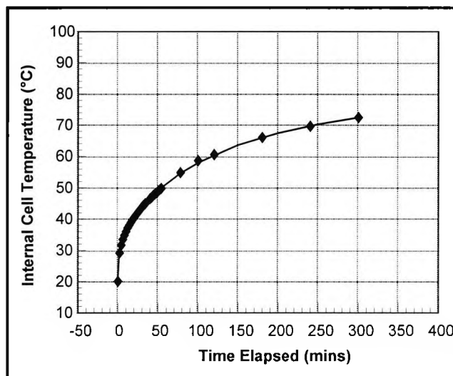
Figure 2.2-9 Temperature rise within PTFE photodecomposition cell as a function of UV irradiation time
