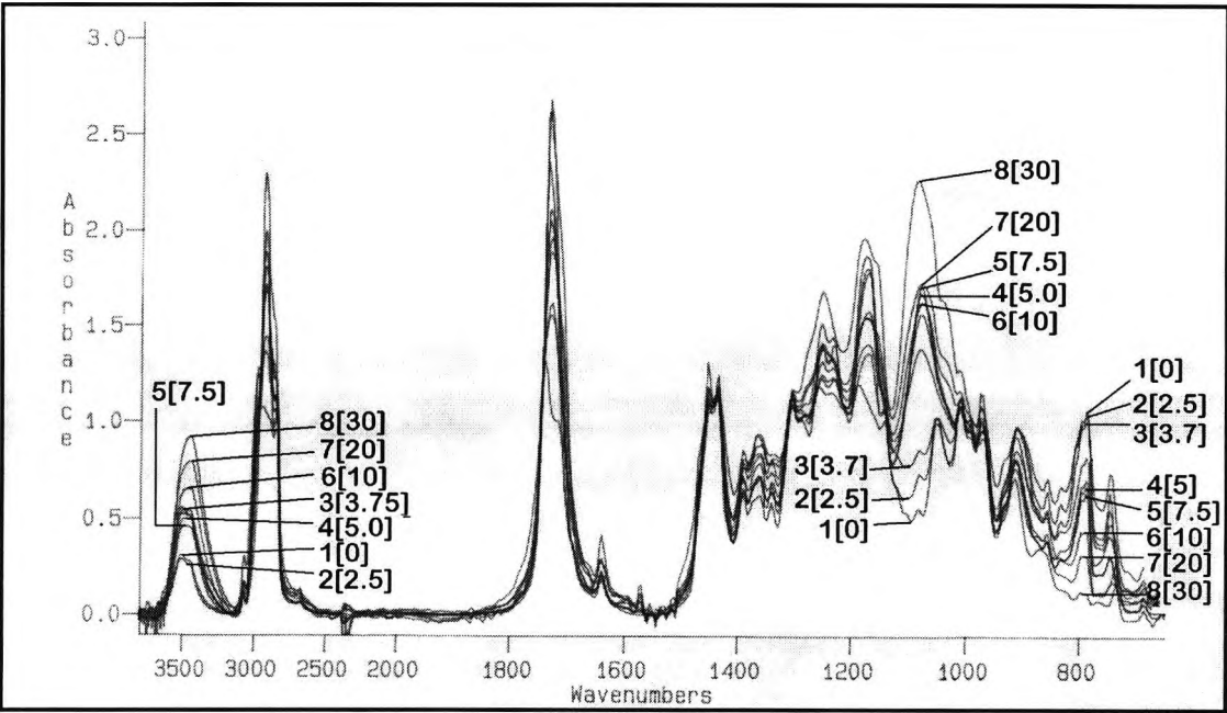
Figure 6.2-2 Remote curing in PTFE apparatus, IR spectra for remote curing of epoxide, 0.2g DPIHFP, resin formulation 4
