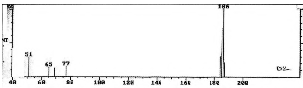
Figure 5.4-3 MS for GC fraction D2 at reference time 326, product obtained from UV irradiation of solid state TPSHFSb
