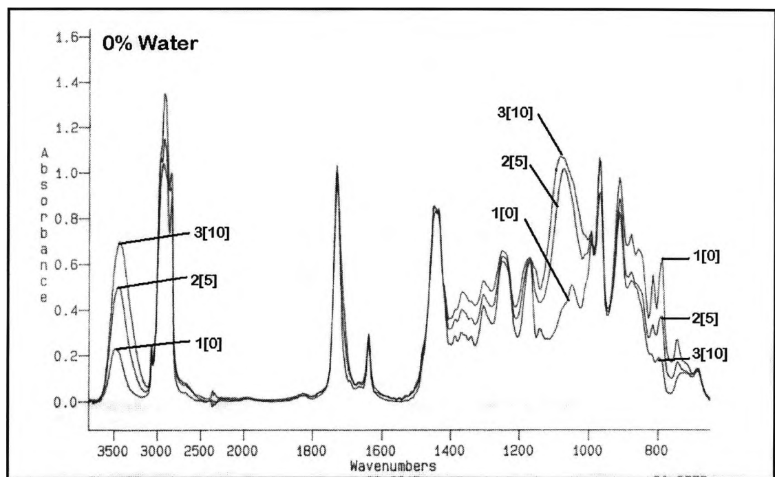
Figure 6.9-1 Direct curing, IR spectra for direct curing of epoxide, 1.5% w/w DPIHFP, resin formulation 2, 0-10 mins. of UV exposure and no added bulk water
