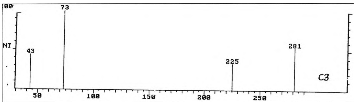
Figure 5.3-4 MS for GC fraction C3 at reference time 407, product obtained from UV irradiation of solid state TPSHFSb
