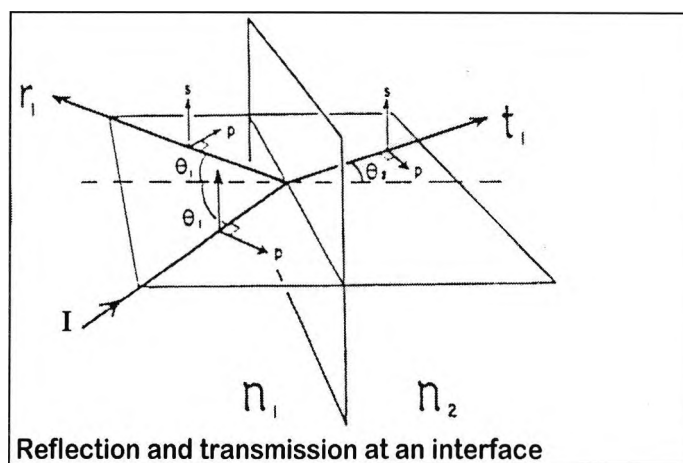
Figure 3.2-5 Optical paths at an interface between transmitting media having different refractive index values
