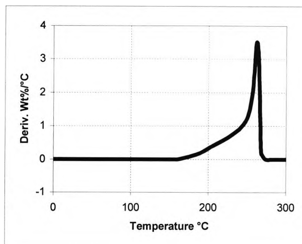
Figure 2.2-11 1st derivative TGA profile for Irgacure 261
