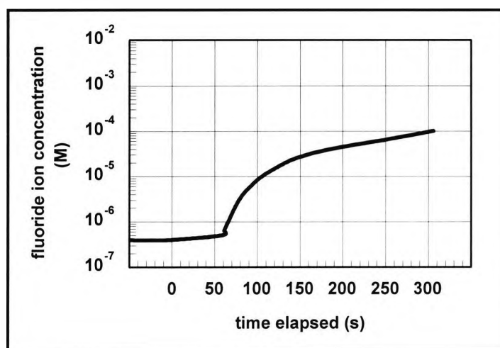
Figure 2.2-6 Onset of fluoride ion detection (FSE) with UV irradiation of solid-state photoinitiator
