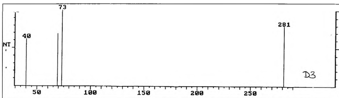
Figure 5.4-4 MS for GC fraction D3 at reference time 403, product obtained from UV irradiation of solid state TPSHFSb
