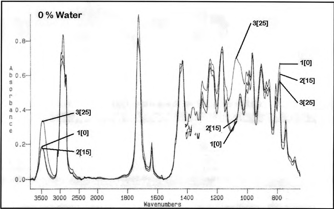
Figure 6.8-1 Remote curing in glass apparatus, IR spectra for remote curing of epoxide, 0.1g DPIHFP, resin formulation 1, 0-25 mins. of UV exposure and no added water
