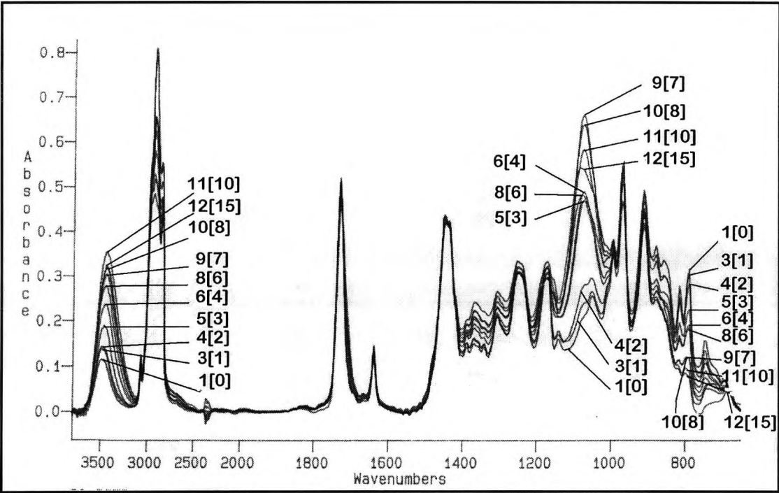
Figure 6.1-1 Direct curing, IR spectra for direct curing of epoxide, 1.5%DPIHFP, resin formulation 2
