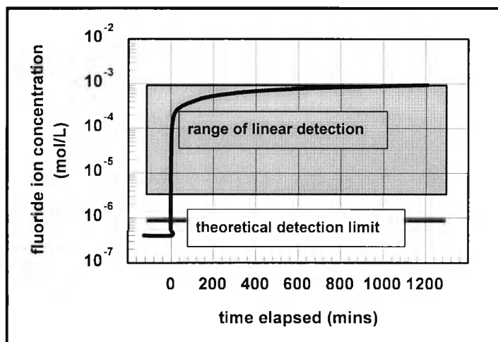
Figure 2.2-5 Typical XY output – fluoride ion detection (FSE) with UV irradiation of solid-state photoinitiator
