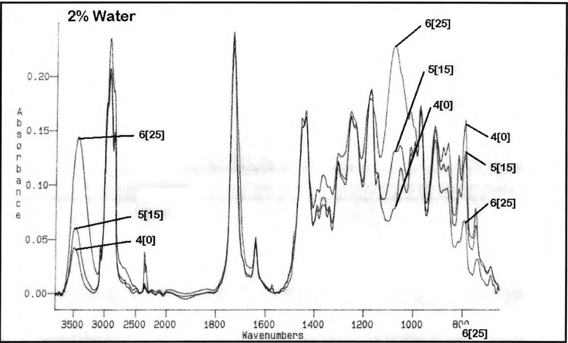
Figure 6.8-2 Remote curing in glass apparatus, IR spectra for remote curing of epoxide, 0.1g DPIHFP, resin formulation 5, 0-25 mins. of UV exposure and 2% w/w added bulk water
