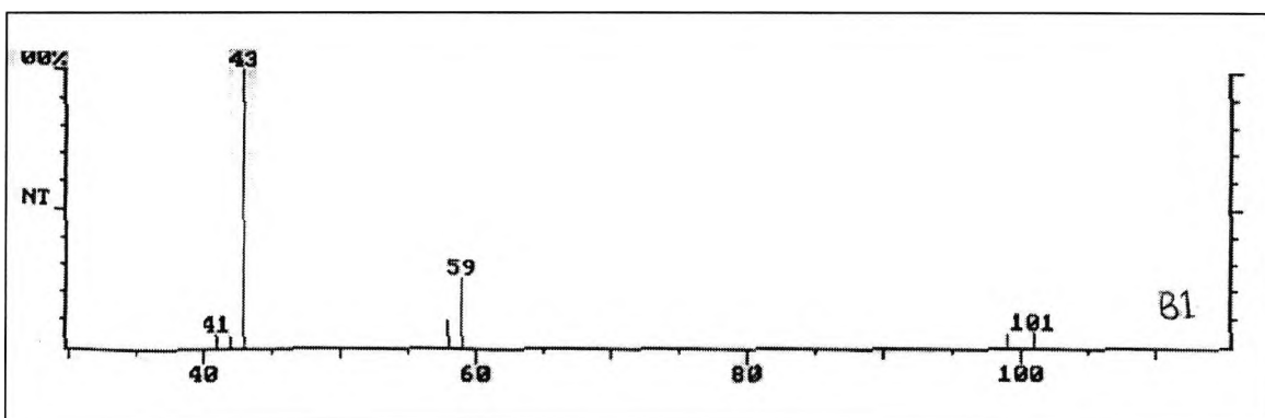
Figure 5.2-2 MS for GC fraction B1 at reference time 89, product obtained from UV irradiation of solid state DPIHFAs
