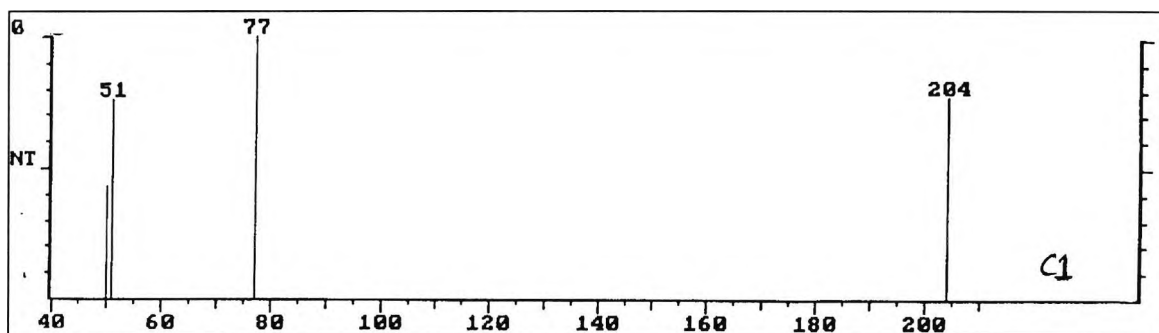
Figure 5.3-2 MS for GC fraction C1 at reference time 135, product obtained from UV irradiation of solid state TPSHFSb
