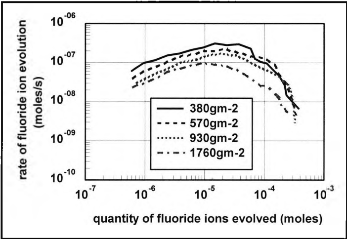
Figure 2.3-16 Rate of fluoride evolution as a function of quantity evolved fluoride ion evolved, UV irradiation of solid-state Irg.261 at various surface density values - effect of photoinitiator surface density
