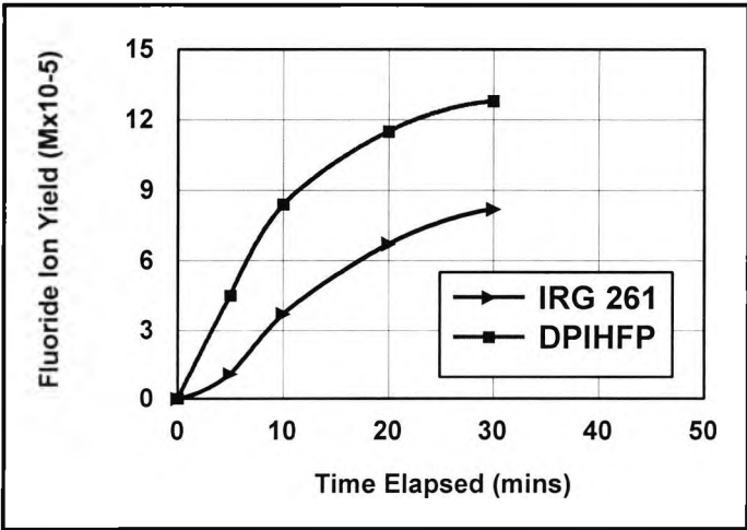
Figure 3.3-12 Fluoride yield from DPIHFP and Irg261 following solid-state photodecomposition
