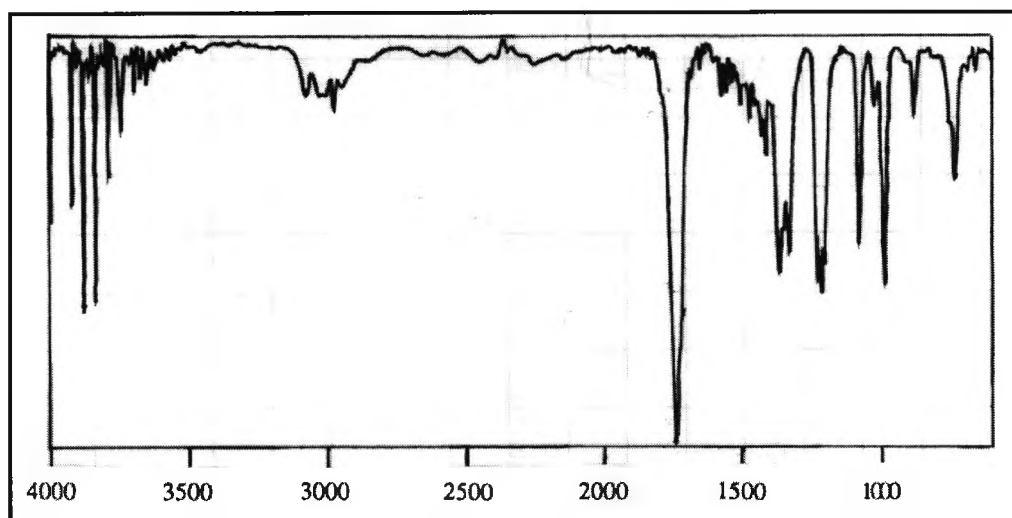
Figure 2.3-2 IR spectrum of gaseous photodecomposition products obtained after UV irradiation of DPIHFP in the solid state
