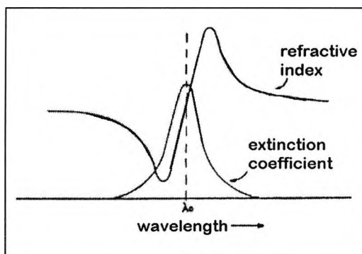
Figure 3.2-8 Influence of IR absorption on the refractive index of an absorbing material
