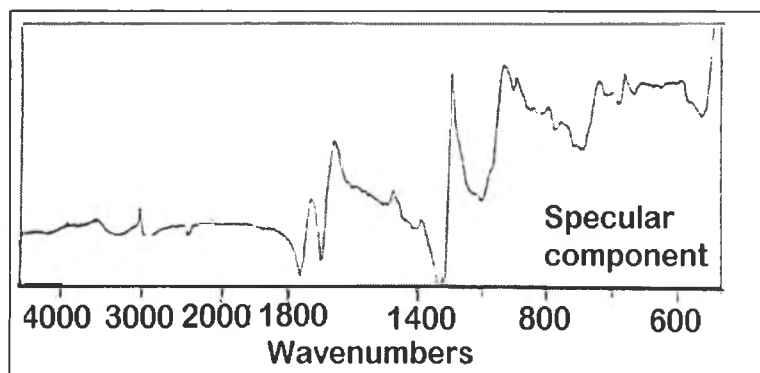
Figure 3.2-9 Specular Reflectance IR spectrum for a cured epoxide formulation at grazing angle (RA component minimal)
