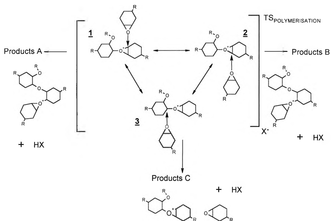
Scheme 1.2-7 Resonance stabilisation of the oxonium ion transition complex
