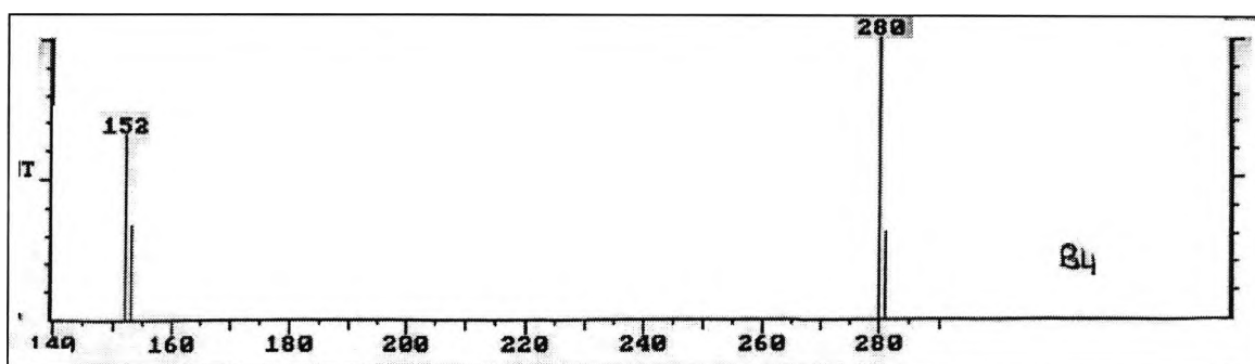
Figure 5.2-5 MS for GC fraction B4 at reference time 391, product obtained from UV irradiation of solid state DPIHFAs
