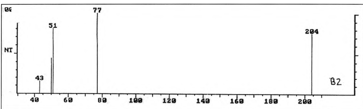
Figure 5.2-3 MS for GC fraction B2 at reference time 135, product obtained from UV irradiation of solid state DPIHFAs
