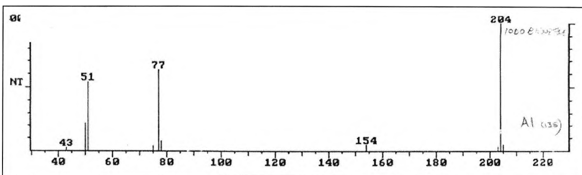
Figure 5.1-2 MS for GC fraction A1 at reference time 135, product obtained from UV irradiation of solid state DPIHFP
