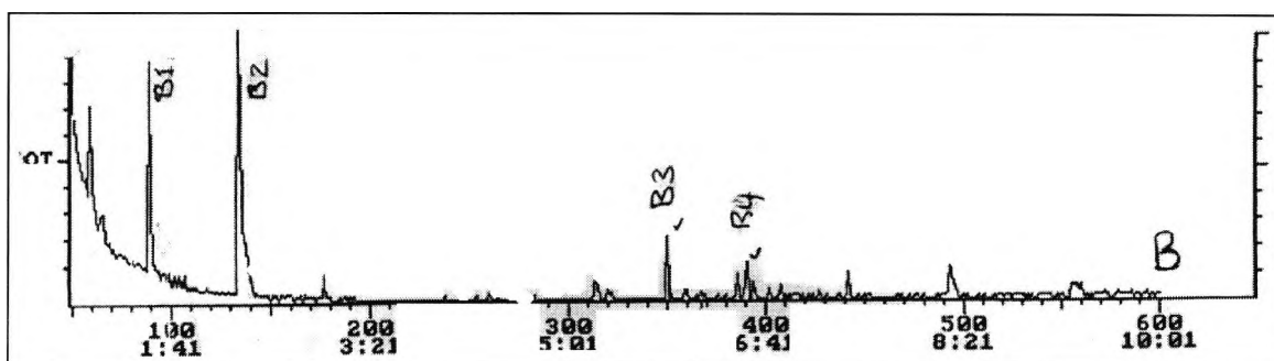
Figure 5.2-1 GC trace for separation of photoproducts obtained after UV irradiation of solid state DPIHFAs, photoproducts dissolved in acetone
