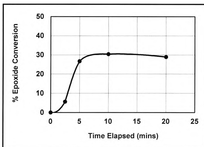
Figure 3.3-8 Remote curing, epoxide conversion showing 'Dark Stage' polymerisation in 2-step process
