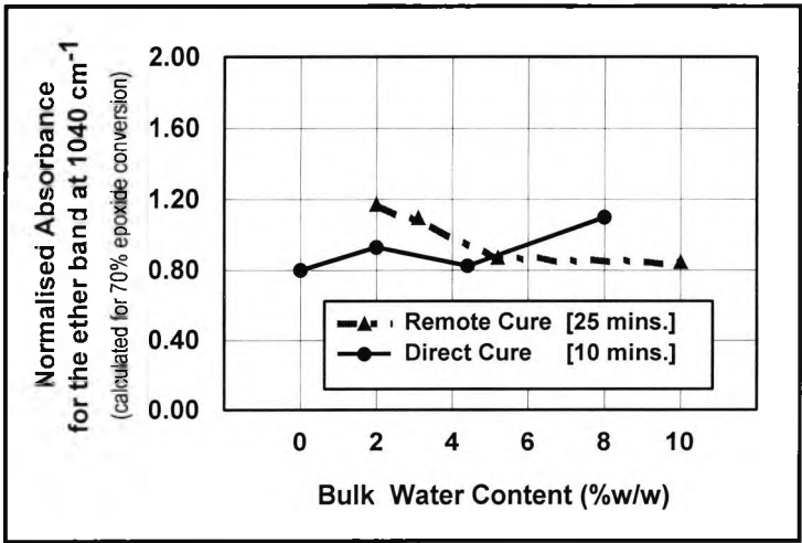
Figure 3.3-25 Normalised IR absorption band for the ether linkage in remote and direct curing in the presence of bulk water
