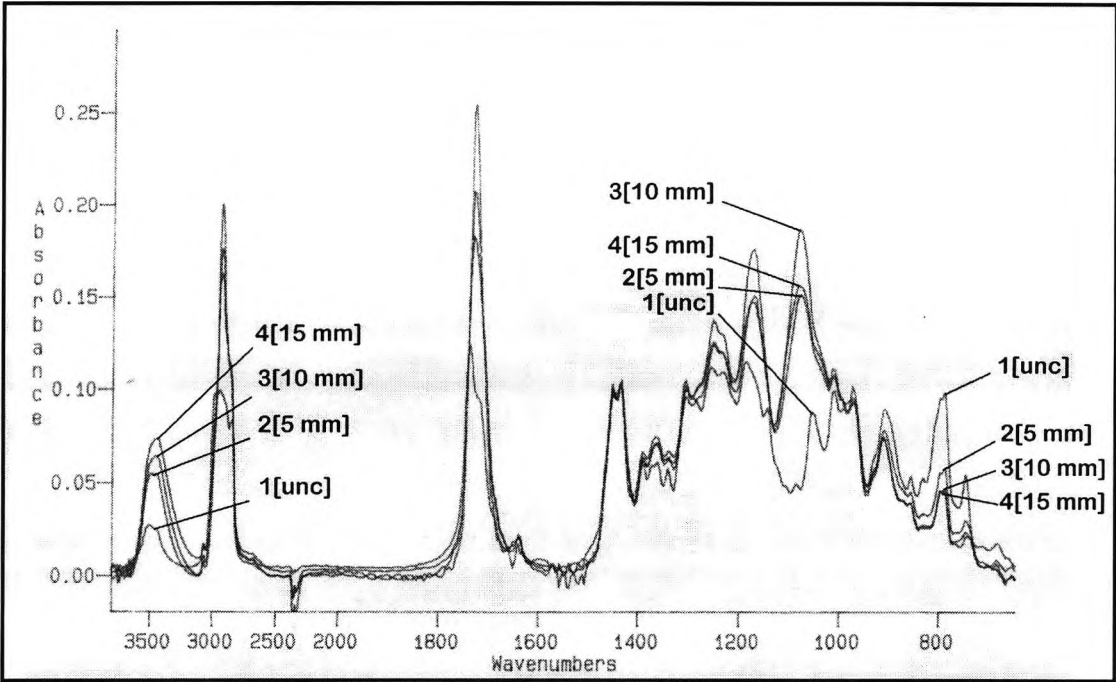
Figure 6.3-1 Remote curing in PTFE apparatus, IR spectra for remote curing of epoxide with variation (5-15mm) of initiator-resin gap width, 0.2g DPIHFP, resin formulation 4
