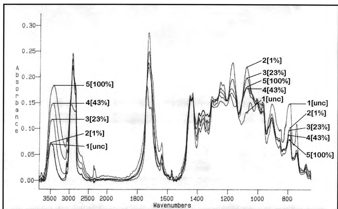
Figure 6.7-1 Remote curing in PTFE apparatus, IR spectra for remote curing of epoxide, 0.1g DPIHFP, resin formulation 4, 1 0 mins. of UV exposure and variation of humidity between 0 and 100%
