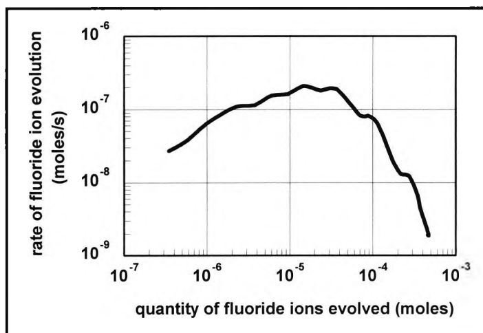
Figure 2.3-7 Rate of fluoride ion evolution as a function of quantity of fluoride ion evolved, UV irradiation of solid-state DPIHFP
