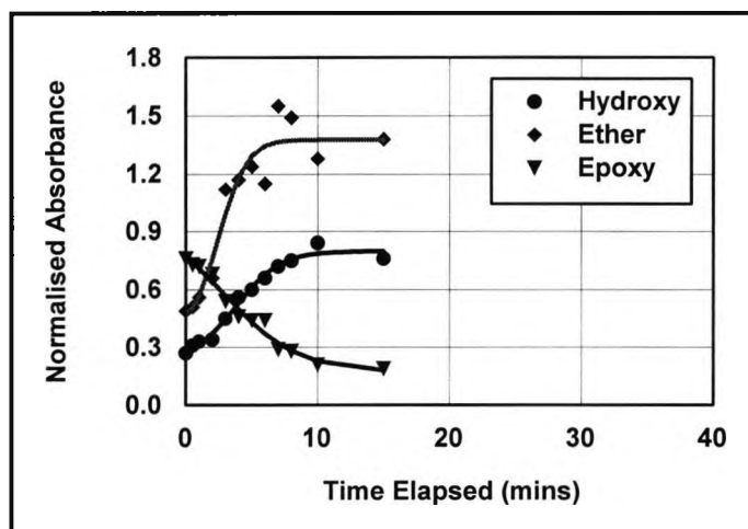
Figure 3.3-3 Direct curing of an epoxide, IR absorbance bands for relevant functional groups for direct epoxide polymerisation
