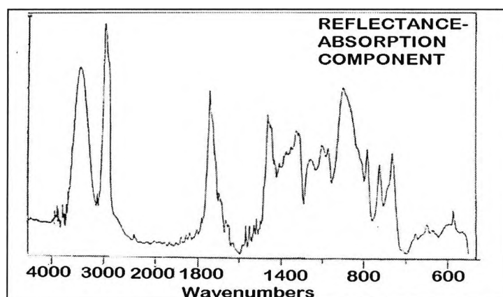
Figure 3.2-6 Reflectance-Absorbance IR spectrum for an uncured epoxide formulation at acute angle of incidence (specular component minimal)
