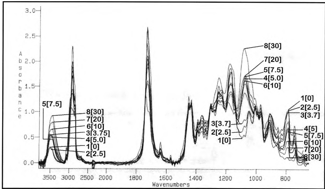
Figure 6.5-1 Remote curing in PTFE apparatus, IR spectra for remote curing of epoxide, 0.2g DPIHFP, resin formulation 4, film thickness = 16 \mu\text{m} +/- 2 \mu\text{m}
