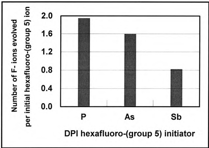
Figure 2.3-10 Relative yield of fluoride ions after UV irradiation of solid-state DPI hexafluoro-(group 5) salts
