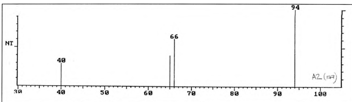
Figure 5.1-3 MS for GC fraction A2 at reference time 177, product obtained from UV irradiation of solid state DPIHFP
