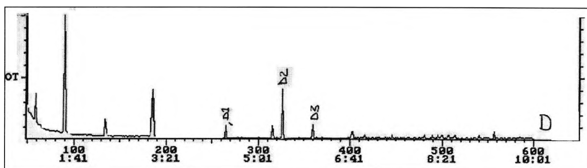
Figure 5.4-1 GC trace for separation of photoproducts obtained after UV irradiation of solid state TPSHFSb, photoproducts dissolved in acetone
