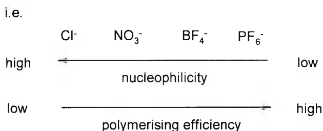
Figure 1.2-2 Relationship between counterion nucleophilicity and polymerising efficiency
