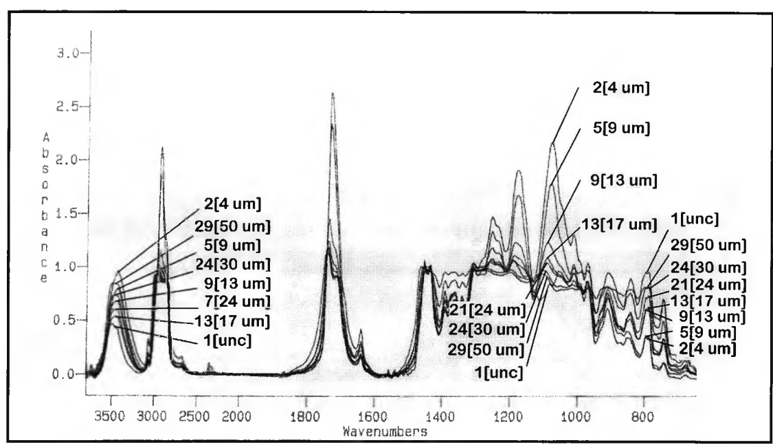
Figure 6.6-1 direct curing, IR spectra for direct curing of epoxide, 2.1% w/w DPIHFP, resin formulation 3, film thickness = 4-50 μm and 1 min. of UV exposure
