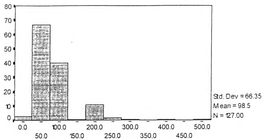
Fig. 4. Frequency distribution of times taken in seconds to answer Question 3.
