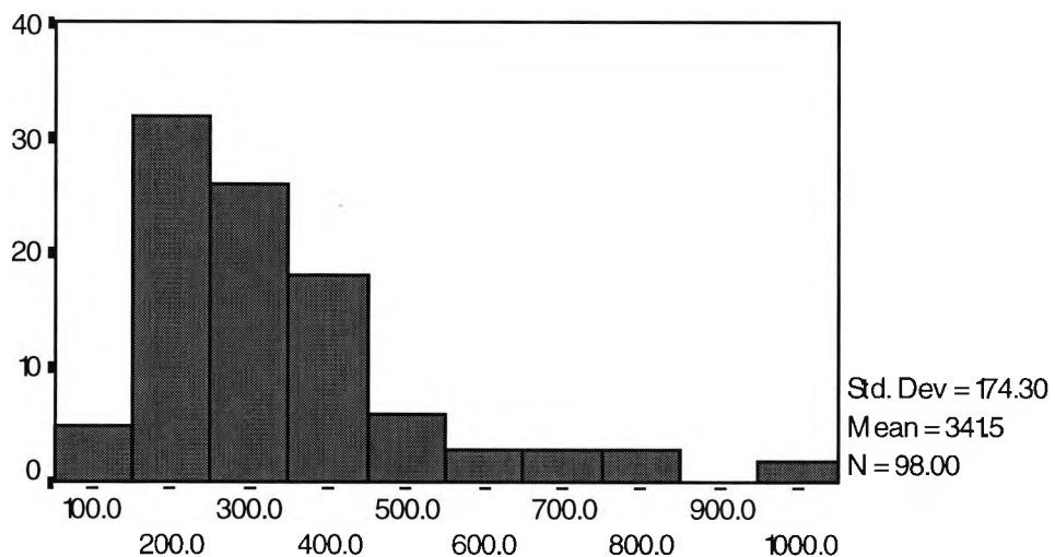
Figure 7.11 Distribution of time taken in seconds to answer all questions
