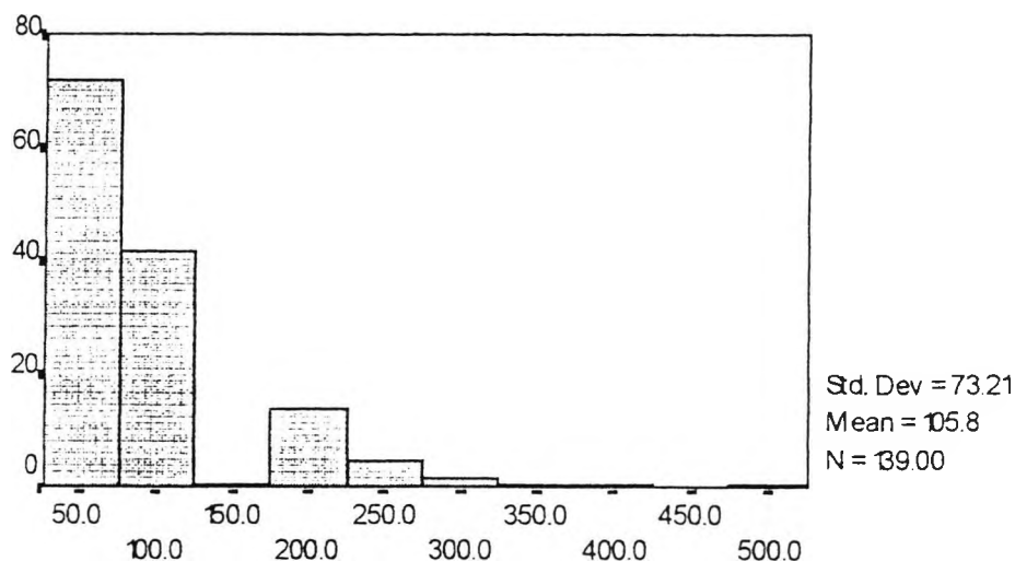
Fig. 3. Frequency distribution of times taken in seconds to answer Question 2.
