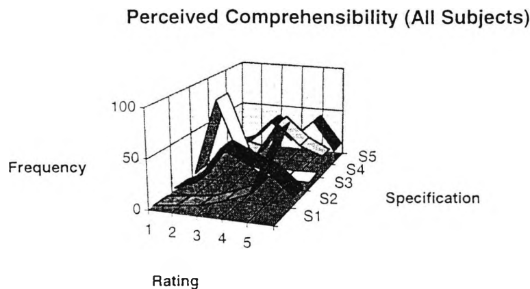
Fig. 7. Frequency plot of perceived comprehensibility, by specification.
