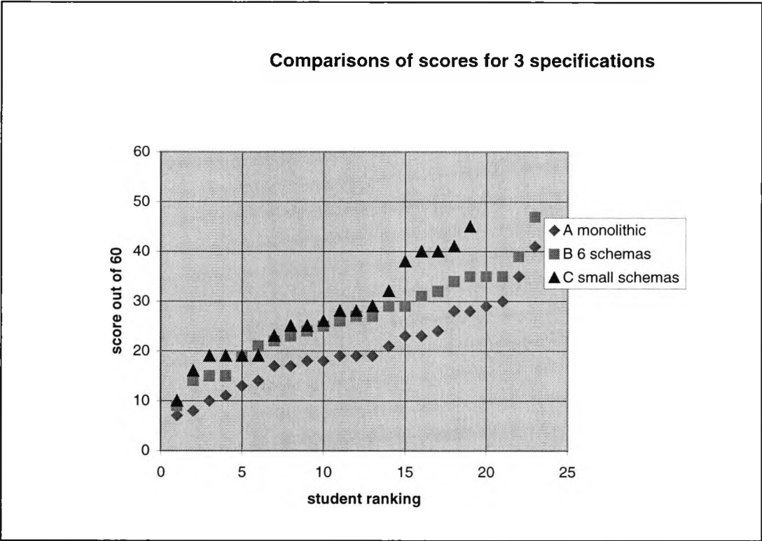
Figure 8.1 Comparison of student scores for each Specification
