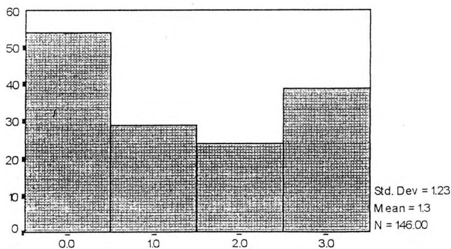
Fig. 6. Frequency diagram of total score.
