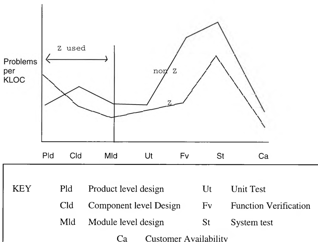
Figure 5.3 Reported comparisons between code resulting from Z and non-Z methods
