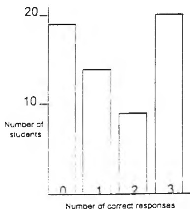
Fig. 2. A chart showing scores obtained.
