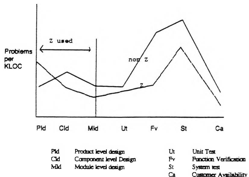
Figure 1. Comparison between Z use and non-Z use.
