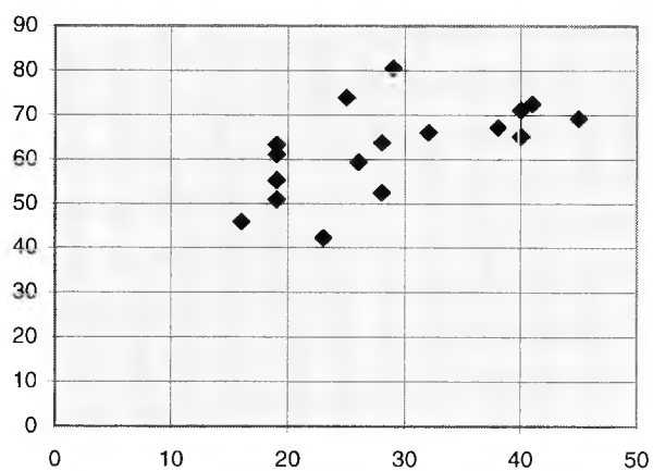
Figure 8.3 Scatter diagram for Specification B
