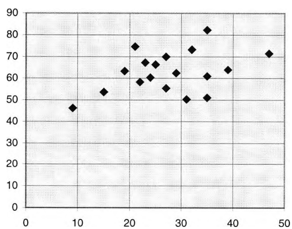
Figure 8.4 Scatter diagram for Specification C
