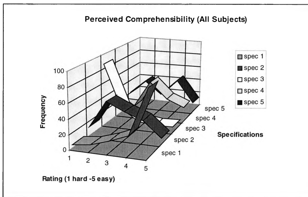
Figure 7.13 Frequency plot of perceived comprehensibility, by specification
