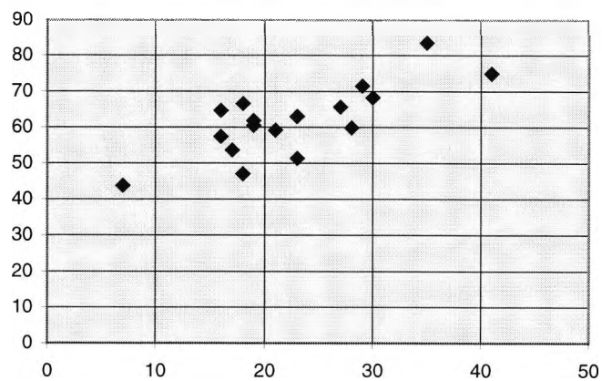
Figure 8.2 Scatter diagram for Specification A
