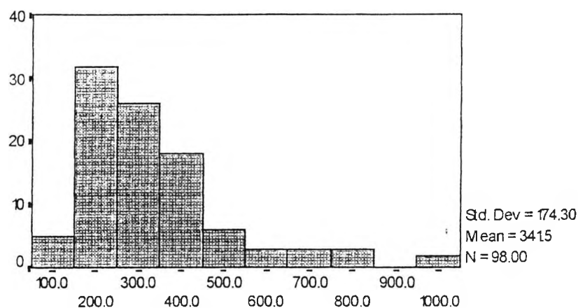
Fig. 5. Frequency distribution of time taken in seconds to answer all questions.
