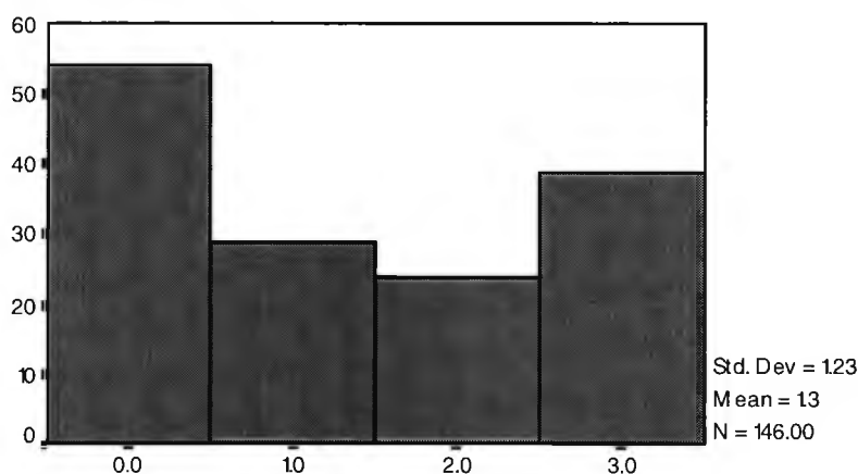
Figure 7.12. Frequency diagram of total score
