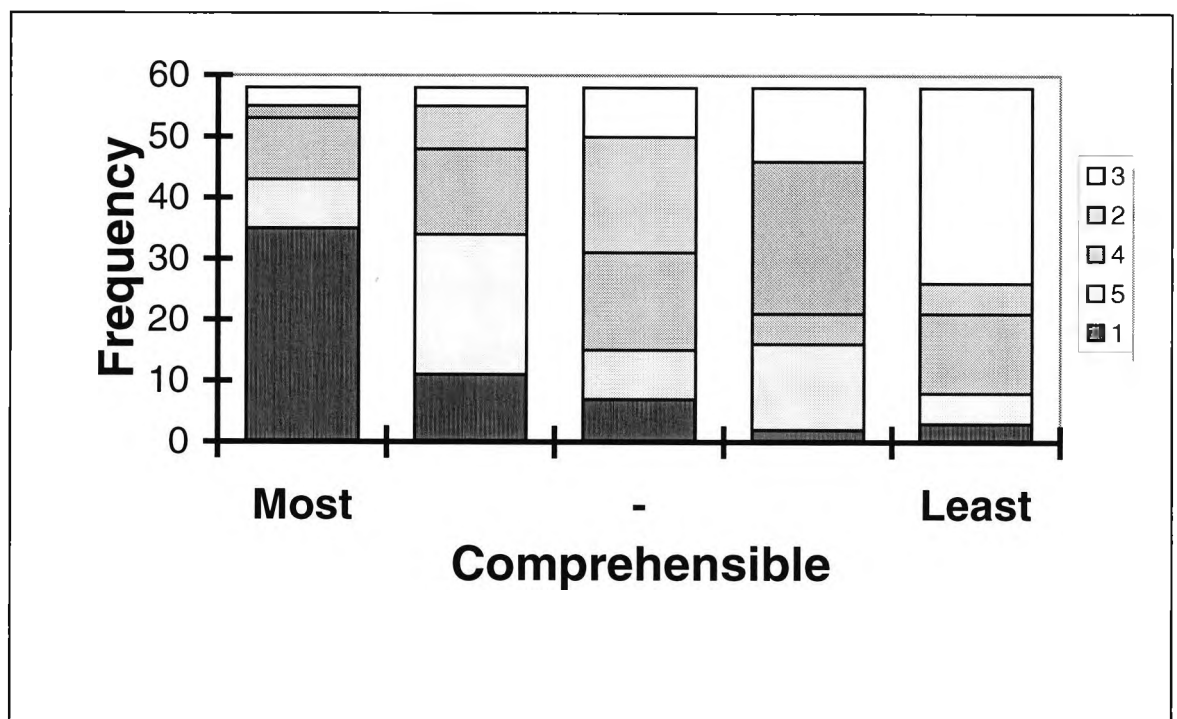
Figure 7.7 The distribution of the rankings over the five specifications
