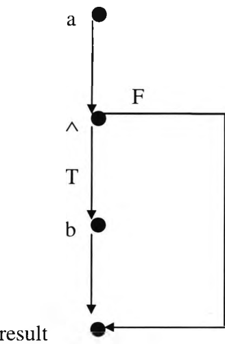
Figure 3.5 Graphical representation of a \wedge b
