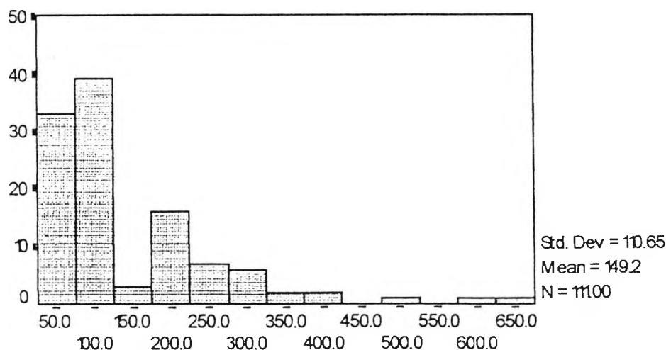
Fig. 2. Frequency distribution of times taken in seconds to answer Question 1.
