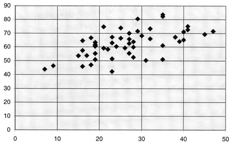
Figure 8.5 All Specifications scores against previous marks
