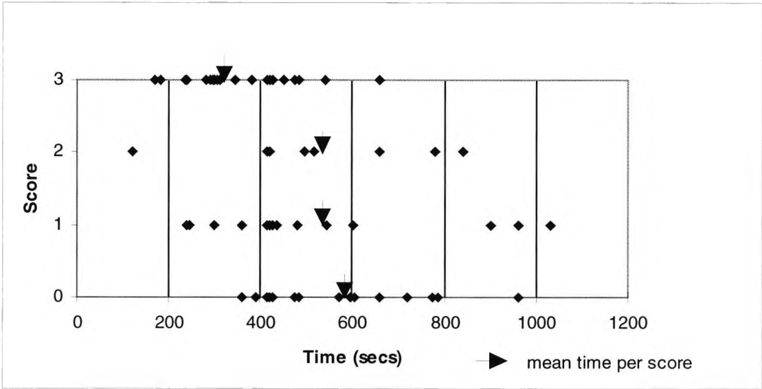
Figure 7.6 The distribution of the scores and times together
