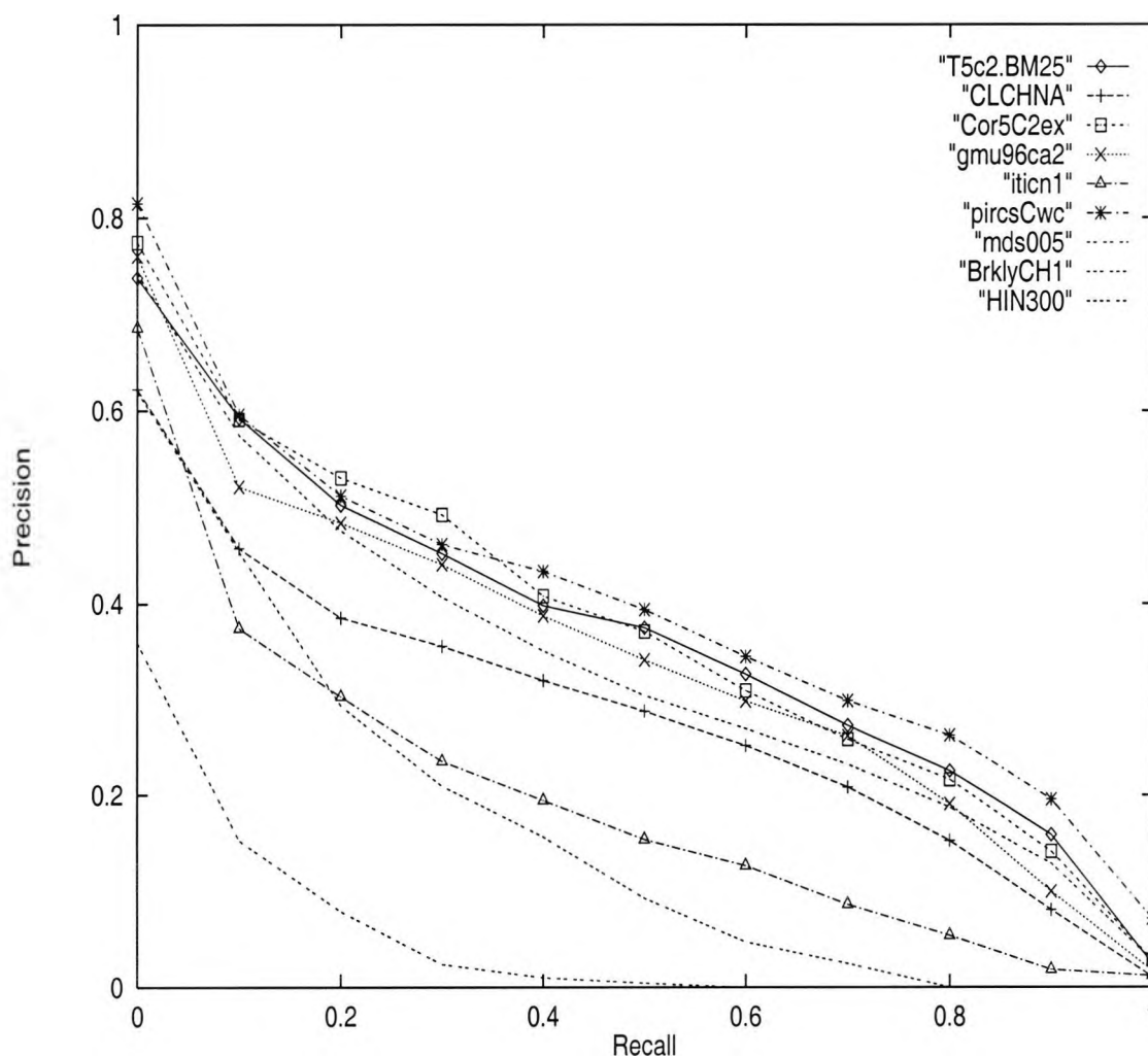
Figure 7.7: Precision-Recall Curves for Some Automatic Runs at TREC-5
