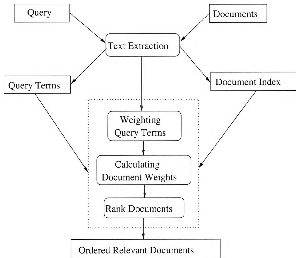
Figure 6.3: A Typical Information Retrieval Process
