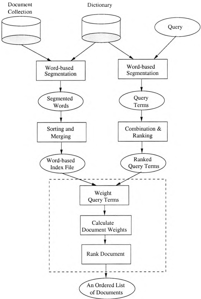
Figure 5.3: System Architecture for Word-based Chinese Retrieval System
