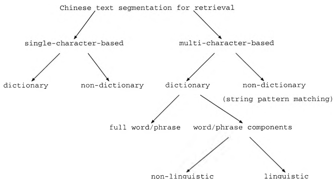
Figure 2.4: Classification of Chinese Text Segmentation
