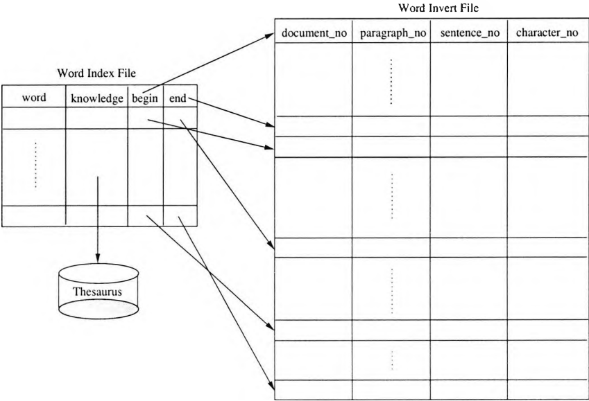
Figure 5.10: Data Structure for Word-based System’s Index File
