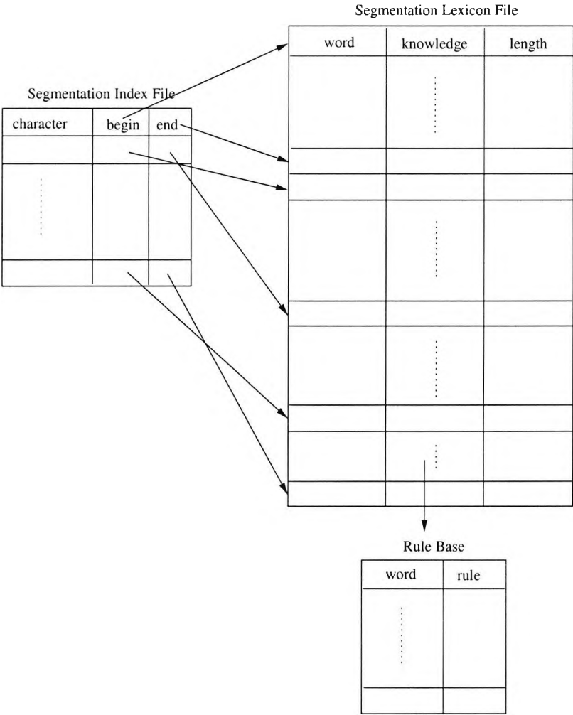
Figure 5.9: Data Structure for Segmentation Dictionary’s Index File
