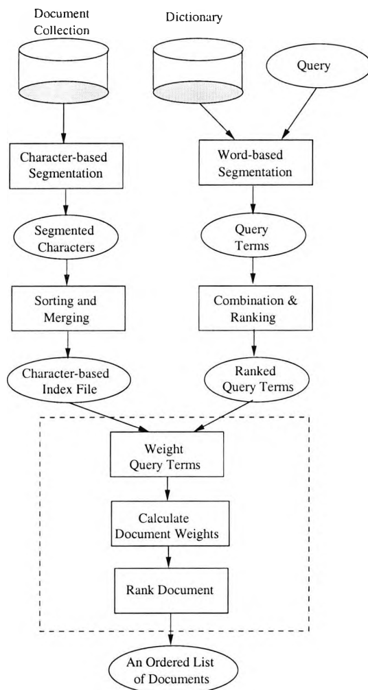
Figure 5.4: System Architecture for Character-based Chinese Retrieval System
