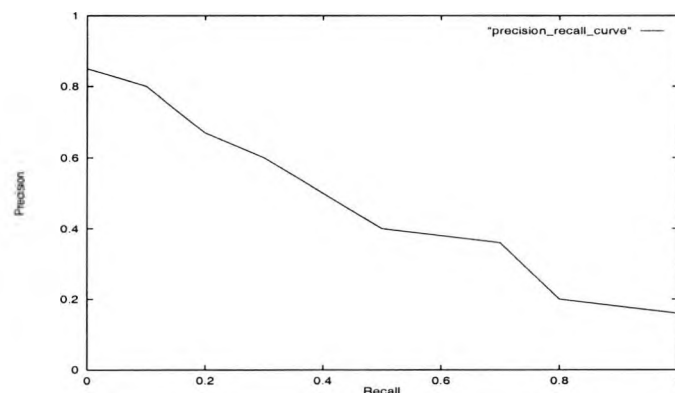
Figure 2.2: Precision versus Recall
