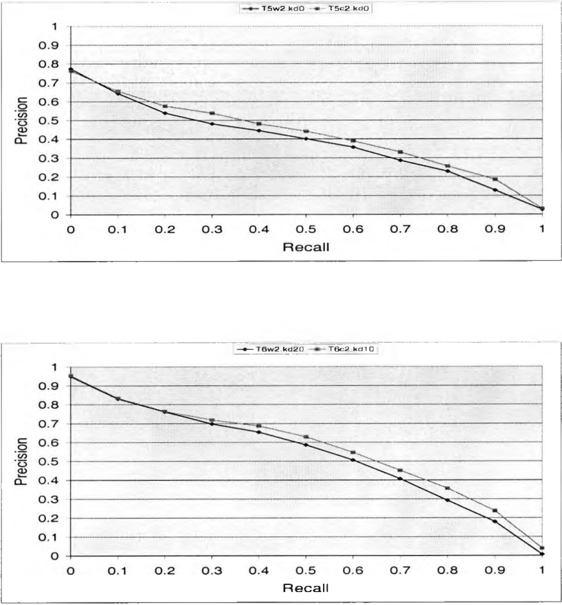
Figure 8.3: Precision-recall curves for the two best runs from word and character approaches at TREC-5 and TREC-6
