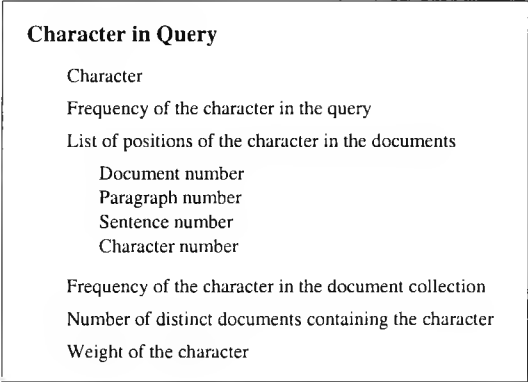
Figure 5.12: Data Structure for Retrieved Character
