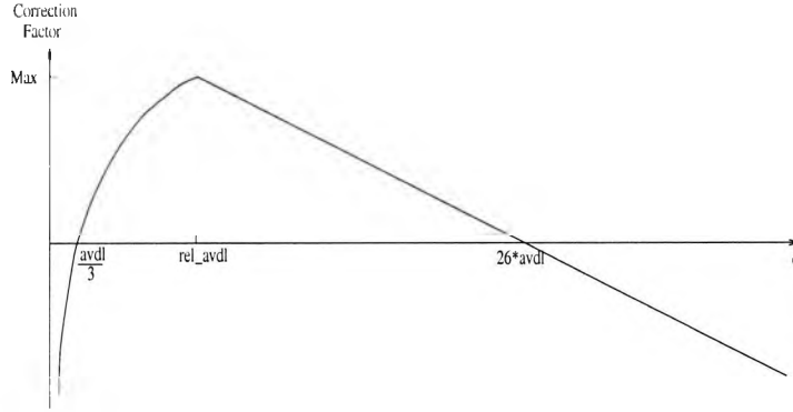
Figure 4.4: Curve for the New Correction Factor with respect to Document Length
