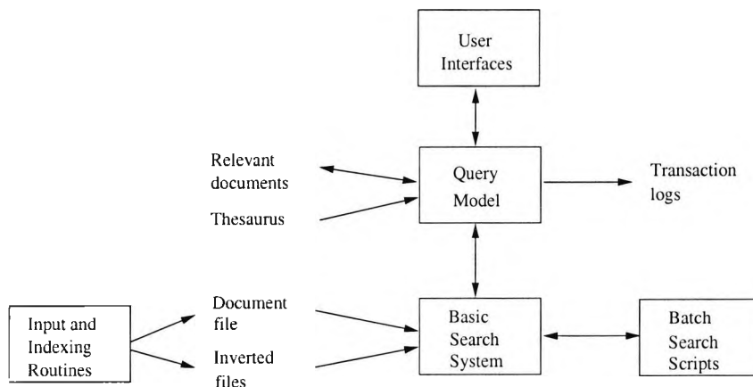
Figure 5.1: Overview of the Structure at Okapi
