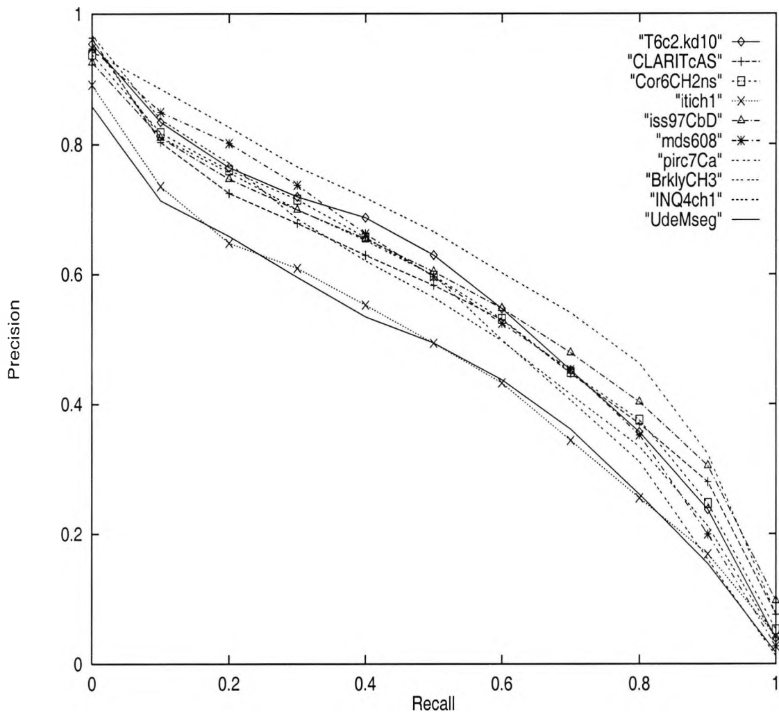
Figure 7.8: Precision-Recall Curves for Some Automatic Runs at TREC-6
