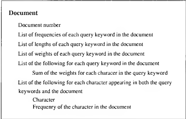
Figure 5.13: Data Structure for Retrieved Document
