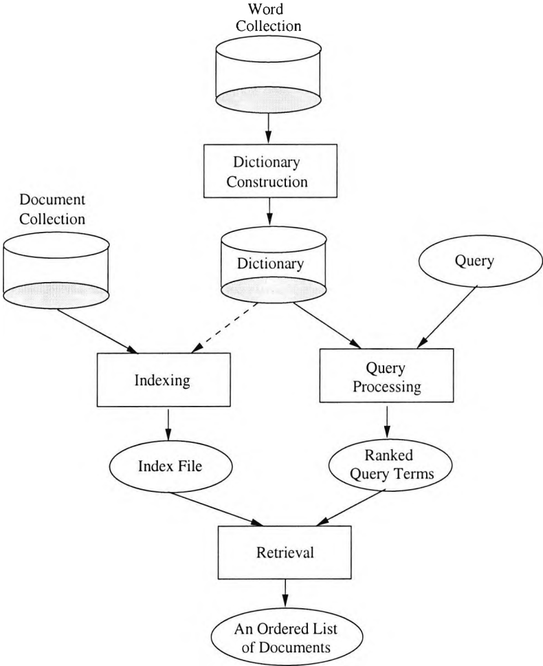
Figure 5.2: System Architecture for Chinese Retrieval System
