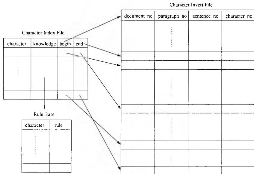
Figure 5.11: Data Structure for Character-based System's Index File
