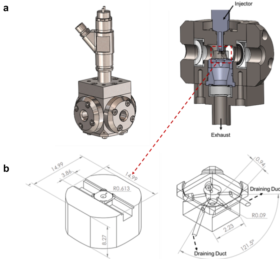
Fig. 1. (a) Overall and section views of the spray chamber employed in the experiments. (b) CAD assembly of the Spray-M test piece with the dedicated acrylic pedestal. All dimensions are in mm.
