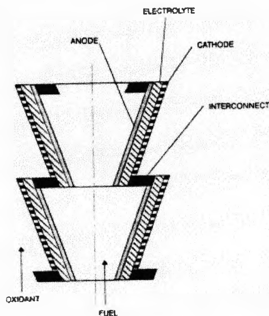
FIG. 2-5. Segmented-cell-in-series design configuration
