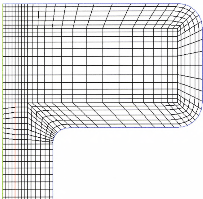
Fig.5-5 Grid used in the half section of the compact manifold design.
