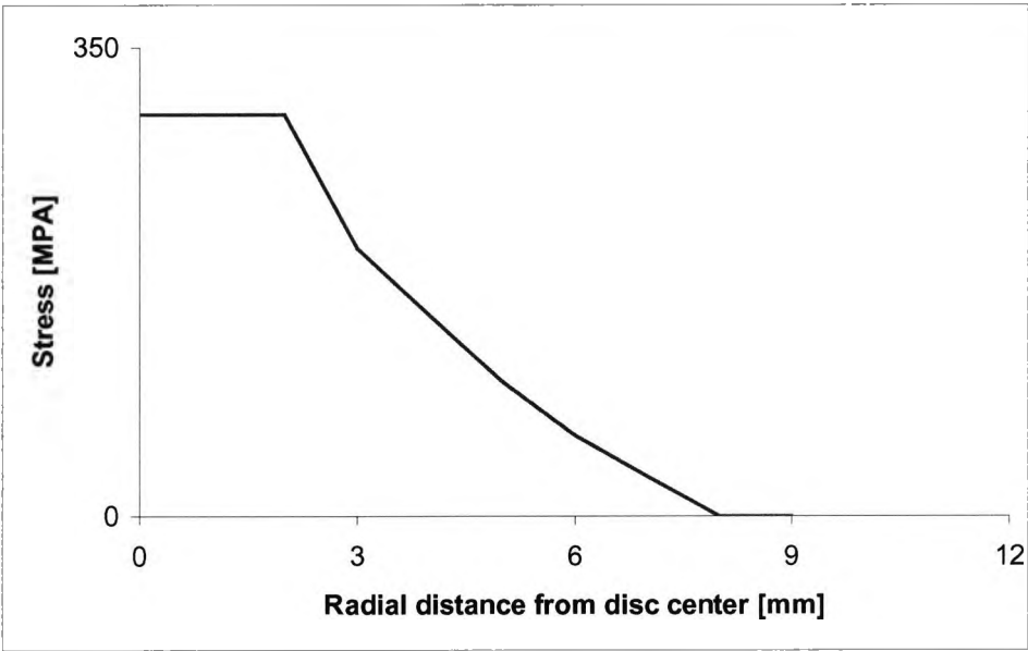
Fig.7-1 Stress distribution in a ring-on-ring test
