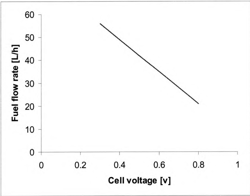
Fig. 6-7 Fuel flow rate as a function of cell voltage
