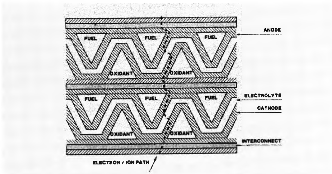
FIG. 2-3. Monolithic cell design configuration
