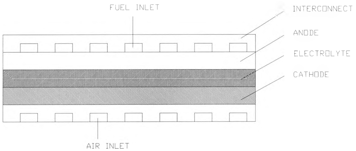
Fig. 4-14 Planar conceptual design
