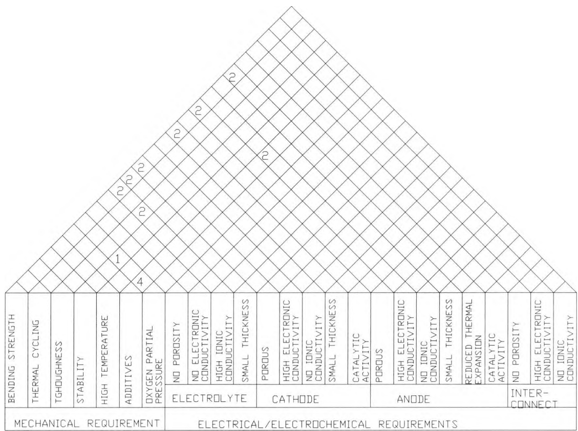
Fig. 4-11 Mechanical – Electrical interactions (Solution oriented)
