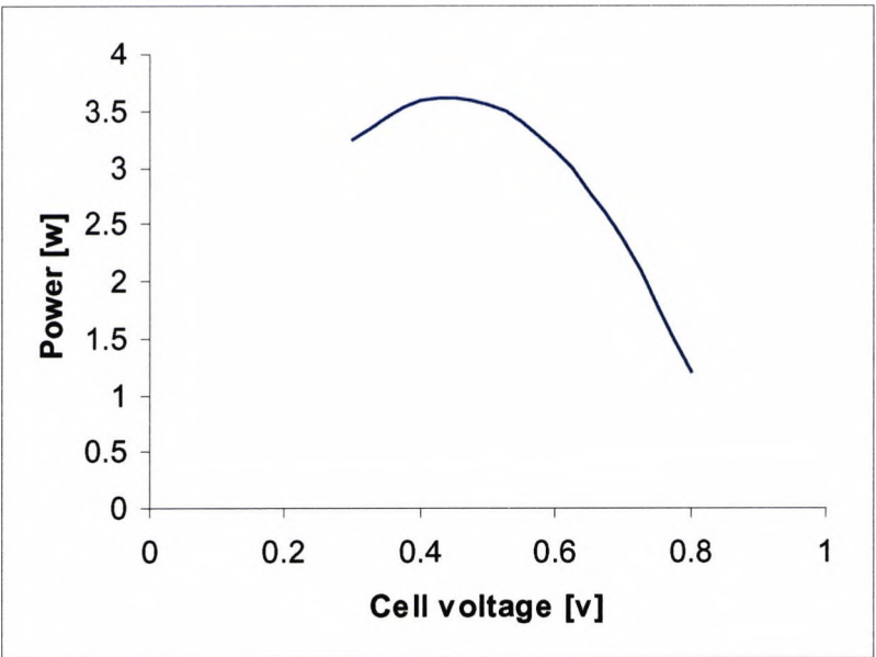
Fig. 6-5 Gross power generation as function of cell voltage
