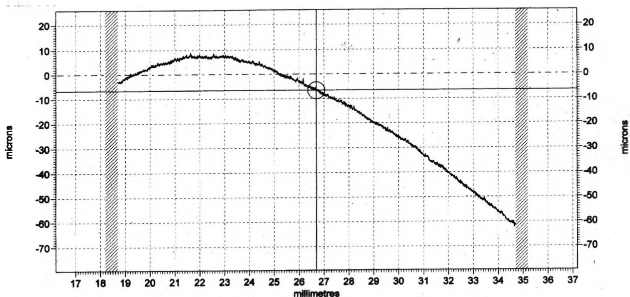
Fig.7-5 A raw surface profile of anode + electrolyte bi-layer
