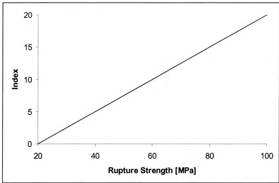
FIG. 8-7 Rupture strength Vs Index
