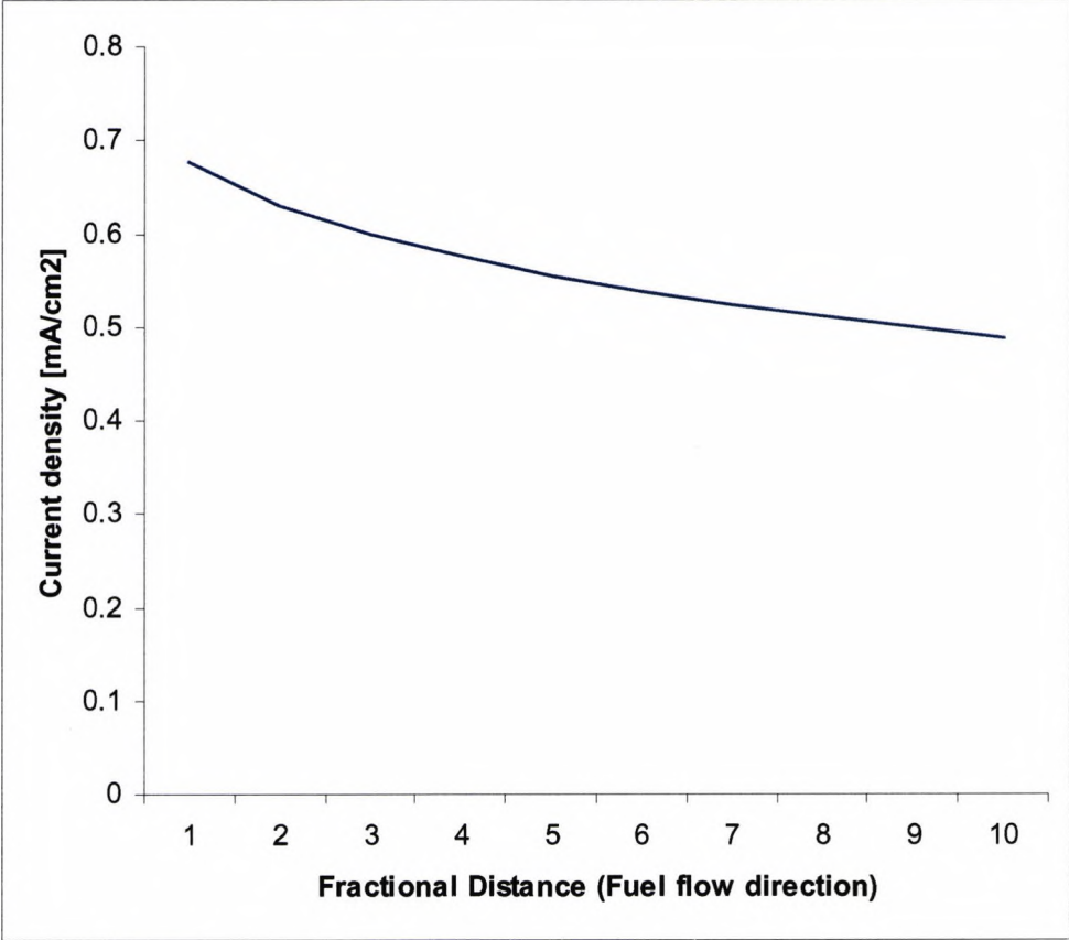
FIG.6-3 Current density distribution across the cell
