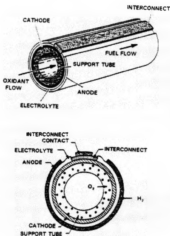
FIG. 2-2. Tubular design configuration
