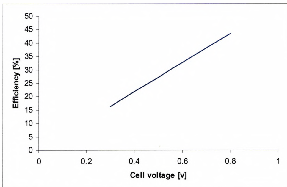
Fig.6-8 Efficiency as a function of cell voltage
