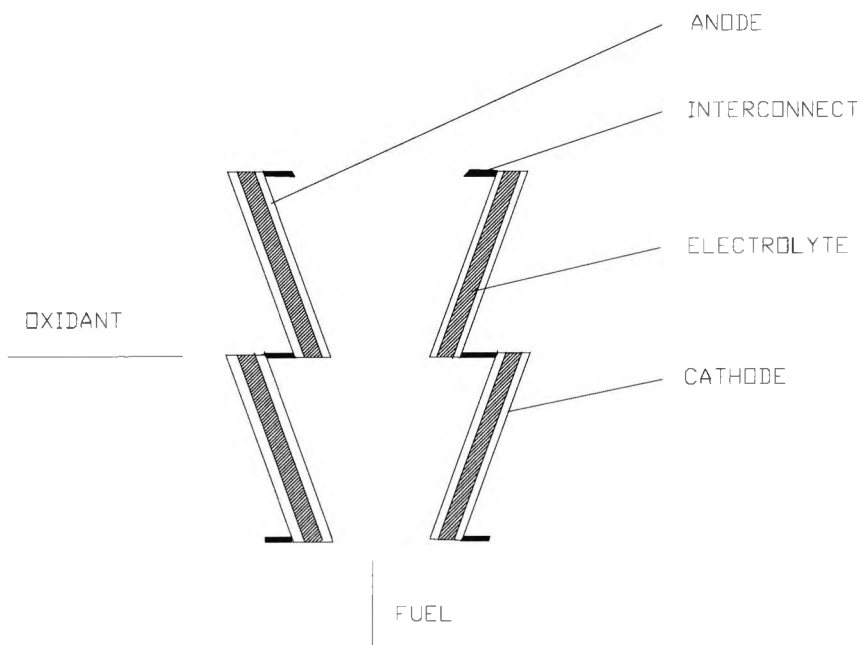
Fig.4-15 Conical conceptual design
