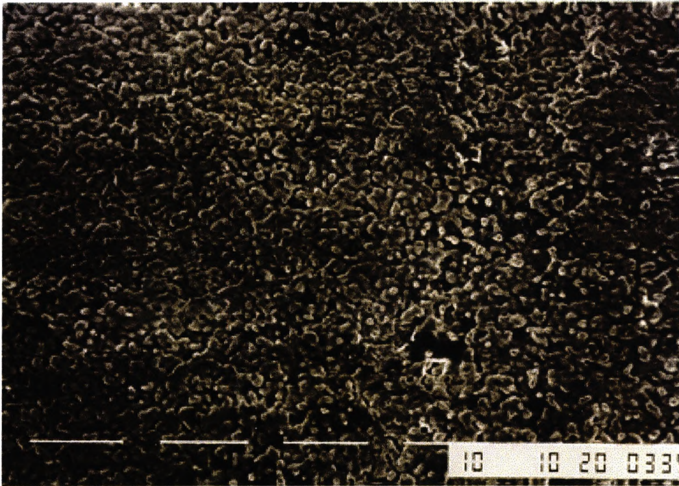
FIG.8-15 Microstructure of fine powder YSZ sintered at 1500°C
