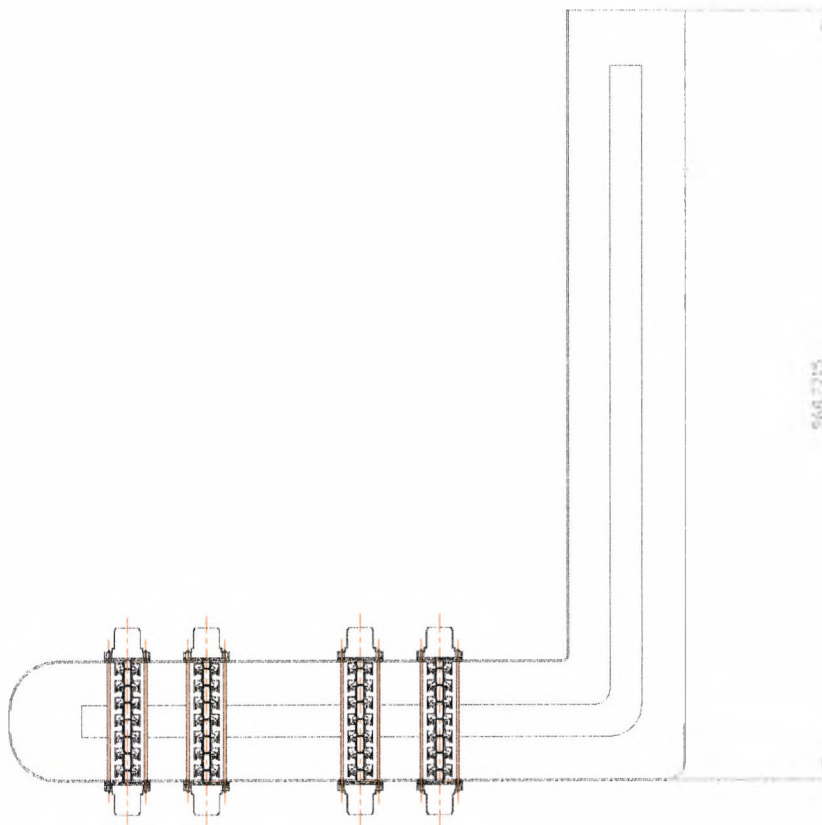
Fig.A-5 Alternative manifold design.
