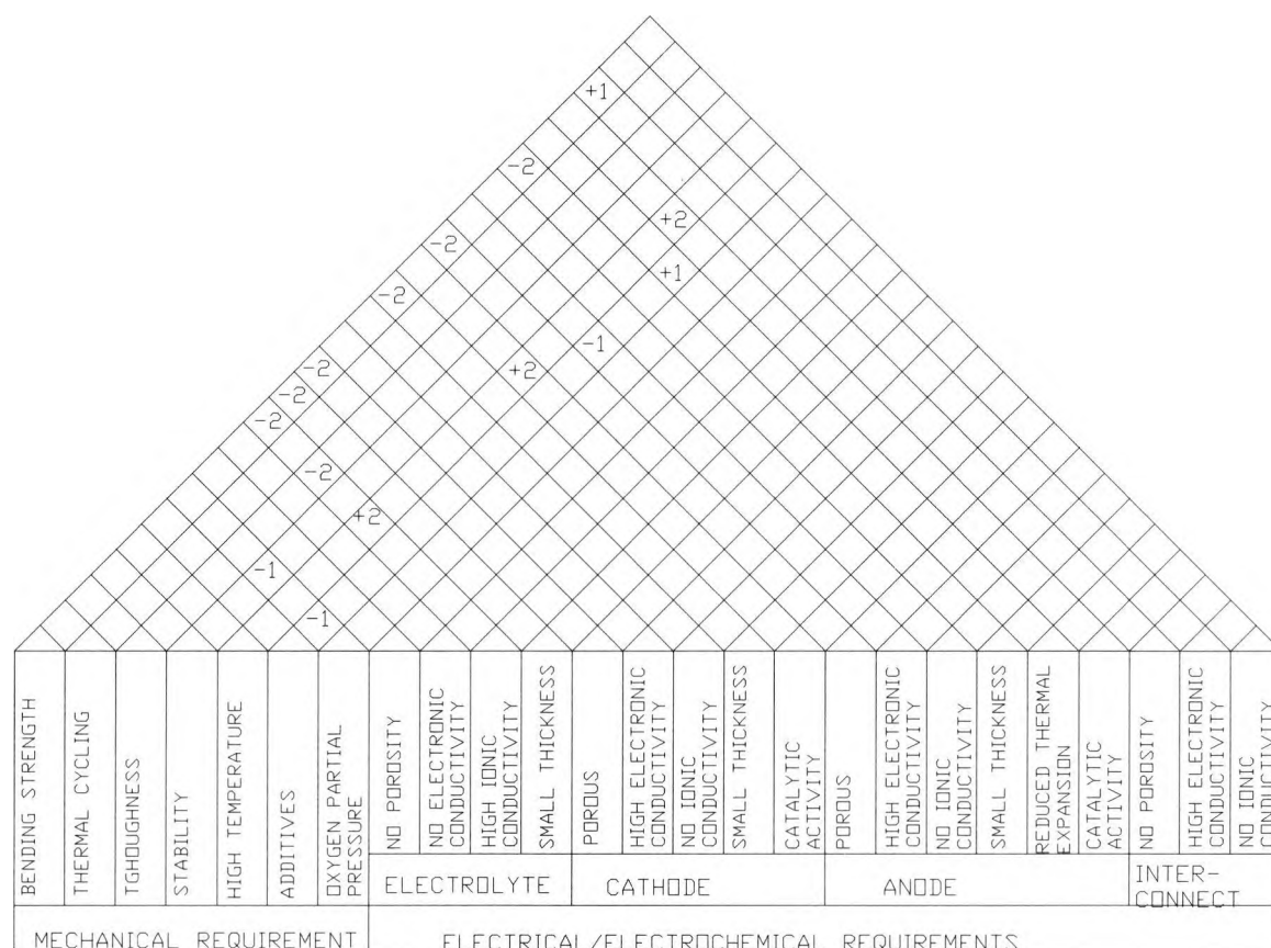
Fig.4-10 Mechanical – Electrical interactions (problem oriented)
