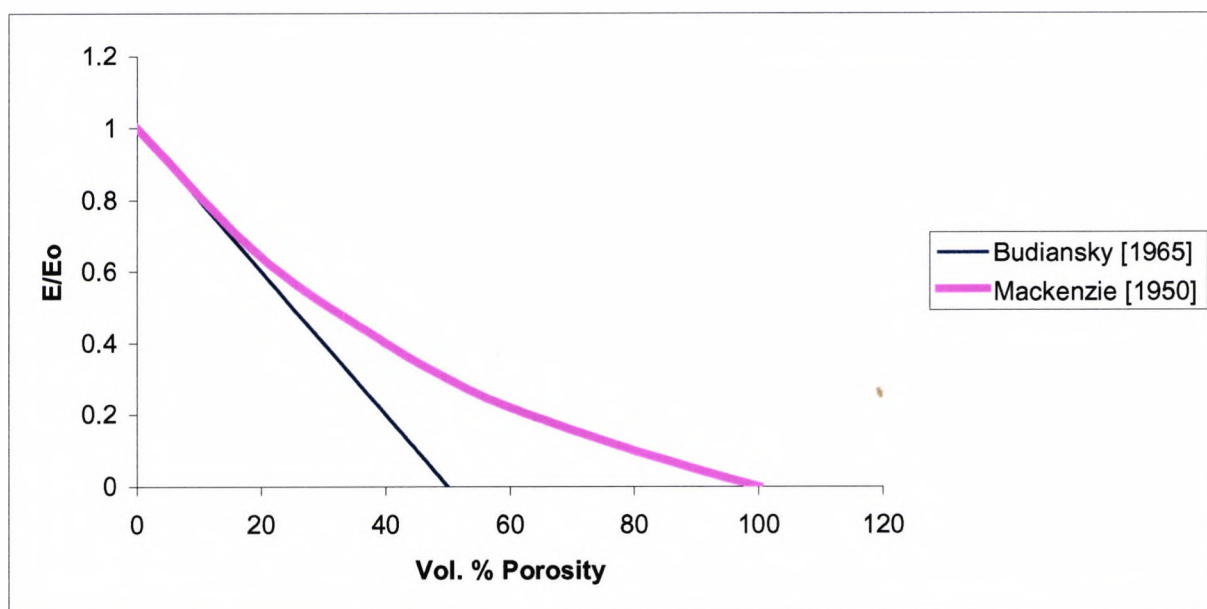
Fig.7-4 Predicted Young's modulus as a function of porosity
