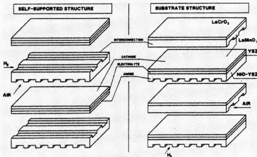
FIG. 2-4. Planar cell design configuration
