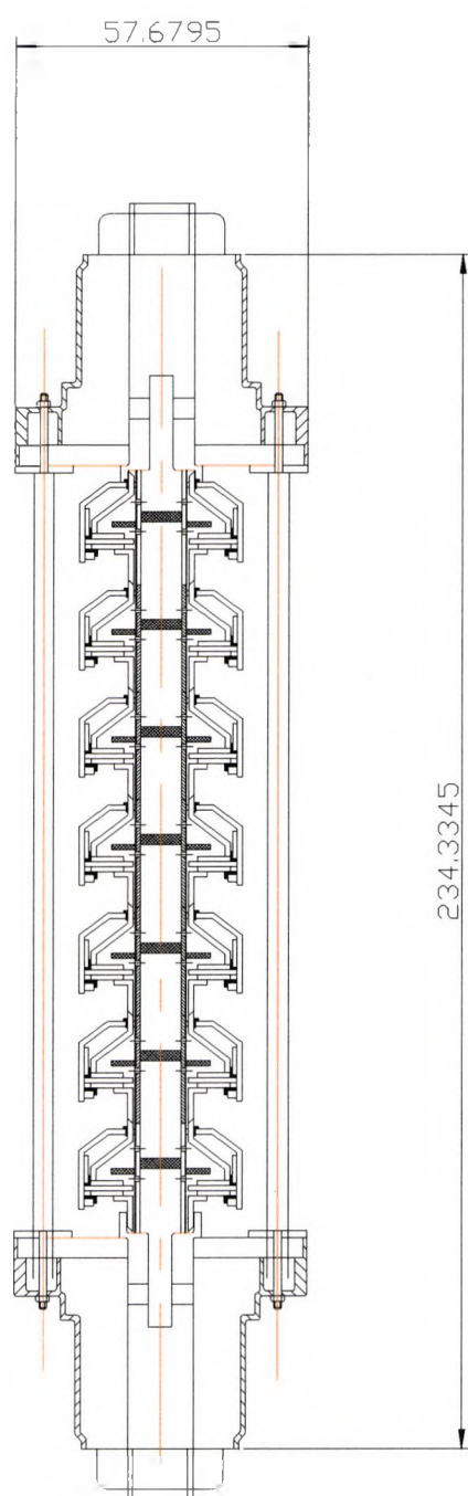
Fig.A-3 A combined SOFC stack
