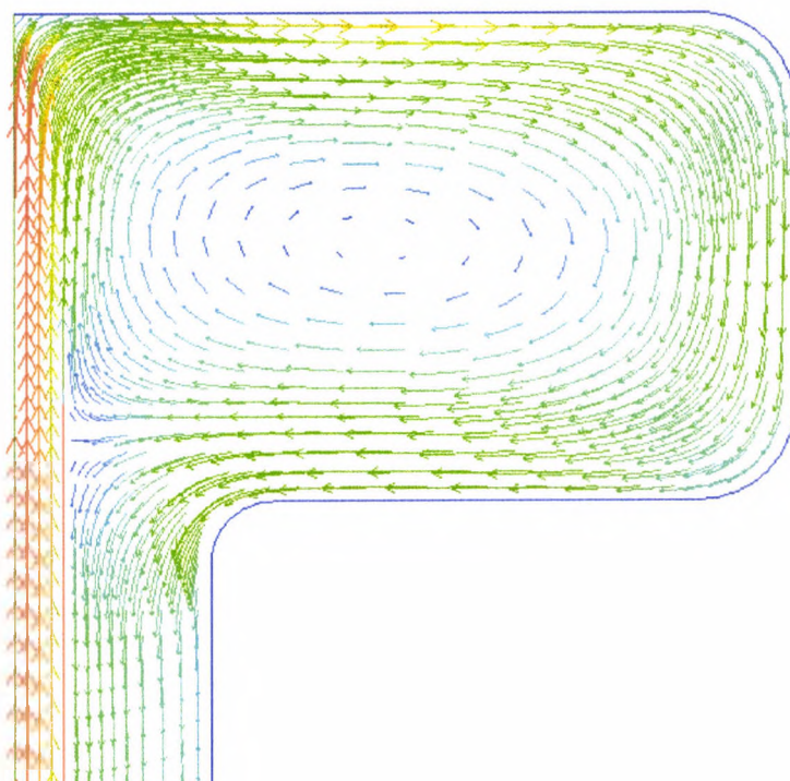
Fig.5-6 Flow pattern in the compact manifold at an inlet velocity of 10m/s.
