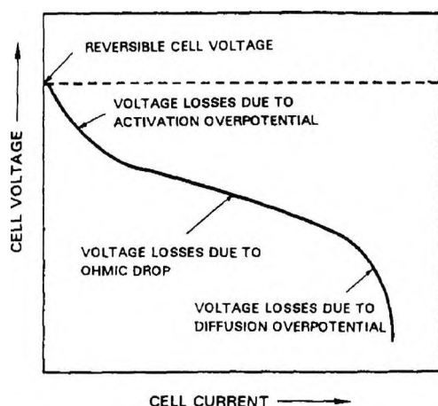
Fig. 2-6 Typical voltage current relation for an operating cell
