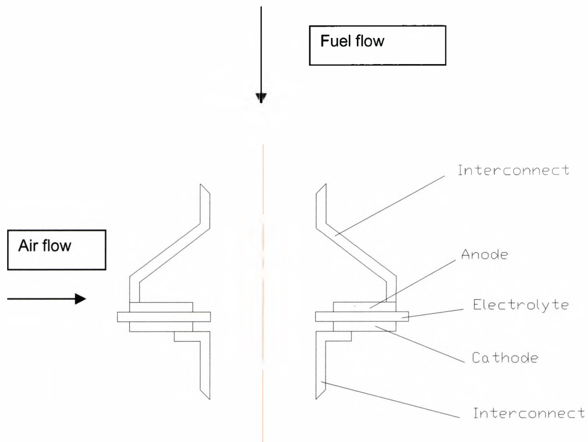
Fig.4-16 Proposed cell configuration
