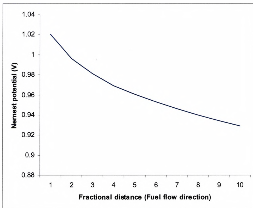
FIG.6-4 Nernst potential distribution across the cell
