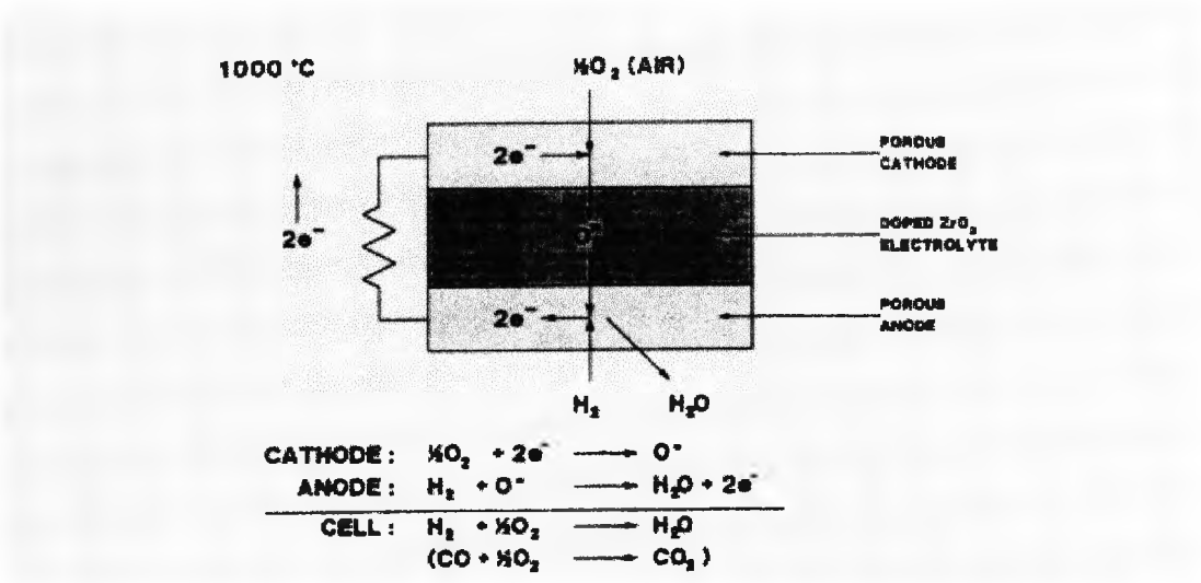
FIG. 2-1 Principle of cell operation
