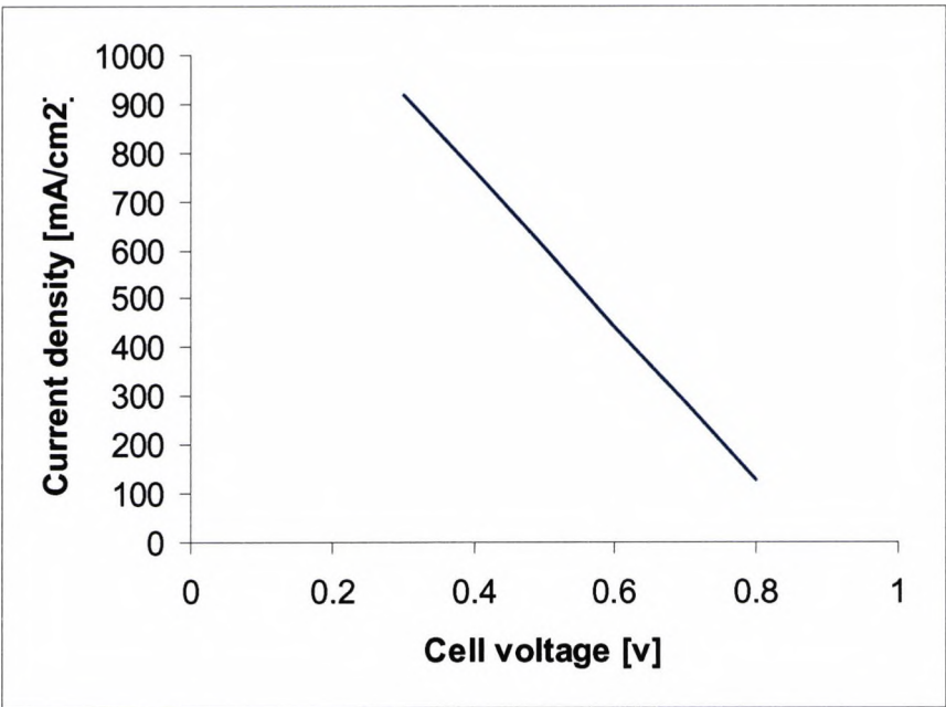
Fig. 6-6 Average current density as a function of cell voltage
