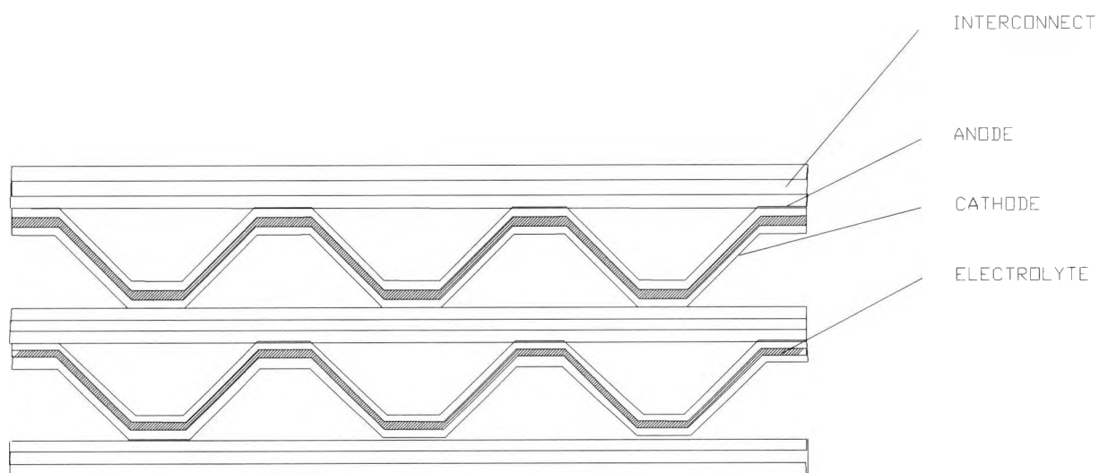
Fig. 4-13 Monolithic conceptual design
