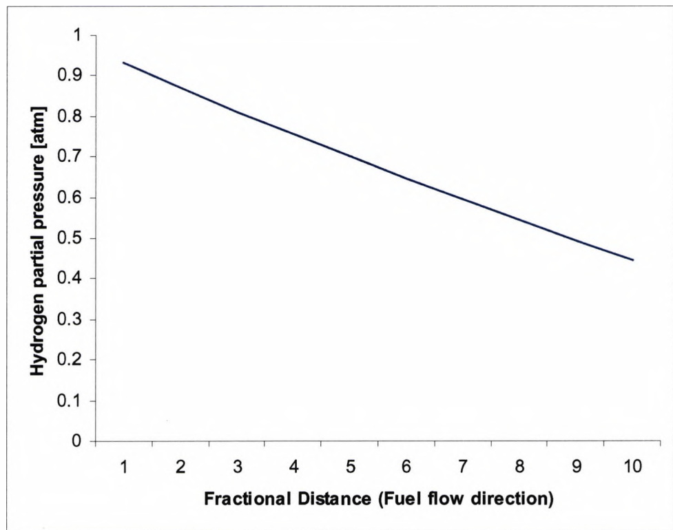
FIG.6-2 Hydrogen partial pressure distribution across the cell
