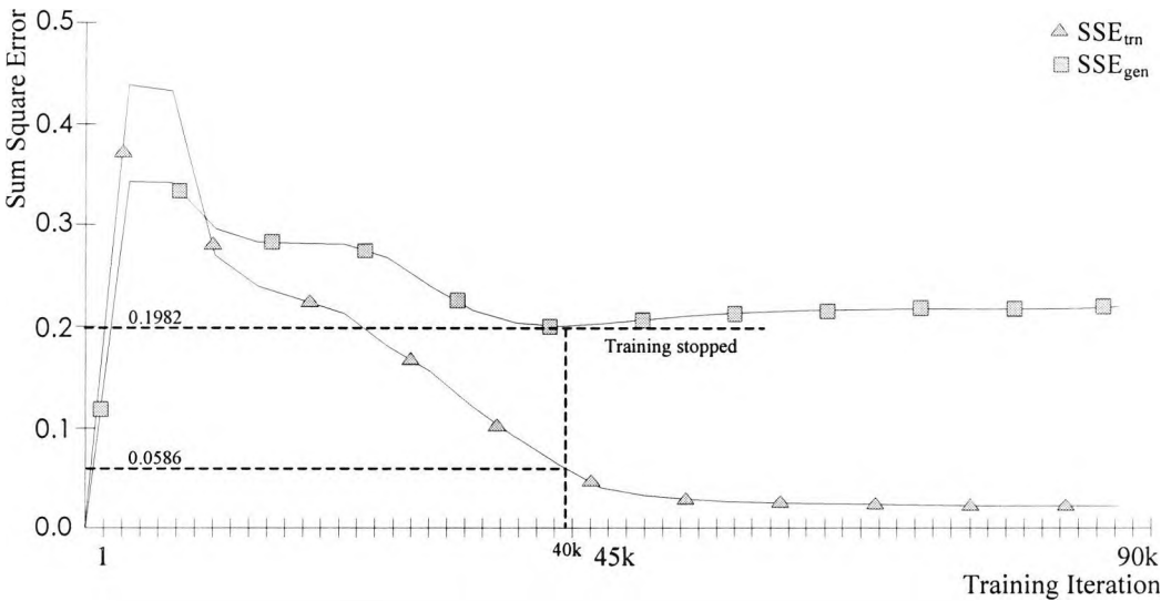
Figure 6.16 Recall and generalisation error of network trained with Co-operative data.
