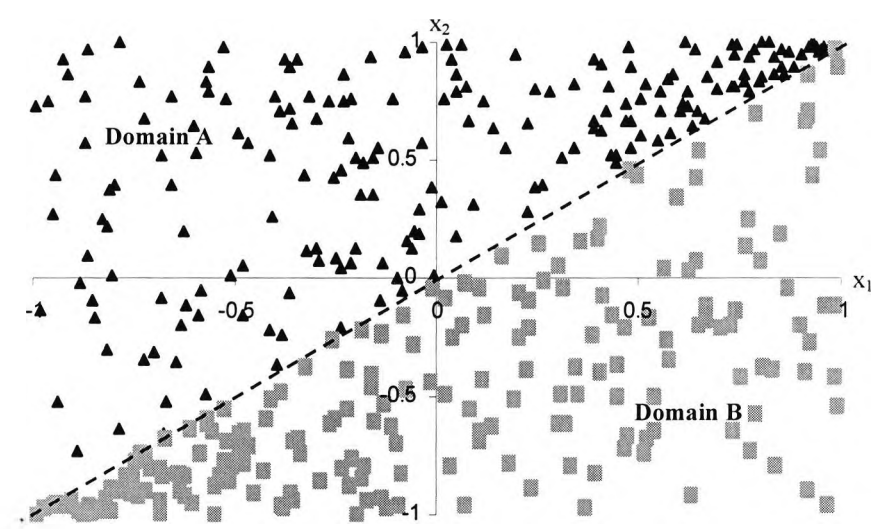
Figure 4.12 Training data for domain A (▲) and B (■).
