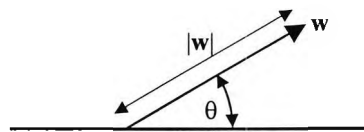
Figure 2.1 Vectors are defined by direction and magnitude.
