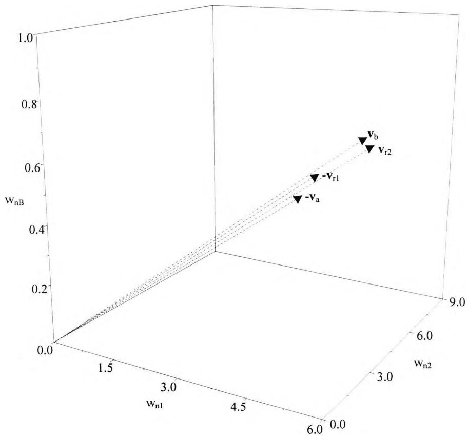
Figure 3.4 Linking of vectors \mathbf{v}_a and \mathbf{v}_b into one vector \mathbf{v}_{r1} and a length adjustment factor F .
