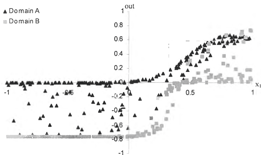
Figure 4.21 Network output for domain A ( \blacktriangle ) and B ( \blacksquare ).
