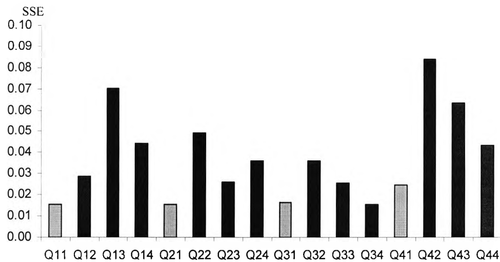
Figure 5.27 Error distribution for each cluster after training of clusters from figure 5.25.
