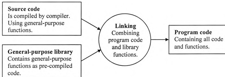
Figure 1.1 Linking source code and functions from a general-purpose library.
