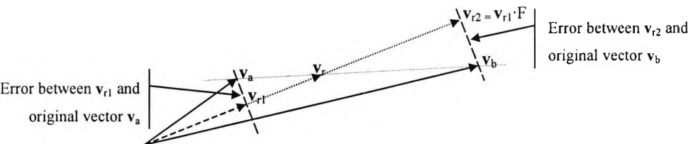
Figure 2.8 Reducing the errors between vectors by vector length multiplication.
