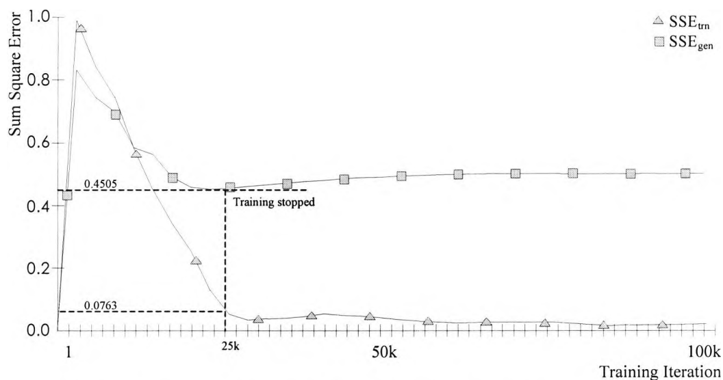
Figure 6.17 Recall and generalisation error of network trained with Legal&General data.
