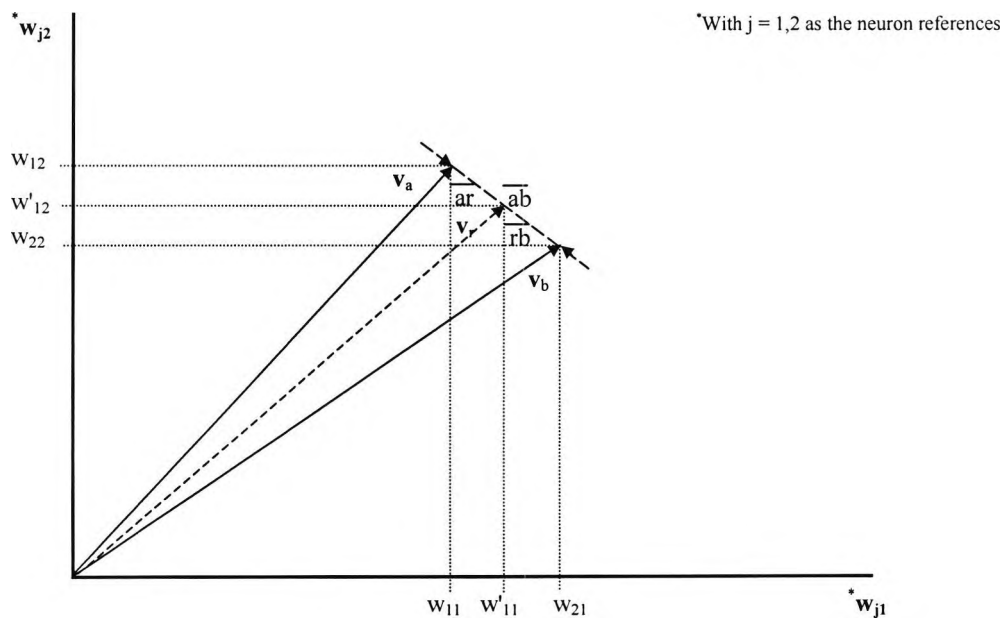
Figure 2.5 Creation of the resulting vector v_r via simple component averaging.
