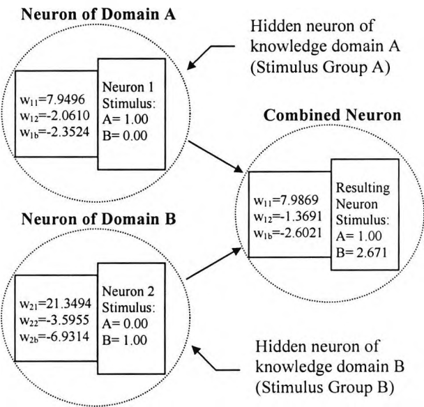
Figure 4.2 Hidden neurons before and after linking.
