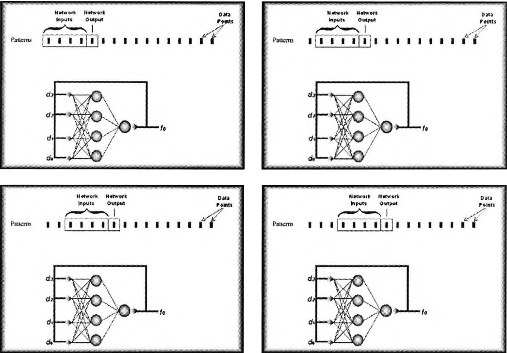
Figure 6.3 Training pattern generation for time series forecasting.
