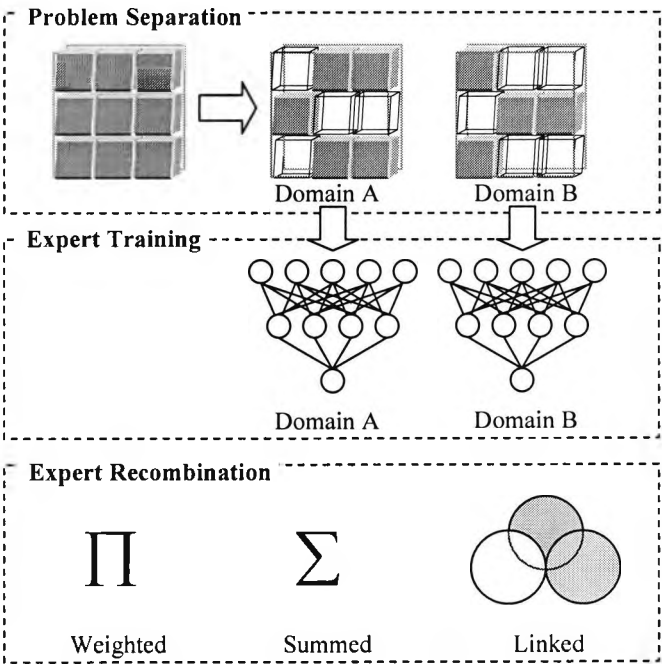
Figure 1.2 Linking can be categorised as an expert recombination method.
