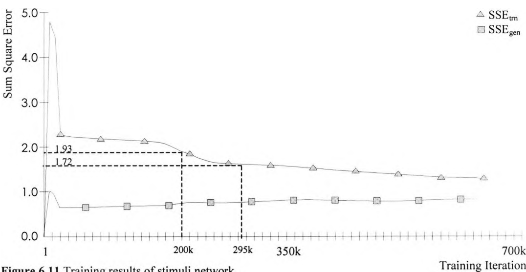
Figure 6.11 Training results of stimuli network.
