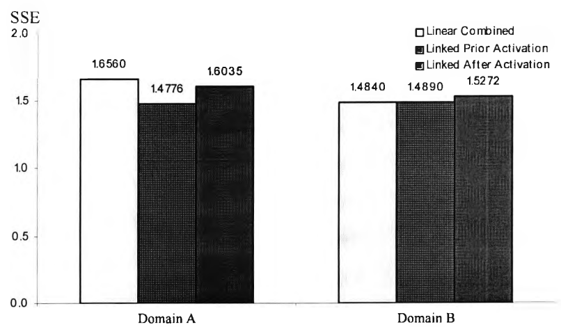
Figure 4.20 Comparison of SSE between different types of network assemblies.
