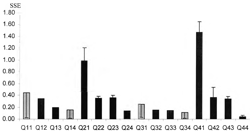
Figure 5.32 Error distribution for each cluster after linking 3 neurons of clusters from figure 5.16.
