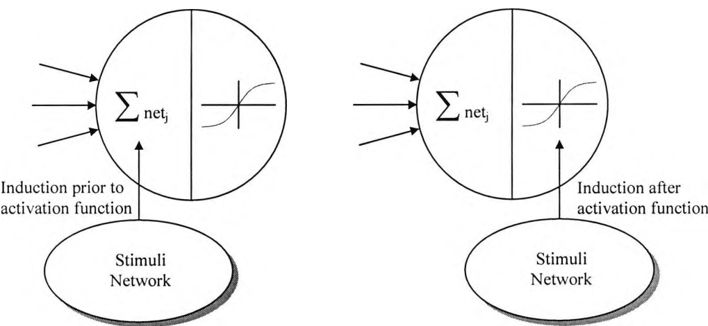
Figure 4.5 Stimuli network induction points prior and after the activation function.
