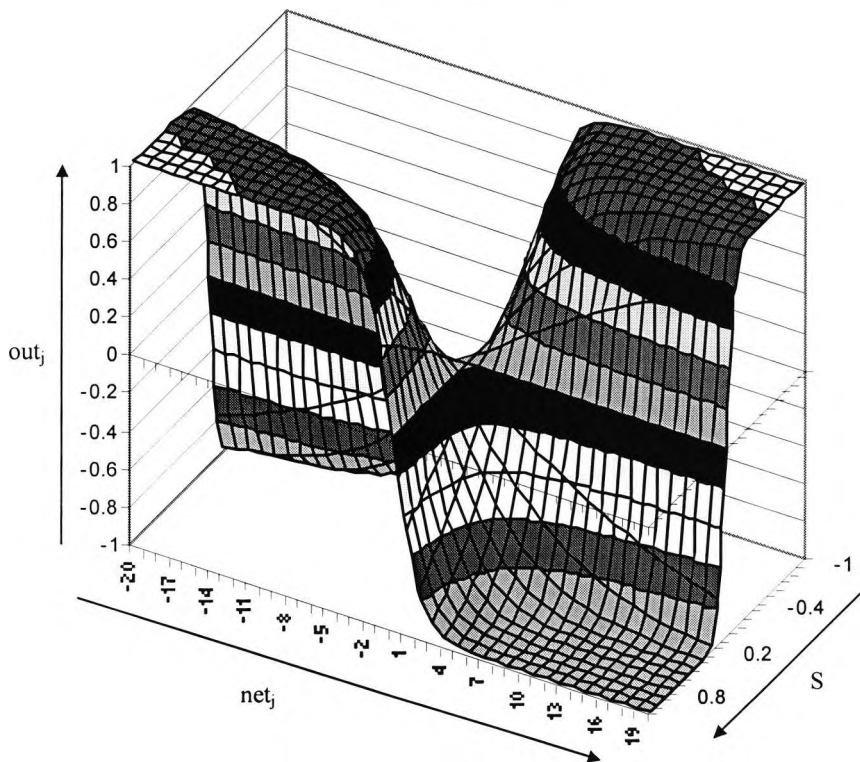
Figure 4.8 Neuron output out_j as a function of net_j and domain membership S .
