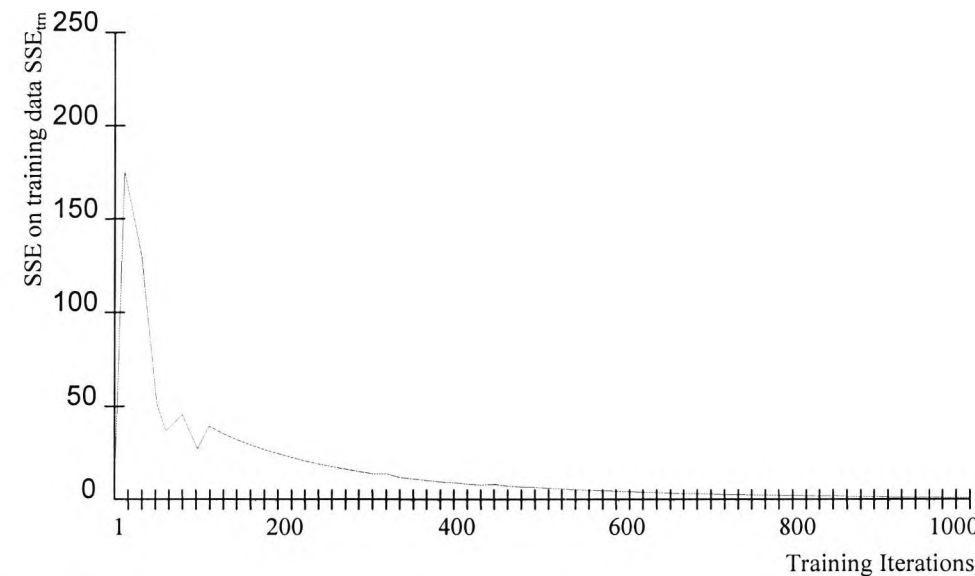
Figure 3.1 SSE_{urn} during training plotted against the number of batch training iterations.
