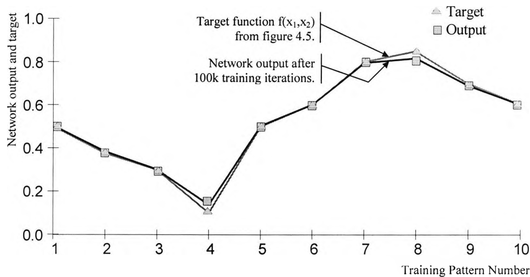
Figure 5.7 The target function plotted against the trained function of network A.
