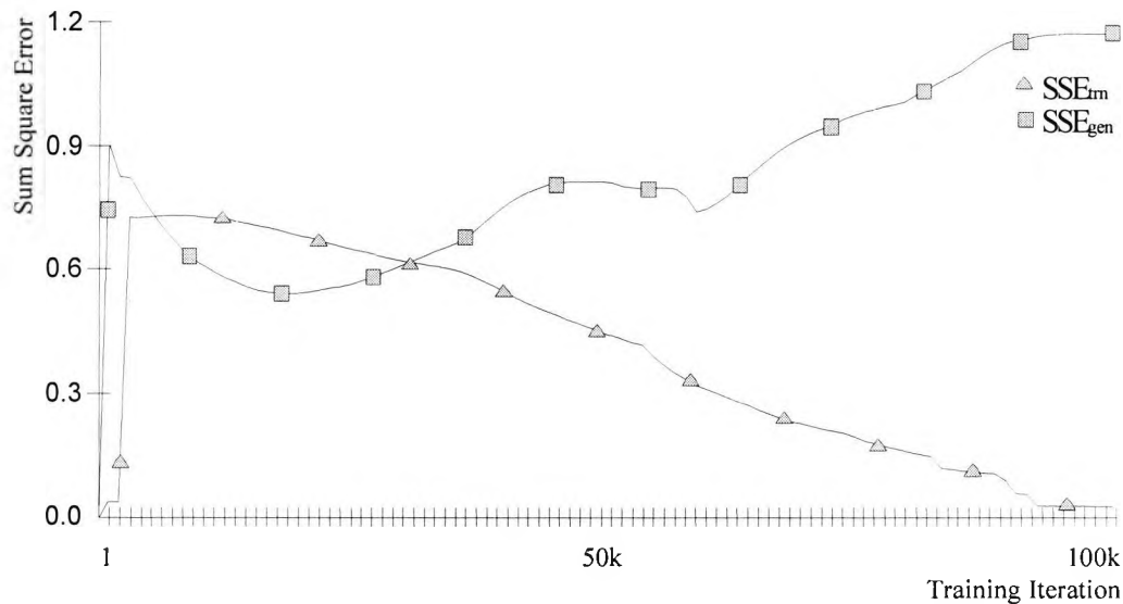
Figure 5.6 The recall and generalisation error during training of network A.
