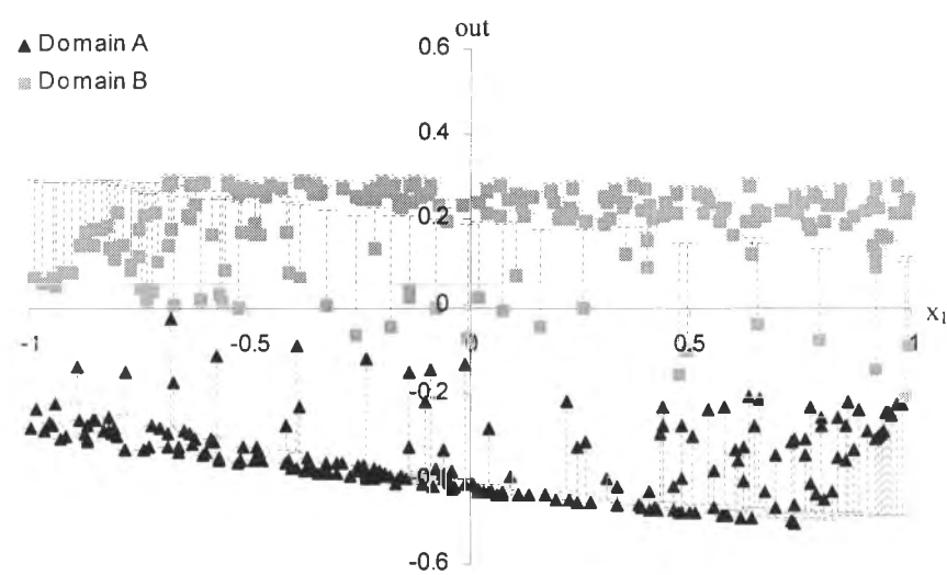
Figure 4.19 Linked output for domain A (▲) and B (■) with stimuli after activation function.
