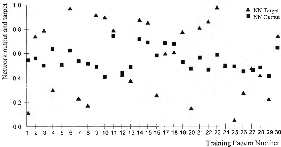
Figure 3.7 The objective function compared with the network output after initialisation.
