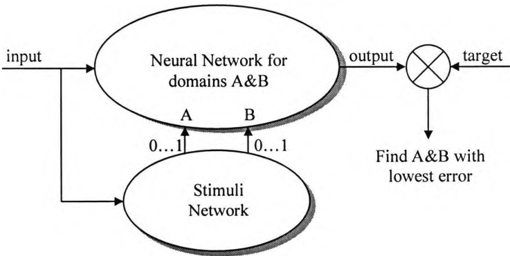
Figure 6.10 Generation of classification data by linear search.
