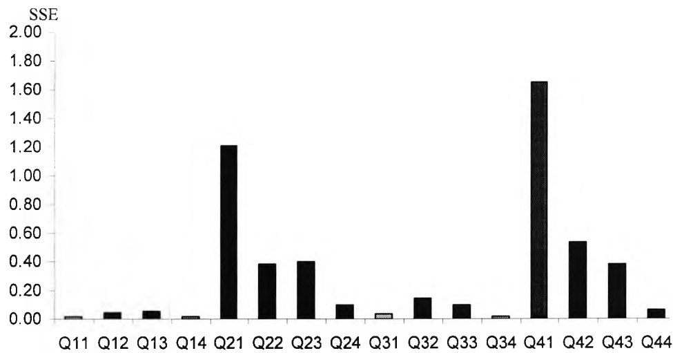
Figure 5.28 Error distribution for each cluster after training of clusters from figure 5.16.
