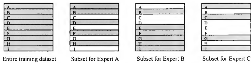
Figure 1.5 Bagging is a bootstrap method where every NN receives different training data.
