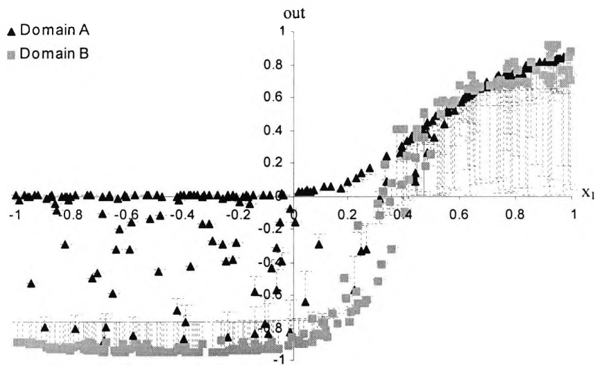
Figure 4.24 Linked output for domain A (▲) and B (■) networks.
