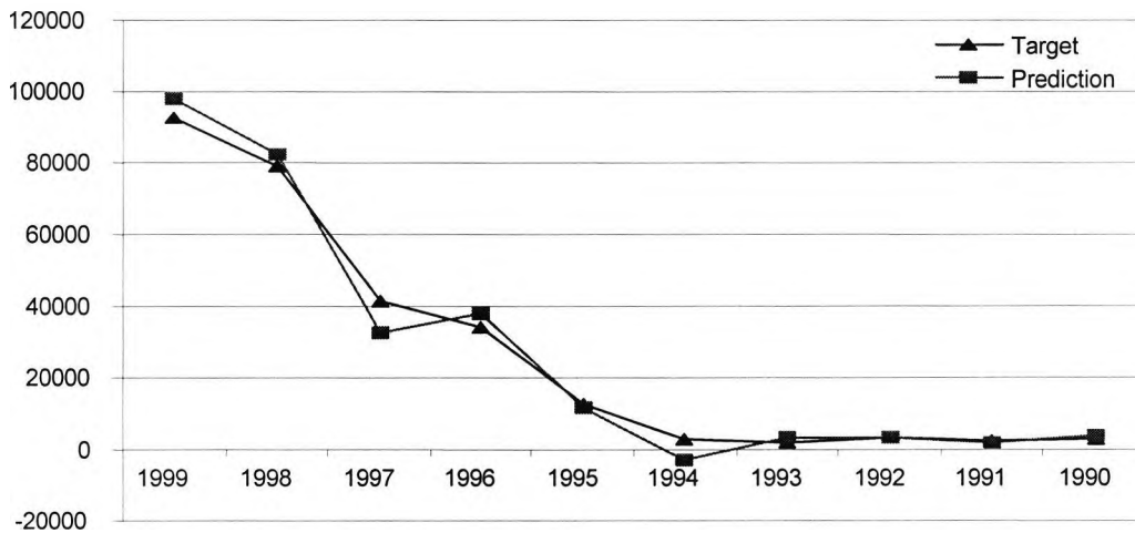
Figure 6.9 Prediction of claims reservation for y-direction after linking.
