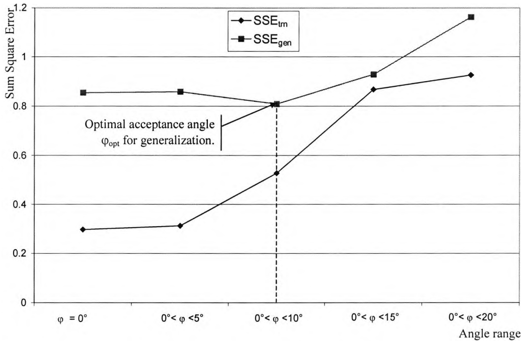
Figure 3.12 SSE_{\text{train}} and SSE_{\text{gen}} as a function of the acceptance angle \varphi for finding \varphi_{\text{opt}} .
