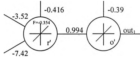
Figure 3.5 Network with only one hidden neuron after linking.
