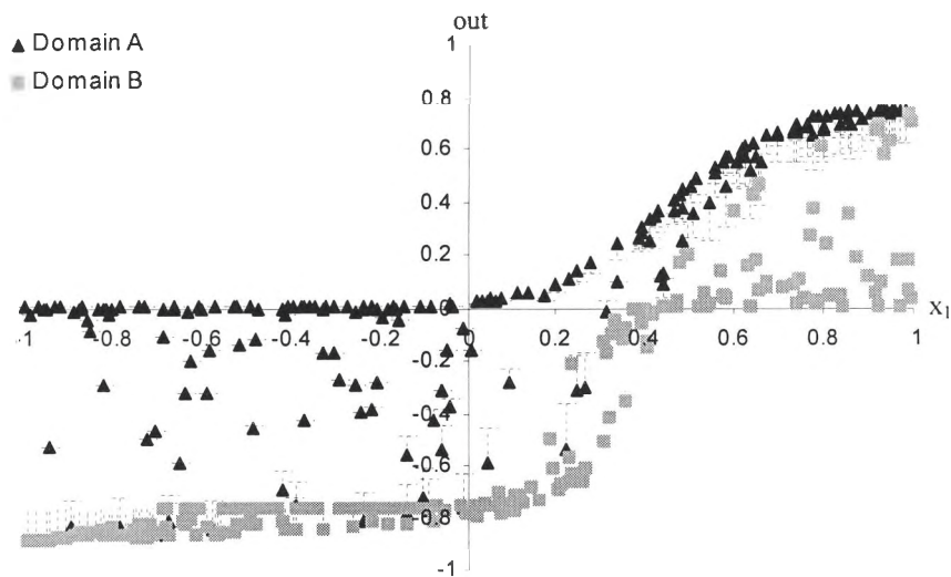
Figure 4.23 Linked output for domain A (▲) and B (■).
