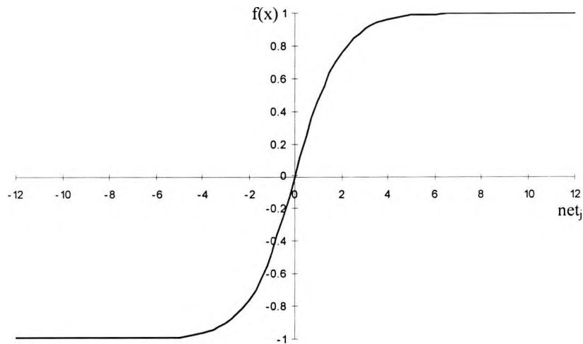
Figure 4.7 Symmetric-sigmoid activation function.
