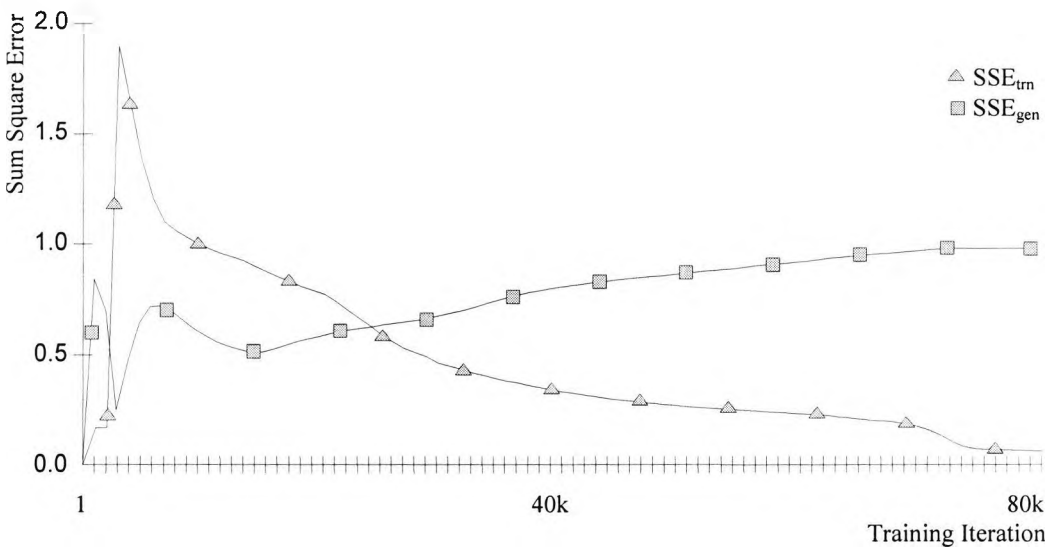
Figure 5.8 The recall and generalisation error during training of network B.
