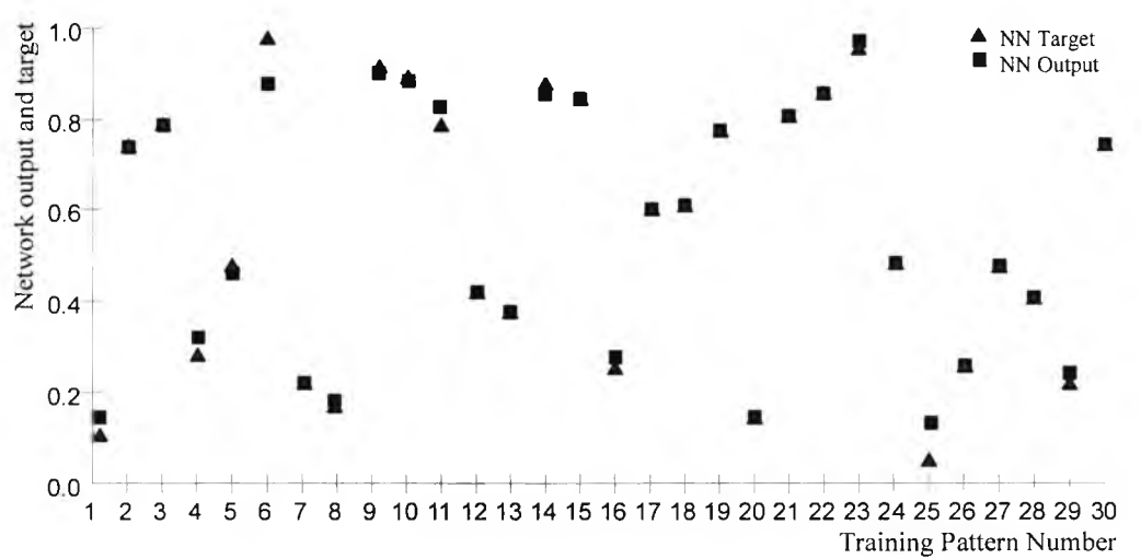
Figure 3.9 The objective function compared with the network output after training.
