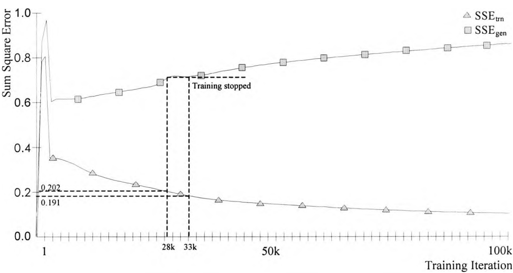
Figure 6.5 Recall and generalisation error of network trained with y-direction data.
