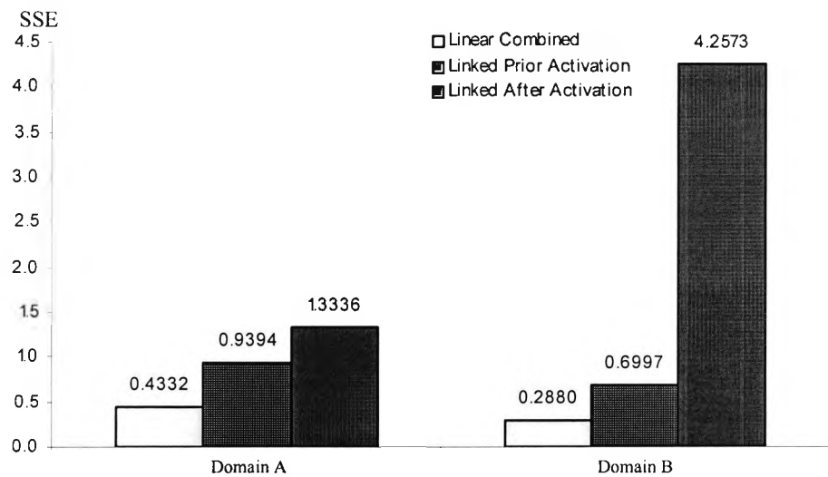
Figure 4.25 Comparison of SSE between different types of network assemblies.
