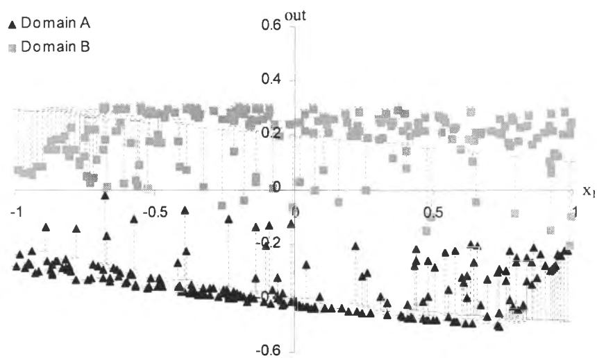
Figure 4.16 Linear combined output for domain A (▲) and B (■) with small weights.
