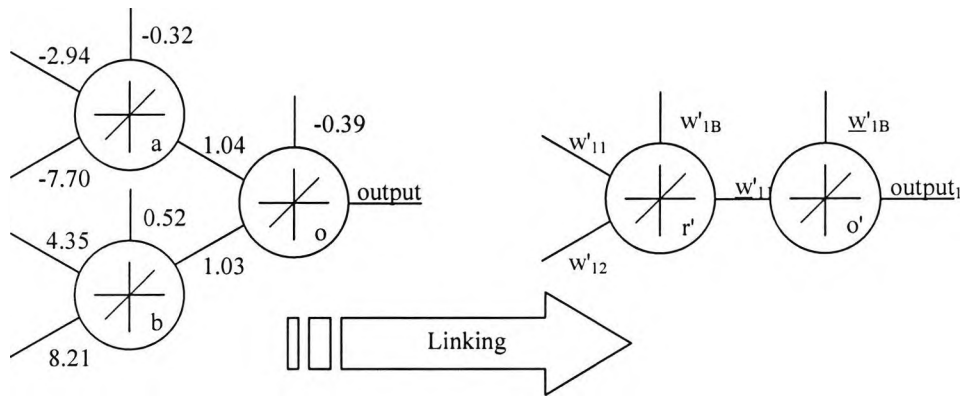
Figure 3.3 Transformation of a 2:2:1 network into a 2:1:1 network by linking of a hidden neuron.
