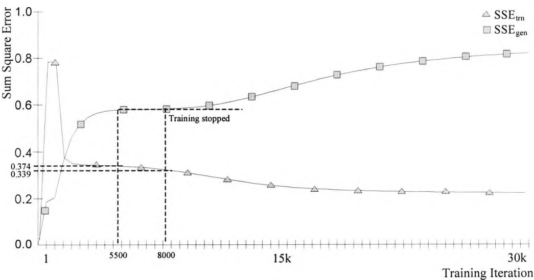
Figure 6.4 Recall and generalisation error of network trained with x-direction data.
