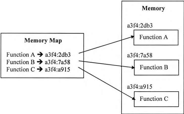
Figure 5.3 In C-based languages use memory maps to locate functions.
