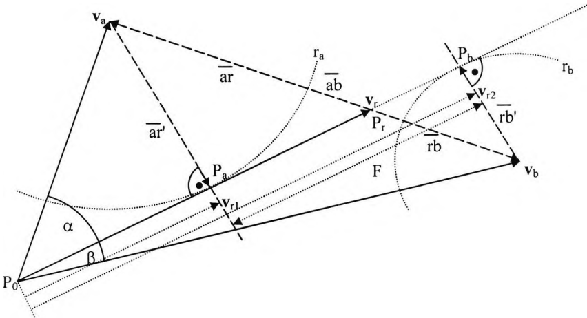
Figure 2.9 Graphical representation of distance reduction by \mathbf{v}_r vector length adjustment.
