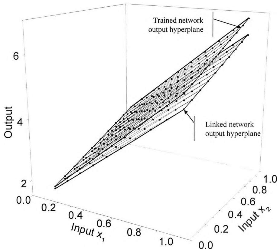
Figure 3.6 The trained and linked network hyperplanes presented for the entire input space.
