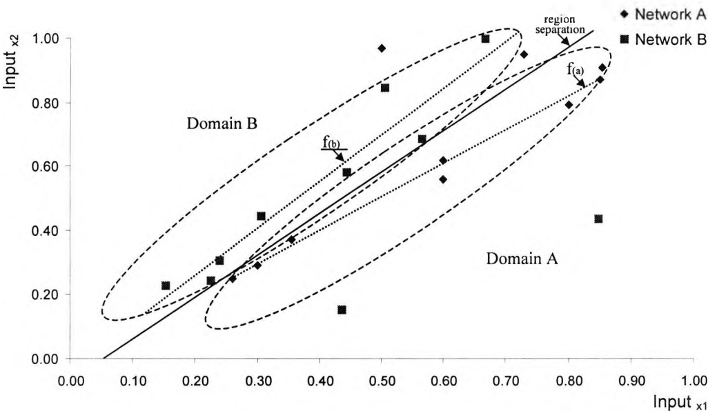
Figure 5.10 Input space separation of the training data.
