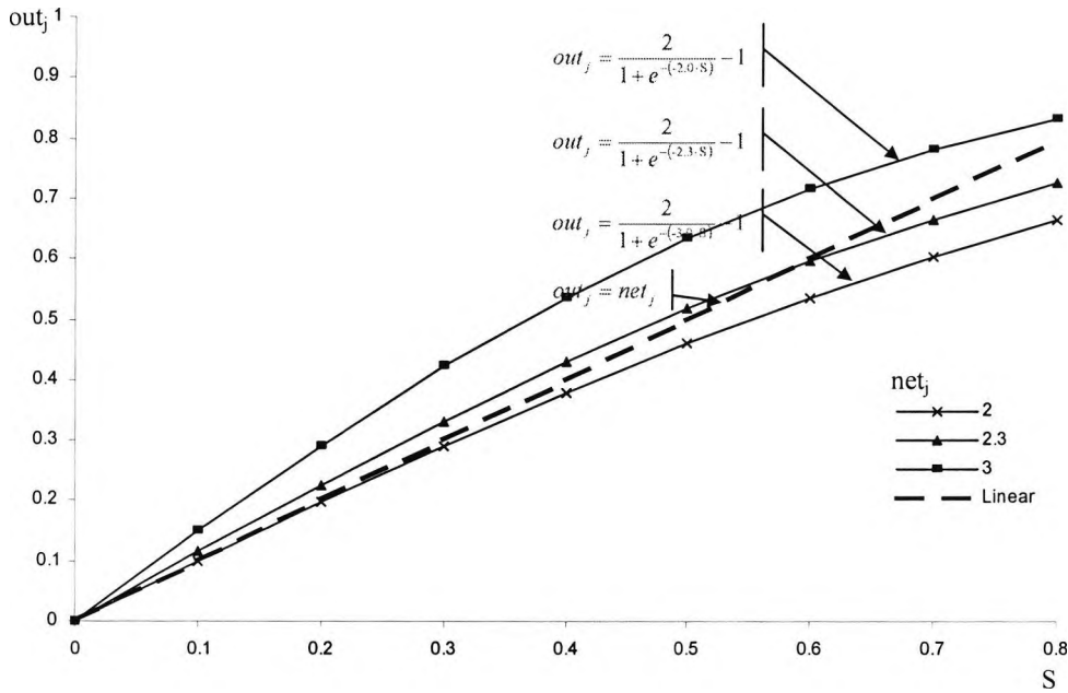
Figure 4.10 Neuron output out_j for to define point of saturation.
