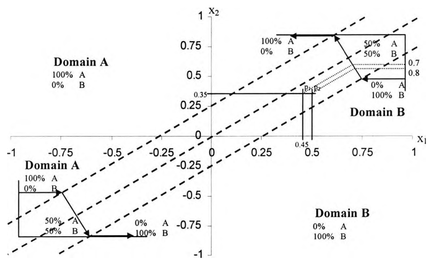
Figure 4.13 Input vector domain membership distribution of domains A and B
