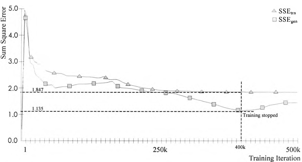
Figure 6.20 Recall and generalisation error of network trained with Legal&General data.
