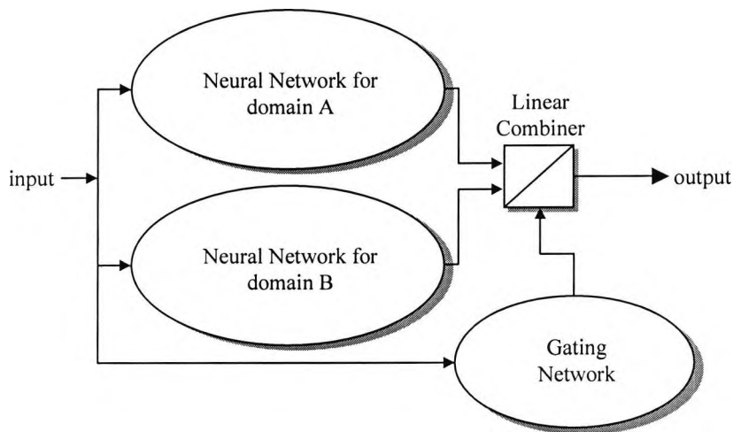
Figure 4.4 Gating networks regulate overall output via a combiner.
