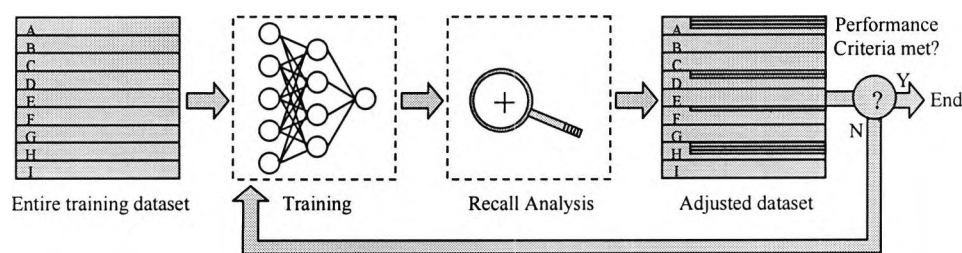
Figure 1.6 With boosting poorly performing records are duplicated to boost performance.
