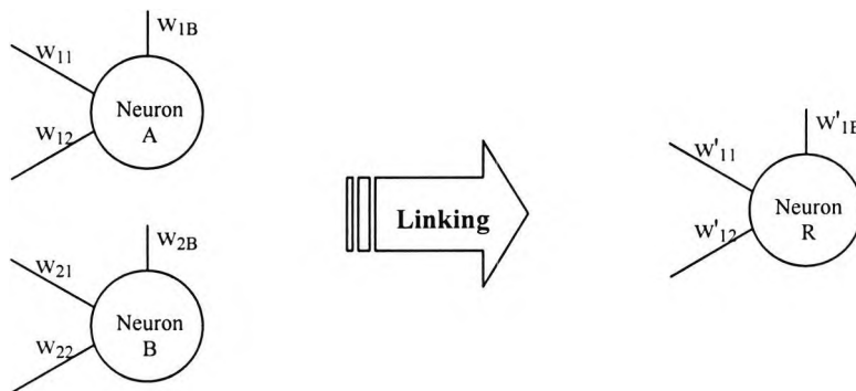
Figure 2.3 Linking of neurons A and B into a neuron R with changes in generalisation.
