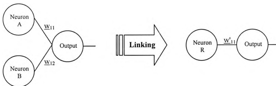
Figure 2.11 Linking hidden neurons requires weight combination from the next layer.
