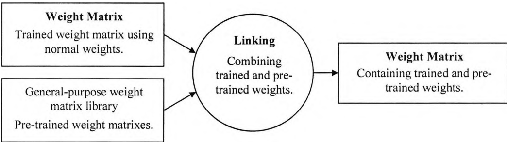
Figure 5.1 Linking trained weights with pre-trained weights from library.
