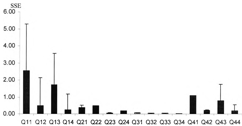
Figure 5.21 Error distribution for each cluster after linking 3 neurons of clusters from figure 5.15.
