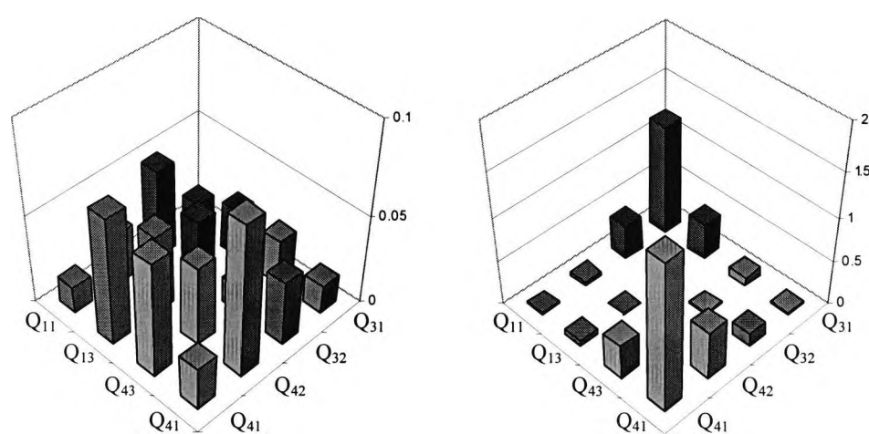
Figure 5.29 Cluster errors after training for A. Figure 5.30 Cluster errors after training for B.
