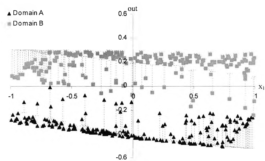
Figure 4.18 Linked output for domain A (▲) and B (■) with stimuli prior to activation function.
