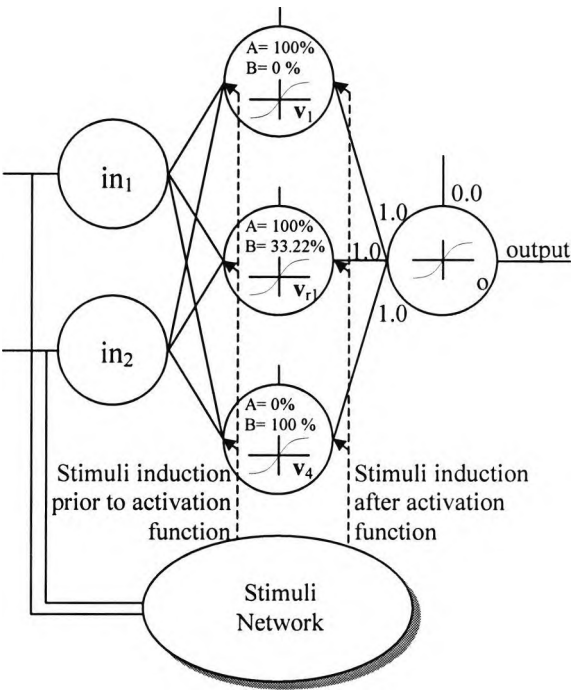
Figure 4.17 Linked neural network for illustration of stimuli induction points.
