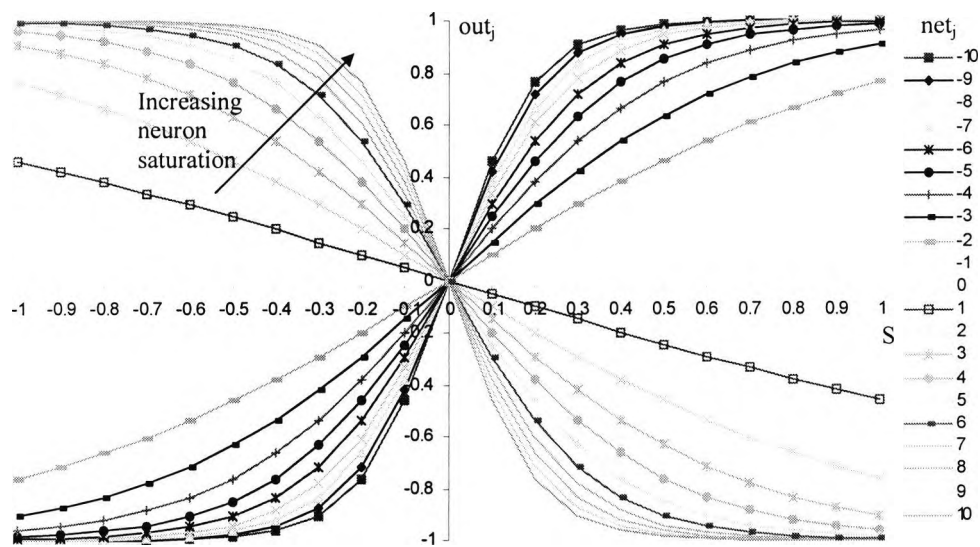
Figure 4.9 Neuron output out_j as a function of parameterised net_j and domain membership S .
