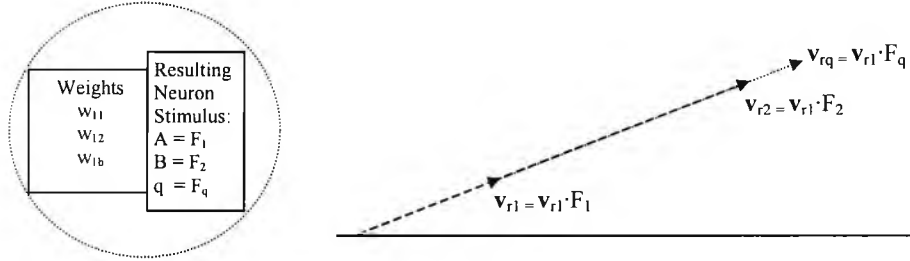
Figure 4.6 Vector length adjustments for recalling information for multiple domains.
