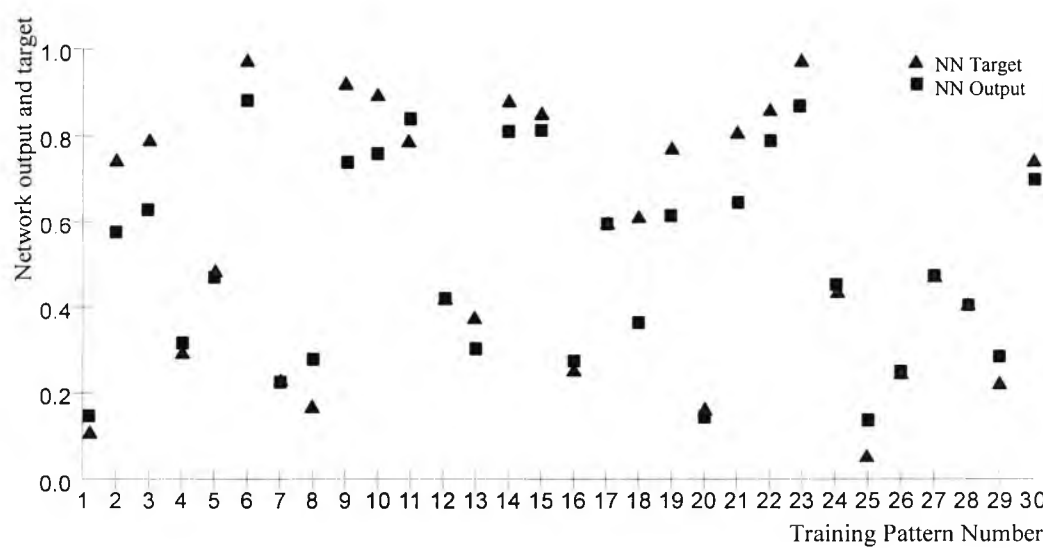
Figure 3.11 The objective function compared with the network output after linking.
