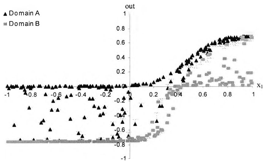
Figure 4.22 Linear combined output for domain A (▲) and B (■).
