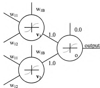
Figure 4.14 Network topology with its frozen output layer.
