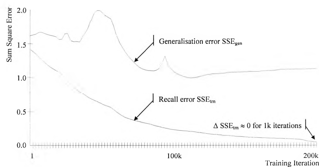
Figure 3.8 The recall and generalisation error during training of the neural network.
