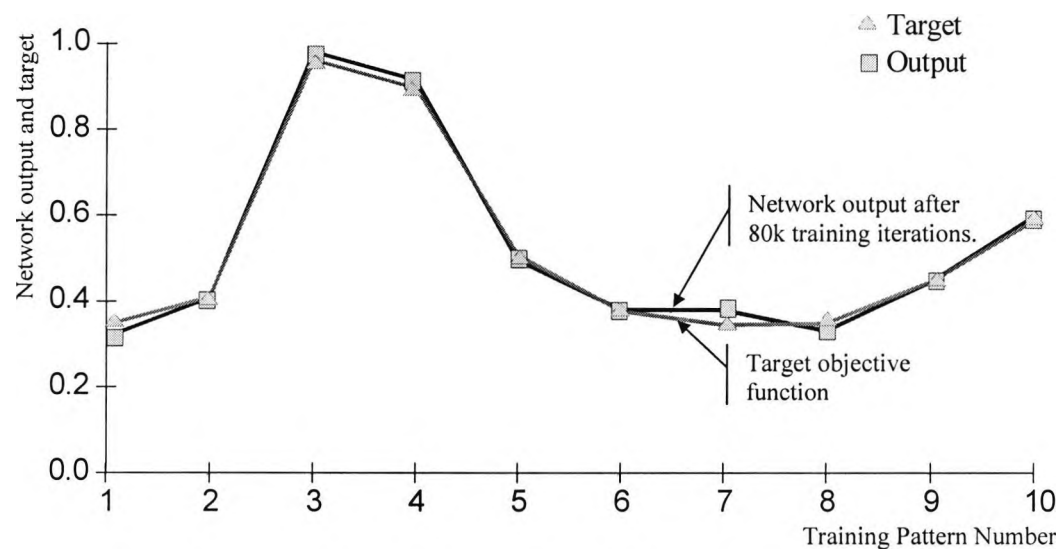
Figure 5.9 The target function plotted against the trained function of network B.
