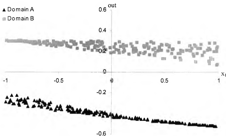
Figure 4.15 Network output for domain A (▲) and B (■) with small weights.
