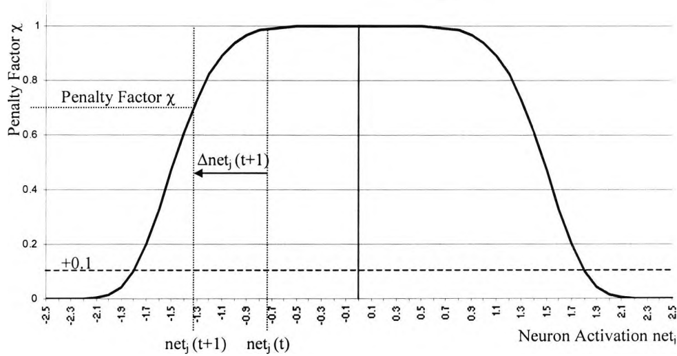
Figure 4.11 Penalty term to adjust the learning factor during training to avoid neuron saturation.
