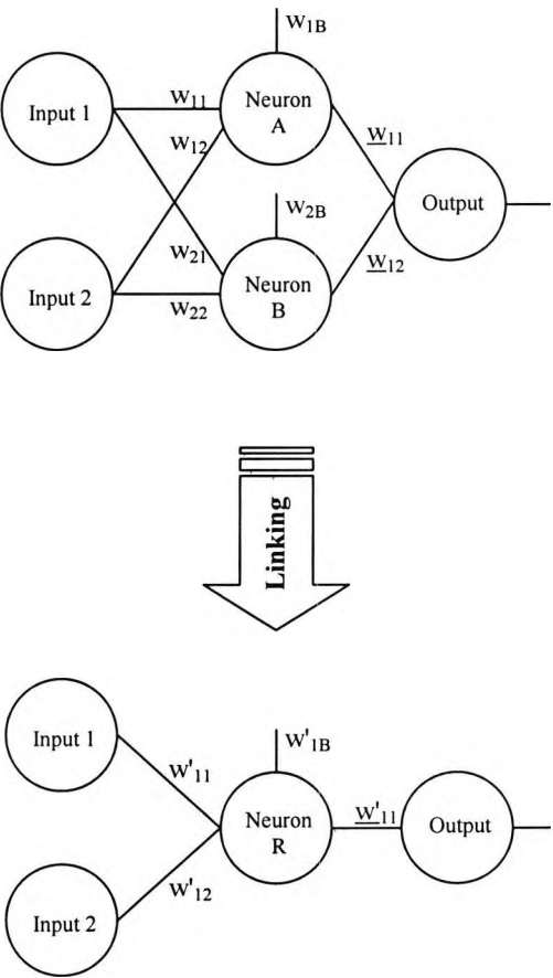
Figure 2.4 Transforming a 2:2:1 network into a 2:1:1 network by linking hidden neurons.
