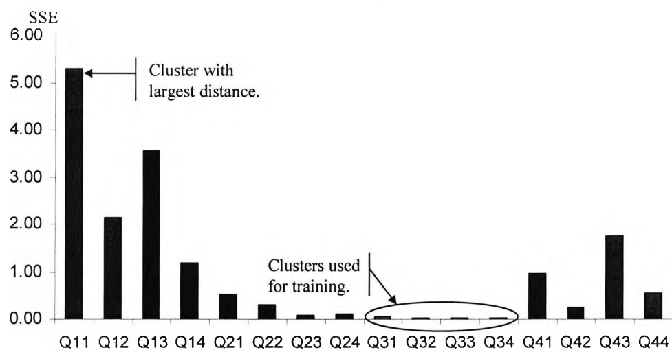
Figure 5.17 SSE for each cluster after training from figure 5.14.
