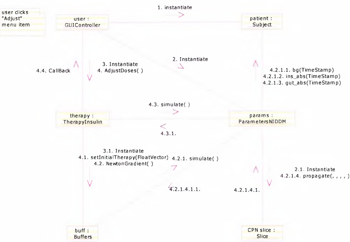
Figure 8.9 Classes involved in the collaboration with interaction represented for the realisation of the ‘Advice’ use case
