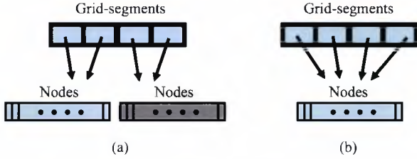
Fig. 13. Grid-segments sharing linear arrangements of node values. (a) Every two grid-segments share a different arrangement of nodes. (b) One arrangement of node values is shared among four grid-segments.
