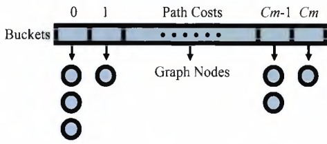
Fig. 4. Priority queue based on buckets. The buckets are arranged linearly and sorted by cost. Each bucket is associated with a list of graph nodes.
