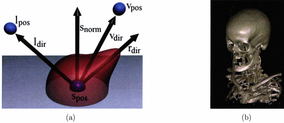
Figure 4.6: The Phong lighting model shown in (a) can be used to compute lighting intensities at each point on the surface. The result is a images like that shown in (b).
