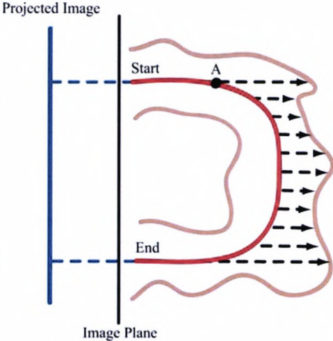
Fig. 5. Rendering a projected Volumetric CPR of a tubular structure. This ray pattern gives an image like Fig. 3a when applied to the colon.
