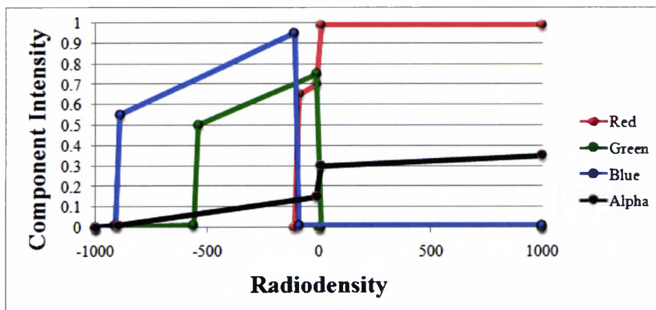
Figure 8.3: The transfer function for translucency rendering in the colon (as originally given by [62]).
