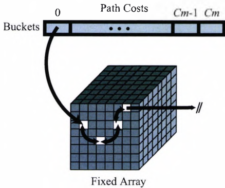
Fig. 5. Three-dimensional linear-time priority queue for the IFT watershed. Four nodes have been enqueued in bucket 0.
