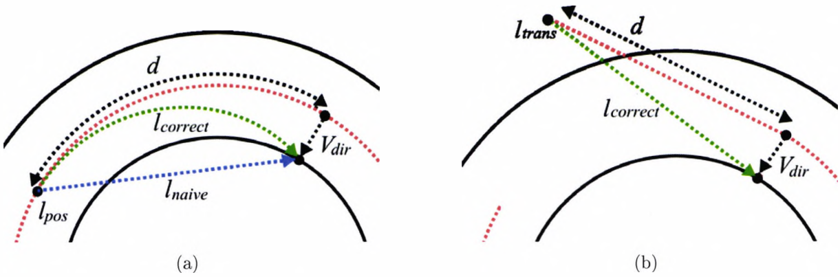
Figure 8.8: Using the naive approach, the light vector l_{naive} is computed straight from the light to the surface; once straightened this results in the light coming from the wrong direction (a). The correct path for the light l_{correct} curves with the structure. Rather than actually curving the light rays, we mimic the effect by transforming the light source as shown in (b).
