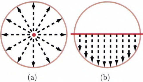
Figure 6.9: Rendering a stretched Volumetric CPR of a tubular structure. This ray pattern gives an image like Figure 6.3(c) when applied to the colon.
