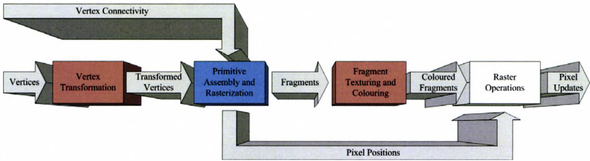
Figure 11.5: The graphics pipeline as implemented on most GPUs. The stages in red are programmable on most GPUs whereas the blue stage is only programmable on the latest NVidia GeForce 8 series. The white stage is generally not programmable.
