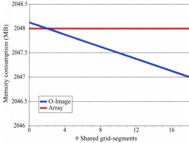
Fig. 12. Comparison of memory consumption between a traditional three-dimensional array and an O-Image in a 32-bit system, with respect to the number of shared grid-segments in the O-Image. The image has a size of 1024^3 and the grid-segment size is 32^3 .
