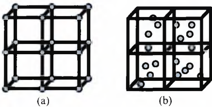
Fig. 6. Sampling methods for three-dimensional images. (a) Samples on a conventional image. (b) Samples in an O-Buffer.
