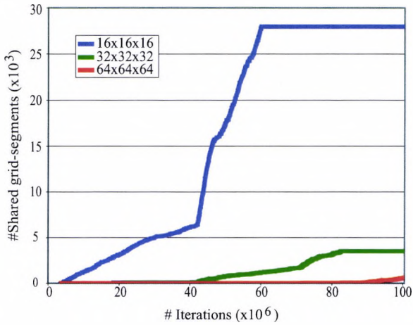
Fig. 15. Varying the grid-segment size in the O-IFT-OB. Comparison of number of shared grid-segments per iteration during the propagation stage in the O-IFT-OB for Dataset 2.
