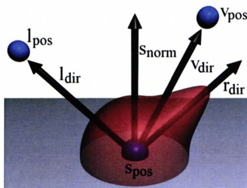
Figure 8.5: The vectors required to compute the Phong lighting for a given point on the surface. s_{norm} is the surface normal, l_{dir} points toward the light source, v_{dir} points toward the camera, and r_{dir} is the reflection of l_{dir} about s_{norm} .
