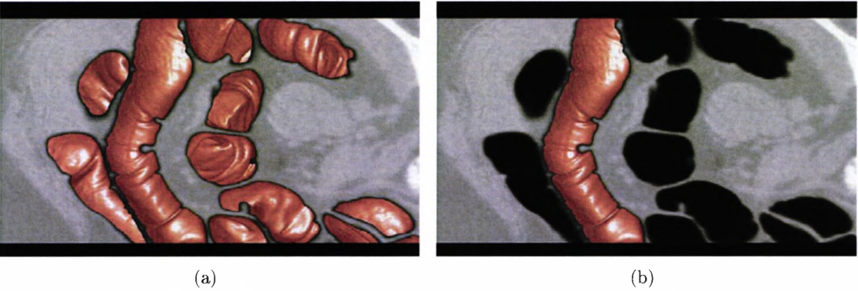
Figure 6.13: Region-growing can be used to restrict the number of pixels for which direct volume rendering is performed. Without region growing (a) areas not of immediate interest are still augmented with direct volume rendering. Using region growing rectifies this (b).
