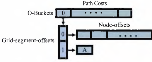
Fig. 11. Example of nodes grouped by their grid-segment-offset in O-Bucket 0. Since nodes are always dequeued from the first grid-segment-offset entry in the O-Bucket, node A is only dequeued after all nodes with grid-segment-offset 0 are.
