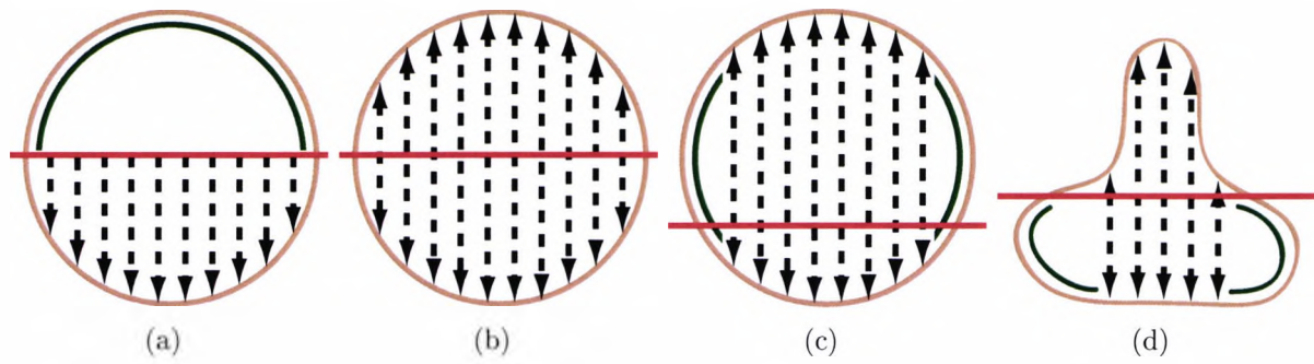
Figure 6.17: In Volumetric CPR only half the surface of the tubular structure is covered (a) as the areas marked in green are missed. This can be rectified by rendering two images with the rays going in opposite directions (b). However, this solution can fail if the centreline is not accurate (c) or if the cross-section is a more complex shape (d).
