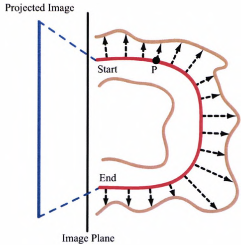
Figure 6.9: Rendering a stretched Volumetric CPR of a tubular structure. This ray pattern gives an image like Figure 6.3(c) when applied to the colon.
