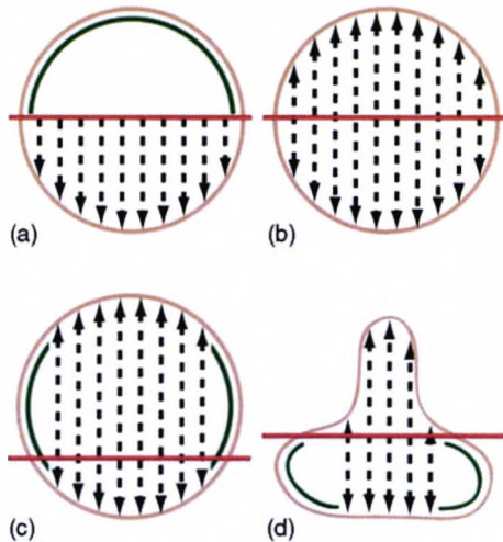
Fig. 16. (a) In Volumetric CPR, only half of the surface of the tubular structure is covered as the areas marked in green are missed. (b) This can be rectified by rendering two images with the rays going in opposite directions. However, this solution can fail if (c) the centerline is not accurate or if (d) the cross section is of a more complex shape.
