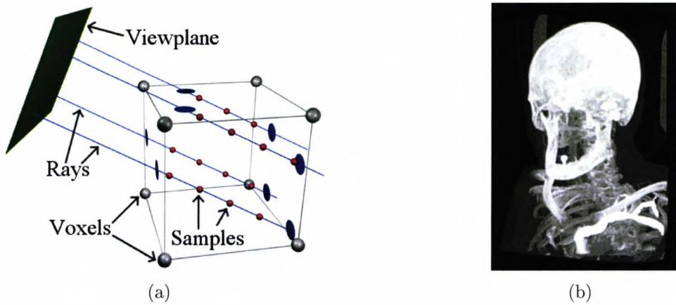
Figure 4.5: Maximum Intensity Projection (MIP) generates images using raycasting (a). The results are particularly useful for visualising high density structures such as bone(b)
