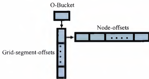
Fig. 9. Schematic drawing of an O-Bucket. The O-Bucket is associated with a set of grid-segment-offsets, each one associated with a set of node-offsets.
