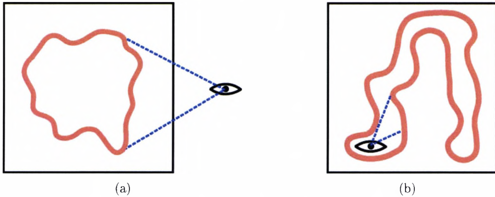
Figure 5.4: In the general case of volume visualisation (a) the majority of the volume can be visible at any given time. In the case of endoscopic rendering (b) there is more occlusion meaning a smaller amount of data has to be taken into account.
