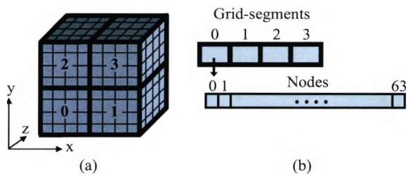
Fig. 8. Example of image subdivision into grid-segments. (a) Original 8x8x4 image divided in 4 grid-segments, in xyz order. (b) The 4 grid-segments are arranged linearly, as are their internal 64 nodes.
