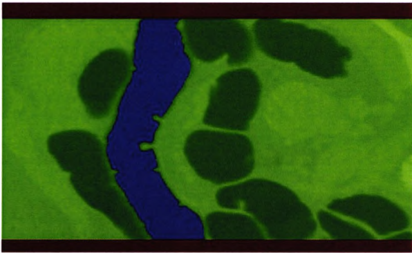
Figure 6.15: Pixels are tinted blue if they were originally black, are inside the image, and are connected to the centreline; these pixels should be raycast. Pixels are tinted red if they were originally black but fell outside the image. The remainder of the pixels are tinted green and either were not originally black or were originally black but not connected to the centreline.
