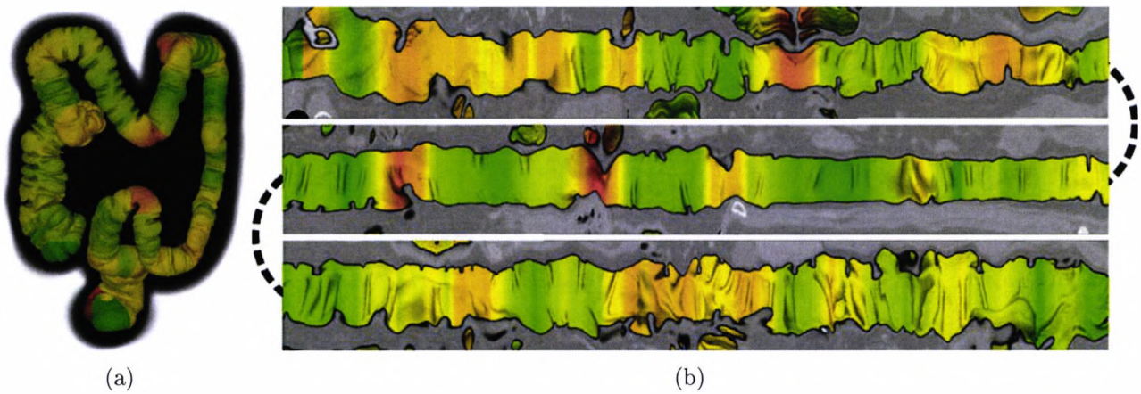
Figure 8.12: The result of mapping the direction of the tangent at a given point to the colour of the light. In this case, Equation 8.10 was used to perform the mapping.
