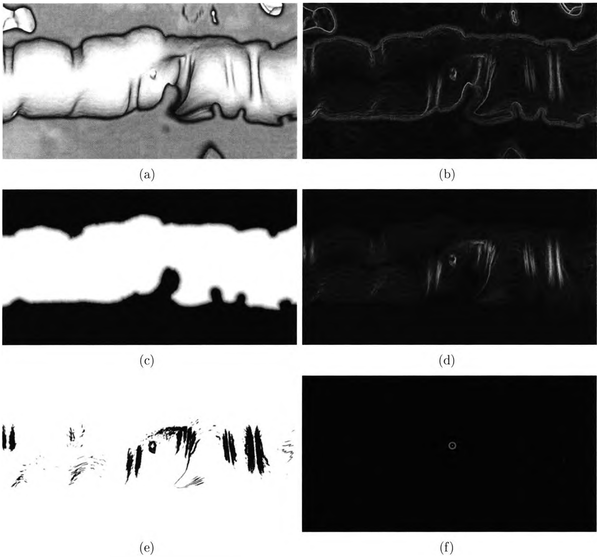
Figure 11.2: Our prototype implementation took the input image (a) and applied a Sobel edge detection image filter (b). To avoid finding polyps outside the colon a mask (c) was applied to give the image in (d). Thresholding was applied (e) and the result was processed using the Hough transform for circle detection. In the final image (f) a bright spot can be seen at the location of the polyp (ringed in red).
