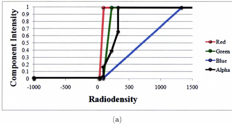
Figure 4.7: The graph in (a) shows the intensity of the red, green, blue and alpha channels corresponding to given radiodensities. Applying this transfer function to the dataset gives the image in (b).
