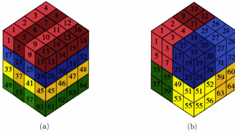
Figure 2.4: The numbers on each voxel show the memory offset at which each voxel is stored. A linear layout (a) places voxels, rows, and slices consecutively in memory. The block memory layout (b) groups adjacent voxels in order to improve cache coherency.
