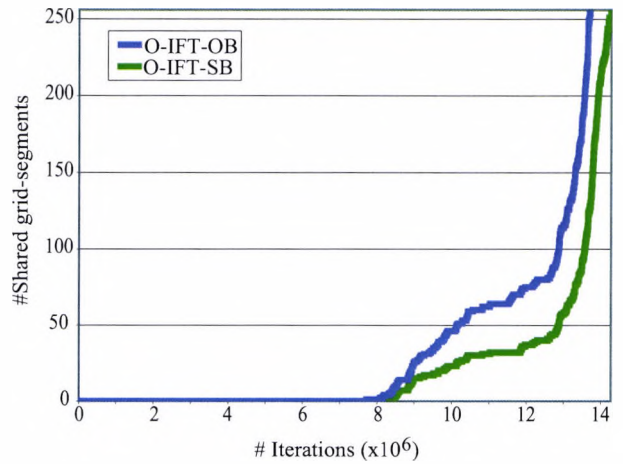
Fig. 16. Comparing the O-IFT-OB with the O-IFT-SB. Number of shared grid-segments per iteration during the propagation stage in the O-IFT-OB and the O-IFT-SB for Dataset 1.
