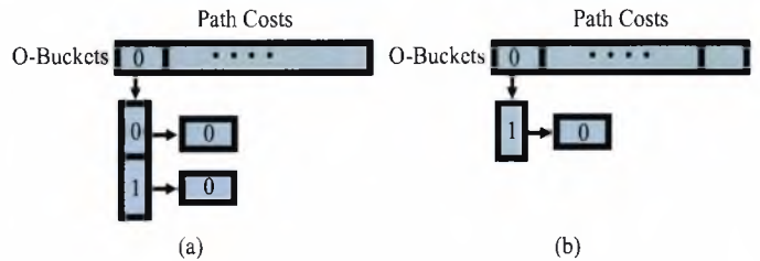
Fig. 10. Examples of operations in the O-Buckets. (a) Example of enqueueing showing insertion of nodes with positions (0,0) and (1,0) in O-Bucket 0. (b) Example of dequeuing showing removal of node (0,0) from the O-Bucket 0 shown in (a).
