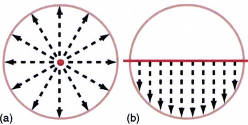
Fig. 10. (a) During colon flattening, the rays radiate from the centerline. (b) During stretched Volumetric CPR, they are all normal to the curve.
