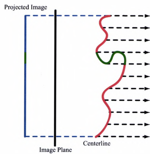
Figure 6.4: Ray pattern for the Volumetric CPR. The area shown in green is where occlusion occurs.
