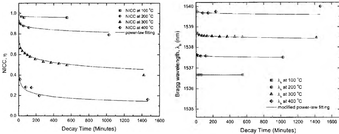
Figure 4-9: Thermal decay characteristics of type I B/Ge FBGs at various temperatures. [23]
