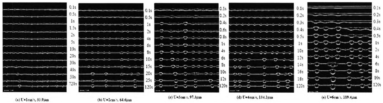
Figure 4-14: Effect of film thickness on the development of instability. Pictures show polypropylene fibres (radius: 100\mu\text{m} ) coated with ethylene oxide/propylene oxide fluid. [32]
