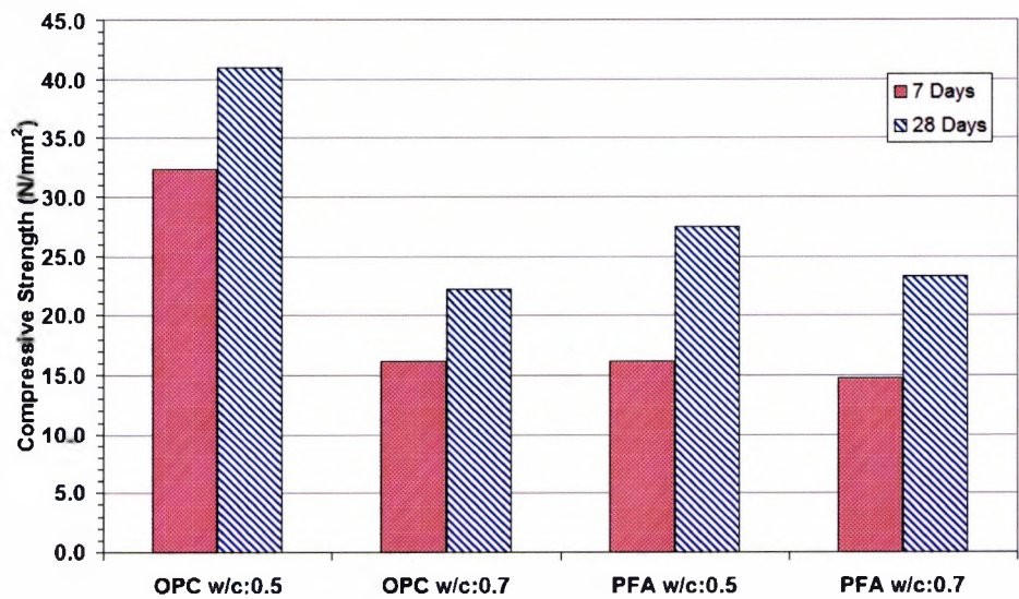
Figure 5-10: Average compressive strength of OPC and PFA samples obtained at 7 days and 28 days.
