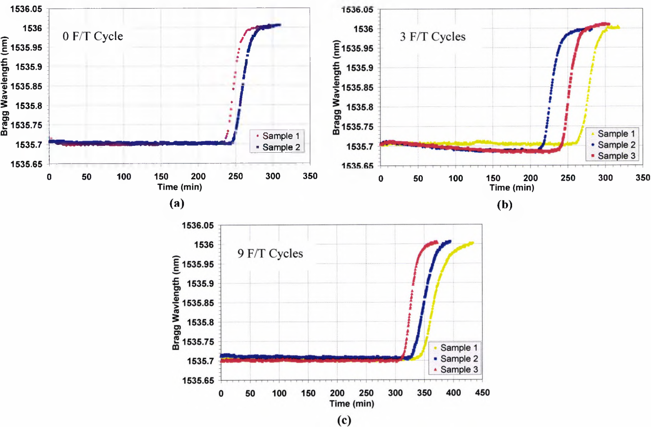
Figure 5-18: Moisture ingress responses of various concrete samples. (a) control samples without freeze/thaw damage, (b) samples with 3 freeze/thaw cycles and (c) samples with 9 freeze/thaw cycles.
