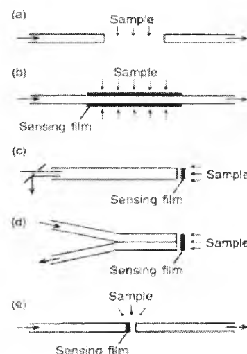
Figure 3-6: Various configurations for spectroscopic fibre-optic sensors. [16]
