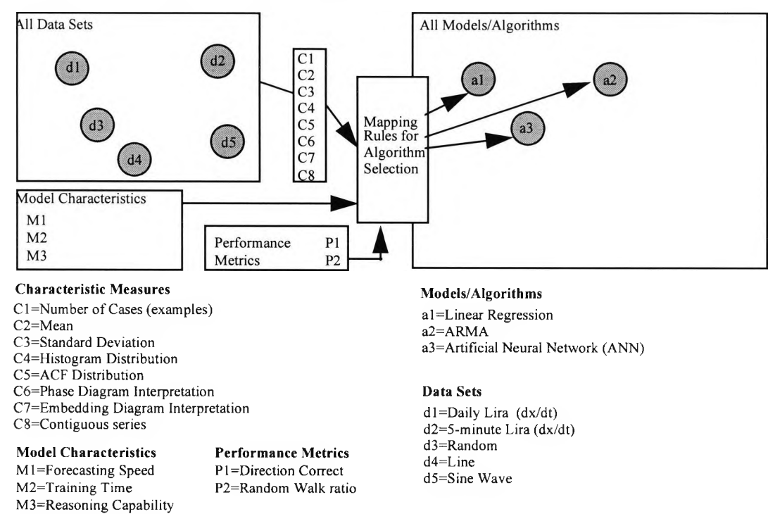
Figure 4.11 - Summary of experimental method : forecasting
