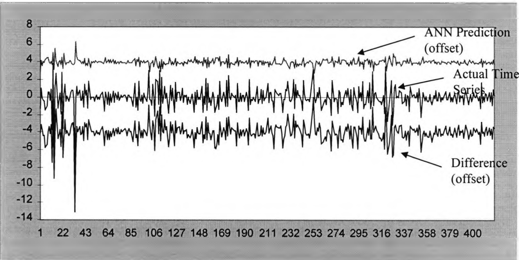
Figure B.15 Experiment 5 prediction (RWR=0.89, DC=59.29%)
