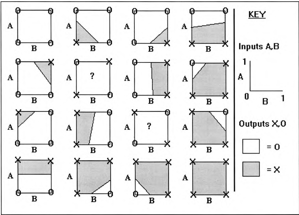
Figure 2.5 - Weight space separation for (arbitrary) solutions to perceptron logic functions
