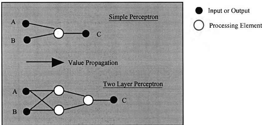
Figure 2.3 - Simple & Two Layer 3 Perceptron.
