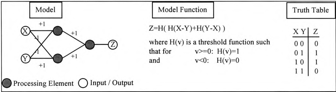
Figure 2.6 MLP solution to the X-OR problem
