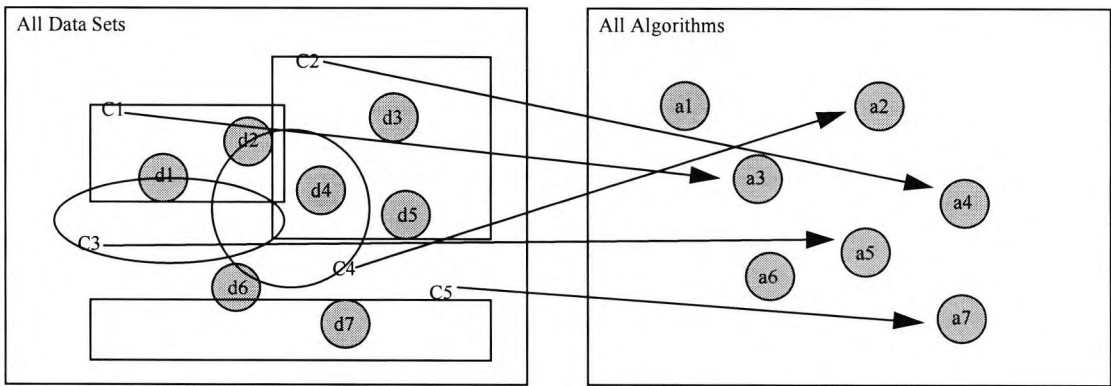
Figure 3.3 - Simple characteristics-algorithms mapping
