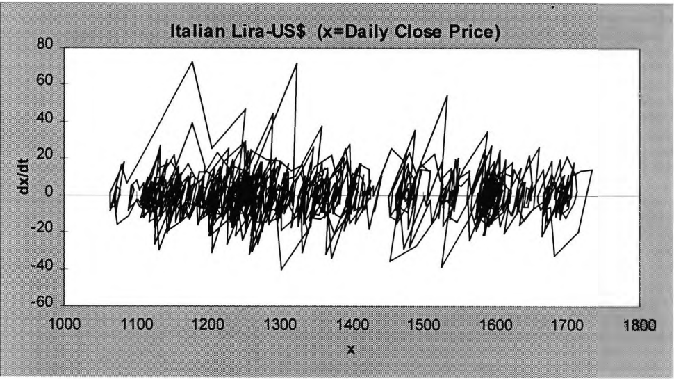
Figure B.11 - Phase diagram of Italian Lira ( x vs dx/dt )
