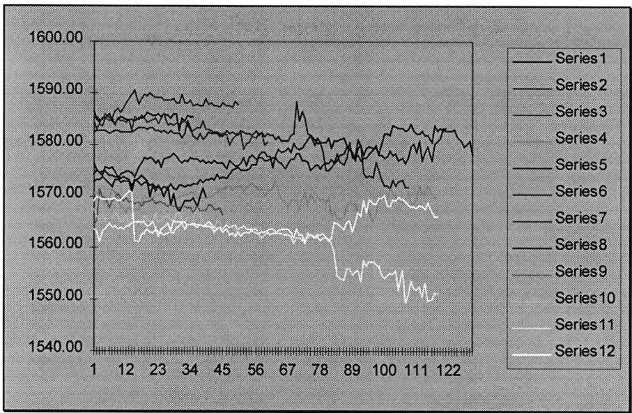
Figure B2 - Twelve continuous Lira time series (five minute samples)
