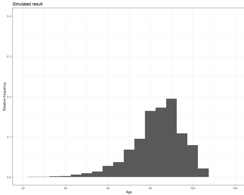
(b) Histogram from the simulation
