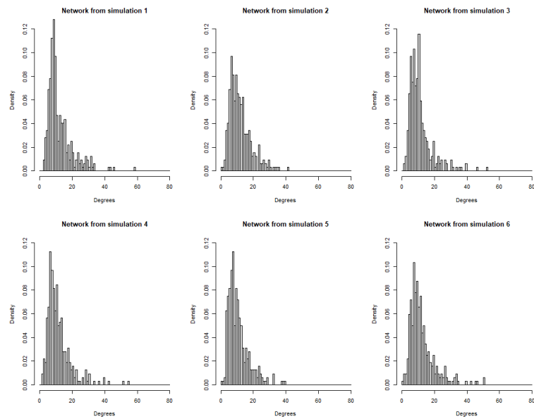
Figure 4.12: Degree distribution of the simulations
