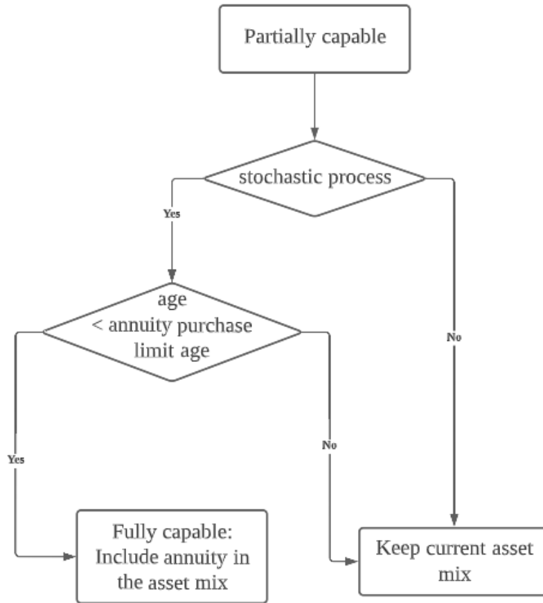
Figure 3.4: Flow chart of the state change
