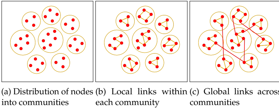
Figure 4.1: BTER model construction
