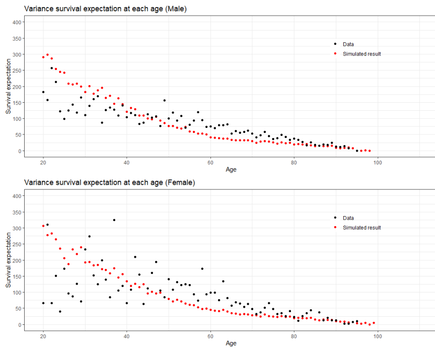
(b) Variance of survival expectation(male& female)
