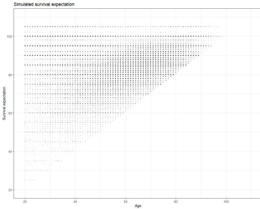
Figure 1.7: Scatter plot of survival expectation from 100 simulations
