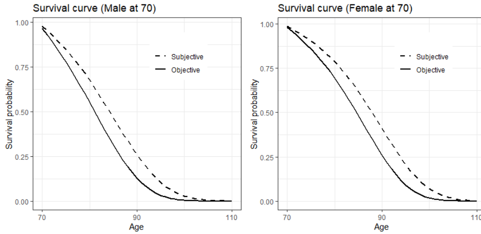
Figure 3.1: Reproduced subjective survival curves from Gan et al., 2015 (dotted) and objective survival curves from 1995 life table (solid).
