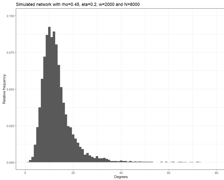
(b) Simulated network
