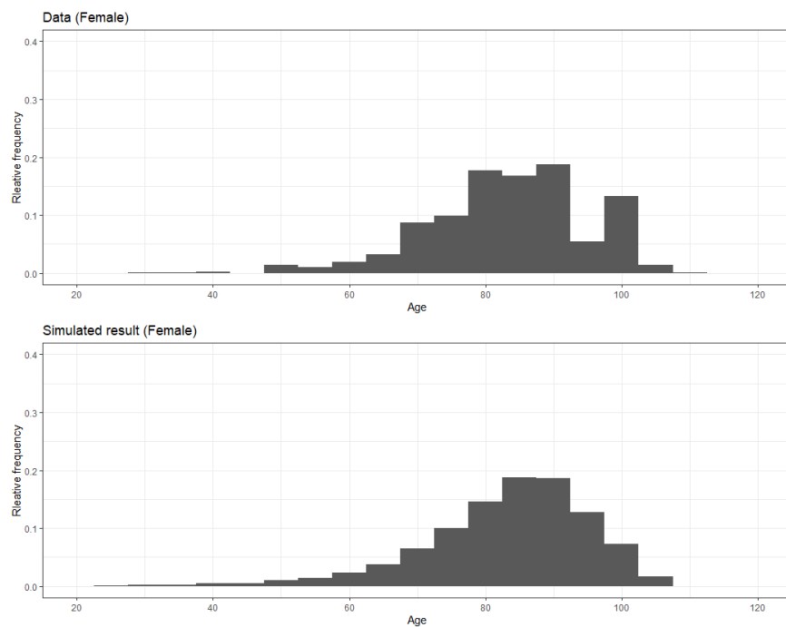
(b) Histogram of female survival expectation from data (above) and simulation (below)
