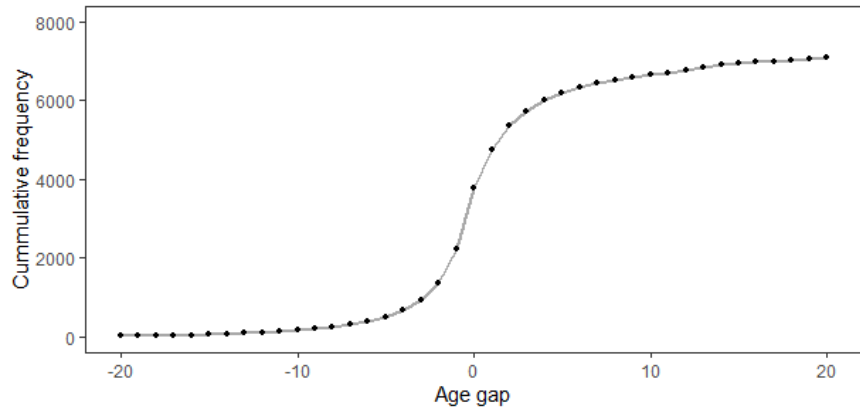
(a) Cumulative frequency of the age gap
