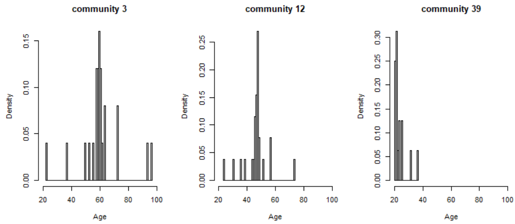
Figure 4.10: Distribution of agents' age within a community
