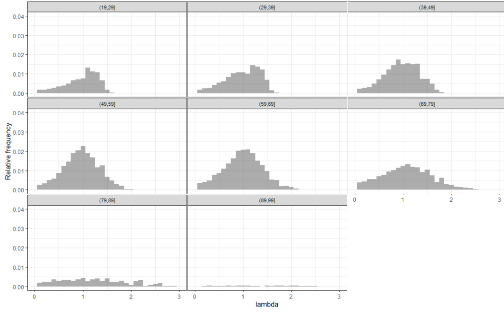
Figure 2.6: Histograms of \lambda_i by cohorts from the 100 simulations
