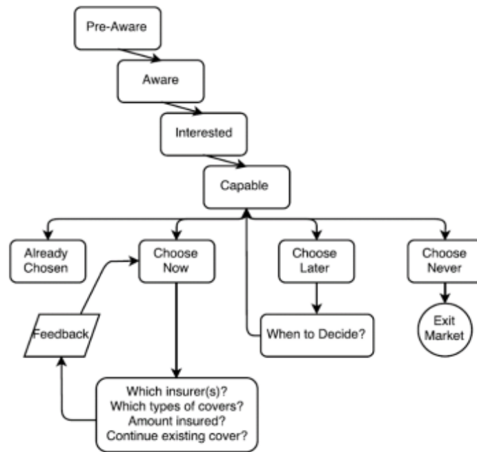
Figure 3.3: Flowchart of decision states model. (Source:Bateman et al. (2020))
