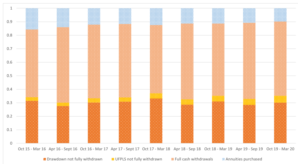
Figure 5.2: Proportion of savings account for each option. Source: The FCA Retirement income market data
