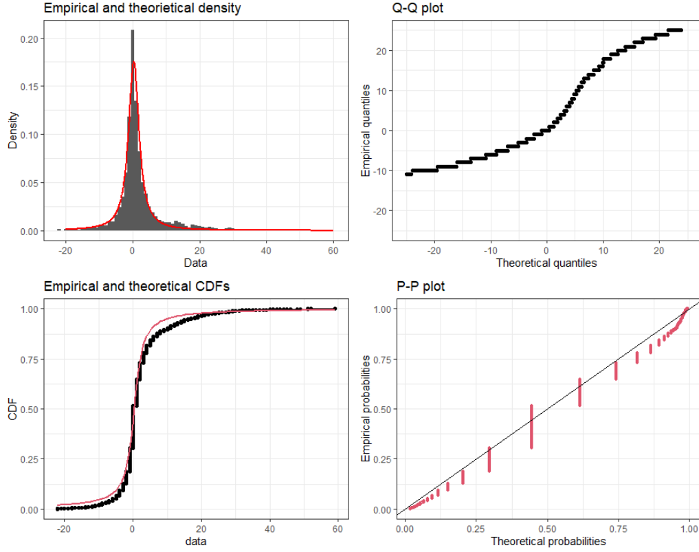
Figure 4.7: Fitting of the t -distribution to the Dutch women friendship age gap data.
