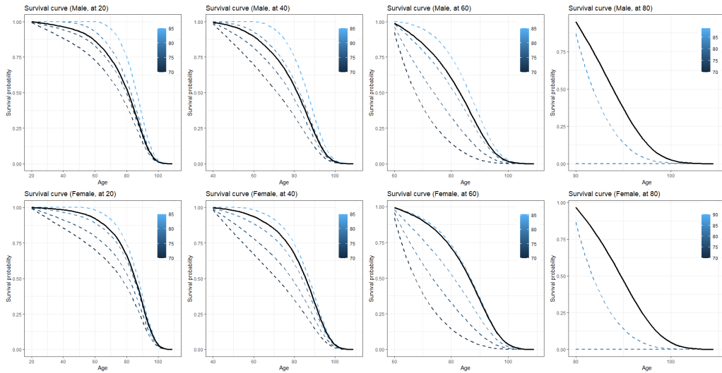
Figure 3.5: Subjective survival curves (dotted) with parameter \omega_i corresponding to the survival expectations from age 70 to 85 and objective survival curves
