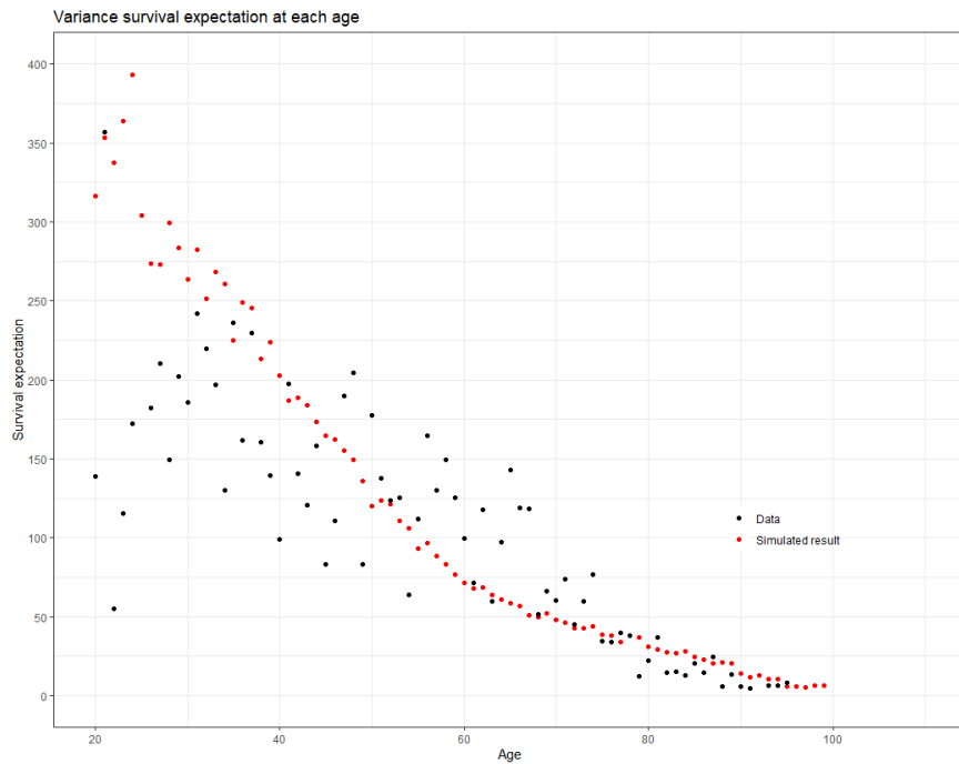
(b) Variance of survival expectation at each age
