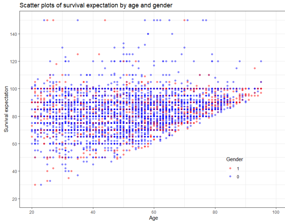
Figure 1.1: Scatter plot of survival expectation by age and gender (Source: The SCF, 2010)
