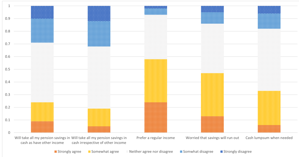
Figure 5.3: NAPF Survey on accessing pension savings at retirement
