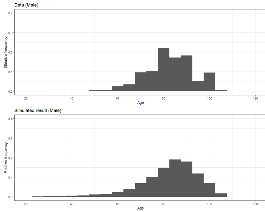
(a) Histogram of male survival expectation from data (above) and simulation (below)
