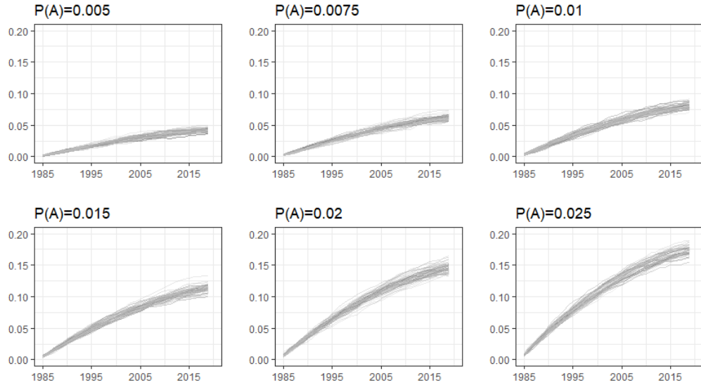
Figure 2.7: 100 simulations with P(A) = 0.005, 0.0075, 0.01, 0.015, 0.02, 0.025 from 1985 to 2020
