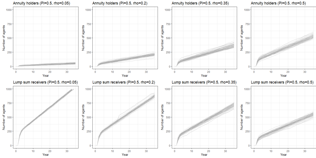
Figure 5.7: Number of annuity holders and lump sum receivers from 50 simulations with \Pi = 0.5 and \rho = (0.05, 0.2, 0.35, 0.5)
