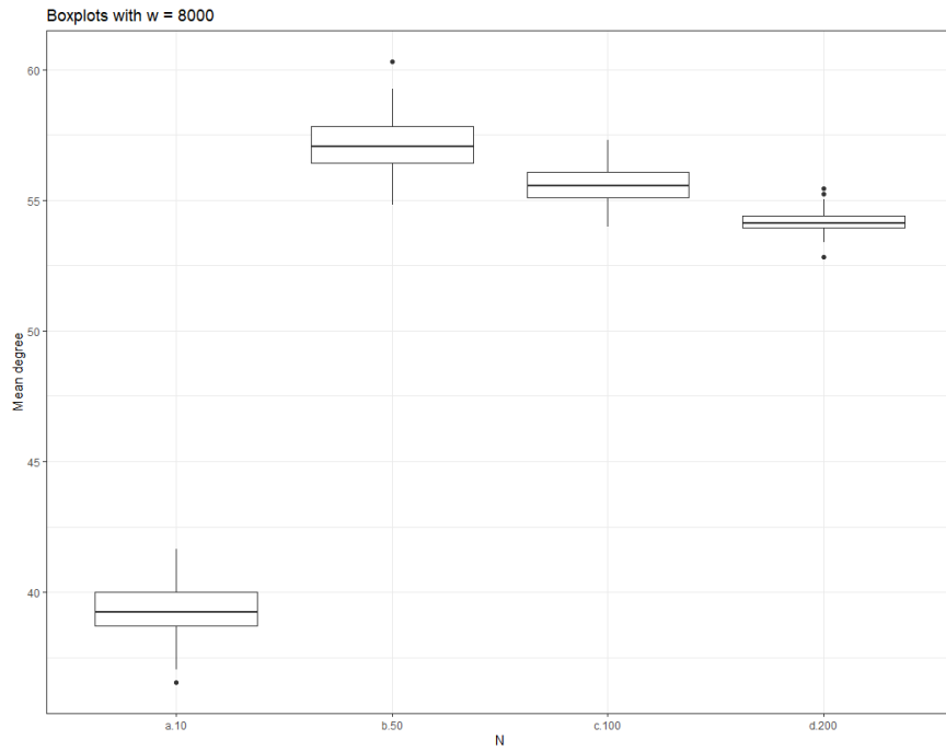
(b) Boxplots of mean degree, w = 8000
