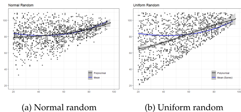
Figure 1.11: Test of randomness
