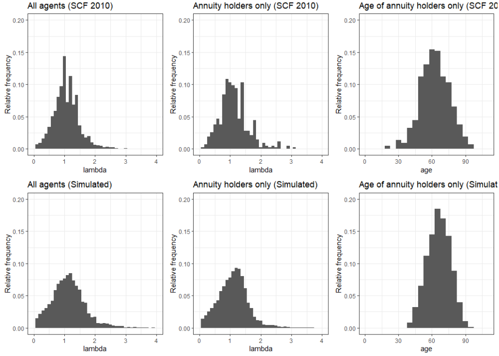
Figure 2.8: Comparison of histograms of data and simulation
