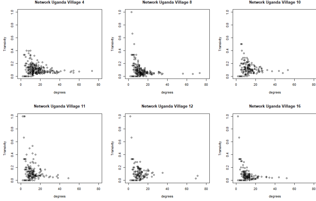
Figure 4.5: Plot of local clustering coefficient against degree for each node in the six Ugandan village networks depicted in Figure 4.3.
