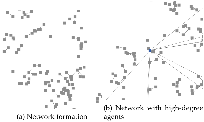
Figure 1.5: Agents and network links illustration on two-dimensional plane
