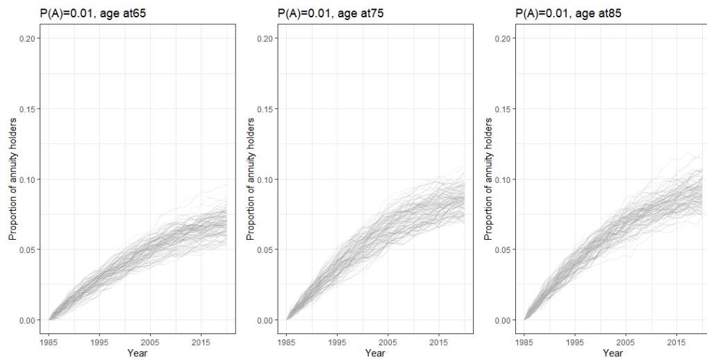
Figure 3.13: Changes in annuity purchase age limit
