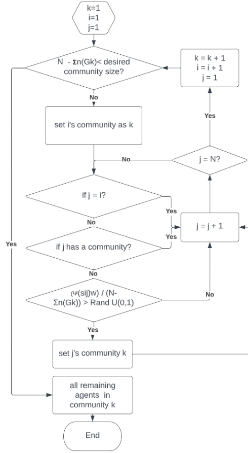
Figure 4.6: Community matching algorithm
