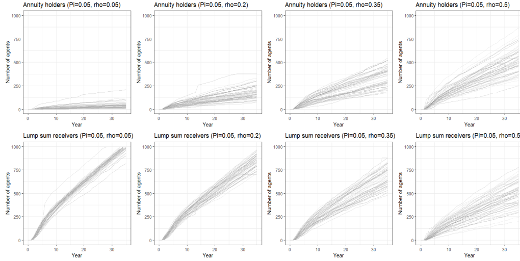
Figure 5.4: Number of annuity holders and lump sum receivers from 50 simulations with \Pi = 0.05 and \rho = (0.05, 0.2, 0.35, 0.5)
