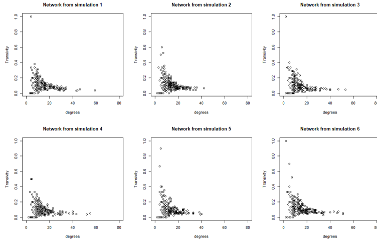
Figure 4.13: Local clustering coefficient for degrees of nodes from simulations
