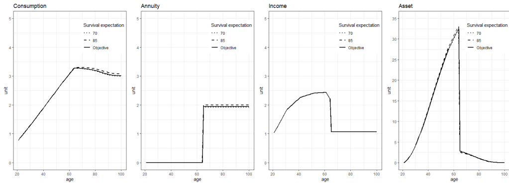
(b) Life-cycle model using subjective survival probabilities with \omega_i
