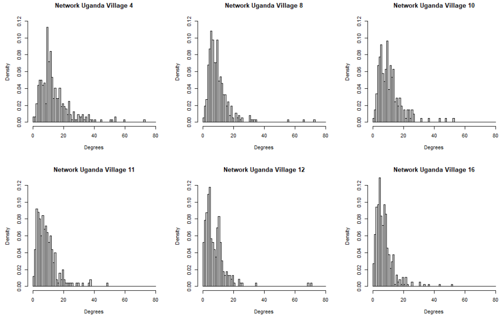
Figure 4.4: Ugandan village degree distribution. (Source: Chami et al. (2017))
