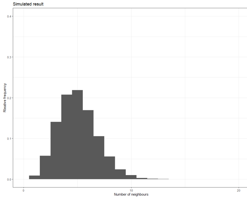
(a) Distribution of the number of network neighbours of each agent
