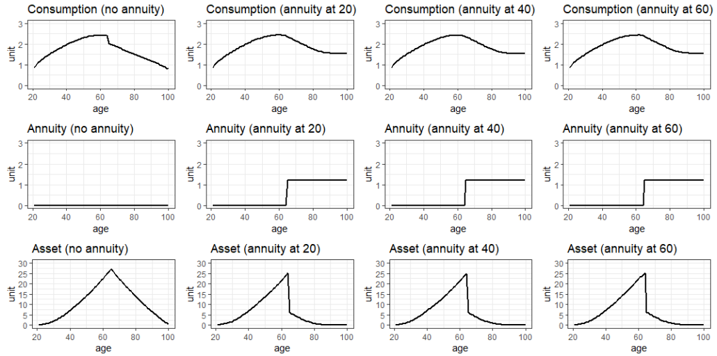
Figure 3.8: Changes in consumption annuity and wealth by annuity decision age
