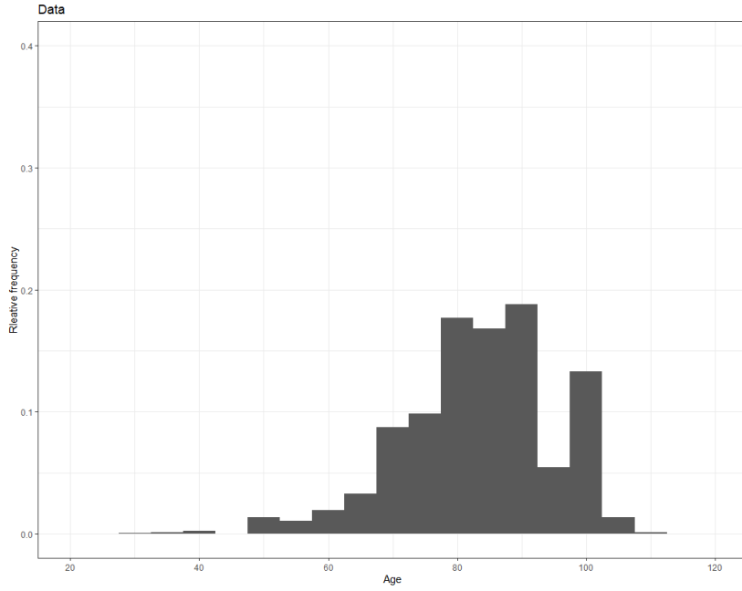
(a) Histogram from the data
