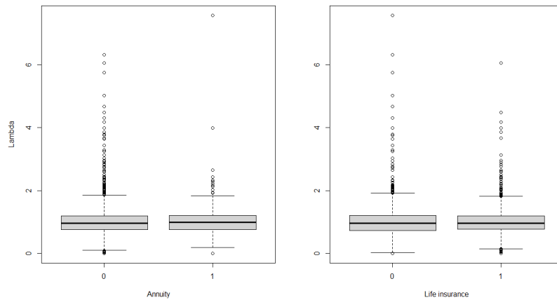
Figure 2.3: Box-and-whisker plots of annuity and life insurance-holder by calculated \lambda_i . (Source: The SCF, 2010)
