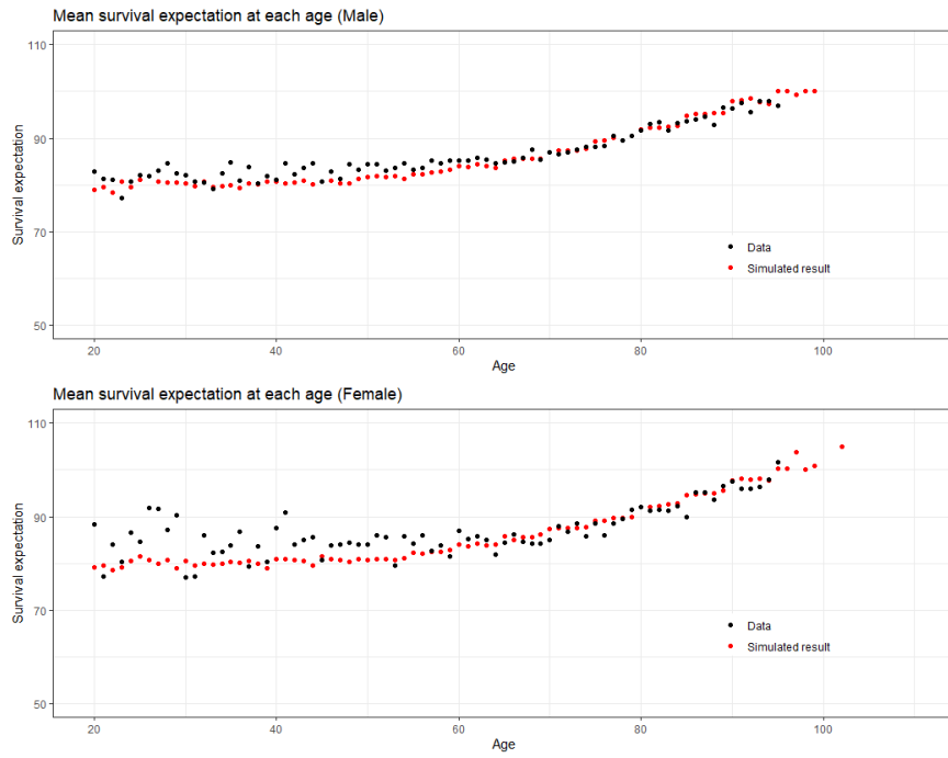
(a) Mean of survival expectation(male& female)
