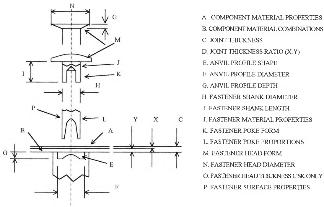
Fig 3.2 Joint Process Parameters - Static
