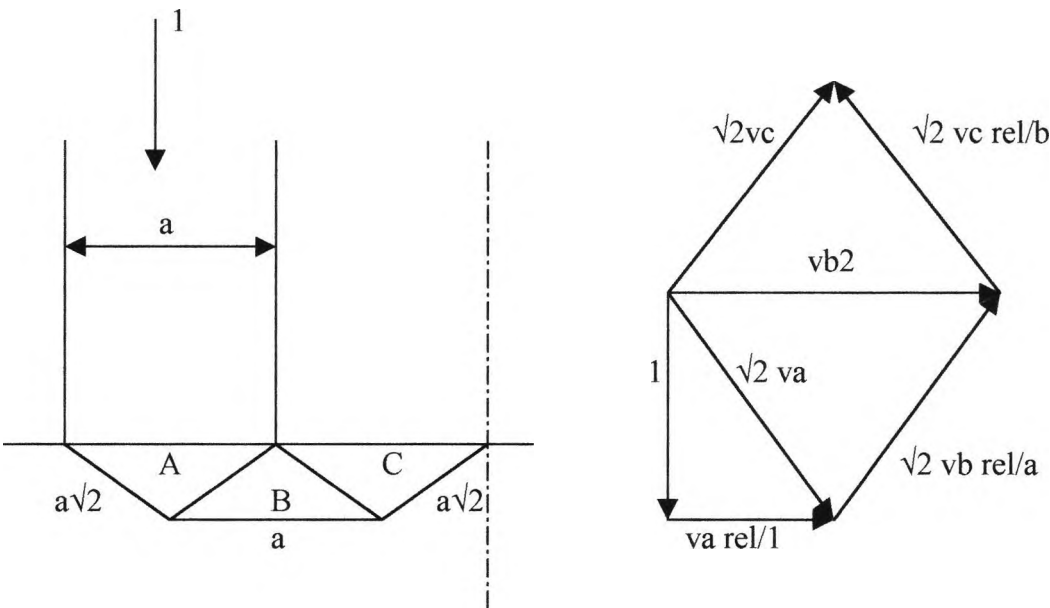
Fig 2.19 Slip Planes and Hodograph for a Self Pierce Rivet
