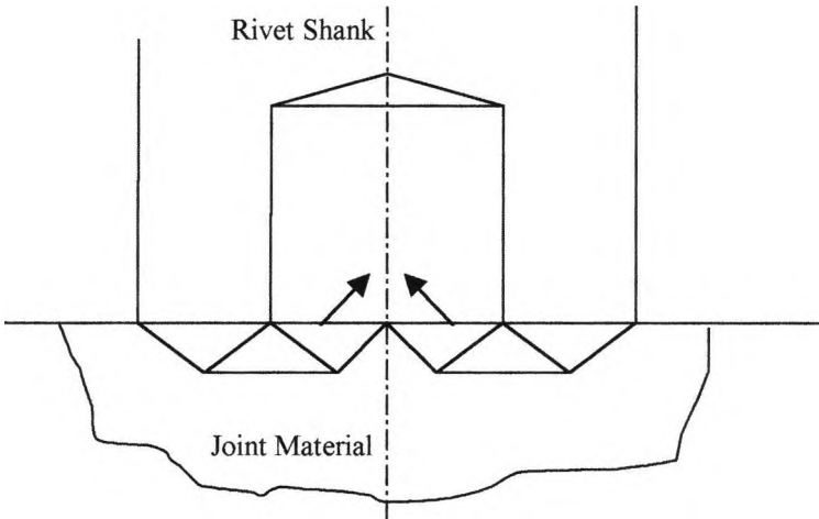
Fig 2.18 Material Flow when Pierced by a Hollow Rivet
