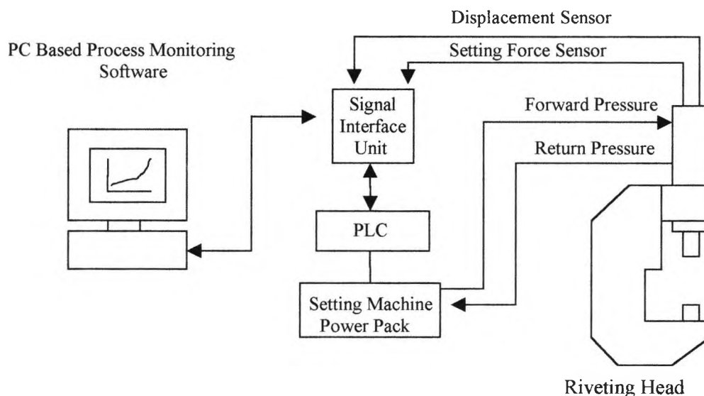
Fig 2.16 Process Monitoring System (King et. al 1996a)
