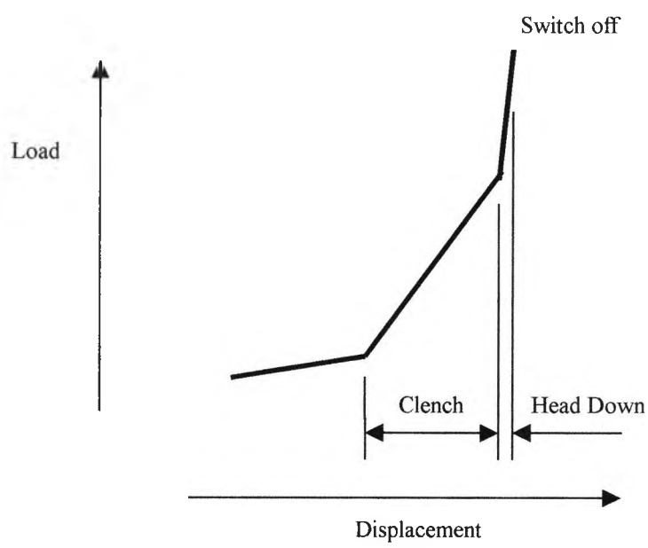
Fig 3.13 Final Phases of Joint Formation
