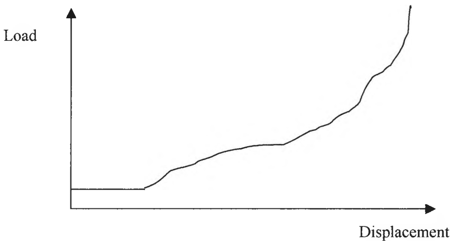
Fig 2.15 Typical Load v Displacement Curve for the Self pierce Riveting Process
