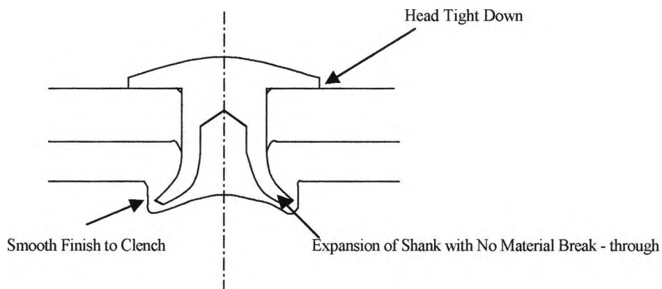
Fig 3.4 Joint Appearance Factors
