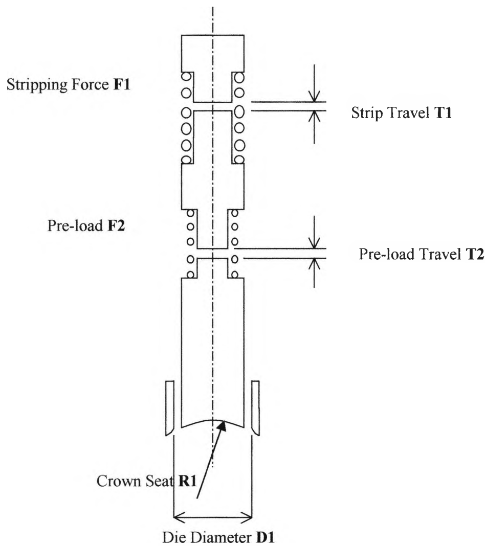
Fig 5.7 Crowning Technology Parameters
