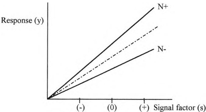
Fig 2.12 Dynamic system subject to noise (Grove & Davis)
