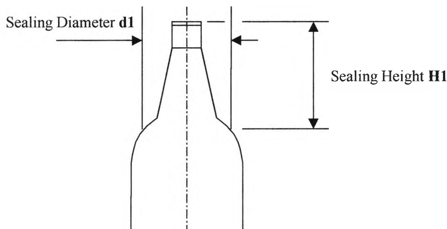
Fig 5.8 Bottle Sealing Dimensions
