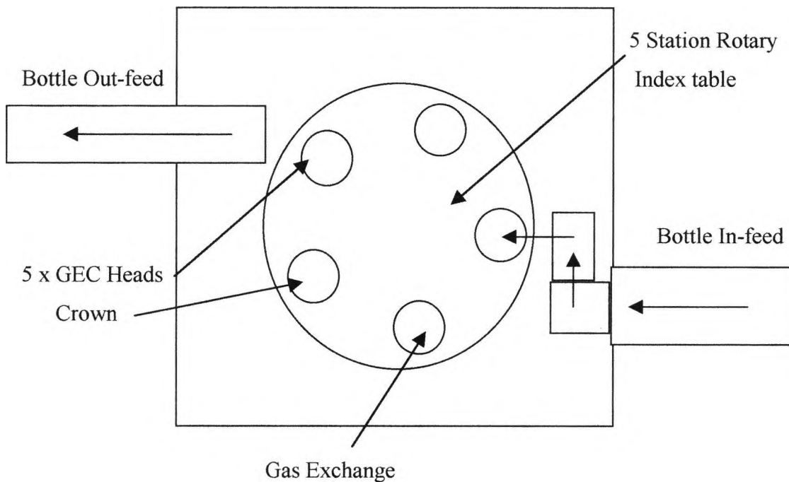
Fig 5.11 Pilot Production Test Machine (Plan View)
