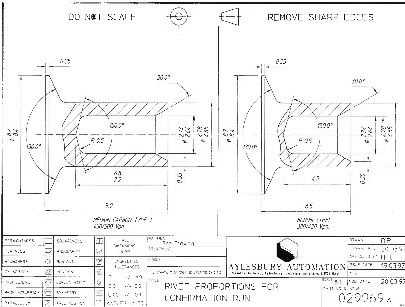
Fig 4.9 Proposed Rivet Design
