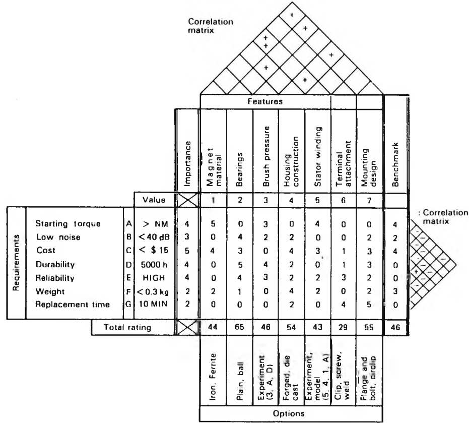
Fig 1.10 QFD Chart for an Electric Motor (O'Connor 1991)
