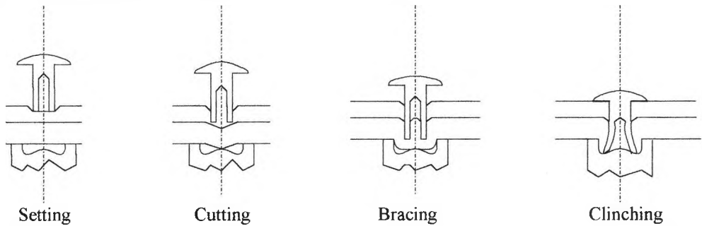
Fig 1.20 Stages of Joint Formation
