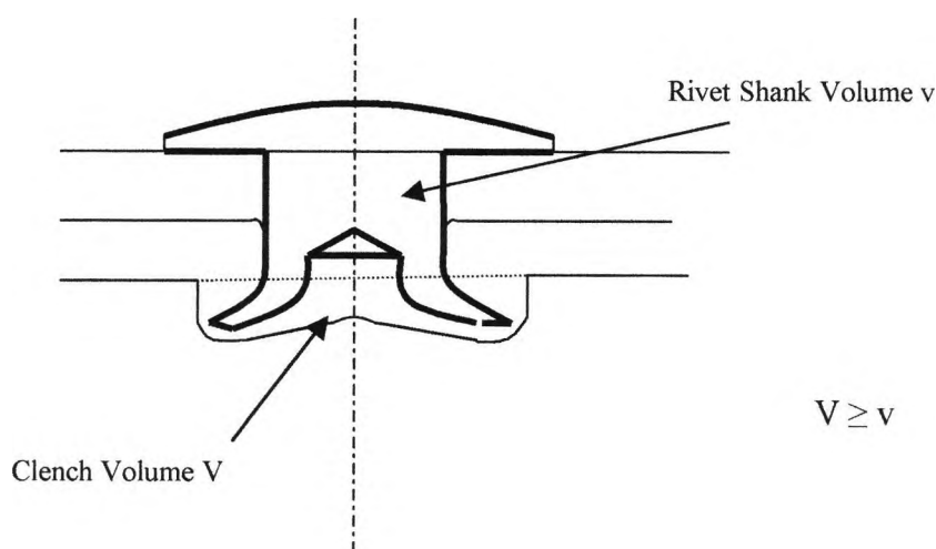
Fig 3.12 Joint Material and Rivet Volume Balance
