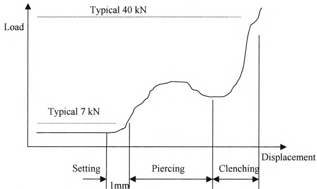
Fig 2.21 Load v Displacement Curve for Steel (type CR4)
