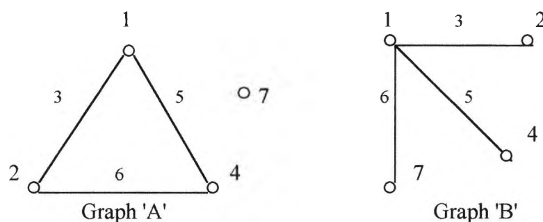
Fig 1.15 Linear Graphs for the L_4 Array
