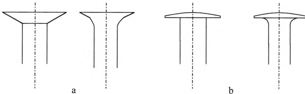
Fig 3.7 Under-Head Radius
