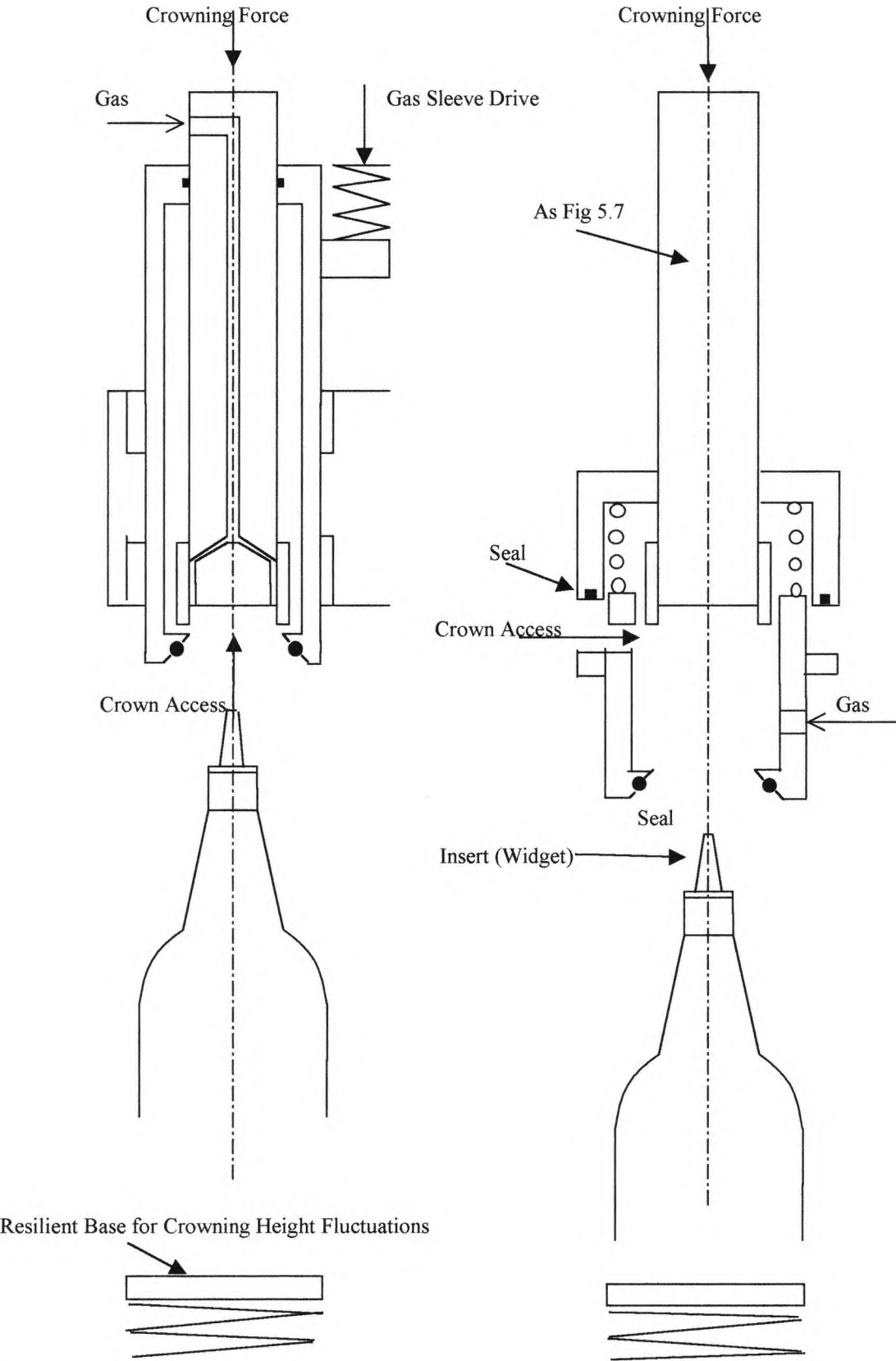
Fig 5.9 GEC Head Design Proposals
