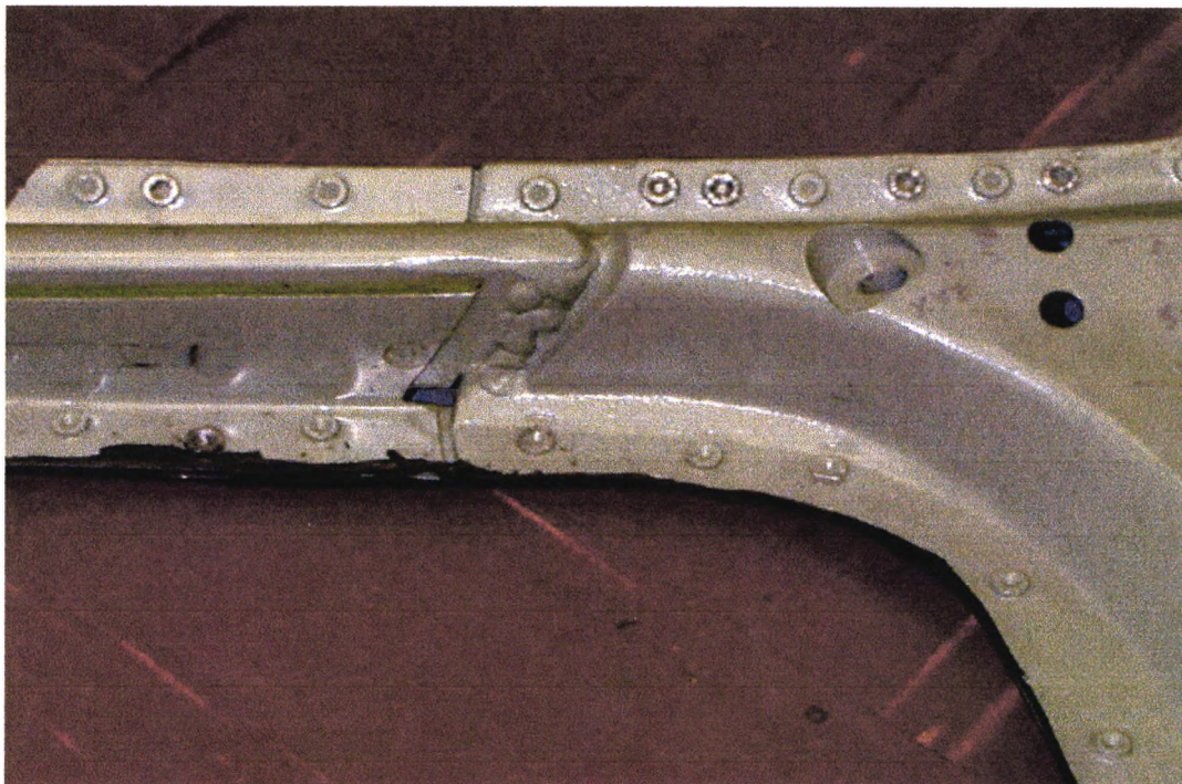
Fig 4.10 Ferrari F131 Riveted Joints
