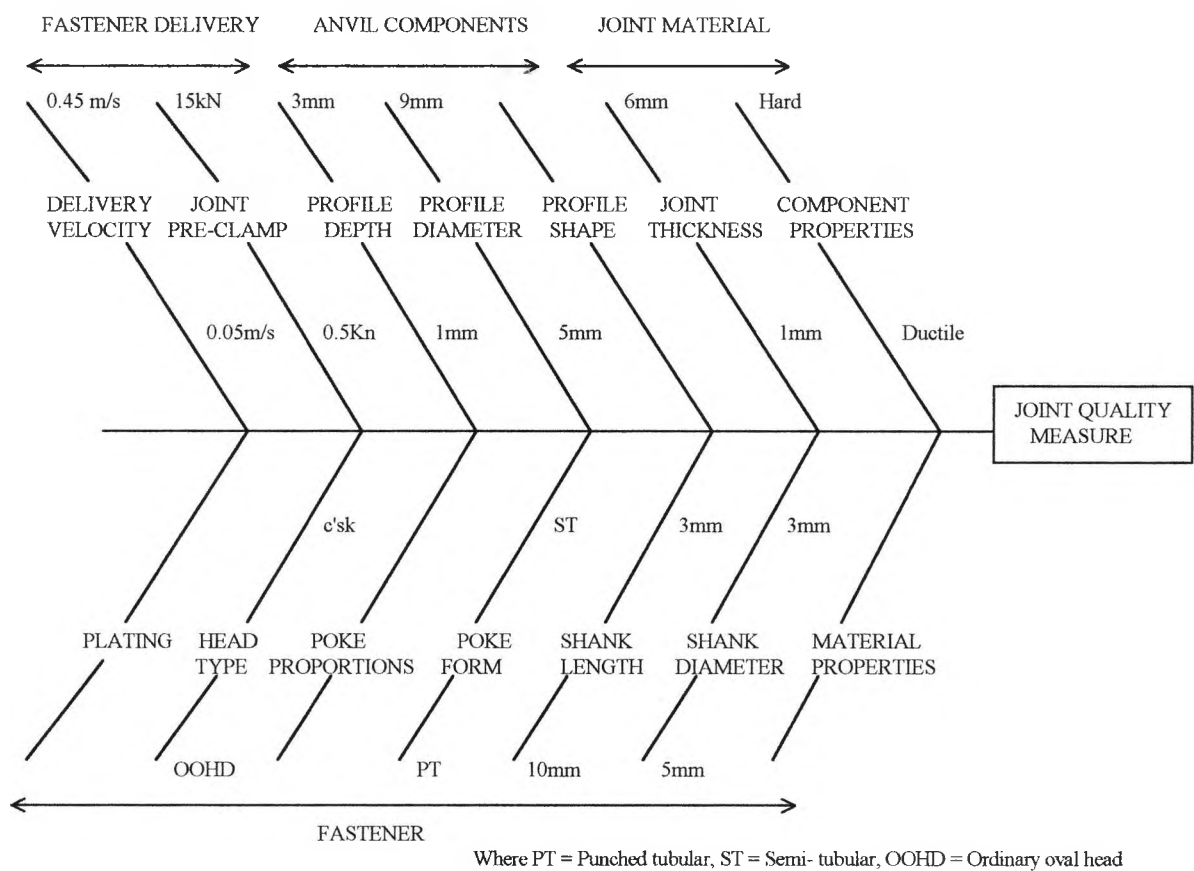
Fig 3.3 Primary Cause and Effect Diagram
