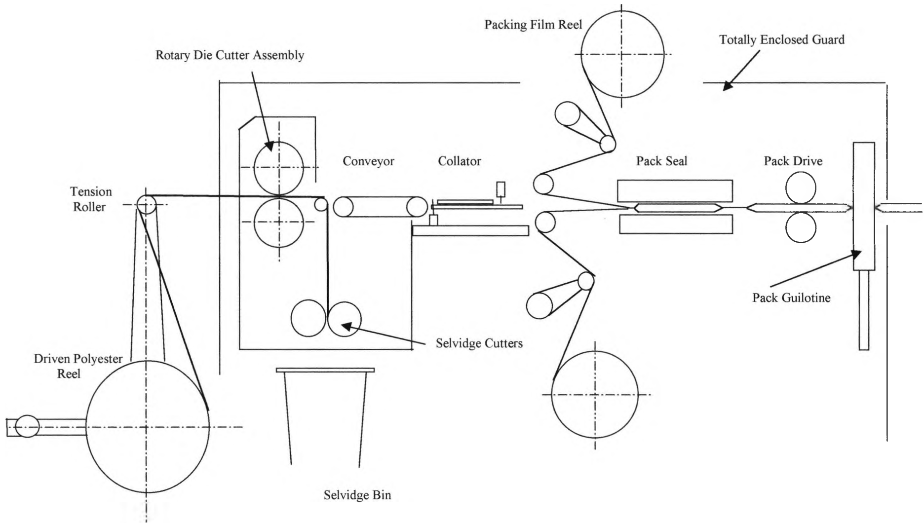
Fig 5.6 Visor Shields Production Machine
