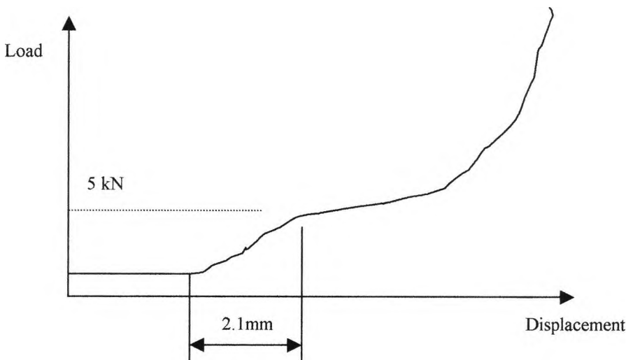
Fig 3.11 Typical Load v Displacement Curve for Alternative Form Rivets
