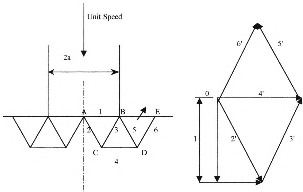
Fig 2.17 Simple indentation, Flow Diagram and Hodograph (Johnson & Mellor 1983)
