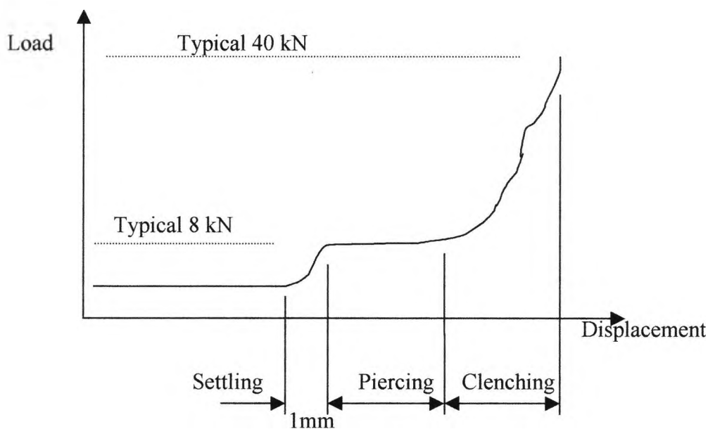
Fig 2.20 Load v Displacement Curve for Aluminium Alloy (type 5251-H3)
