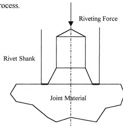
Fig 3.8 Alternative Form Rivet
