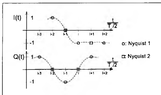
Fig. 4. I- and Q-channel signals at the receiver filter output which satisfy Nyquist criteria 1 and 2.
