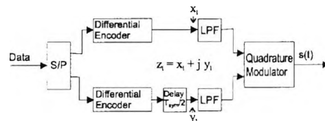
Fig.1 DOQPSK Transmitter Model
