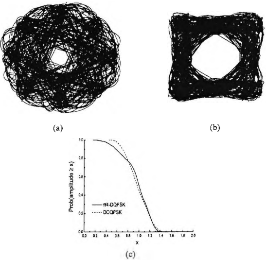
Figure 3: Complex phase plots of (a) \pi/4 -QPSK and (b) OQPSK with a square root raised cosine Nyquist filter ( r = 0.35 ); (c) Inverse amplitude distribution
