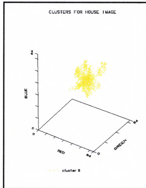
Figure 4.26 Cluster 8
