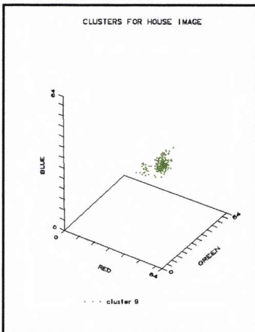
Figure 4.27 Cluster 9
