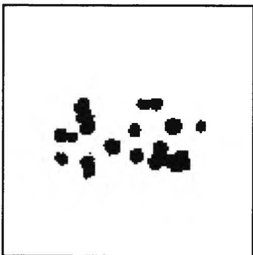
Figure 4.36 Red Regions
