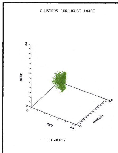
Figure 4.20 Cluster 2
