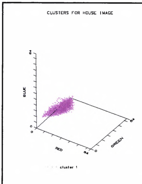
Figure 4.19 Cluster 1
