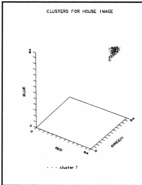
Figure 4.25 Cluster 7
