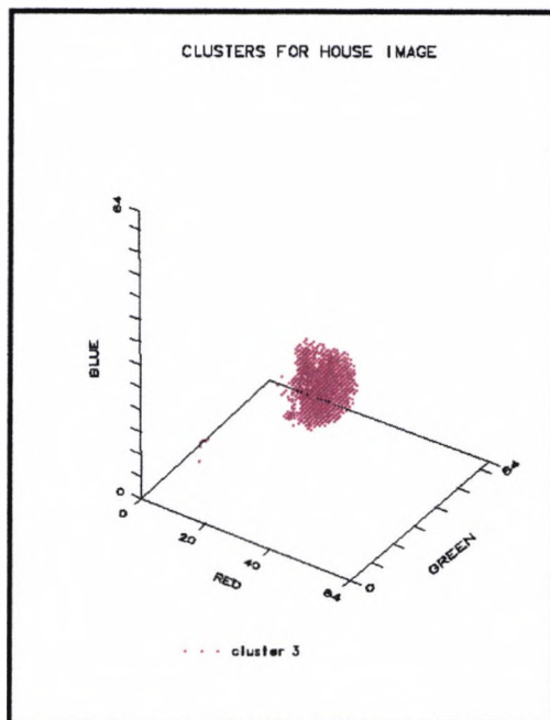
Figure 4.21 Cluster 3
