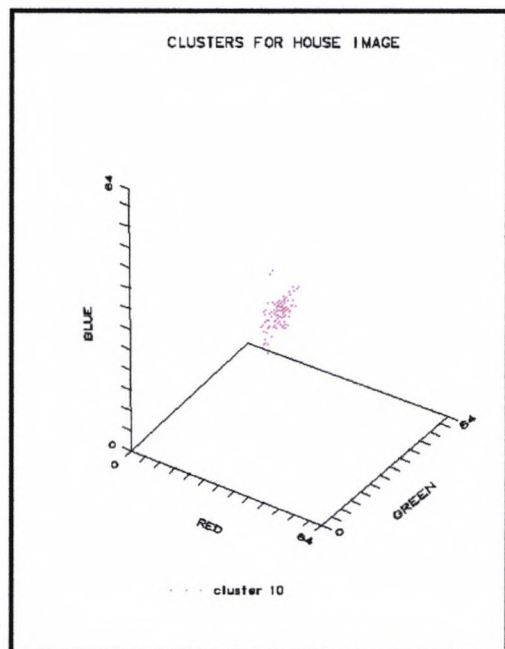
Figure 4.28 Cluster 10
