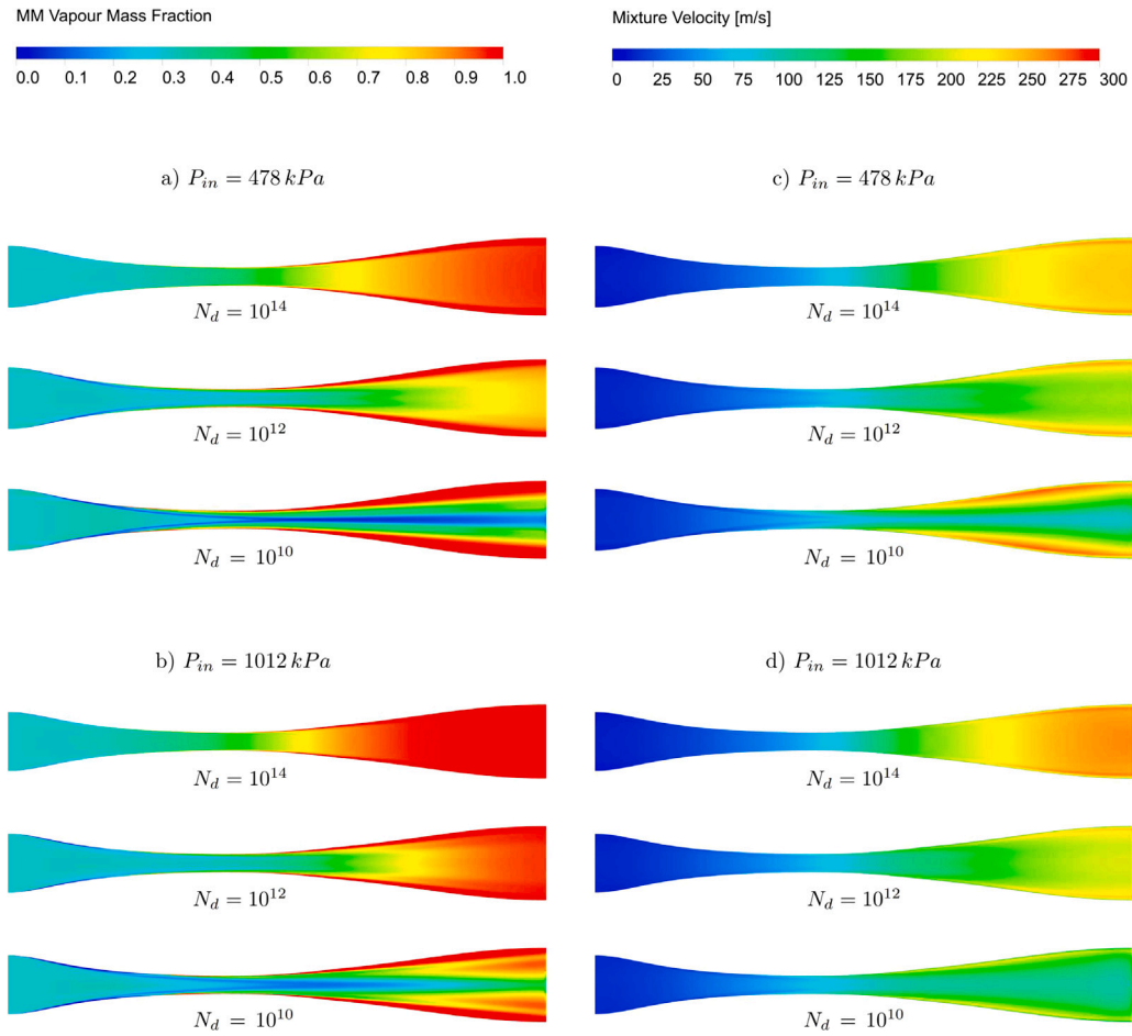
Fig. 14. Two-dimensional variations of vapour mass fraction and mixture velocity within the nozzle.
