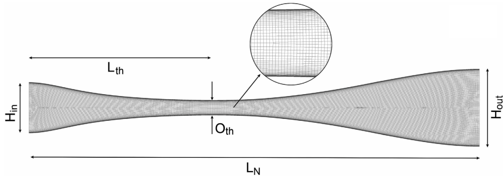
Fig. 5. Nozzle geometry for the expansion from 478 kPa and inlet quality of 0.3; the figure also illustrates the type of mesh used in the simulations — similar mesh was constructed for all other geometries.
