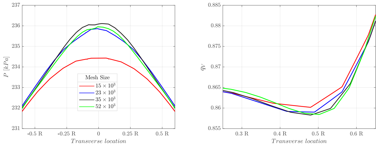
Fig. 6. Dependence of transverse profiles of static pressure P and vapour quality q_v on the mesh resolution; the profiles were taken approximately midway between the throat and the outlet and were capped to illustrate only the regions where the parameters were sensitive to mesh resolution.
