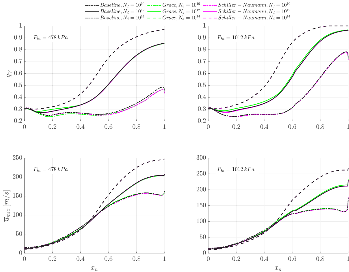
Fig. 7. Streamwise variation of average vapour mass fraction \bar{q}_V and average mixture velocity \bar{u}_{mix} obtained using alternative interphase drag models. The plot shows two expansion cases: the expansion from 478 and 1012 kPa with inlet quality of 0.3.
