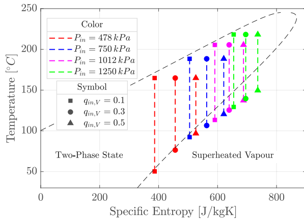
Fig. 4. The temperature-entropy diagram of the twelve simulated expansion cases; the depicted expansions define the boundary conditions used in the nozzle design and CFD simulations, and are generated under the assumption of isentropic homogeneous-equilibrium flow.
