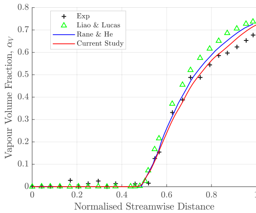
Fig. 2. The variation of static pressure and vapour volume fraction along the centre line of the BNL nozzle; comparison between the current study, other numerical studies and the experimental measurements.
