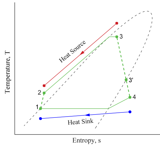
Fig. 1. Temperature-entropy diagram of the wet-to-dry cycle.
