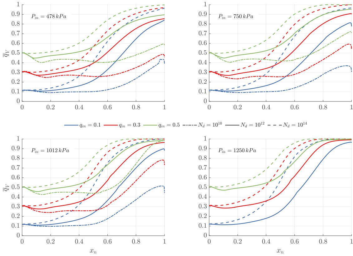
Fig. 9. Streamwise variation of average vapour mass fraction \bar{q}_v for twelve wet-to-dry expansions from four different inlet pressures P_{in} : 478, 750, 1012 and 1250 kPa, and from three different vapour inlet qualities: 0.1, 0.3 and 0.5. The variation of \bar{q}_v for each expansion case has been shown for three different droplet density numbers N_d : 10^{10} , 10^{12} and 10^{14} .
