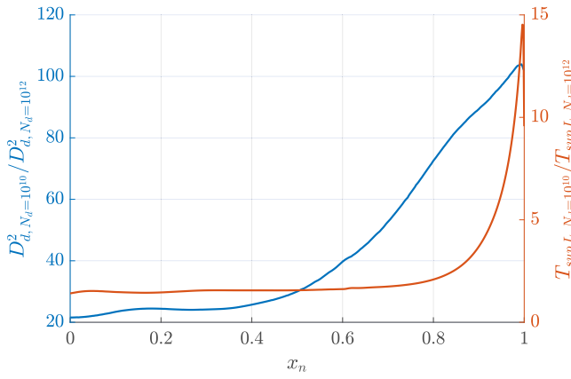
Fig. 11. Streamwise variation of the ratios of droplet diameter square and liquid superheat; the lines represent the ratios of the values obtained with N_d = 10^{10} to the values obtained with N_d = 10^{12} for the expansion from 1012 kPa and inlet quality of 0.3.
