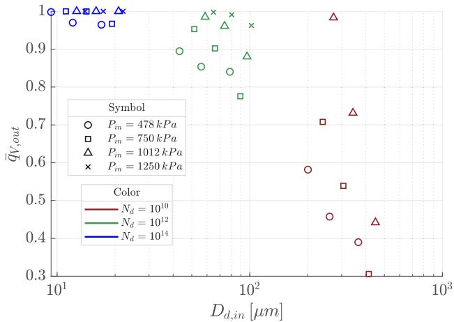
Fig. 10. The relationship between average outlet vapour quality \bar{q}_v and inlet droplet diameter D_{d,in} for all the simulated expansion cases and droplet density numbers; for a given P_{in} - N_d pair, smaller droplets correspond to higher inlet quality.
