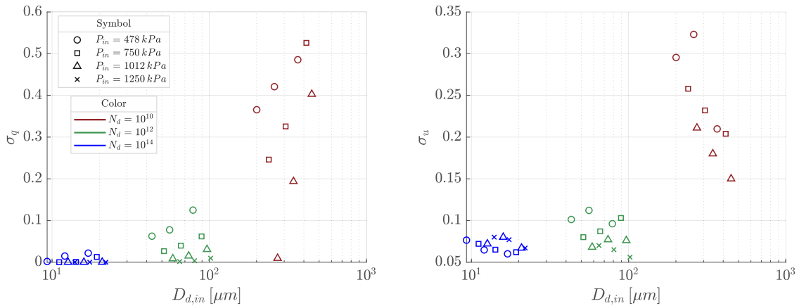
Fig. 15. The relationship between the inlet droplet diameter and normalised standard deviations of vapour mass fraction ( \sigma_q ) and mixture velocity ( \sigma_u ) across the nozzle outlet; the standard deviations were normalised by mean outlet values of q_v and u_{mix} .
