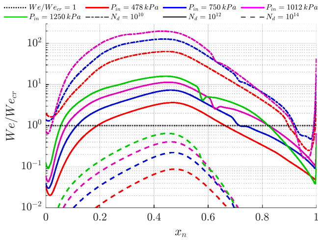
Fig. 16. The streamwise variation of the ratio of the average Weber number to the critical Weber number; droplet breakup is expected to occur if the ratio We/We_{cr} exceeds unity. The mixture was expanded from inlet quality of 0.3 for each presented case.
