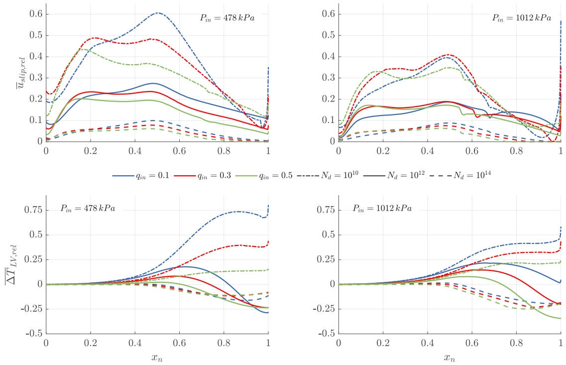
Fig. 13. Streamwise variation of average relative velocity \bar{u}_{slip,rel} and average relative thermal non-equilibrium \bar{\Delta T}_{LV,rel} in the expansions from 478 kPa and 1012 kPa, with three inlet qualities q_{V,in} of 0.1, 0.3 and 0.5 and three different droplet density numbers N_d of 10^{10} , 10^{12} and 10^{14} ; \bar{u}_{slip,rel} is the velocity slip normalized by the mixture velocity, while \bar{\Delta T}_{LV,rel} is temperature difference between the phases normalised by the saturation temperature.
