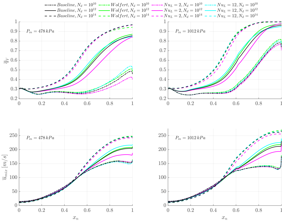
Fig. 8. Streamwise variation of average vapour mass fraction \bar{q}_v and average mixture velocity \bar{u}_{mix} obtained using alternative heat-transfer coefficient models. The plot shows two expansion cases: the expansion from 478 and 1012 kPa with an inlet quality of 0.3.
