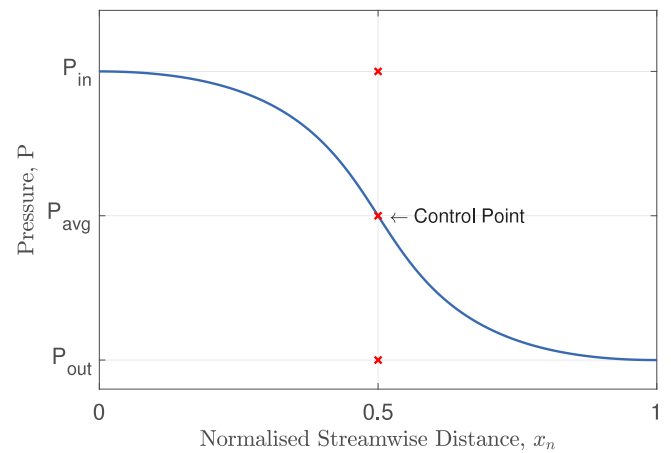
Fig. 3. The imposed pressure profile constructed using a Bezier curve with three control points.
