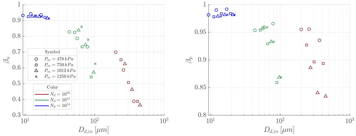
Fig. 12. The relationship between the inlet droplet diameter D_{d,in} and the \beta parameters; \beta_p is the ratio of the pressure drop to the design pressure drop, while \beta_u is the ratio of the mixture outlet velocity to the design outlet velocity.
