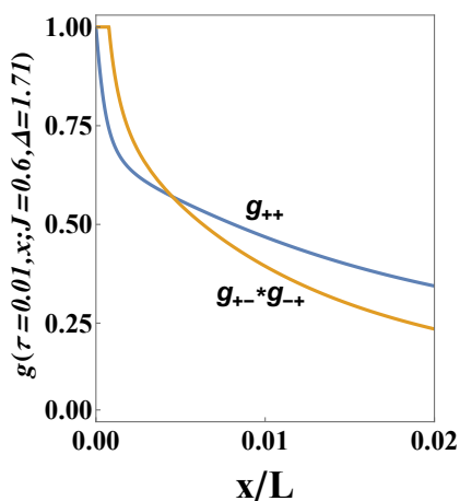
FIG. 1. Decay in space of Green's functions g_{++}(z, \bar{z}) and g_{+-}(z, \bar{z}) * g_{-+}(z, \bar{z}) \equiv g_{\cap}(z, \bar{z})g_{\cup}(z, \bar{z}) , used to compute the free energy ( \cap \equiv +- , while \cup \equiv -+ ), at almost equal time \tau - \tau' = 0.01 . The figure shows them for the specific fixed values \Delta = 1.71 , \tau \equiv u_0(\tau - \tau')/L = 0.01 and J \equiv J/\pi u_0 = 0.6 , in the gapped regime. g_{+-}(z, \bar{z}) * g_{-+}(z, \bar{z}) has been chopped close to x - x' \sim 0 .
