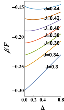
FIG. 3. Blow-up of the appearance of the absolute minimum of the free energy \beta F at \Delta \geq 0 , which develops continuously at \Delta > 0 for increasing coupling J \equiv J/(\pi u_0) > 0.4 .
