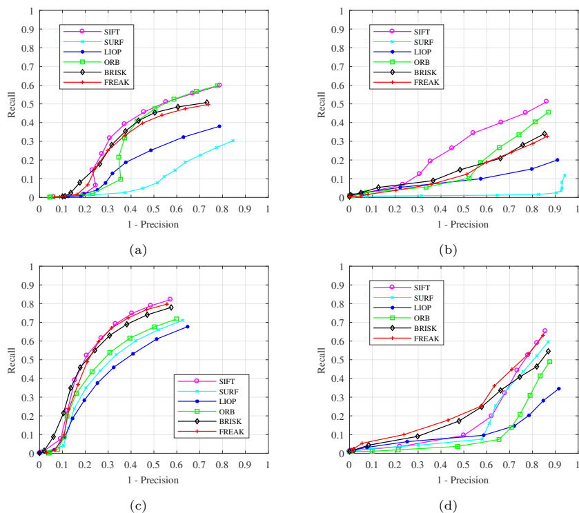
Figure 21: Descriptor ROC curves for the visible band, cold case. (a, b) DoG features with small and large transformations. (c, d) Fast-Hessian features with small and large transformations.
