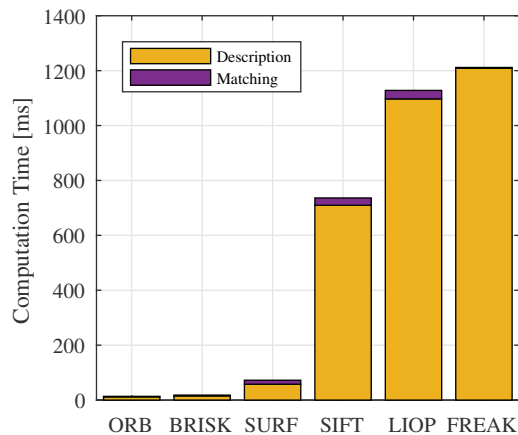
Figure 25: Comparison of average feature description and matching times per frame.
