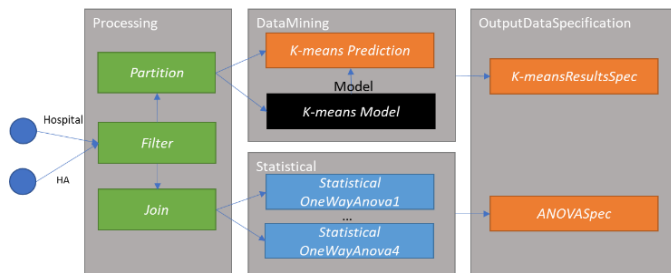
Fig 11: The Workflows as implemented in BDA.
