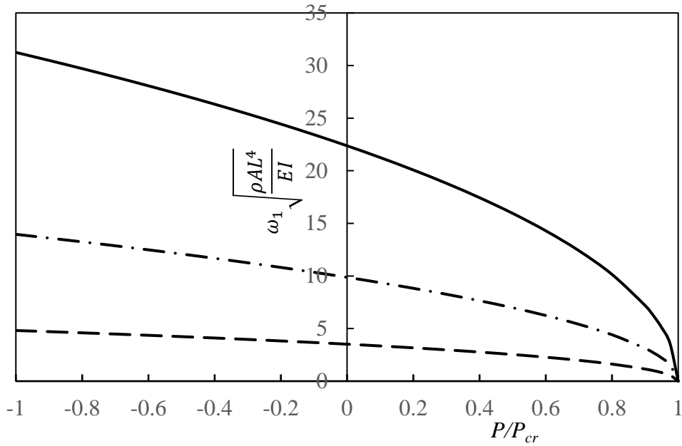
Fig. 3. The effect of axial load on the fundamental natural frequency of a Bernoulli Euler beam for different boundary conditions. — CC; - · - · - · PP; - - - - CF
