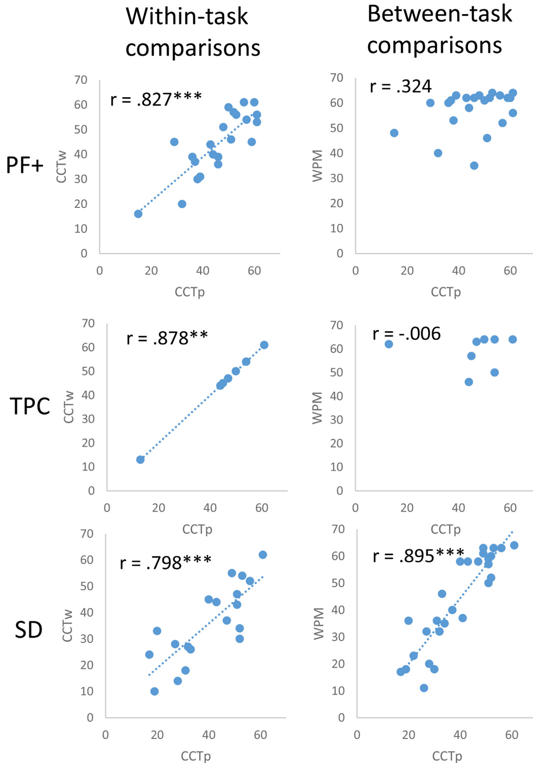
Fig. 2 – Correlations between and within tasks per group. CCTp = picture Gamel and Cactus test; CCTw = word Gamel and Cactus test; WPM = word-picture matching.
