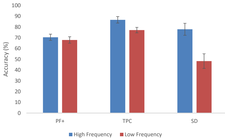
Fig. 3 – The impact of frequency on accuracy across groups. Error bars show standard error of mean.
