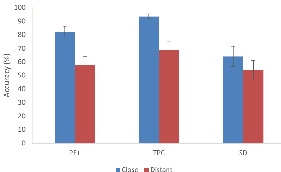
Fig. 5 – The impact of semantic distance on performance across groups. Error bars show standard error of mean.
