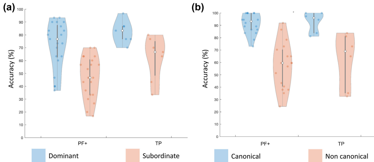
Fig. 6 – The impact of semantic control manipulations on (a) retrieval of dominant and subordinate meaning of ambiguous words, and (b) canonical and non-canonical use of objects. The white dot in these violin plots shows the median, with the line representing the interquartile range, and individual participants shown in red/blue dots, surrounded by kernel density.
