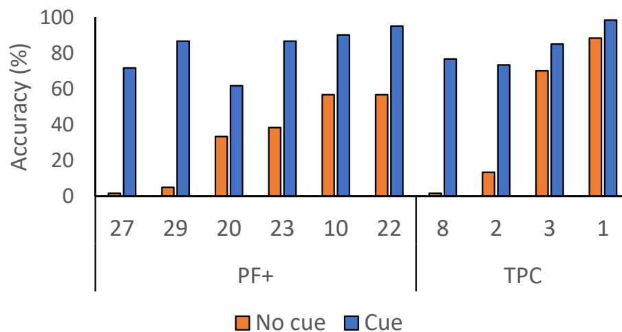
Fig. 4 – The impact of cueing on picture naming.
