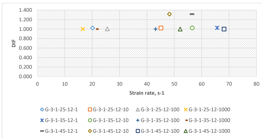
Figure 168: DIF as a function of strain rate.
