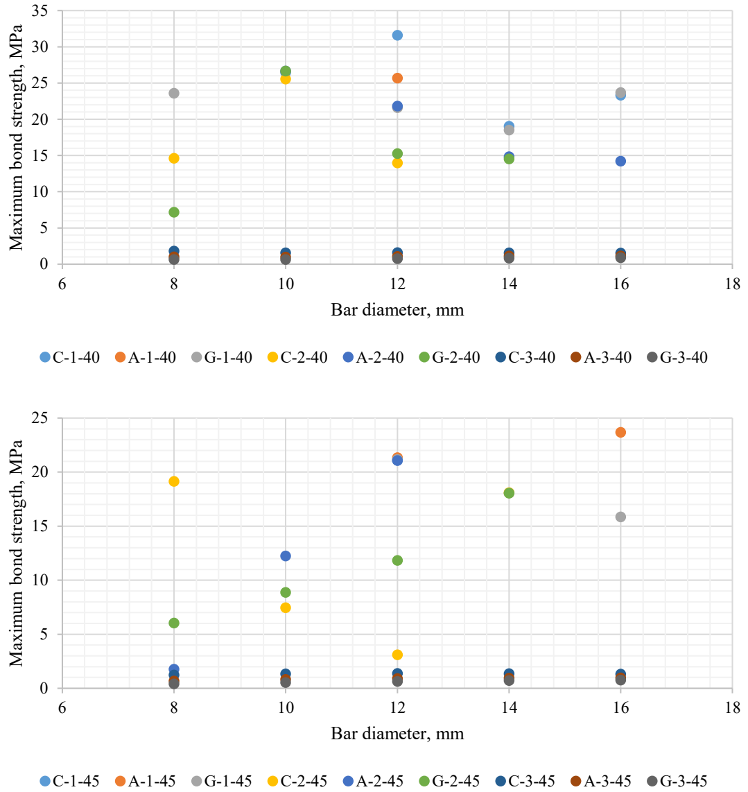
Figure 83: Maximum average bond strength versus bar diameters of models with similar concrete compressive strength.
