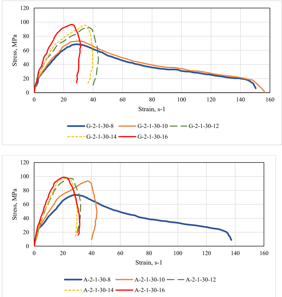
Figure 113: Stress-strain of FRP RC beams response under 80kN Impact load with respect to DIF factor.
