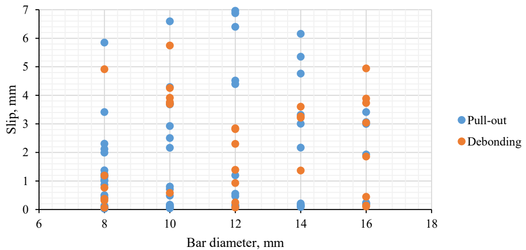
Figure 85: bond slip versus bar diameter.
