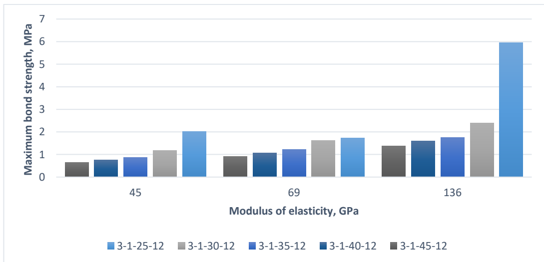
Figure 95: Effect of modulus of elasticity of FRP bars on maximum bond strength on beam models under impact loading.
