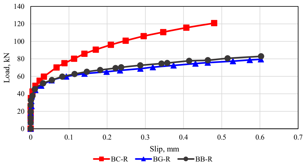
Figure 25: Load-Slip curvature for different FRP bar types in RC beams with ribbed surface from Zhang experimental test.
