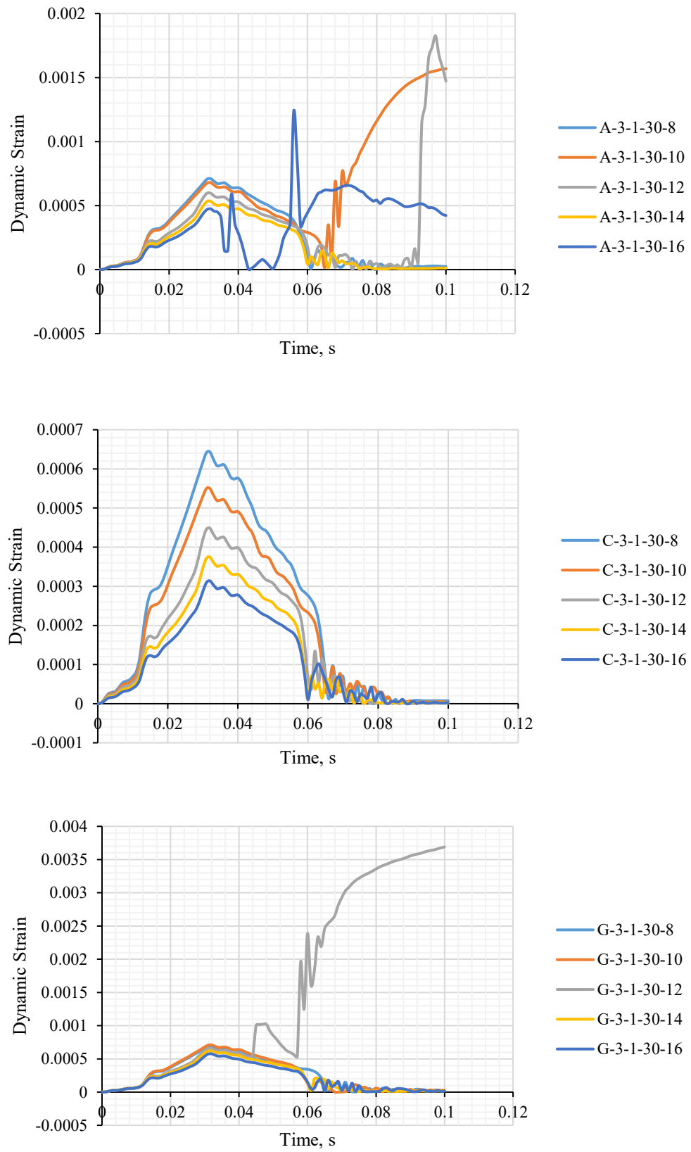
Figure 76: Dynamic strain time histories for AFRP, CFRP and GFRP RC beam models with concrete compressive strength of 30 MPa under 40 kN impact load.
