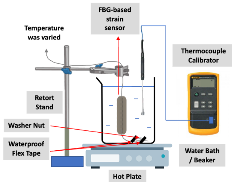
11 Fig. 6 Setup for temperature sensitivity determination for the incorporated FBG-based strain sensors (FBG- 12 PLA, FBG-TPU, FBG-PC, FBG-ABS, and FBG-Nylon)
