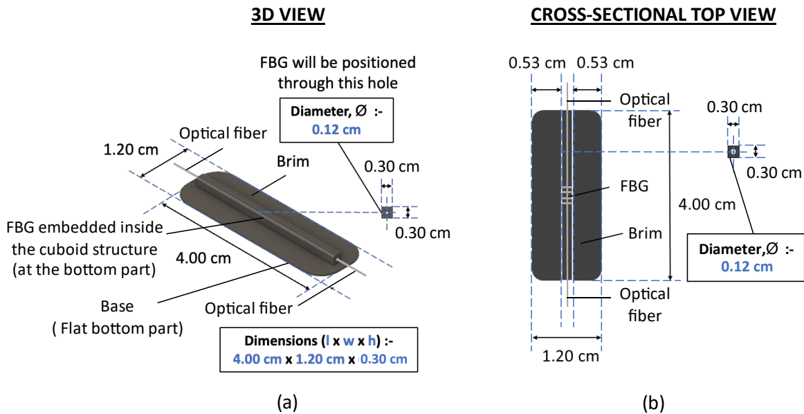
6 7 Fig. 1 Illustration of the sensor design, showing the (a) 3D view and (b) cross-sectional top view of the 8 embedded FBG-based strain sensor with dimensions. 9
