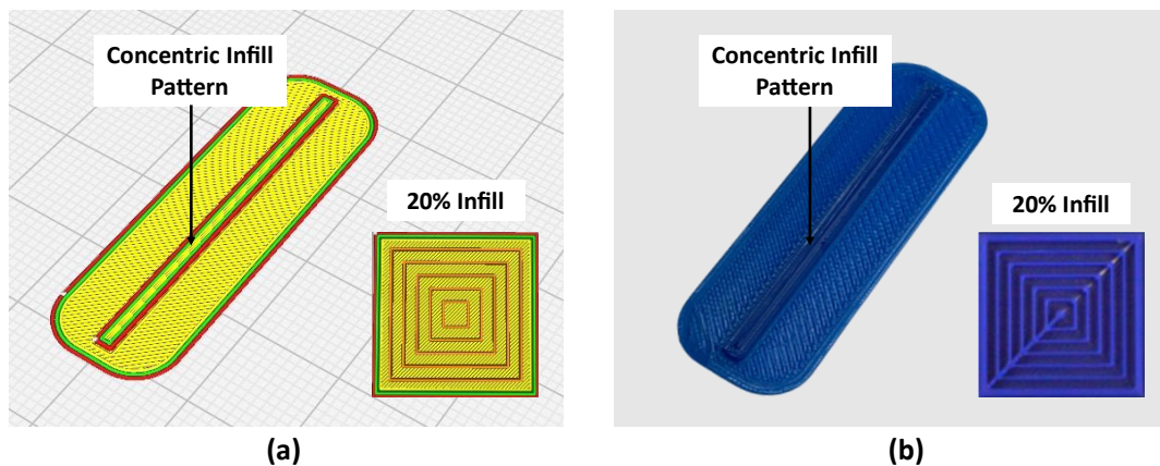
24 Fig. 3 Illustration of the layer view of the 3D printed structure, showing the 20% concentric infill pattern in 25 (a) Cura slicing software (represented by green and orange parallel lines inside the cuboid structure) and (b) 26 actual picture (represented by dark blue parallel lines inside the cuboid structure).
