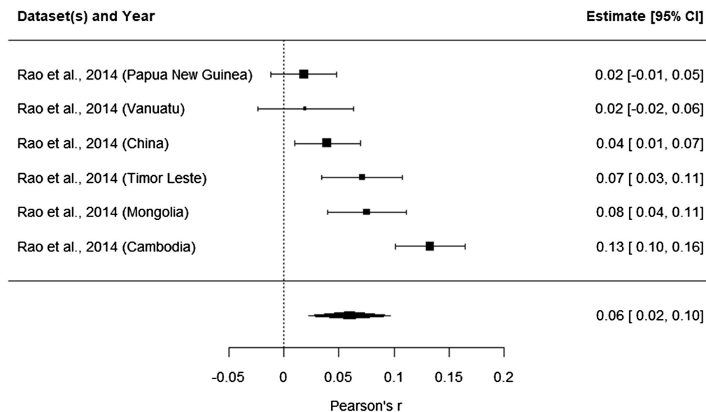
Figure 5 Forest Plot of All Effects of Interest for EAP-ECDS Multisite Framework Studies
