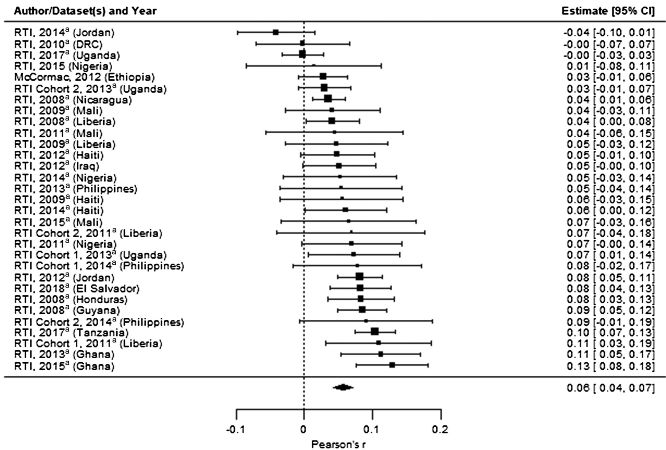
Figure 3 Forest Plot of All Effects of Interest for RTI Multisite Framework Studies
