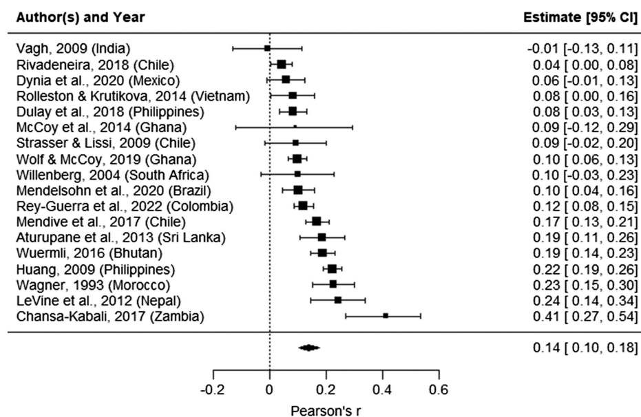
Figure 2 Forest Plot of All Effects of Interest for Customized Framework Studies
