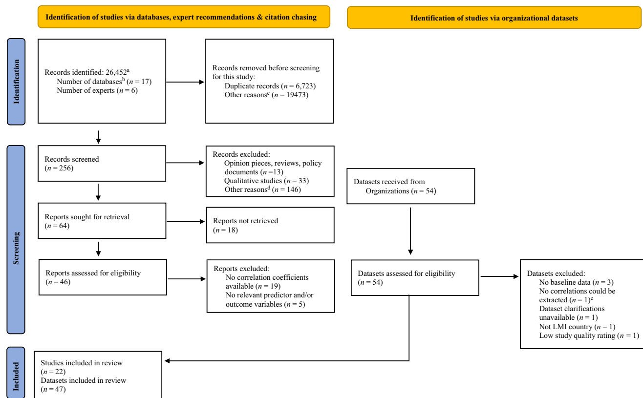
Figure 1 Flow Diagram for the Search and Inclusion of Studies
