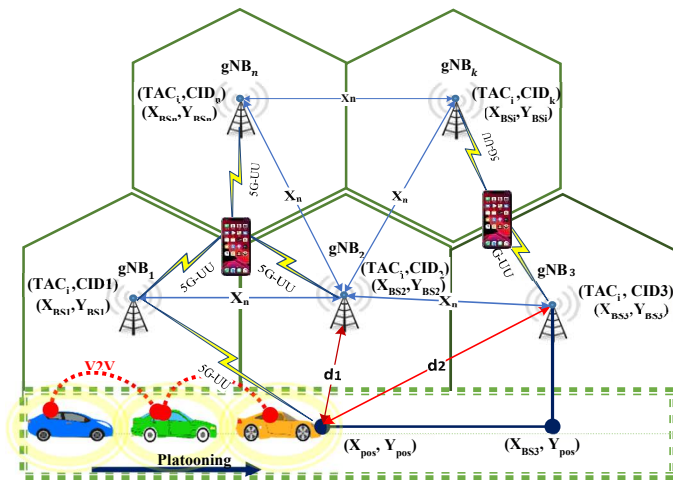
Fig. 1. Legitimate base station signal coverage. X_n : the connection between two gNB; TAC: Tracking Area Code; CID: Cell Identifier; (X_{pos}, Y_{pos}) : location of Platoon's Leader; 5GUU: 5G uplink and downlink; d : distance between base station and Leader; and, gNB: gNodeB.
