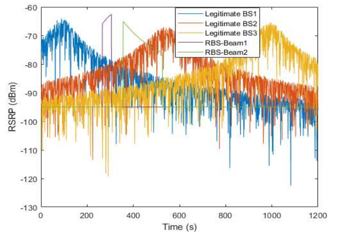
Fig. 6. Received signal strength for a mobile UE from a Rogue Base Station with two beams
