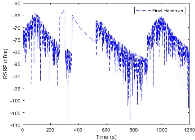
Fig. 7. Received signal strength for a mobile UE after the handover protocol in the attack model
