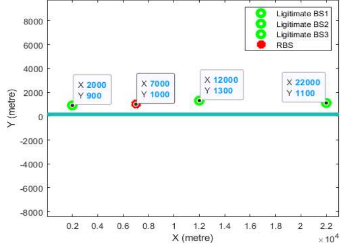
Fig. 2. The simulation geography, motorway width=300 metres, motorway length= 23000 metres
