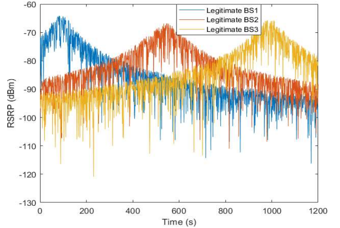
Fig. 3. Received signal strength for a mobile UE from several standalone legitimate base stations
