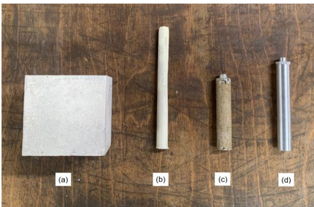
Figure 3. Samples used for roughness parameter comparison (a) concrete block (b) resin cast pile (c) sand coated pile (d) smooth aluminium pile.
