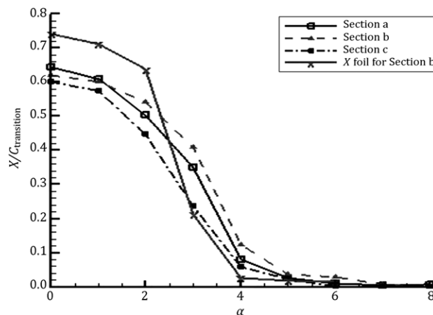
Figure 7: Comparison of the transition point from the skewness data for three sections; V_\infty = 50 m/s.
