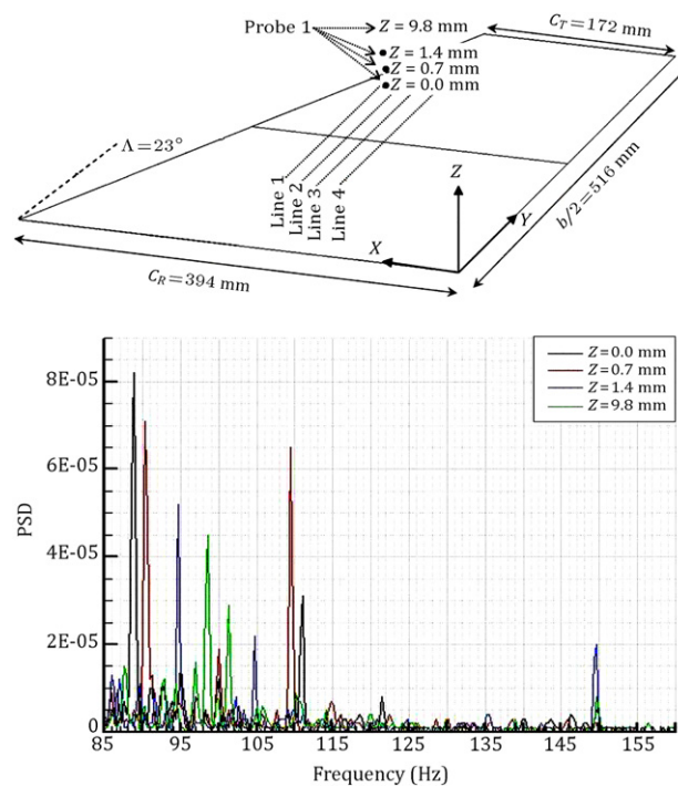
Figure 8: Comparison of the measurement signals at position 1 for different Z locations; \alpha = 0^\circ , V_\infty = 50 m/s.
